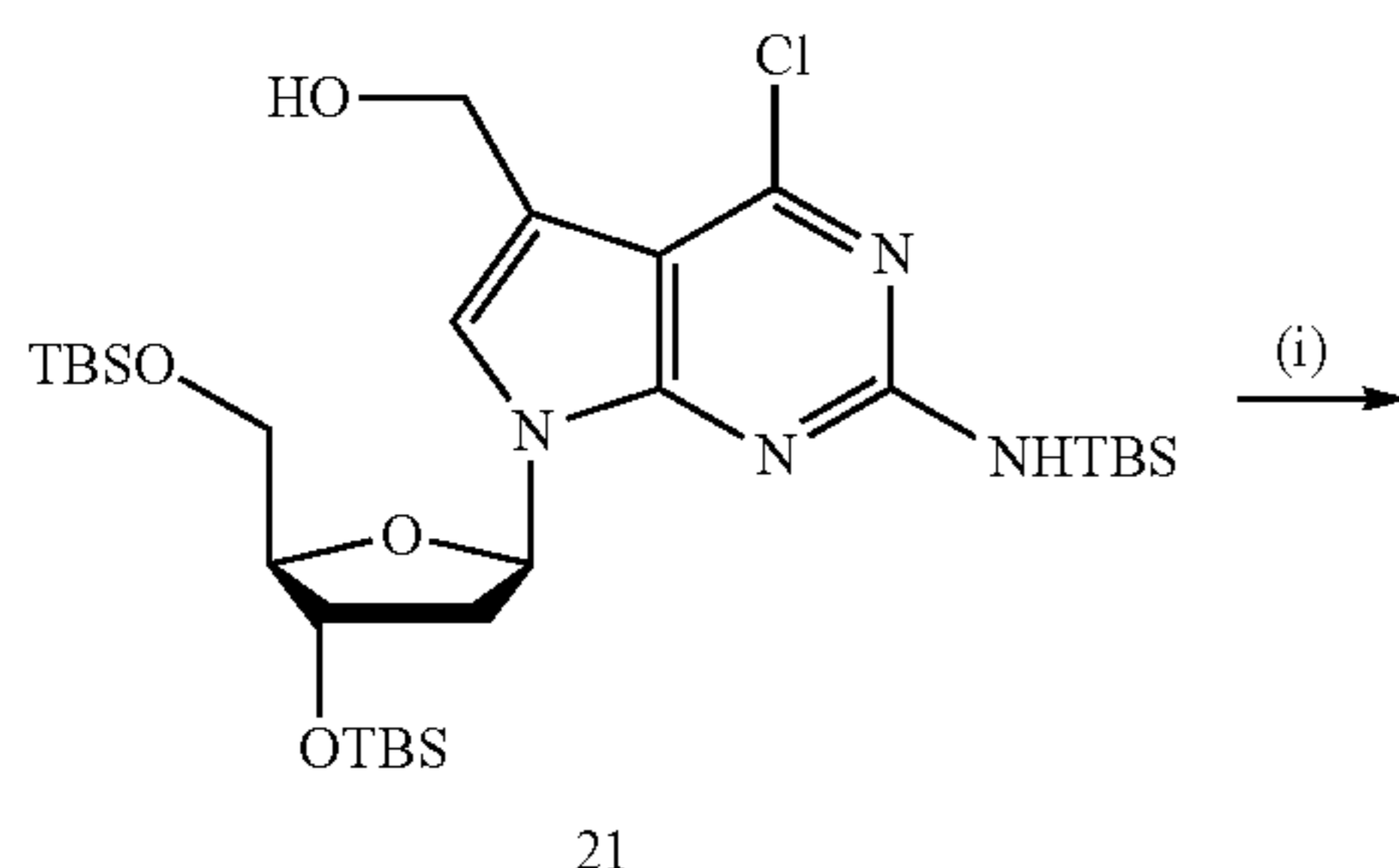
Scheme S16. Synthesis of 7-[1-(5-methoxy-2-nitrophenyl)-2,2-dimethyl-propyloxy]methyl-7-deaza-2'-deoxyguanosine-5'-triphosphate.
