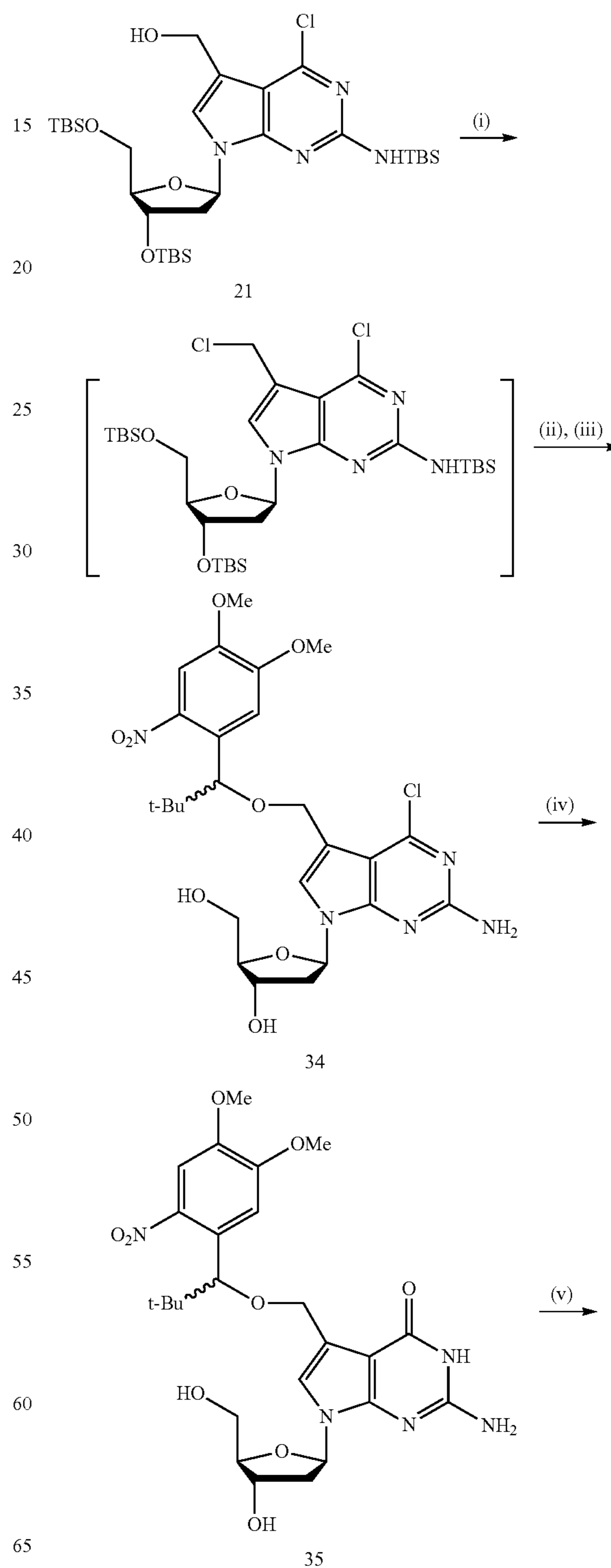
Scheme S17. Synthesis of 7-[1-(4,5-dimethoxy-2-nitrophenyl)-2,2-dimethyl-propyloxy]methyl-7-deaza-2'-deoxyguanosine-5'-triphosphate.
