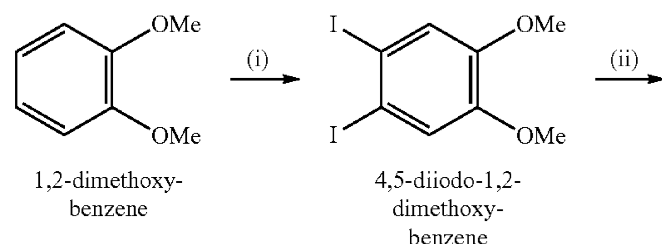
Scheme S5. Synthesis of (R/S)-1-(4,5-dimethoxy-2-nitrophenyl)-2,2-dimethyl-1-propanol.
