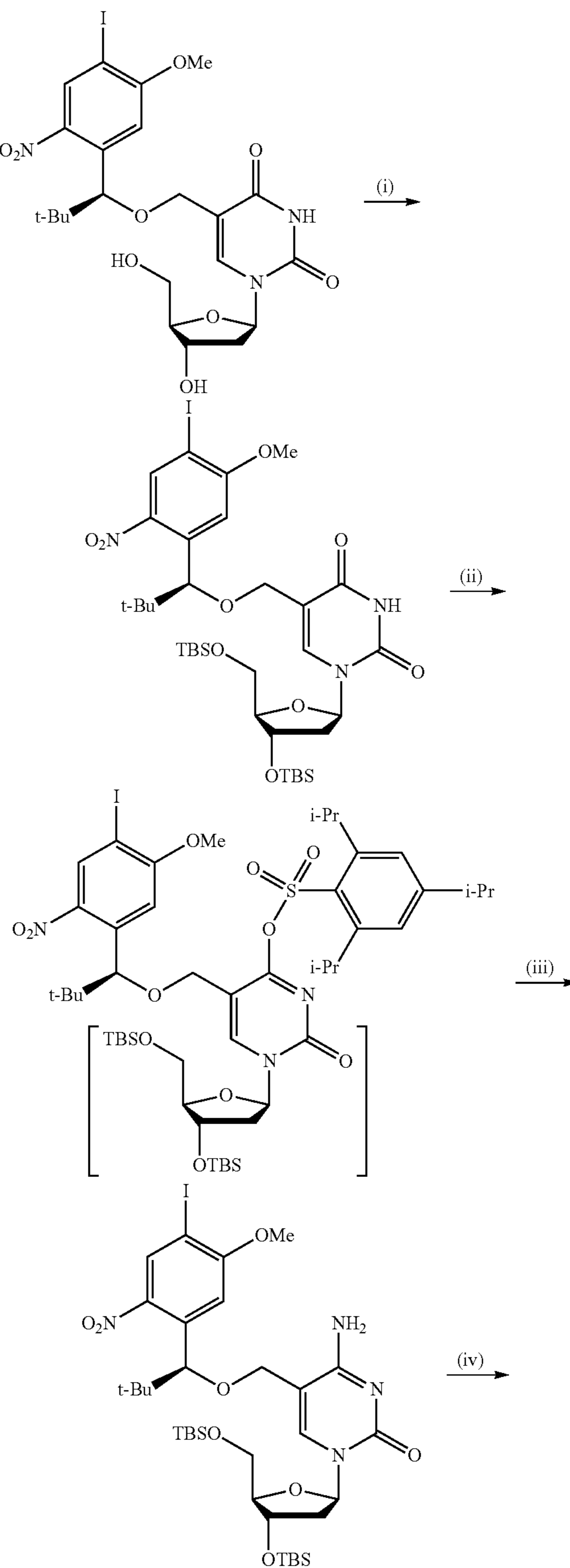
Scheme 5a. Synthesis of dye labeled 5-[(S)-1-(5-methoxy-2-nitrophenyl)-2,2-dimethyl-propyloxy]methyl-2'-deoxycytidine-5'-triphosphate.
