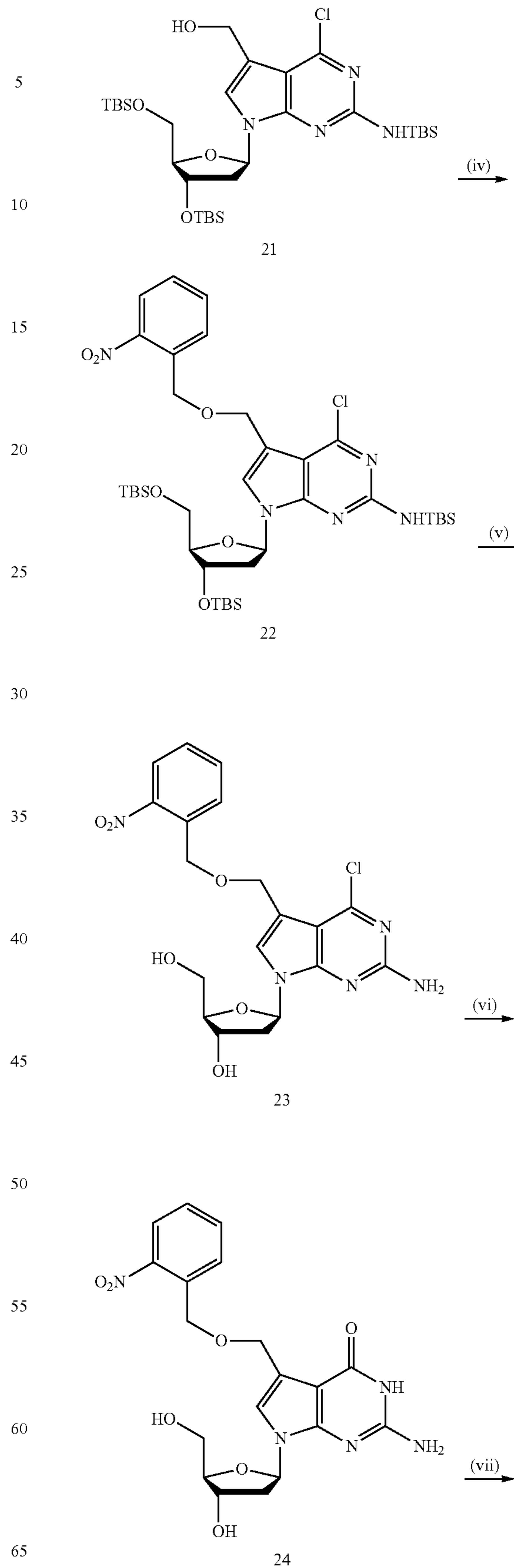
Scheme S12. Synthesis of 7-(2-nitrobenzyloxy)methyl-7-deaza-2'- deoxyguanosine-5'-triphosphate.
