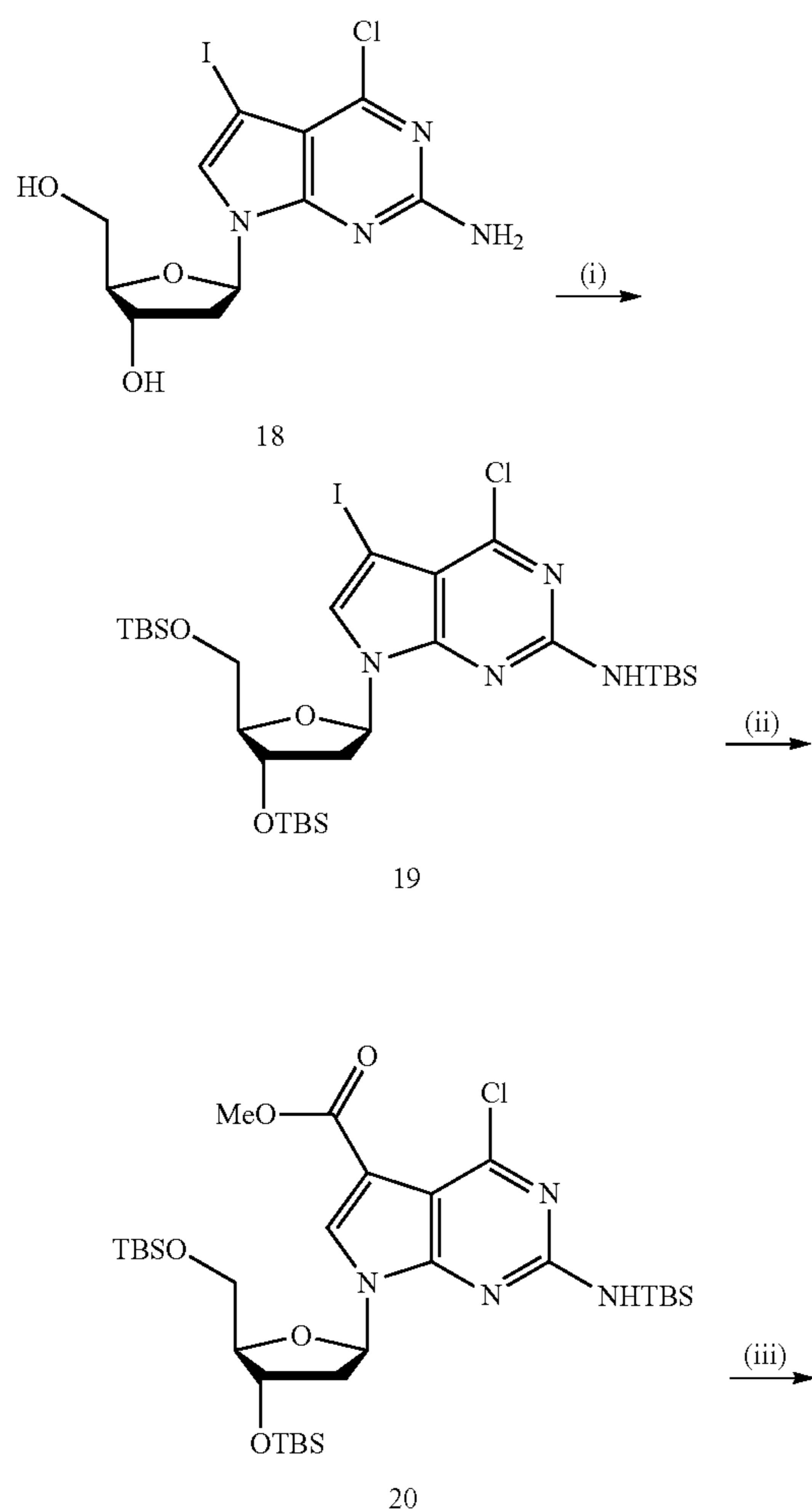
Scheme S12. Synthesis of 7-(2-nitrobenzyloxy)methyl-7-deaza-2'- deoxyguanosine-5'-triphosphate.
