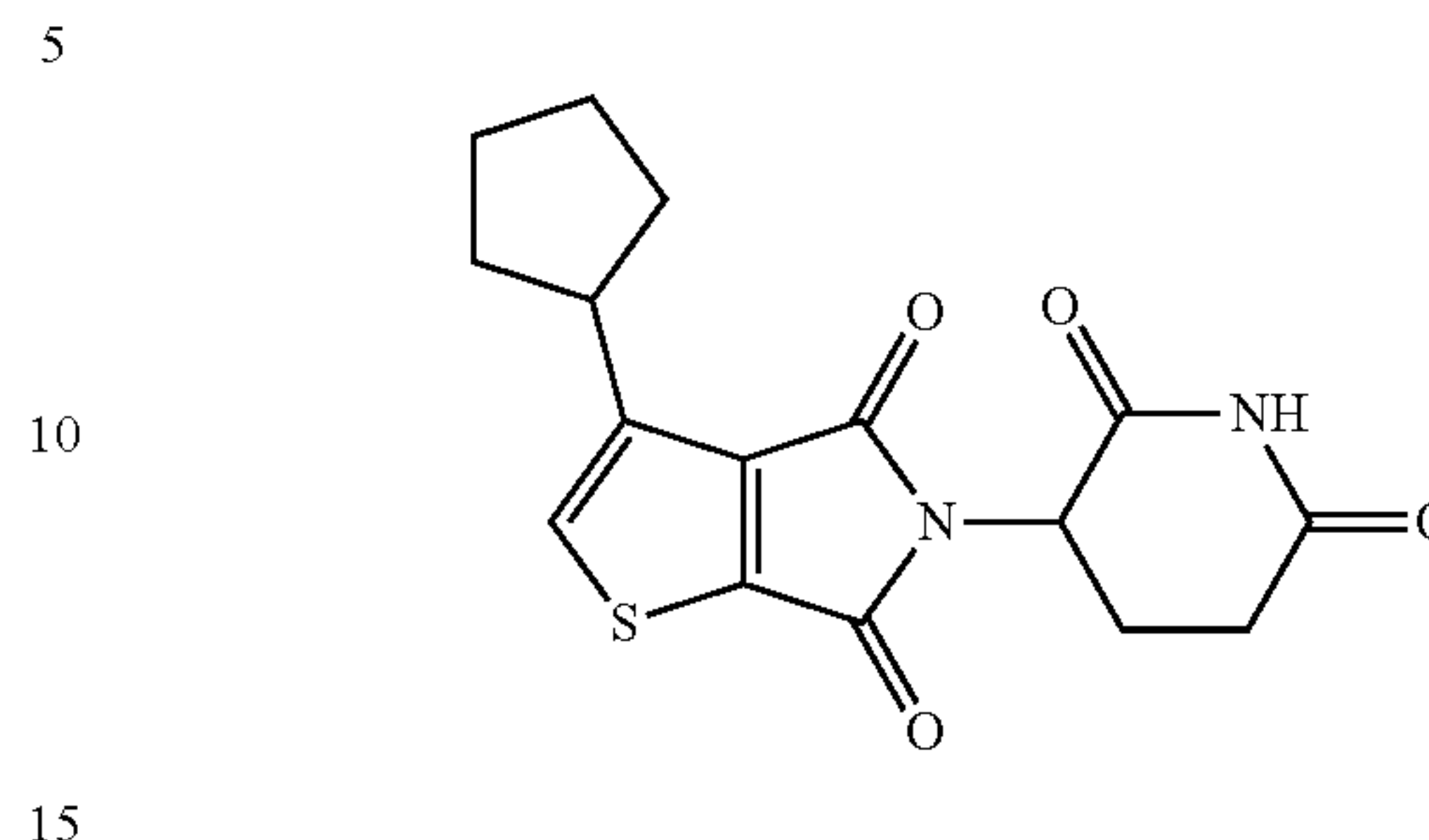
Compound 21: 3-(4-Oxo-4H-thieno[2,3-c]pyrrol-5(6H)-yl)piperidine-2,6-dione
