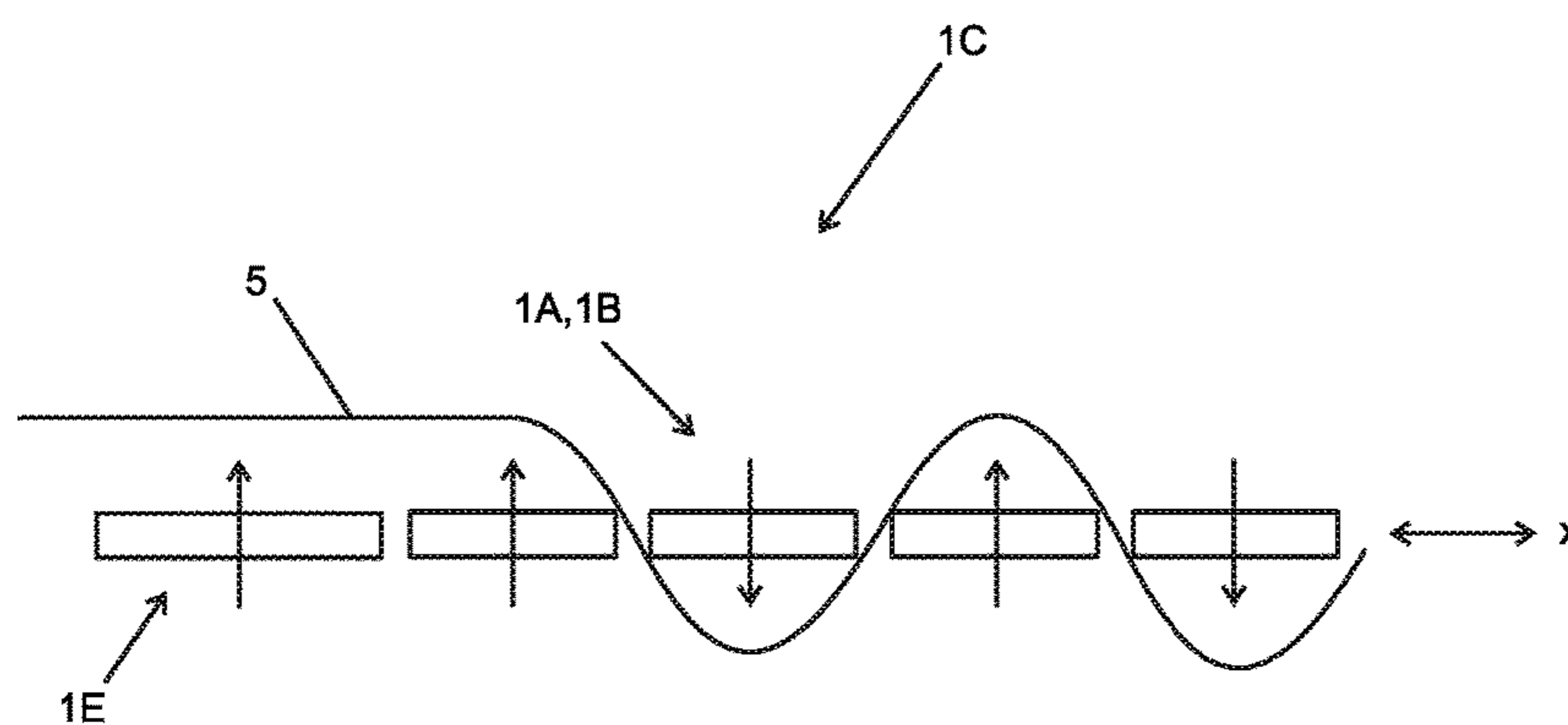
1A,1B,1C,1E: permanently-magnetized position identifiers 5: sinusoidal magnetic field x: trajectory
