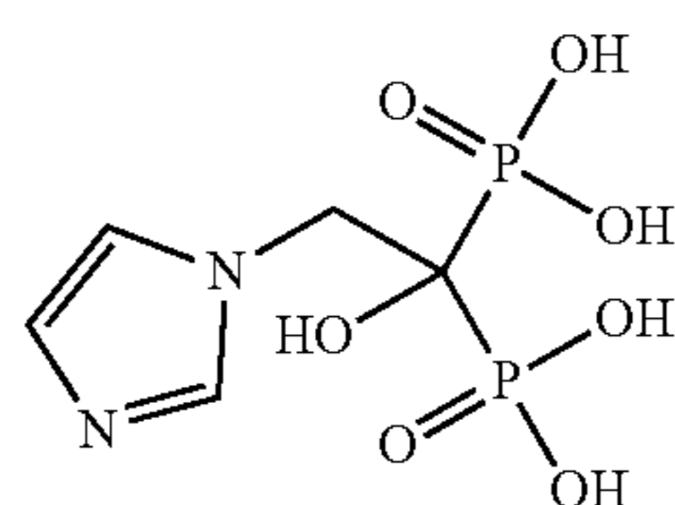
Zoledronic acid
