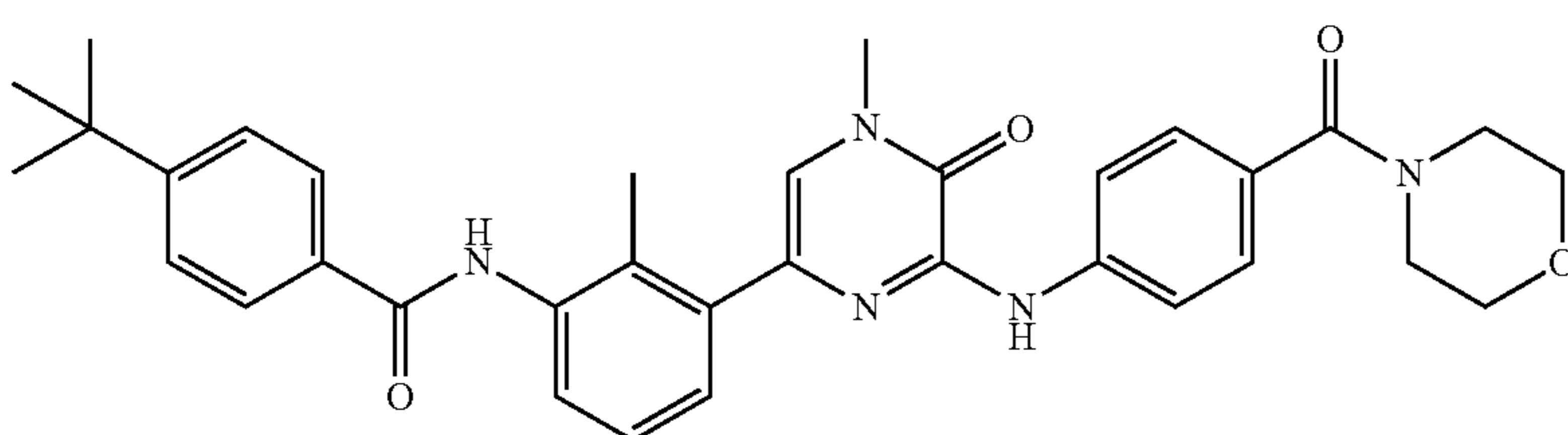
CGI-1746
