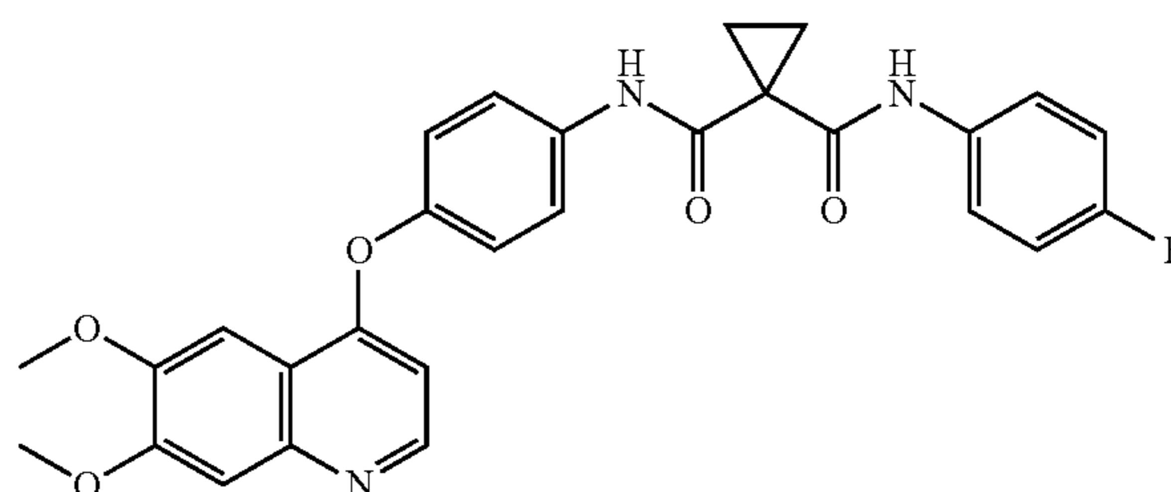
Compound I
