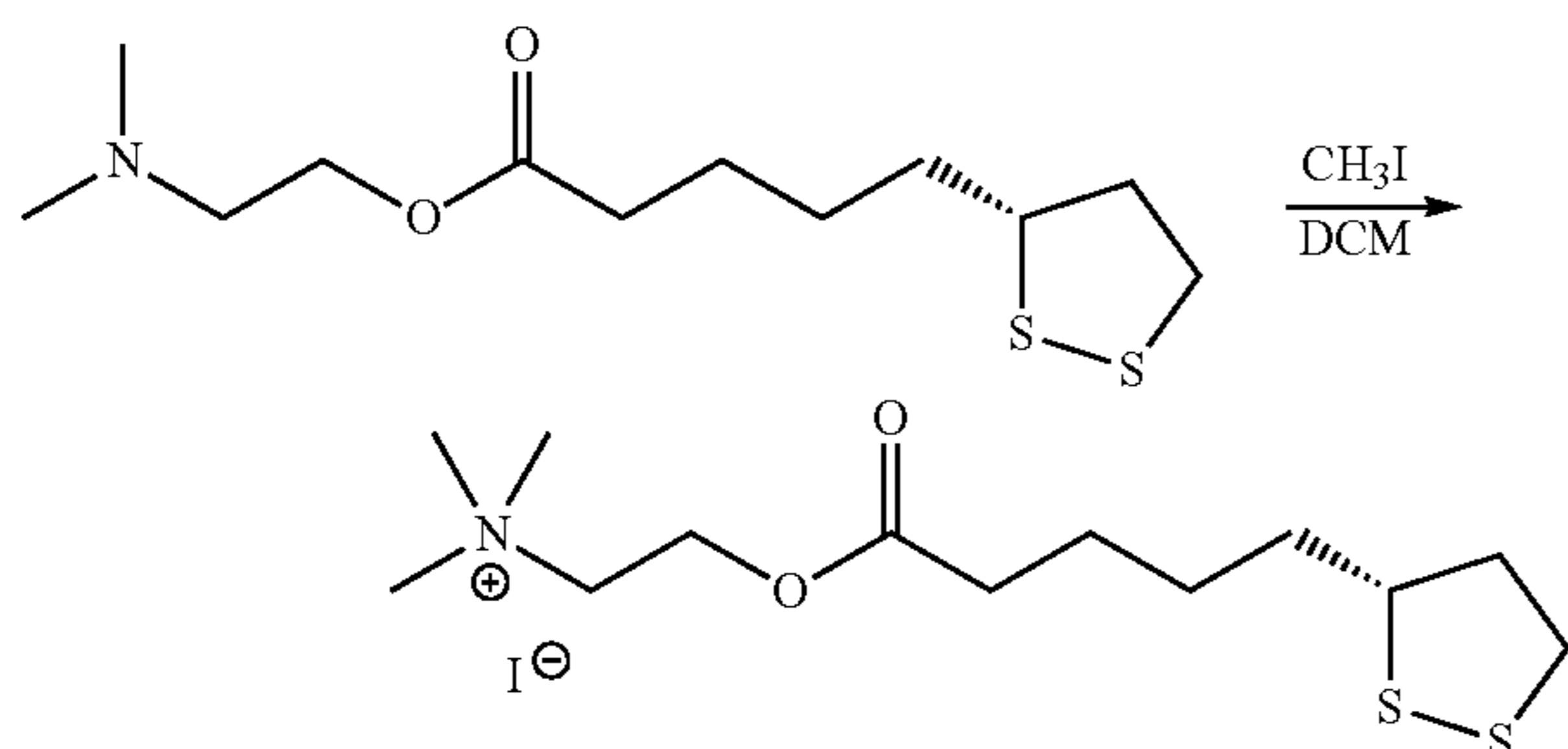
(R)-2-(5-(1,2-dithiolan-3-yl)pentanoyloxy)-N,N,N-(trimethyl)ethylammonium Iodide
