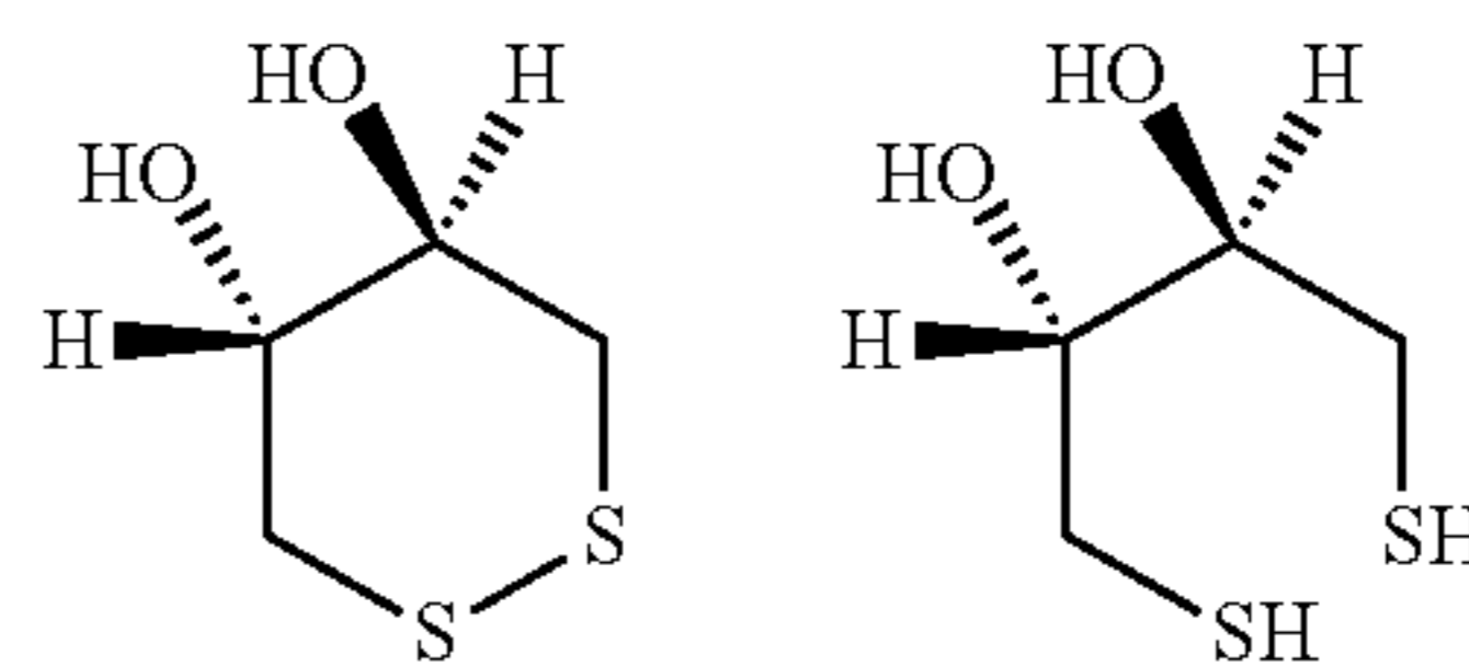
Trans-4,5-dihydroxy-1,2-dithiane (Non-lethal DTT)
