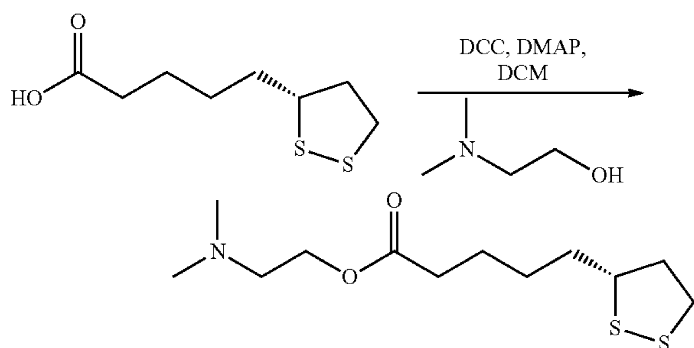
(R)-2-(dimethylamino)ethyl 5-(1,2-dithiolan-3-yl)pentanoate
