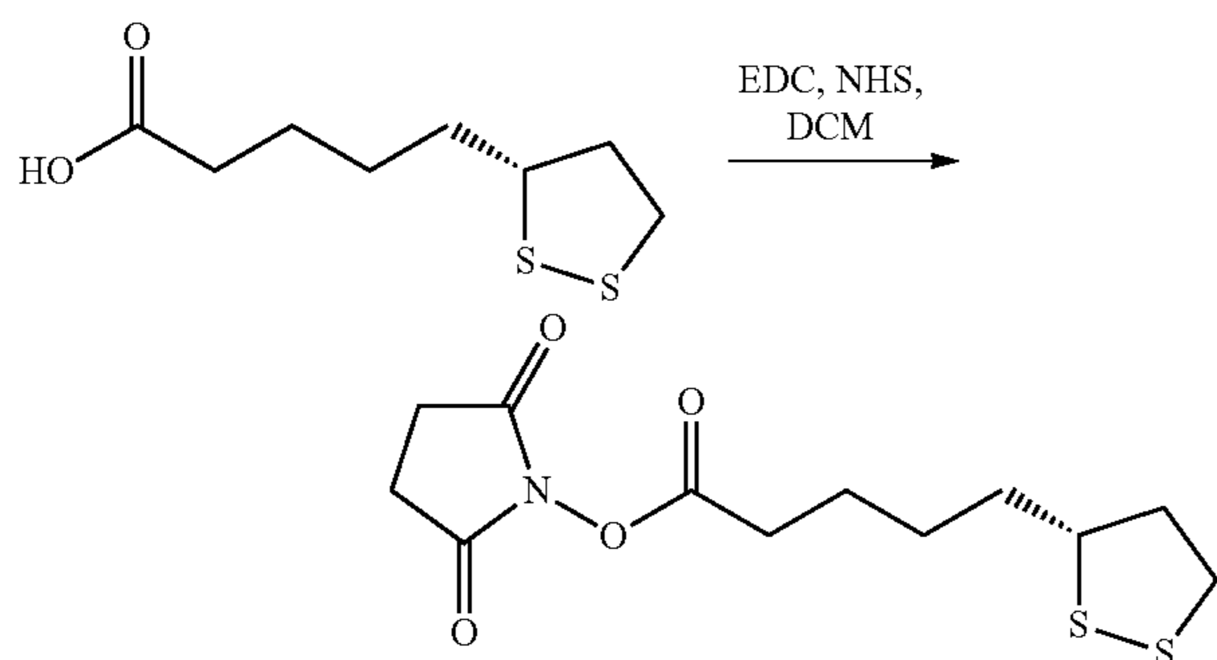
Scheme 1. Synthetic scheme for NHS-ester of (R)-lipoic acid.
