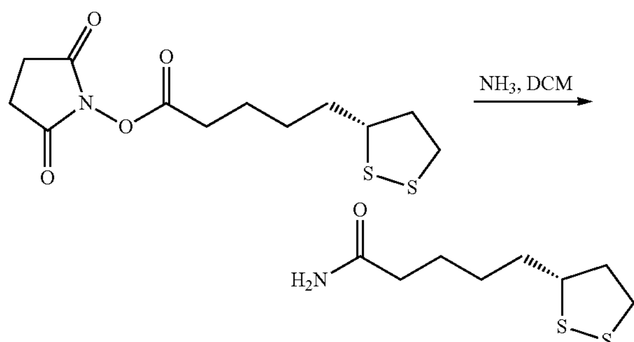
Scheme 2. Synthetic scheme for (R)-lipoamide.
