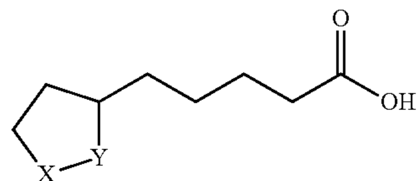
Lipoic acid
