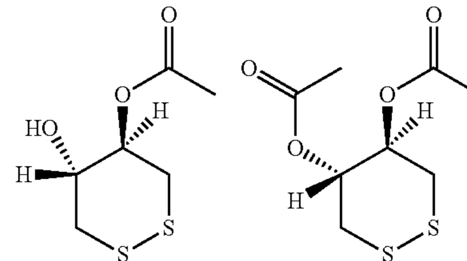
(4R,5R)-5-hydroxy-1,2-dithian-4-yl acetate
