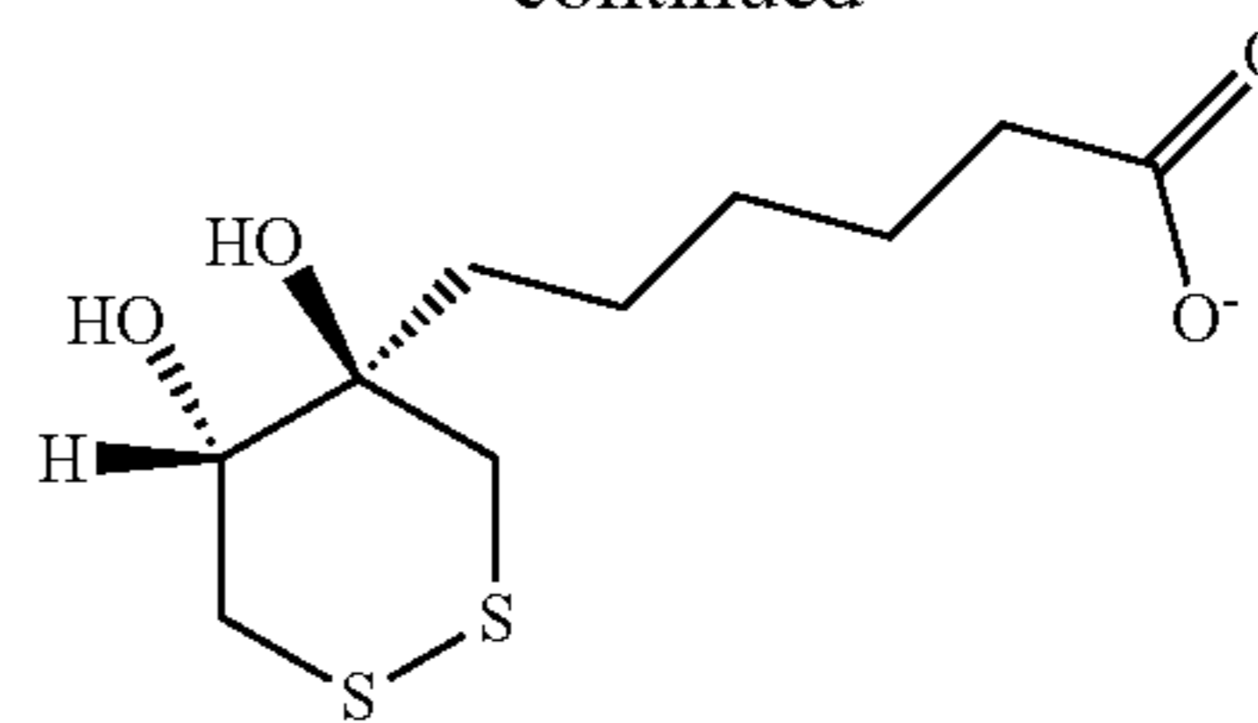
6-((4R,5R)-4,5-dihydroxy-1,2-dithian-4-yl) hexanoate
