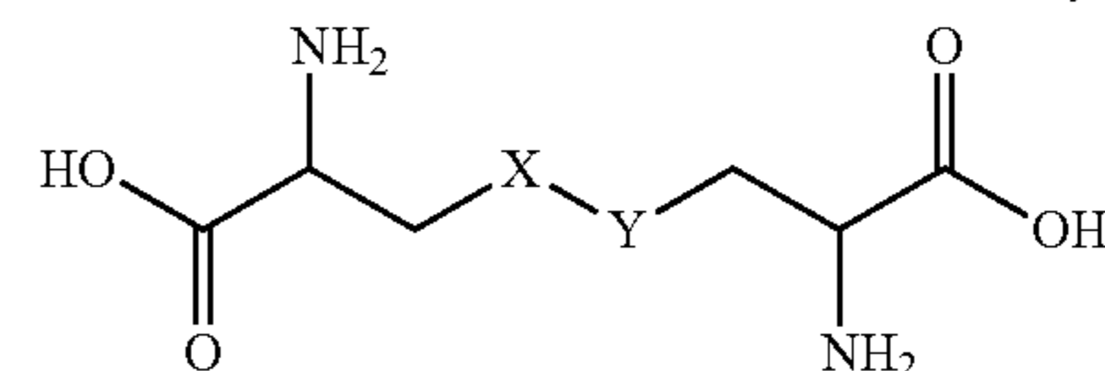
cystine
