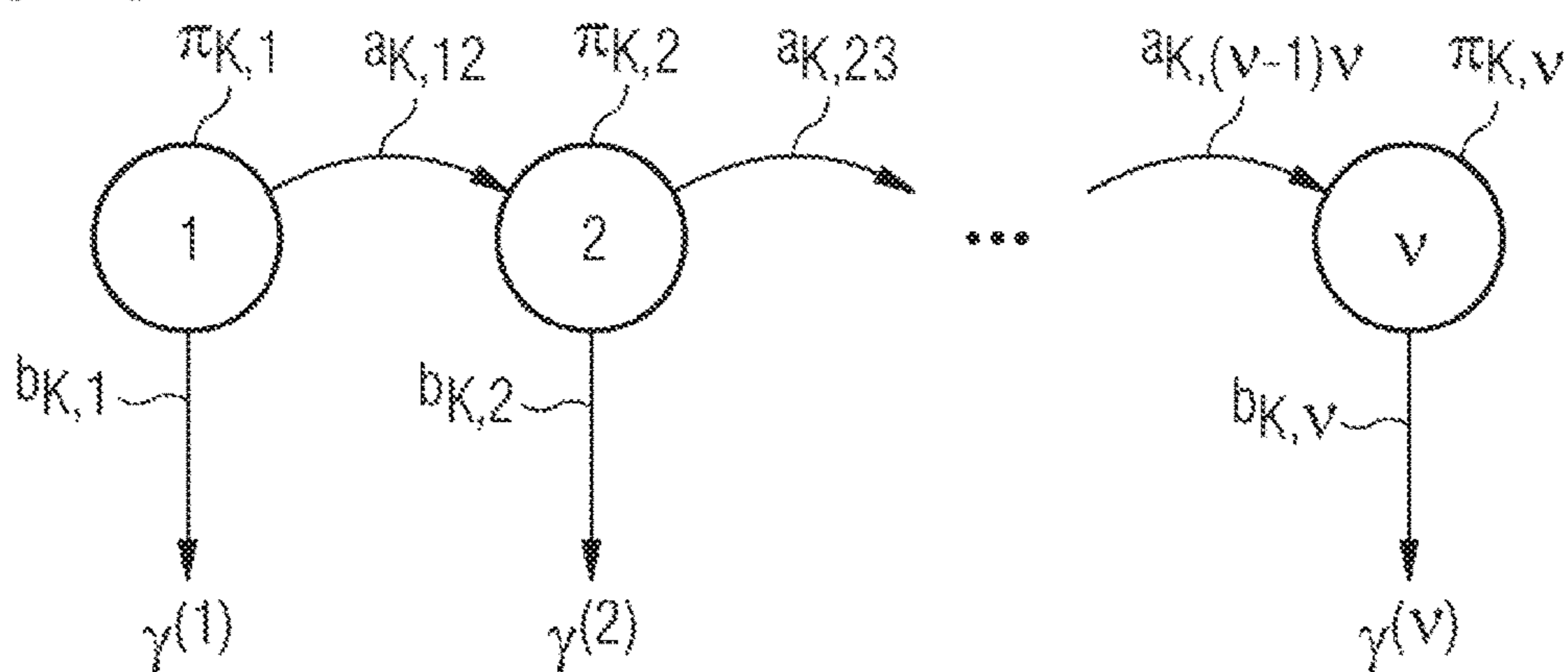
HMM of the event to be determined with the states z_K \in \{1, \dots, v\} , outputs \gamma and parameters \Theta_K = \{A_K, B_K, \pi_K\}
