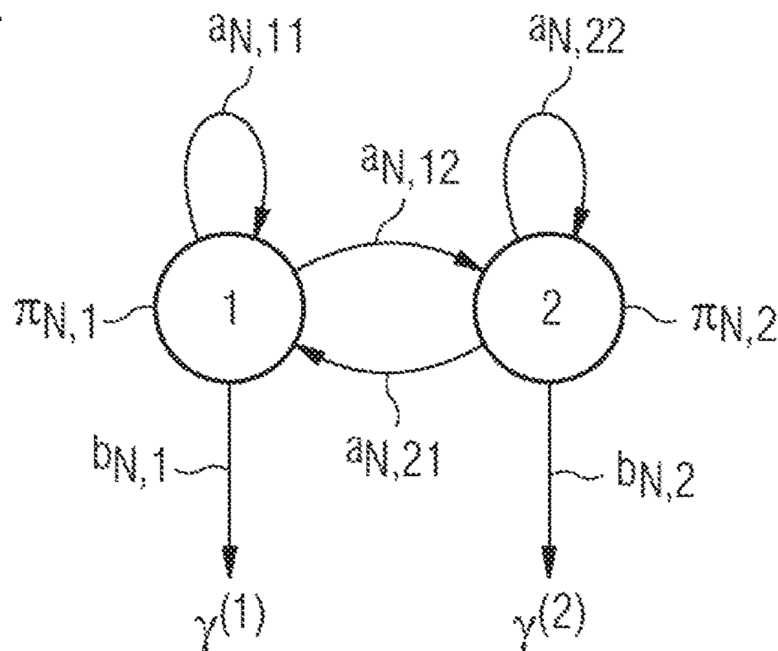
HMM of the NULL class with the states z_N \in \{1, 2\} , outputs \gamma and parameters \Theta_N = \{A_N, B_N, \pi_N\}
