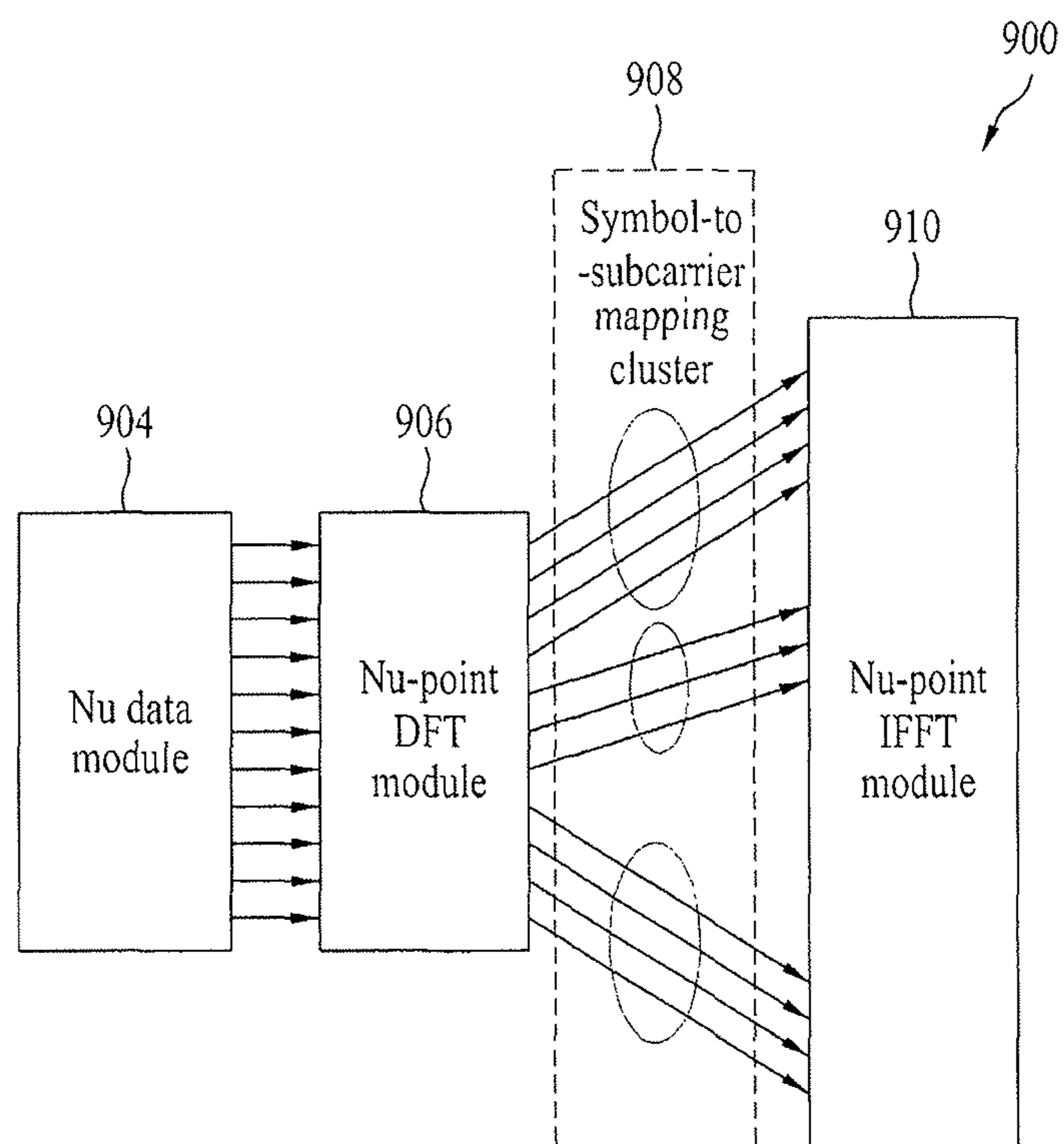
Clustered DFT-s-OFDMA
