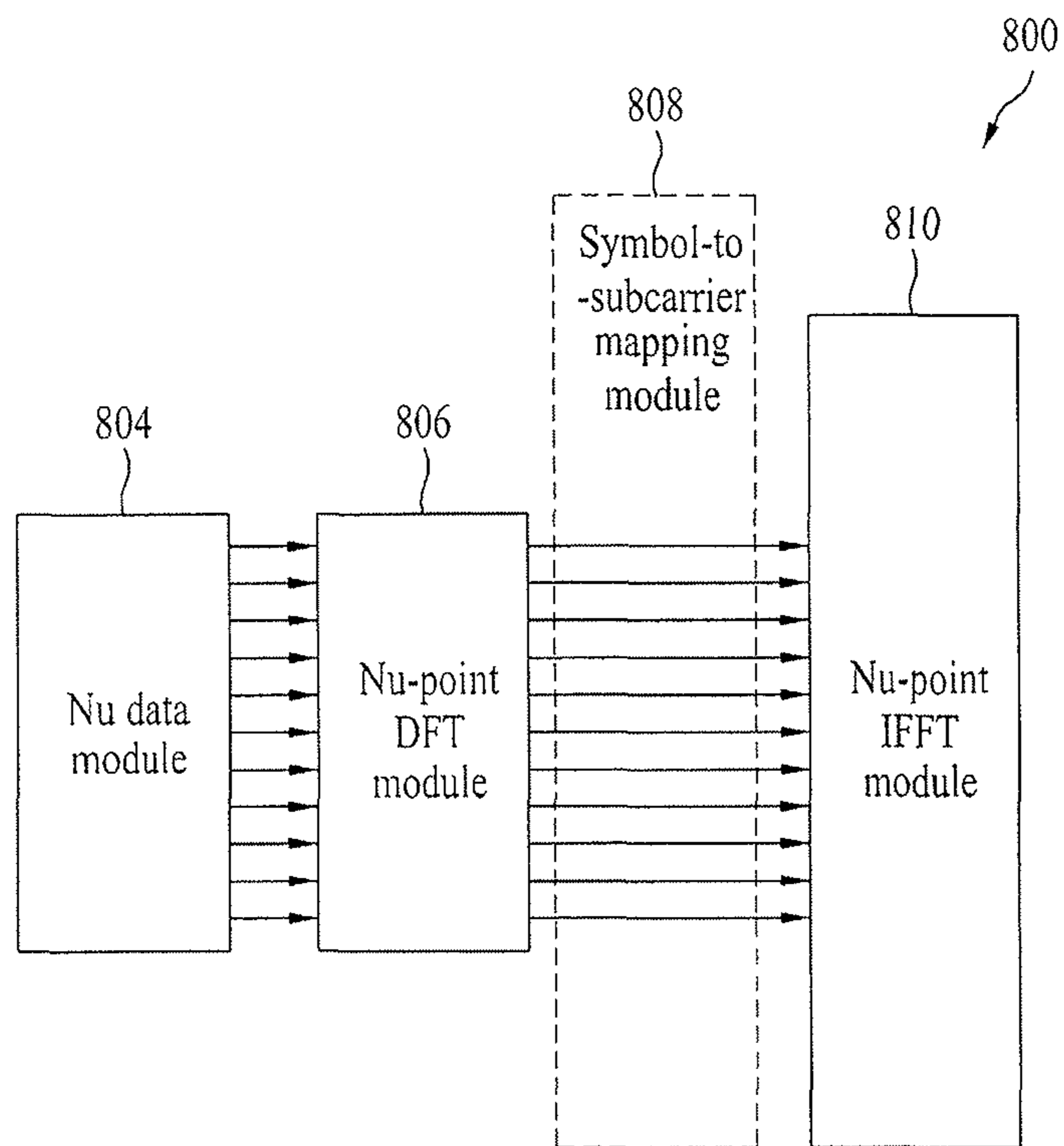
Localized DFT-s-OFDMA
