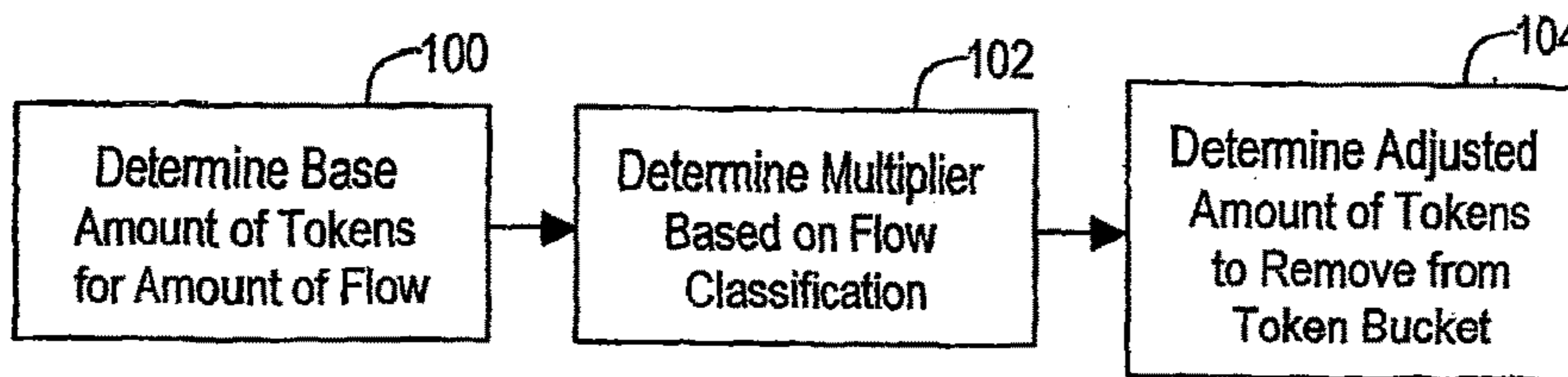
Dynamically Adjust Token Bucket Configuration Based on Network Demand
