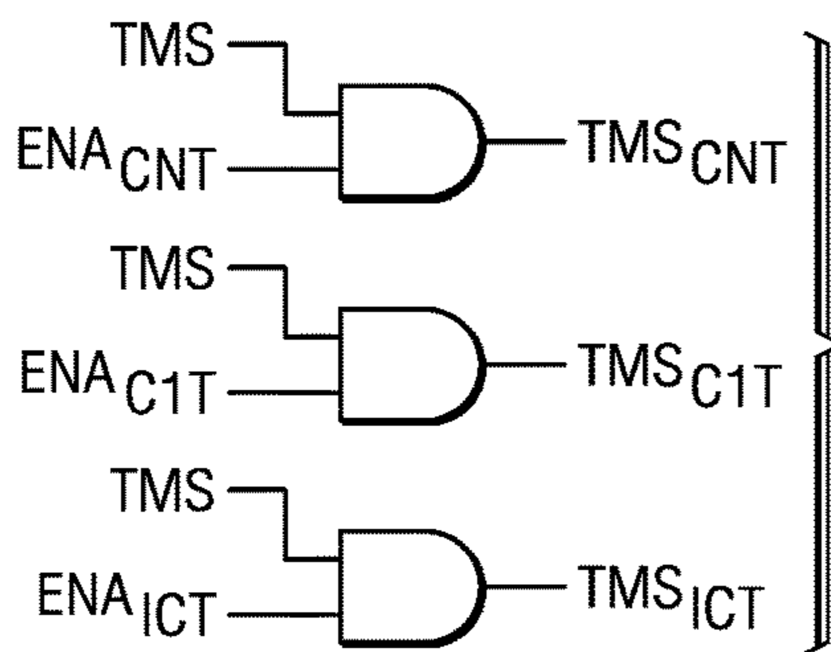
FIG. 5 (PRIOR ART)
