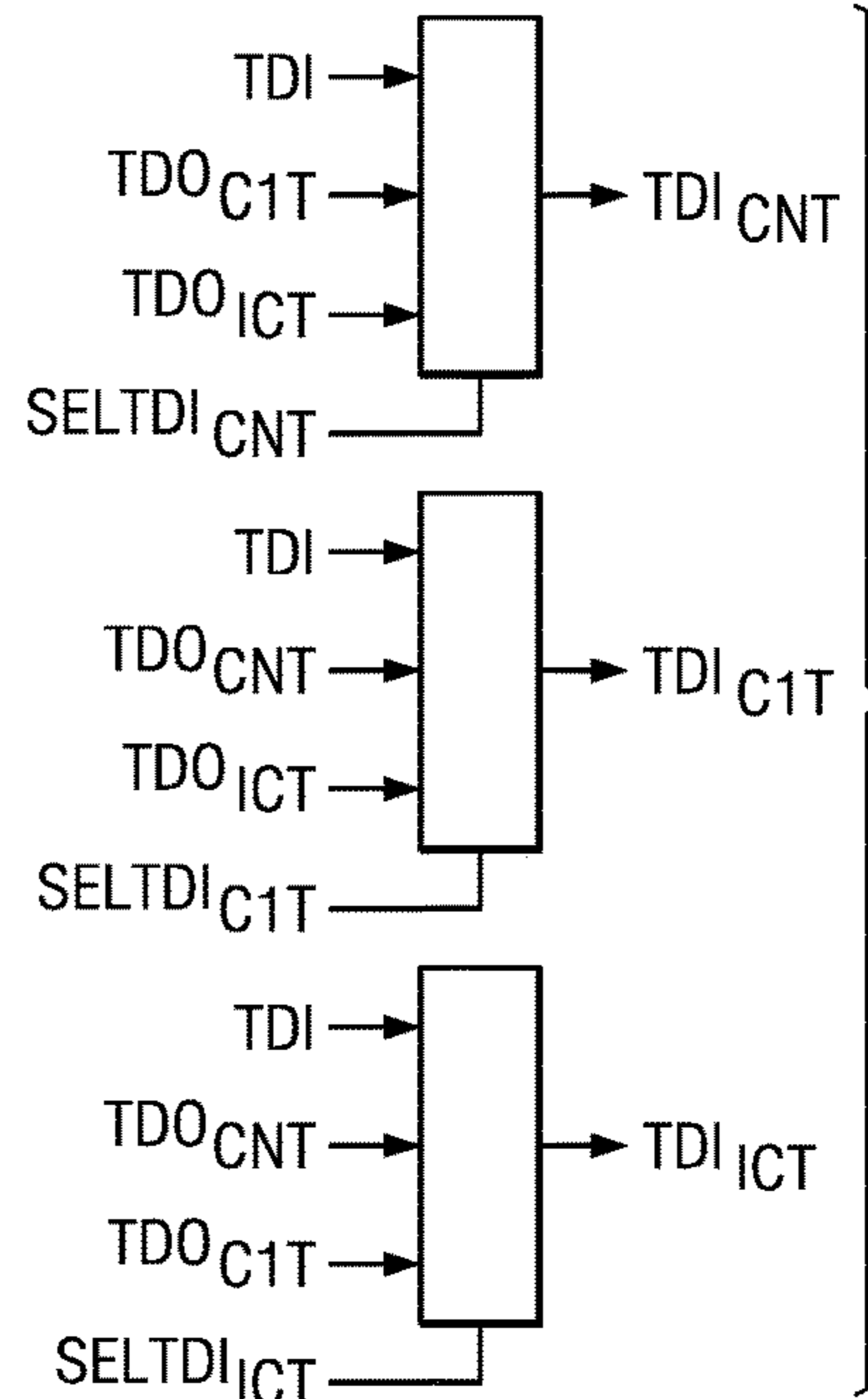
FIG. 6 (PRIOR ART)
