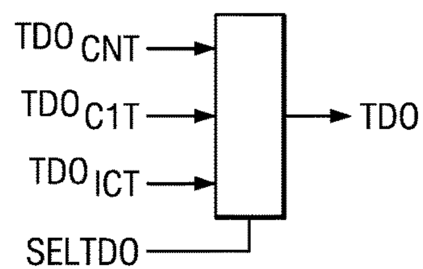
FIG. 7 (PRIOR ART)
