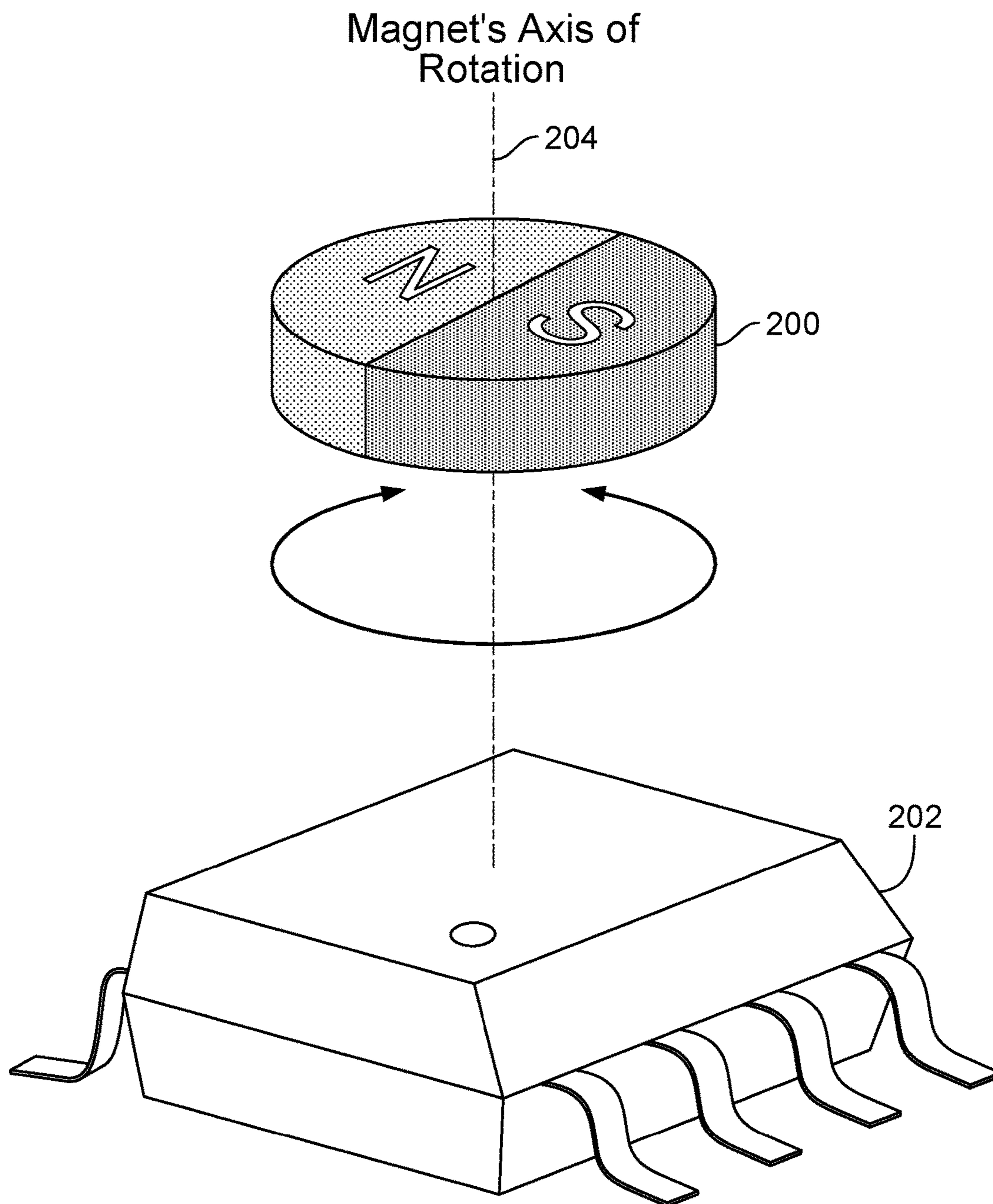
IC with Linear Hall Sensors
