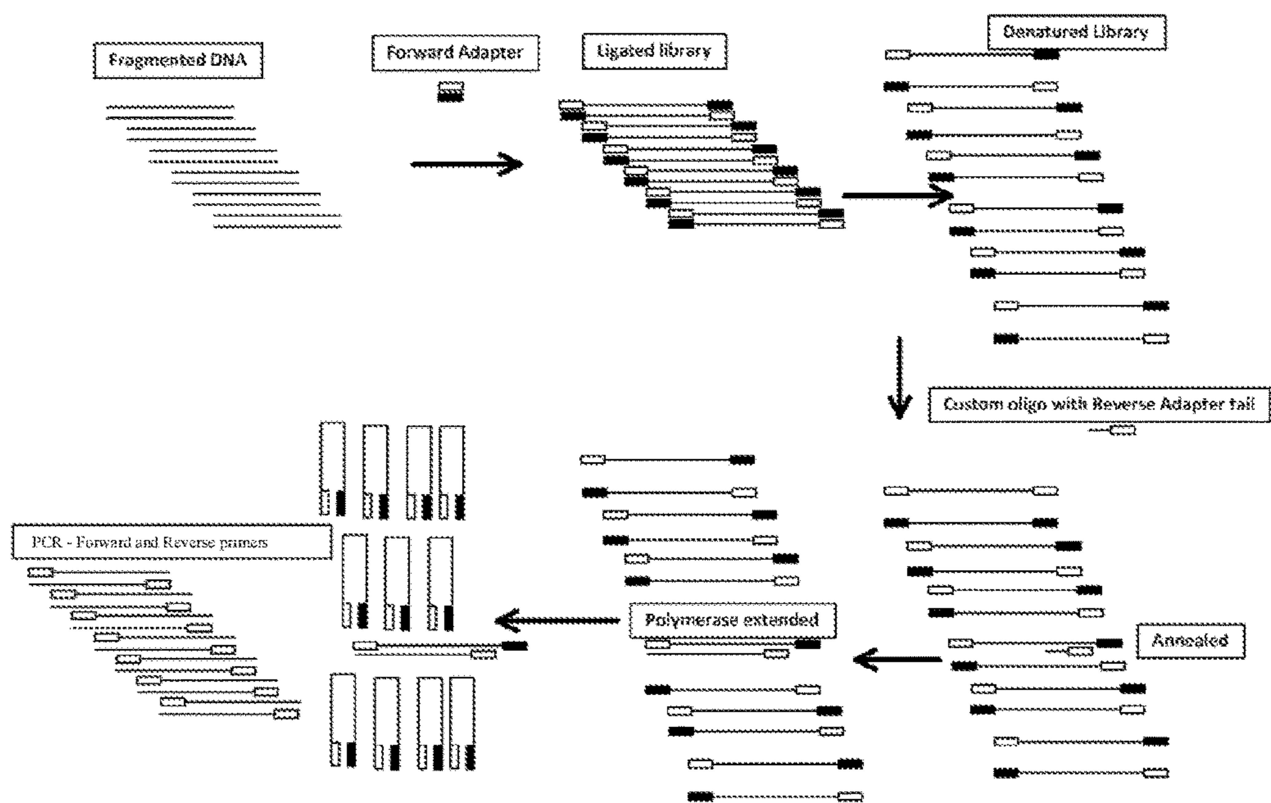
FIG. 1 Subtractive PCR Enrichment
