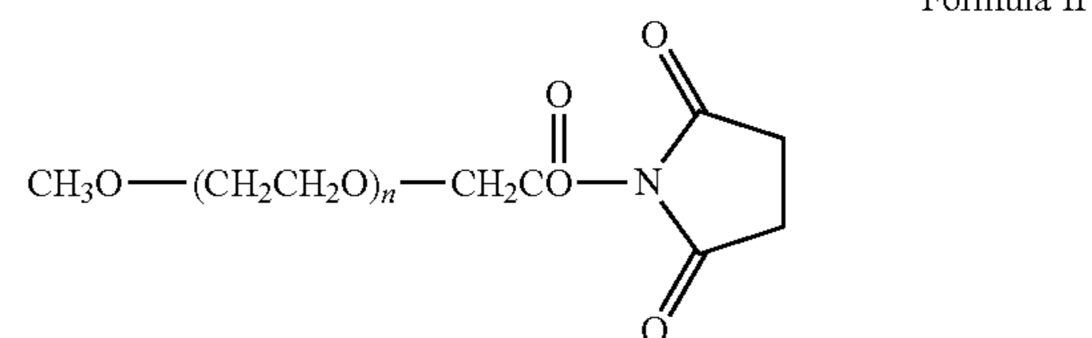
Formula II
