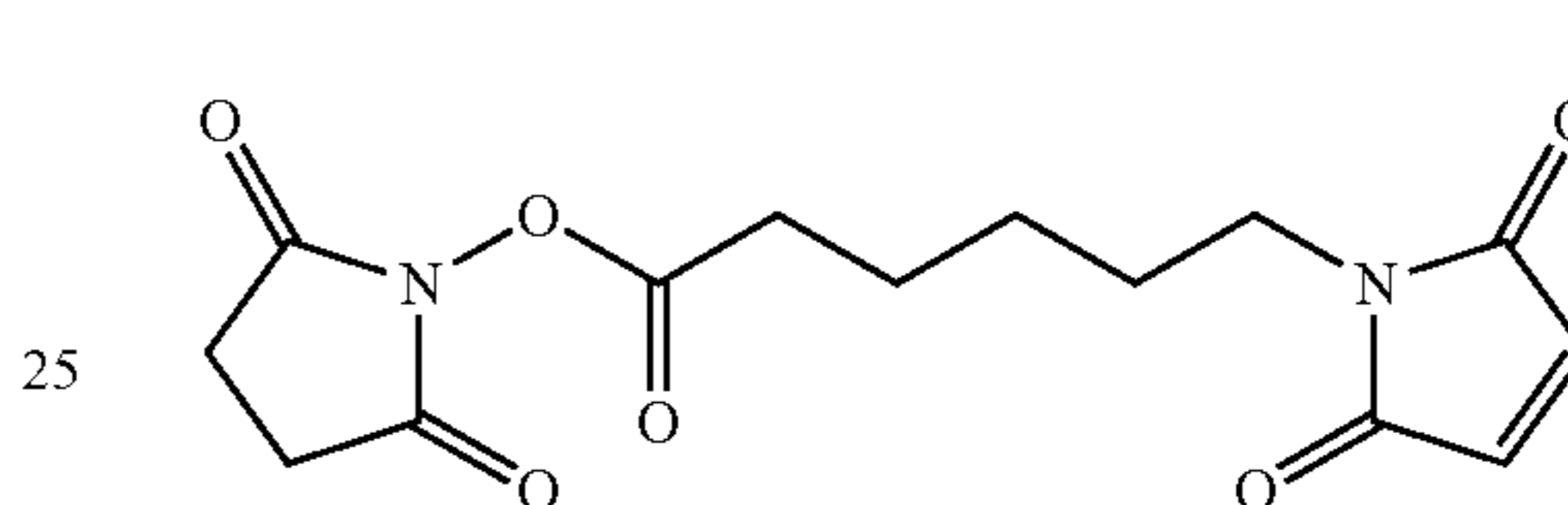
Compound II
