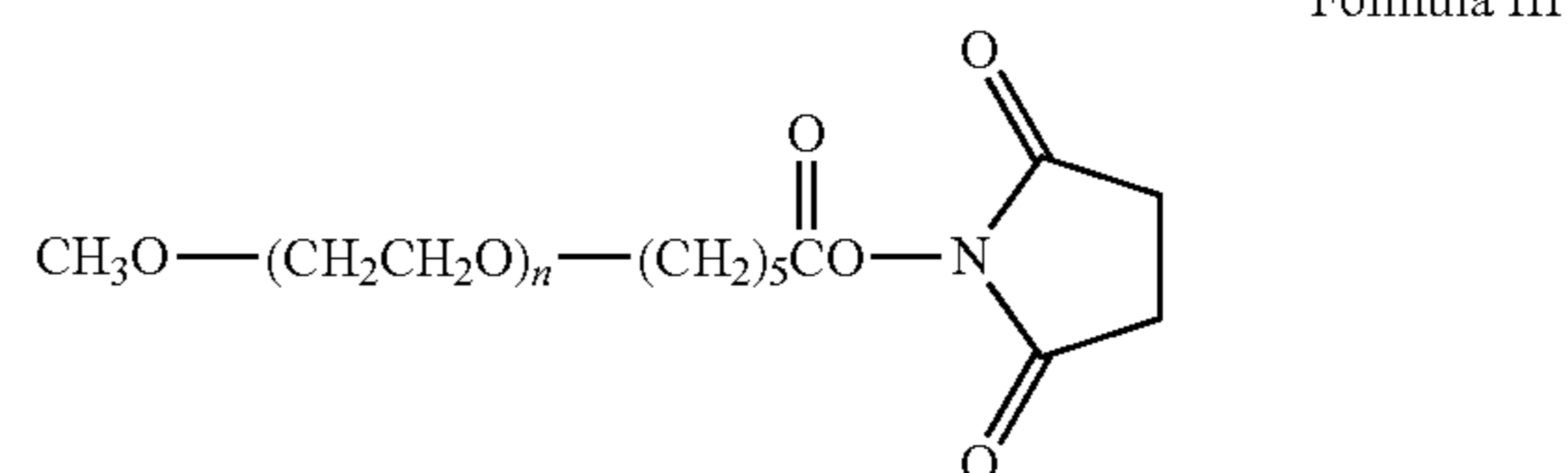
Formula IIIa
