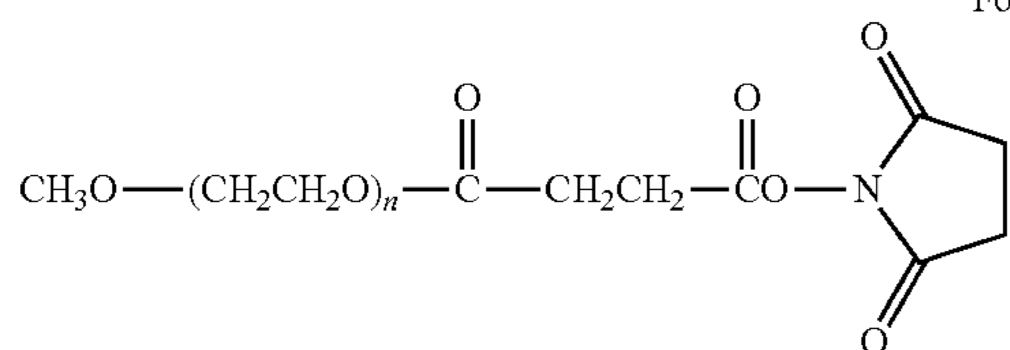
Formula I 55
