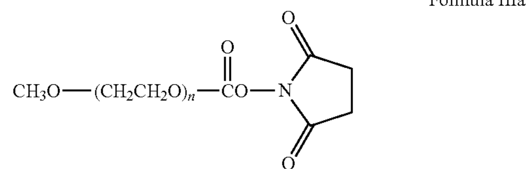
Formula IIIa
