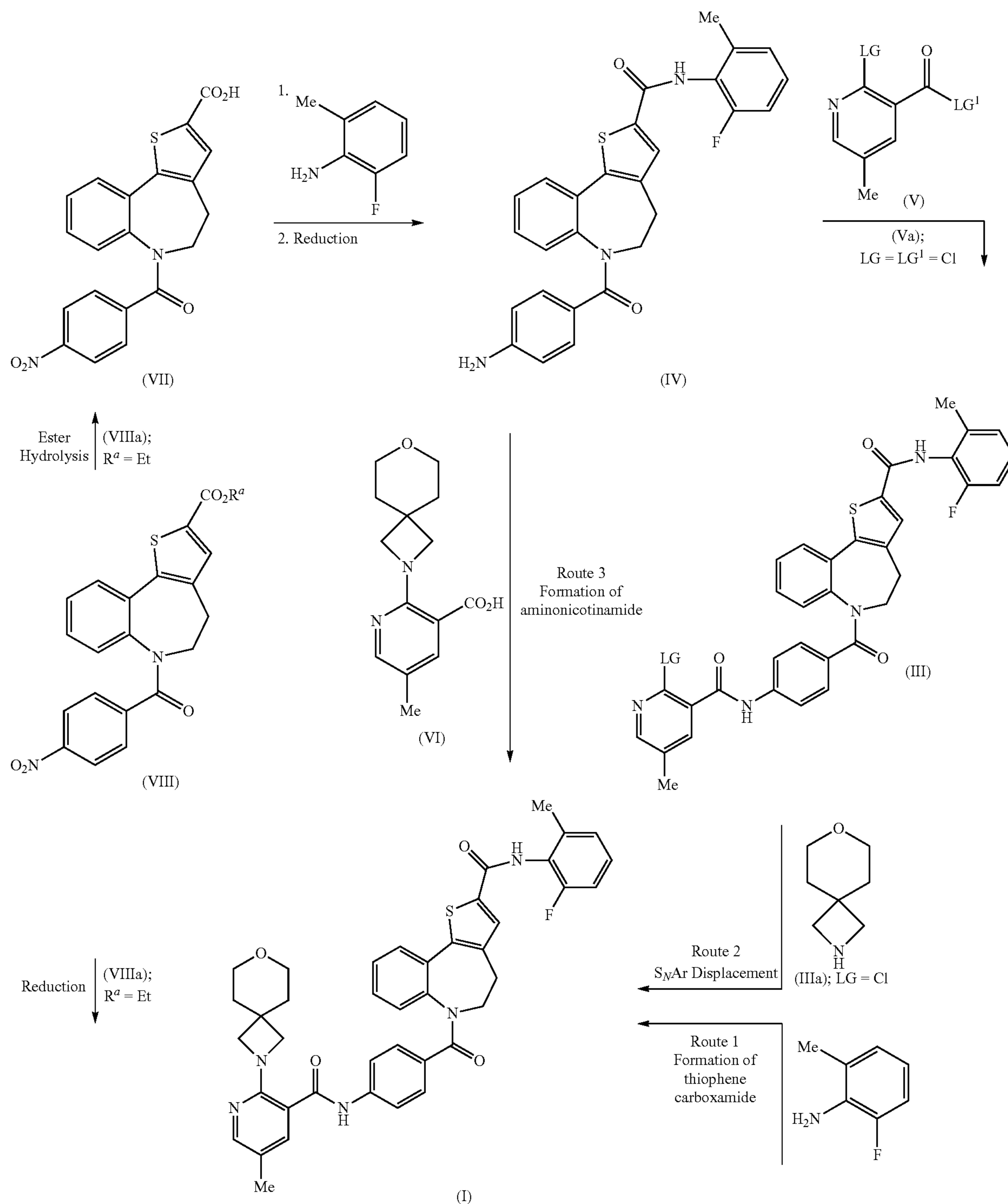
Scheme 1: Synthetic routes used for the preparation of Compound (I).
