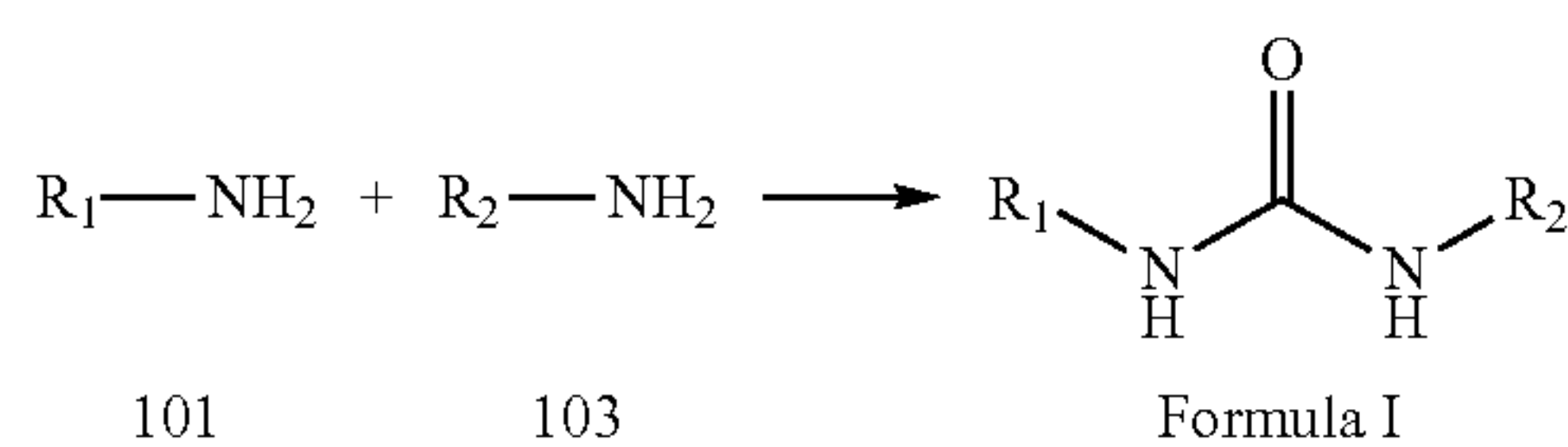
REACTION SCHEME 1
