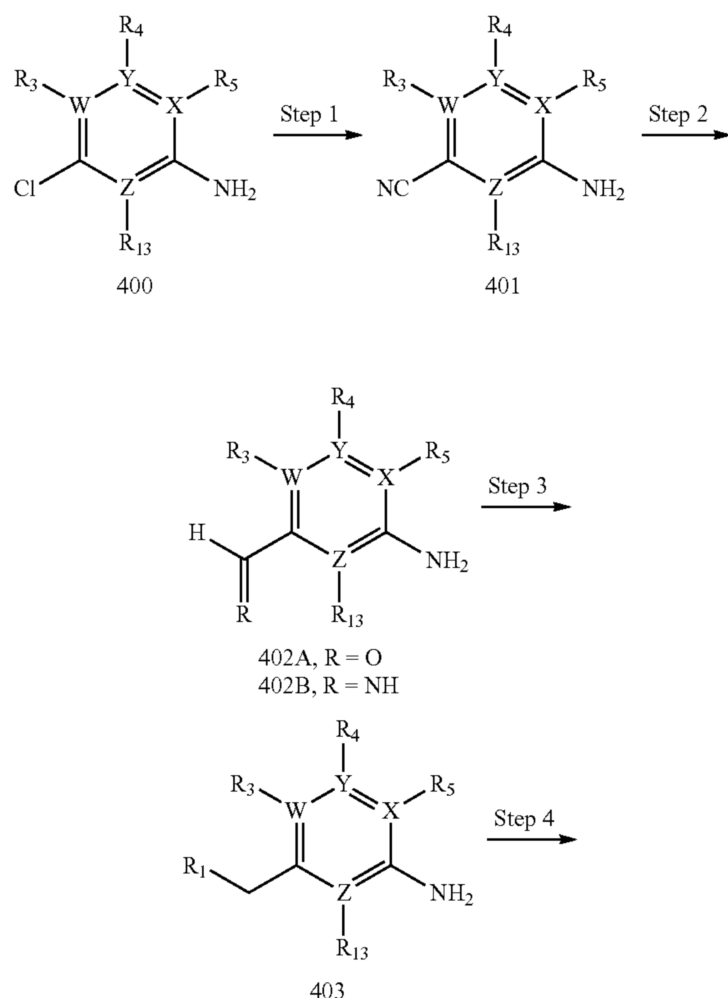
Reactions Scheme 4
