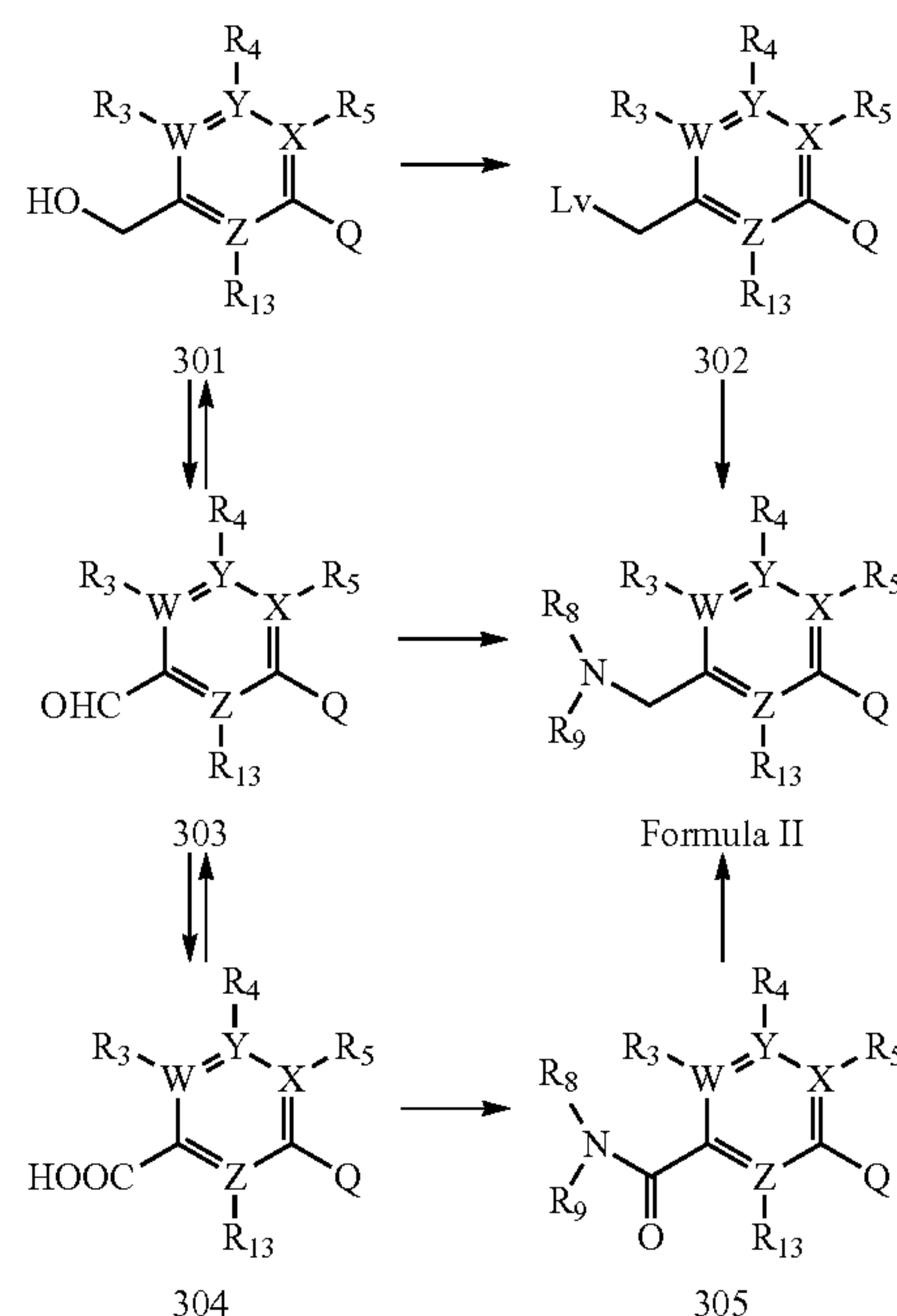
REACTION SCHEME 3
