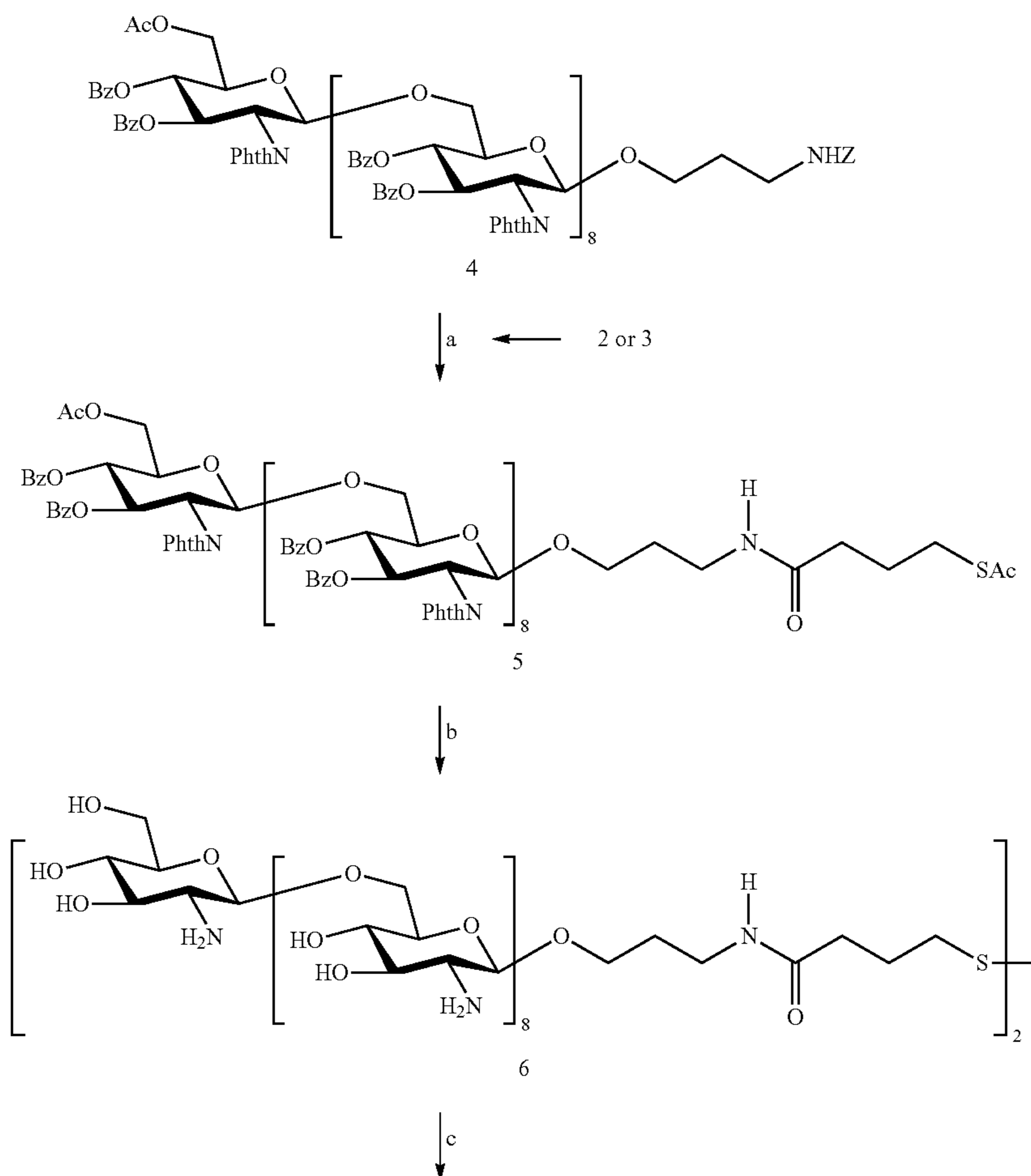
Scheme 3. Synthesis of the ligands.
