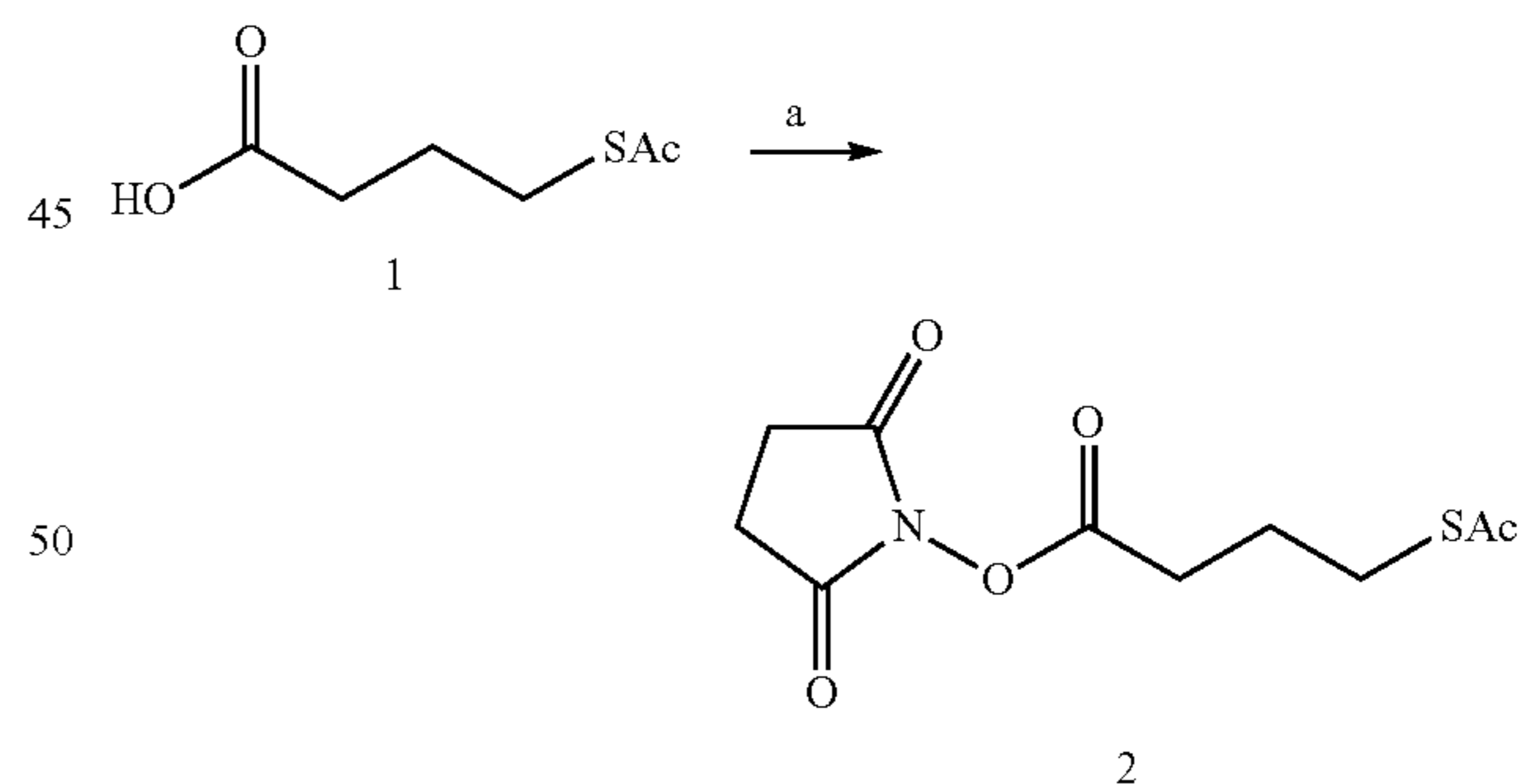
Scheme 1. Synthesis of the linking reagent 2.
