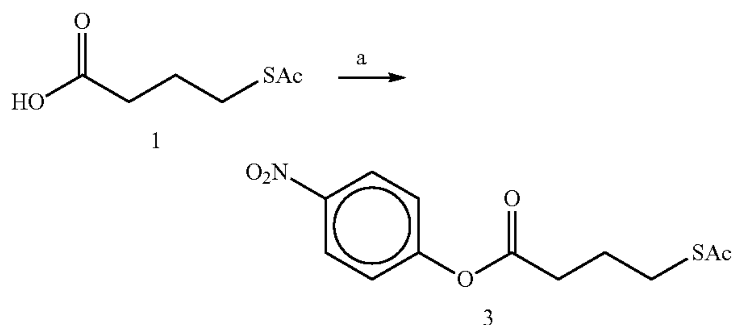
Scheme 2. Synthesis of the linking reagent 3.
