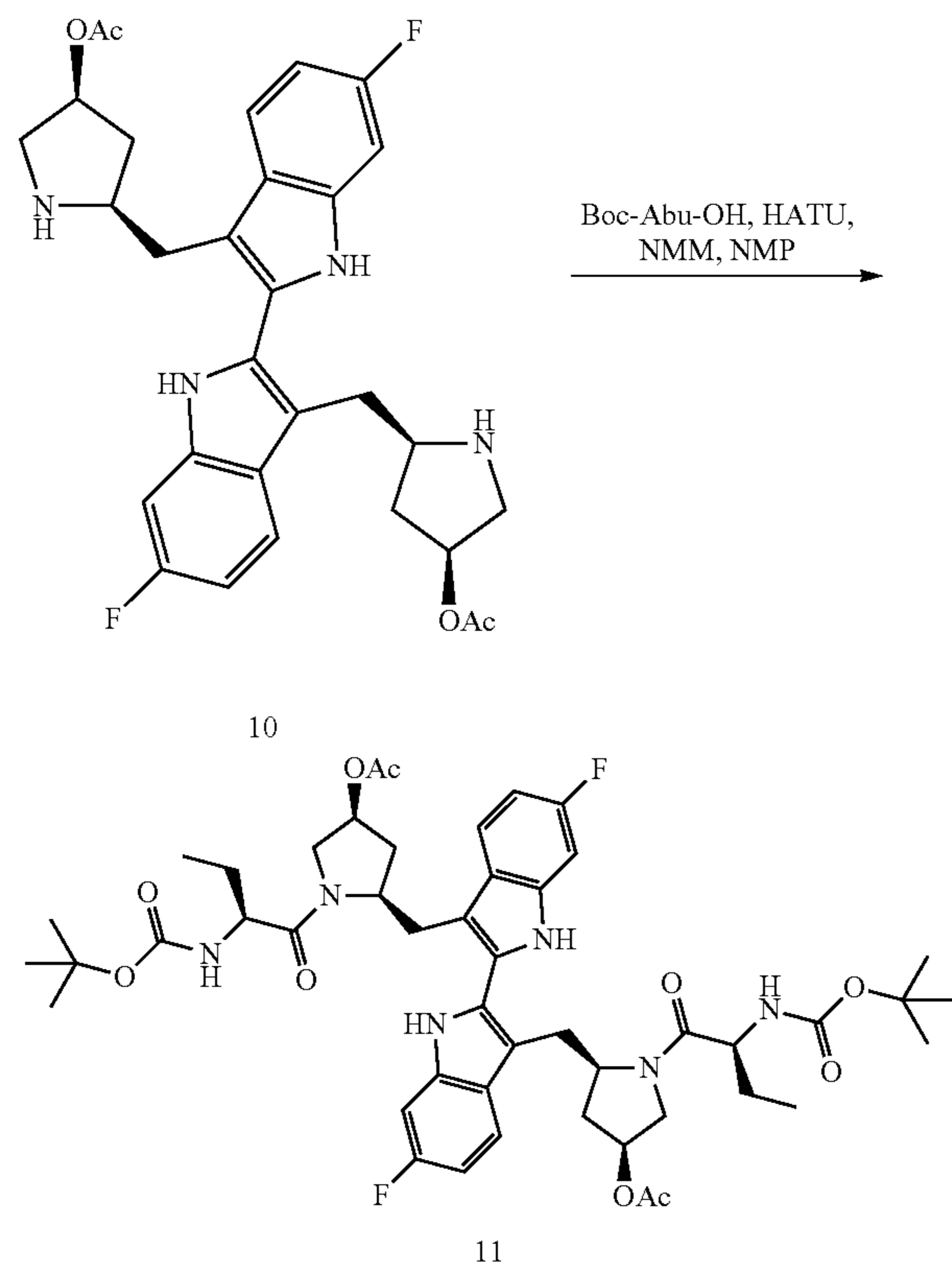
Scheme X
