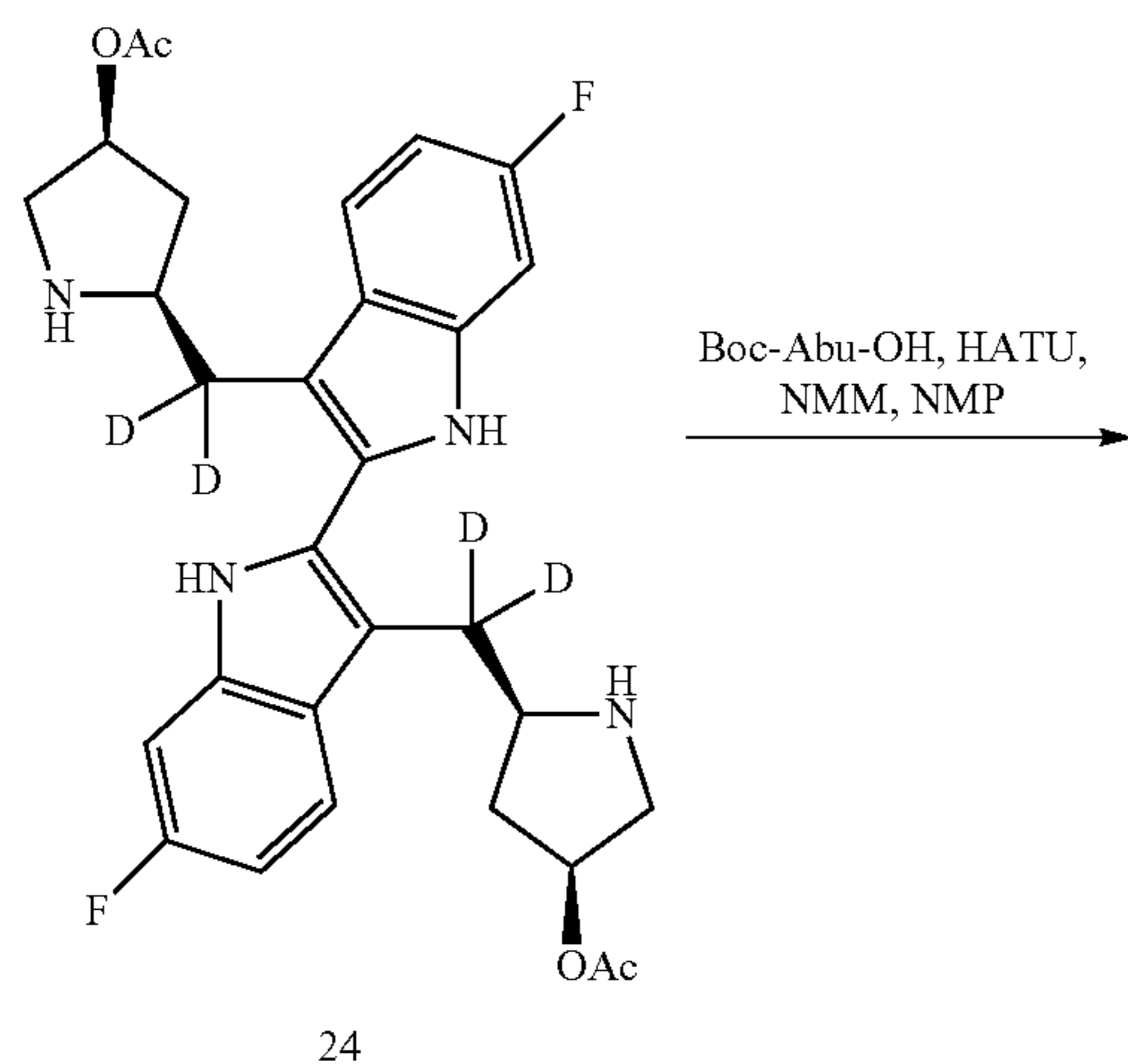
Scheme XXIII
