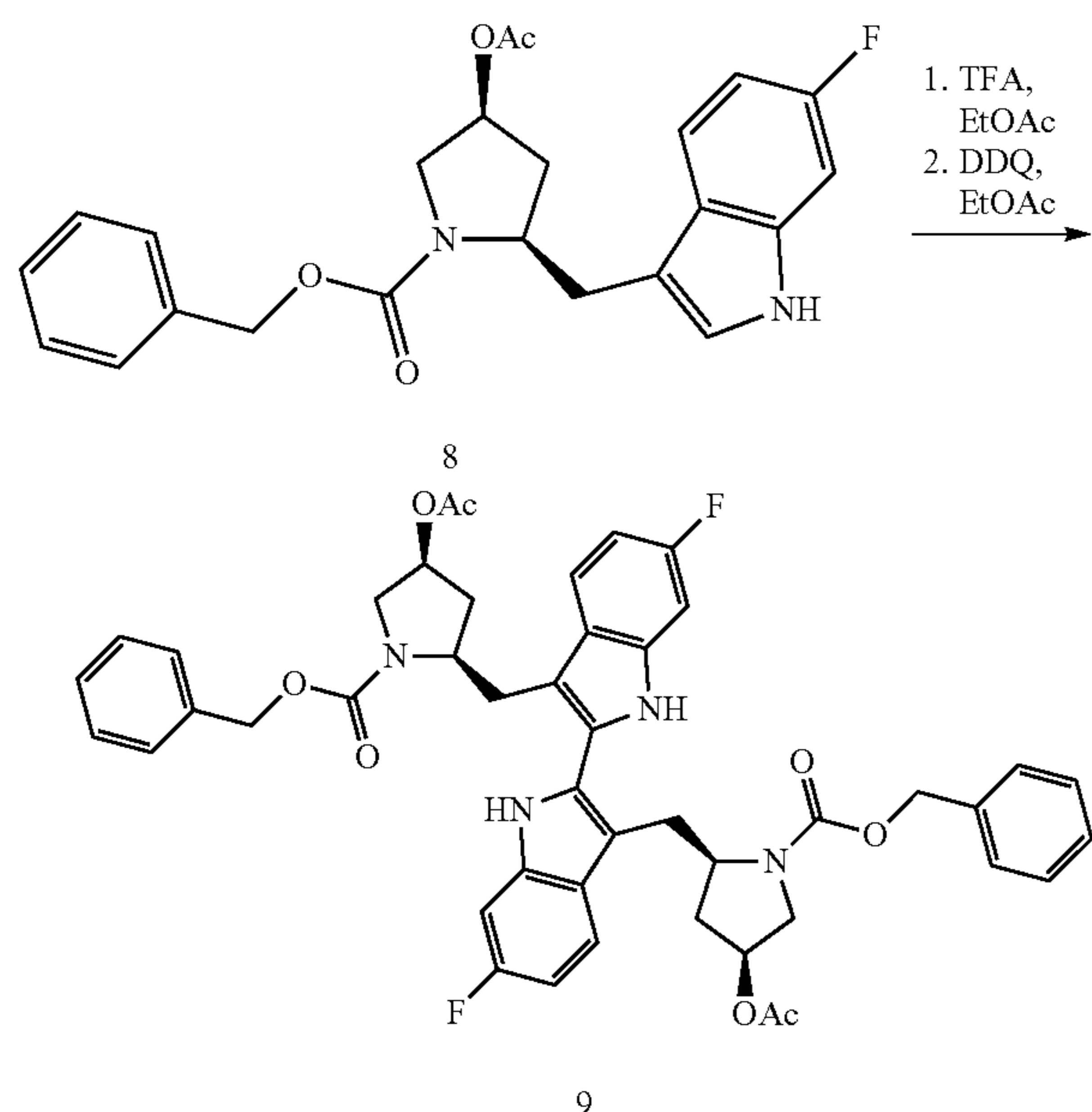
Scheme VIII
