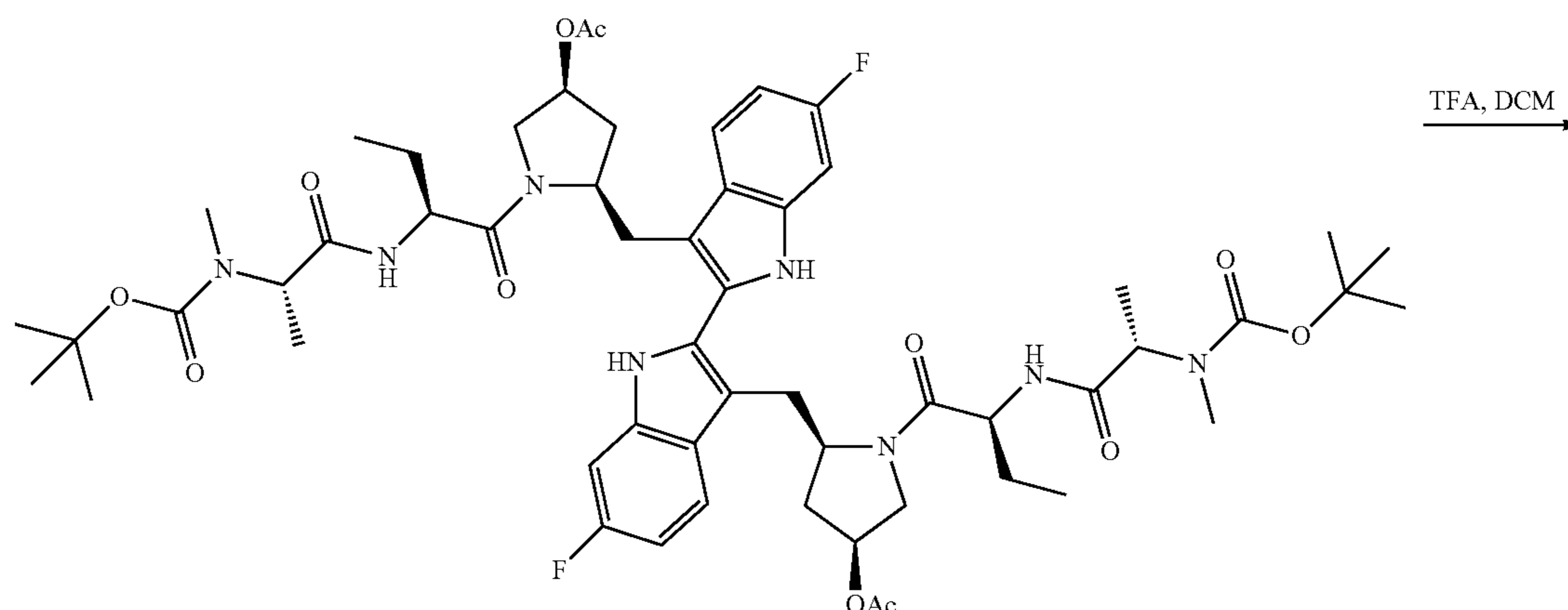
Scheme XIII
