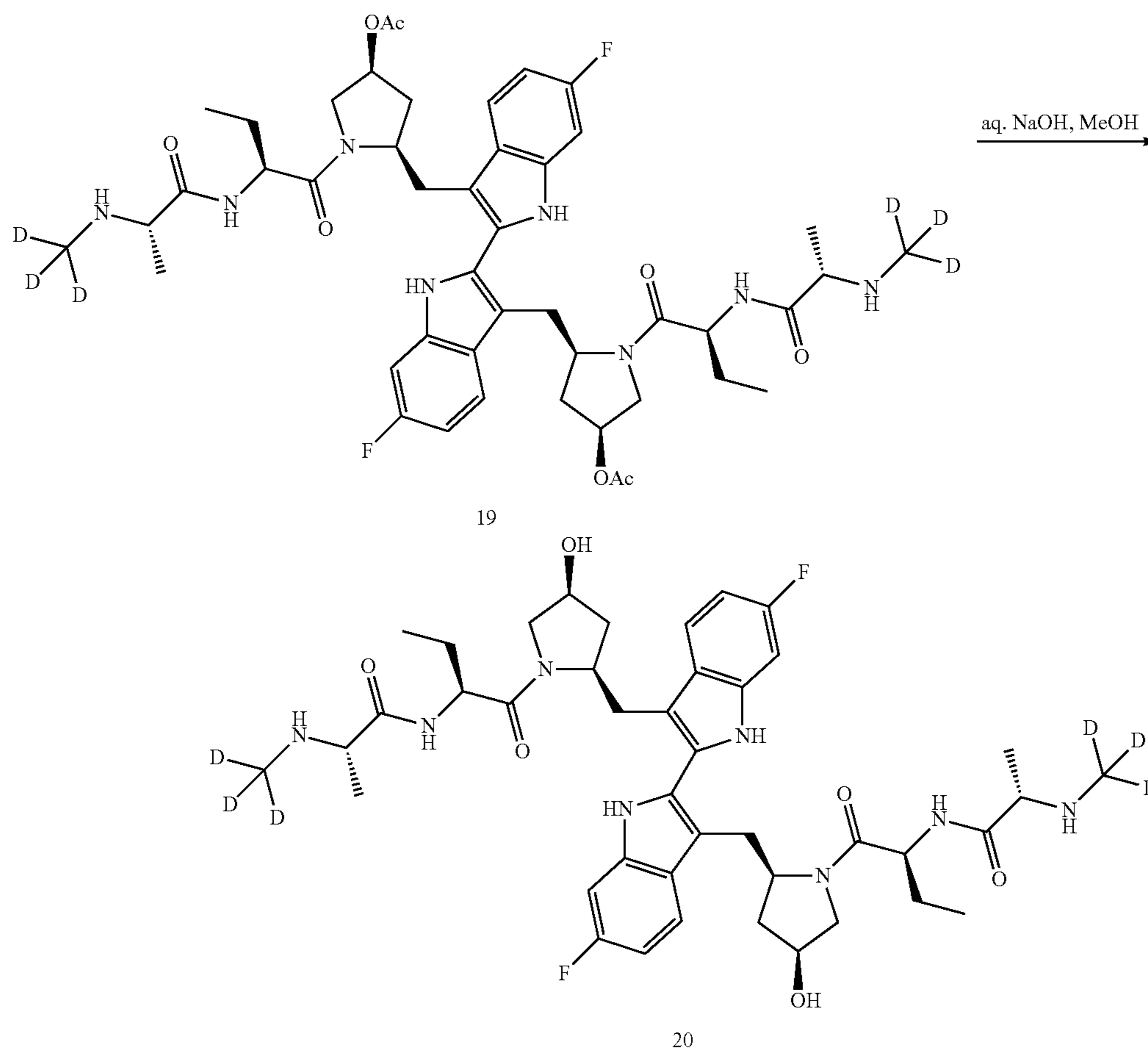
Scheme XVIII
