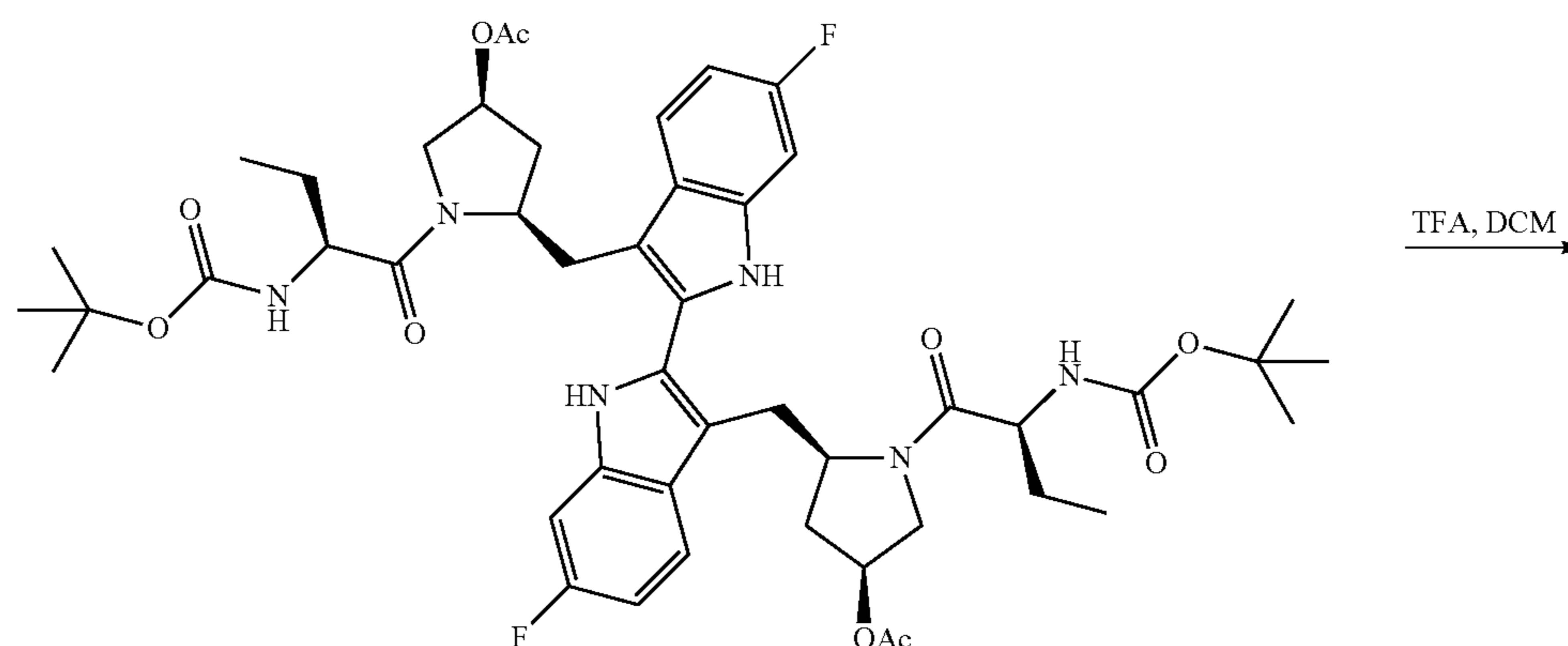
Scheme XI
