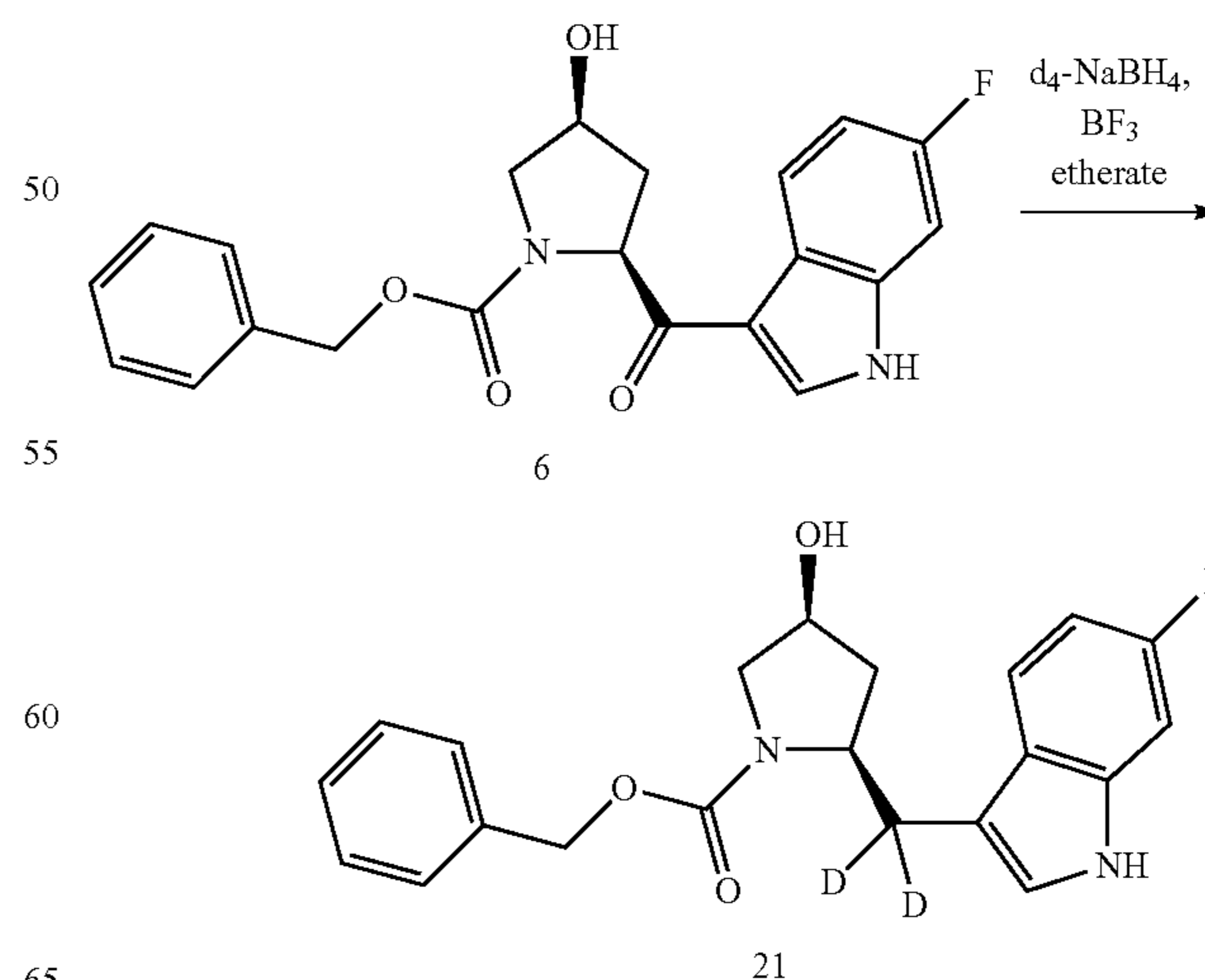
Scheme XIX
