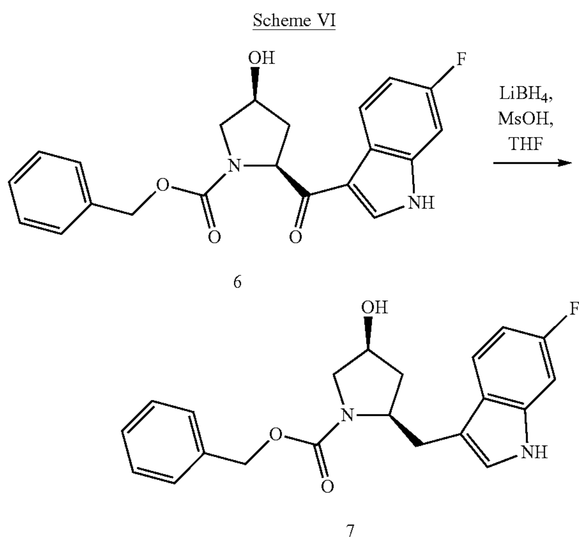
2-(6-Fluoro-1H-indol-3-ylmethyl)-4-hydroxy-pyrrolidine-1-carboxylic acid benzyl ester (7)
