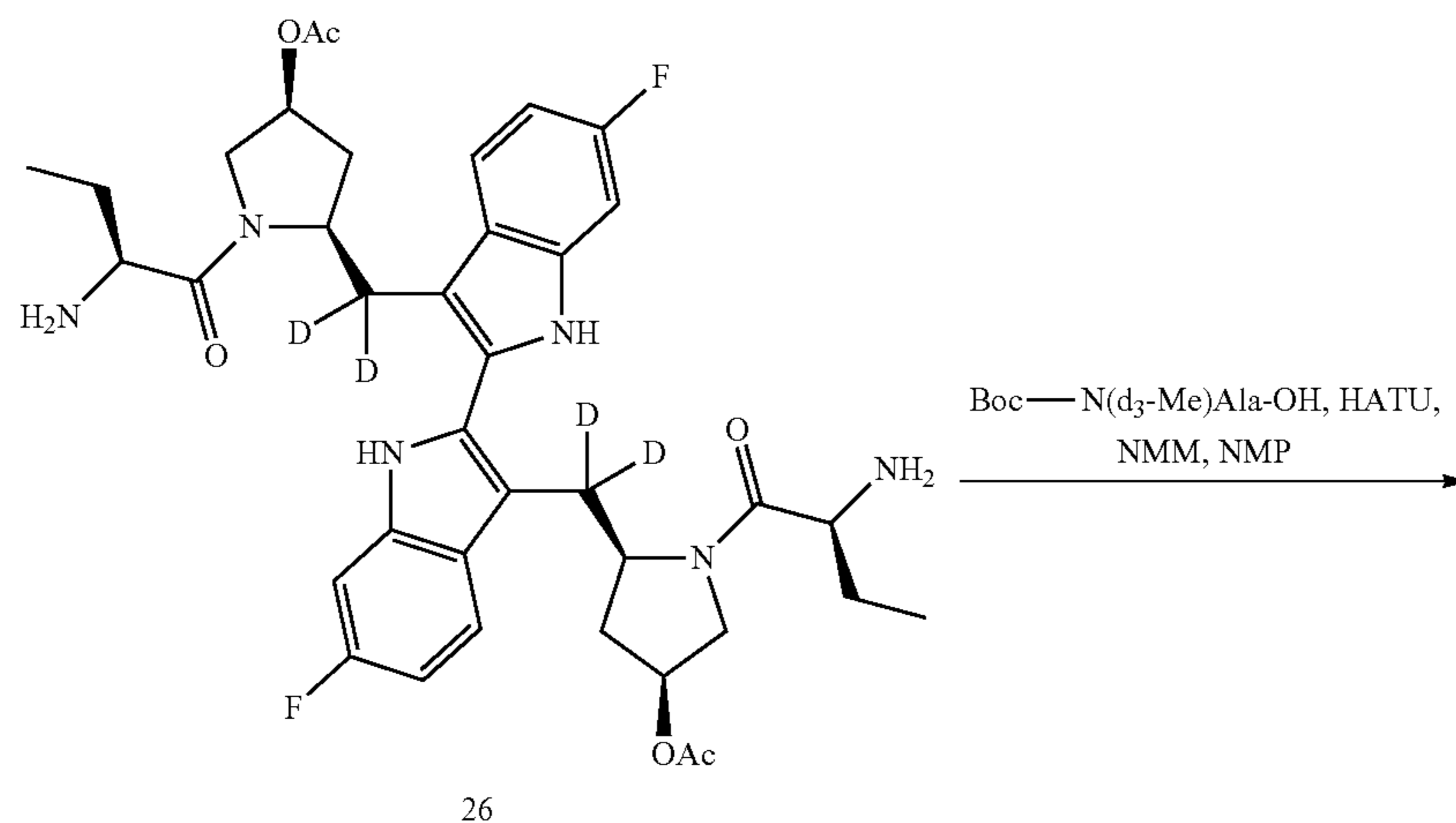
Scheme XXVIII
