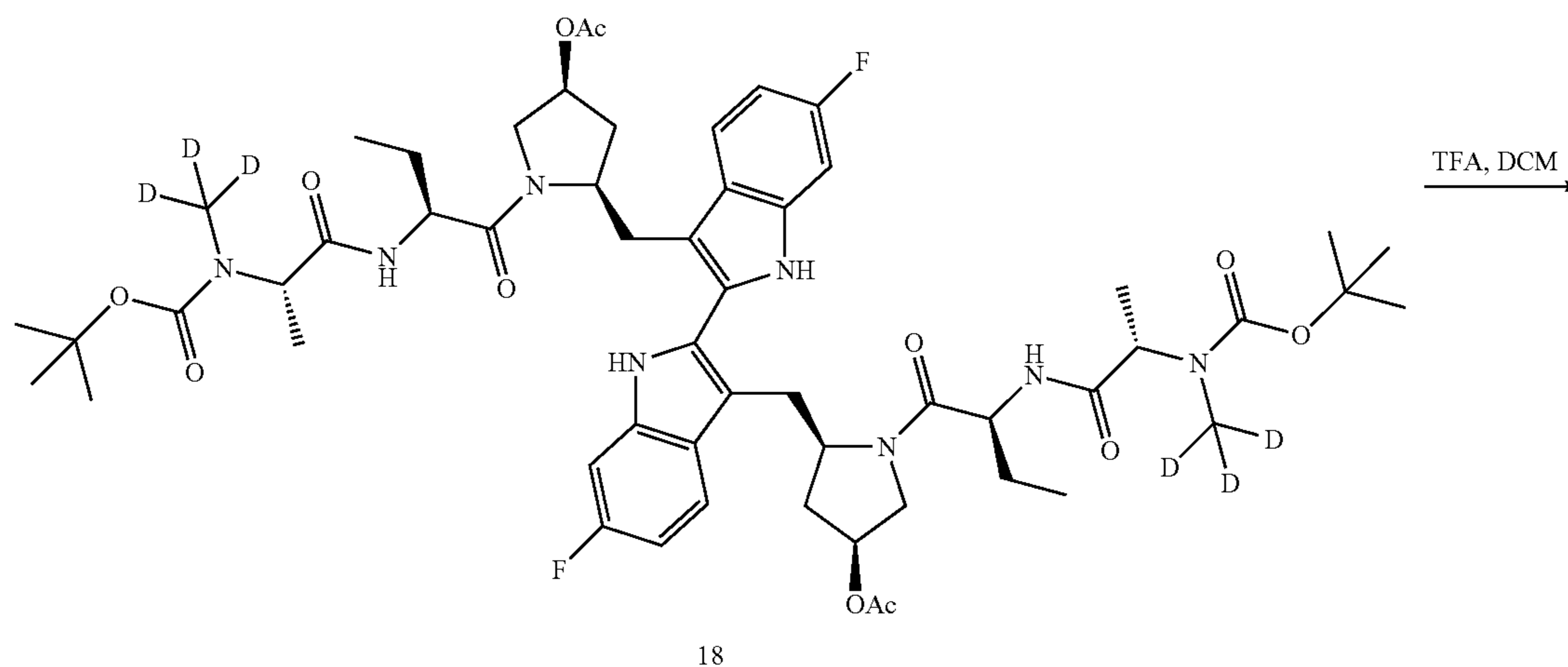
Scheme XVII
