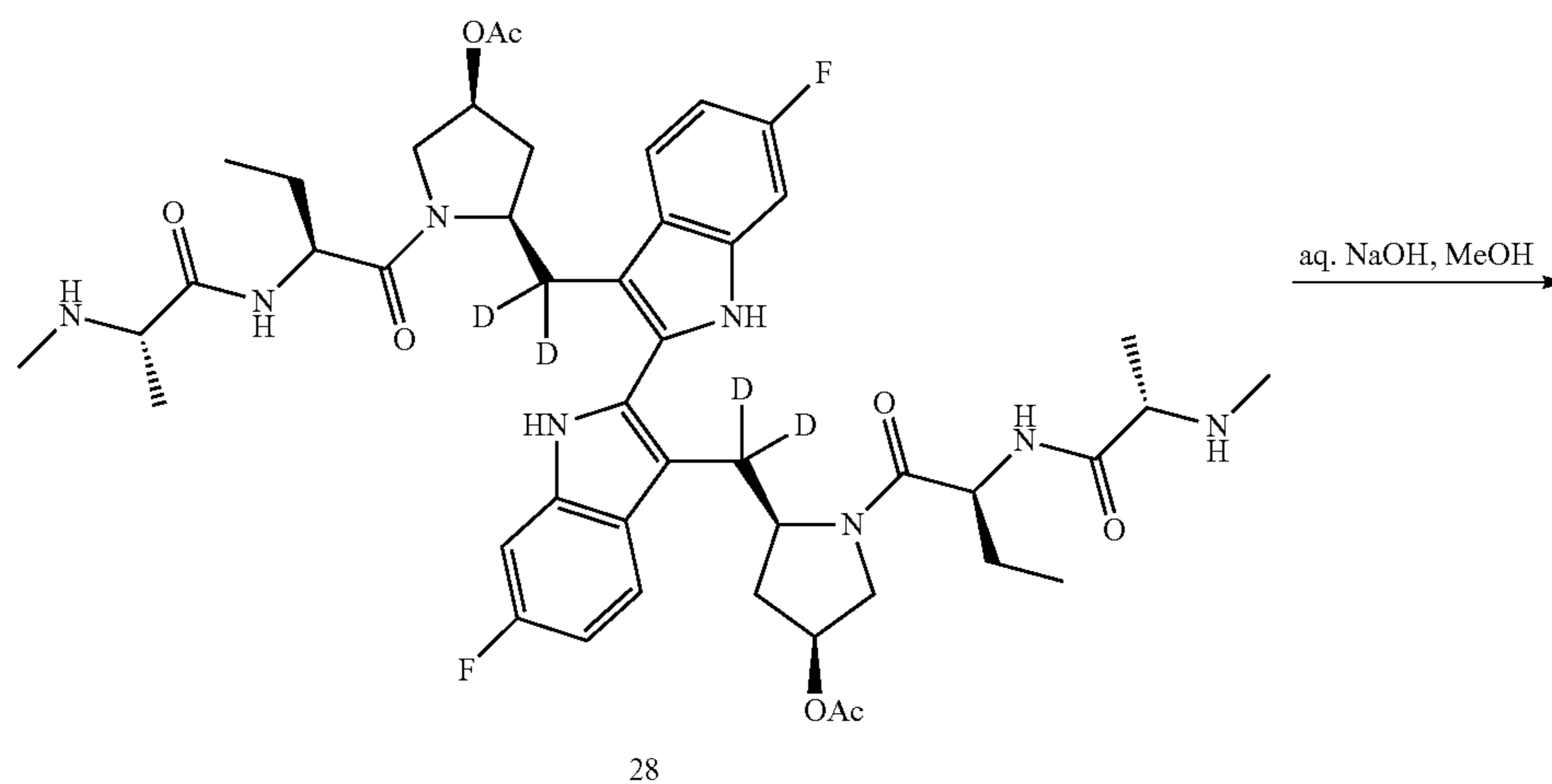
Scheme XXVII
