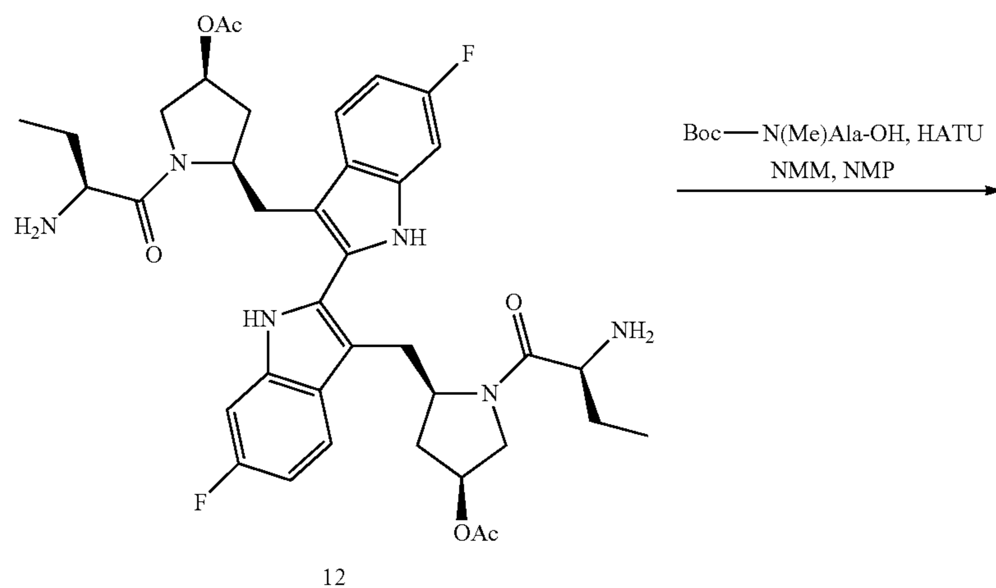
Scheme XVI
