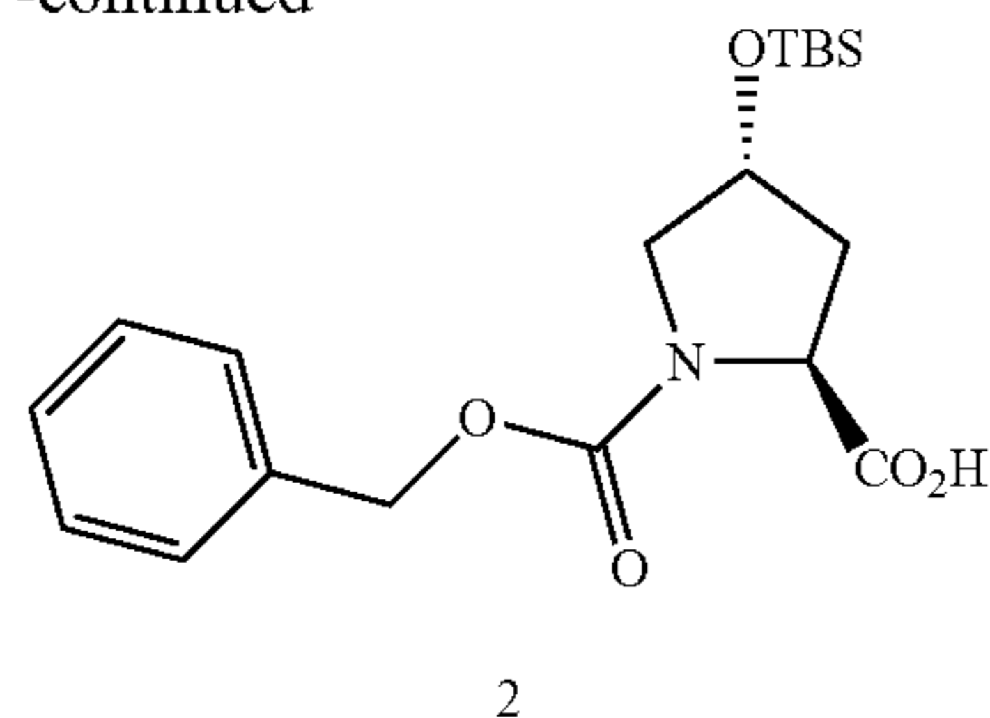
4-(tert-Butyl-dimethyl-silyloxy)-pyrrolidine-1,2-dicarboxylic acid 1-benzyl ester (2)
