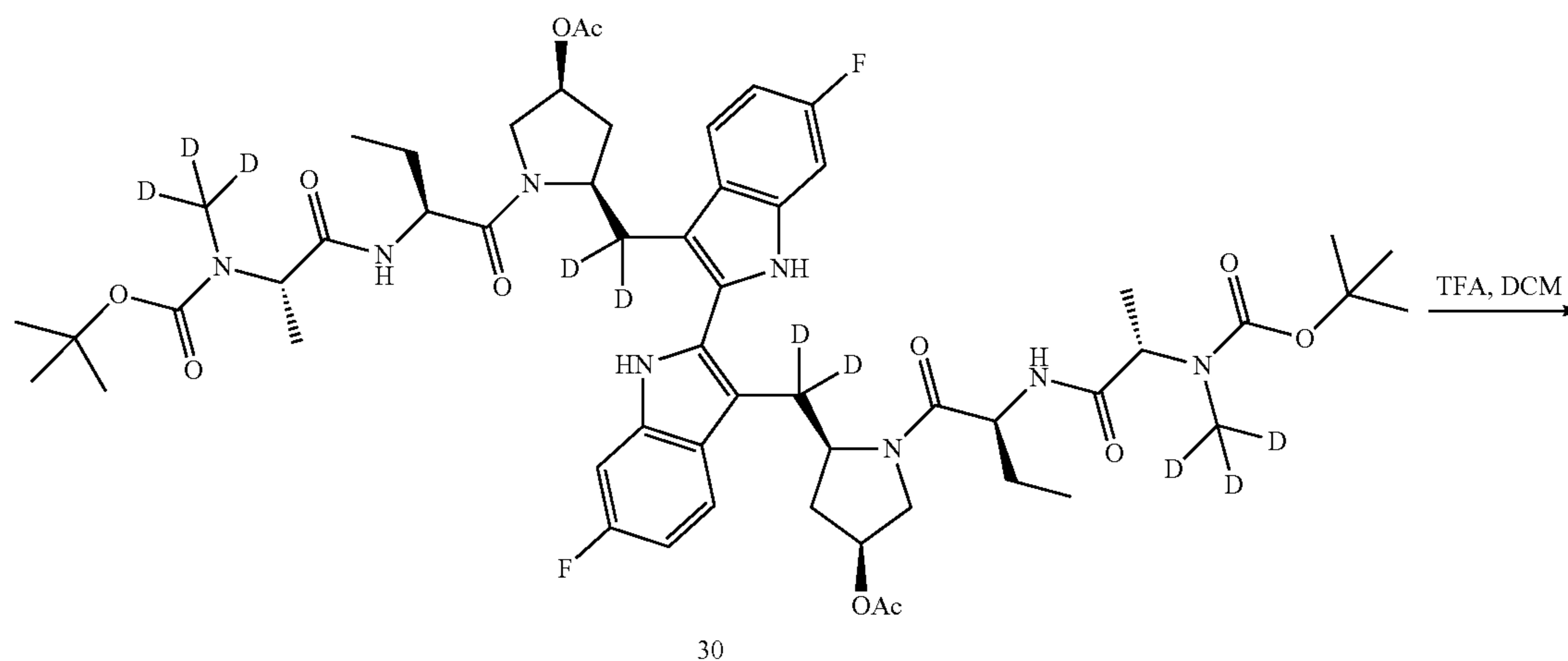
Scheme XXIX
