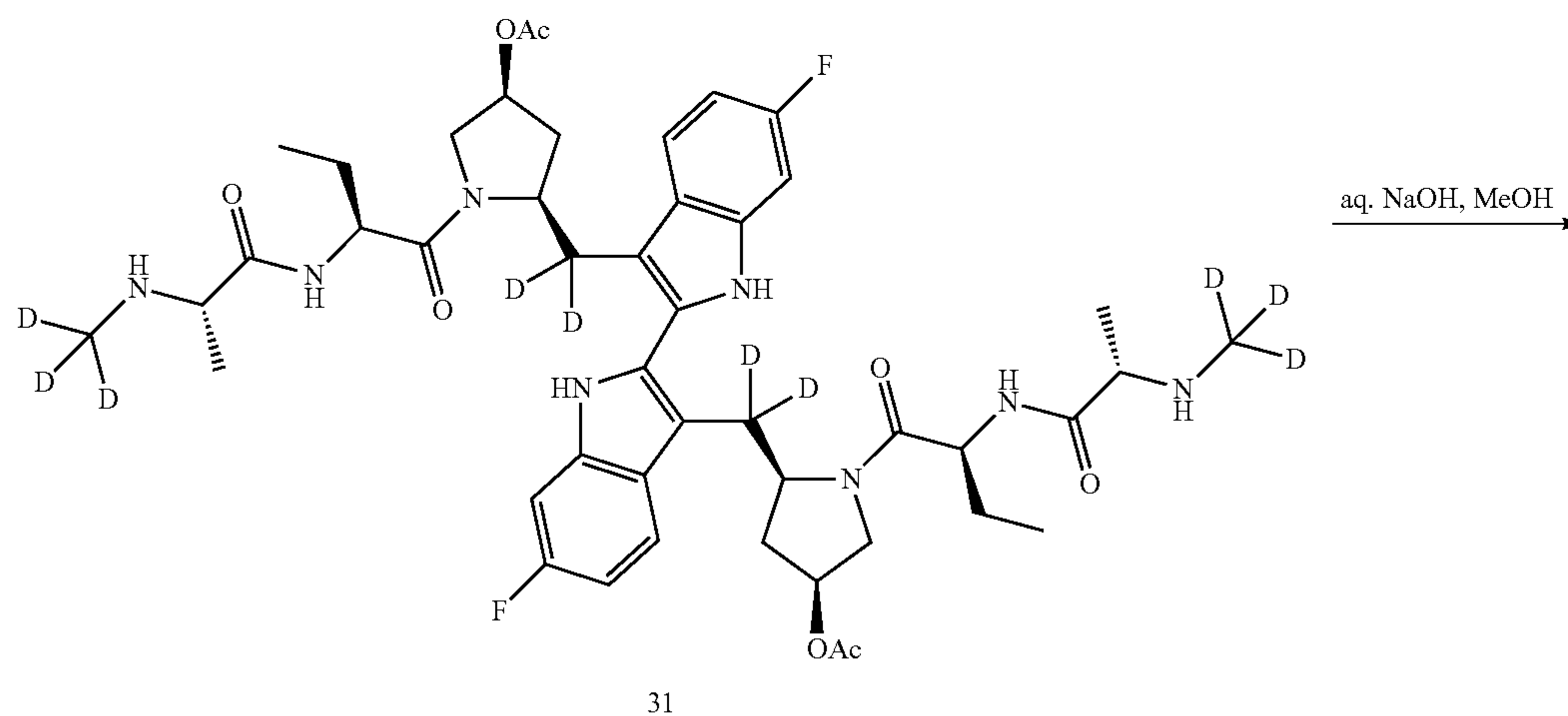
Scheme XXX
