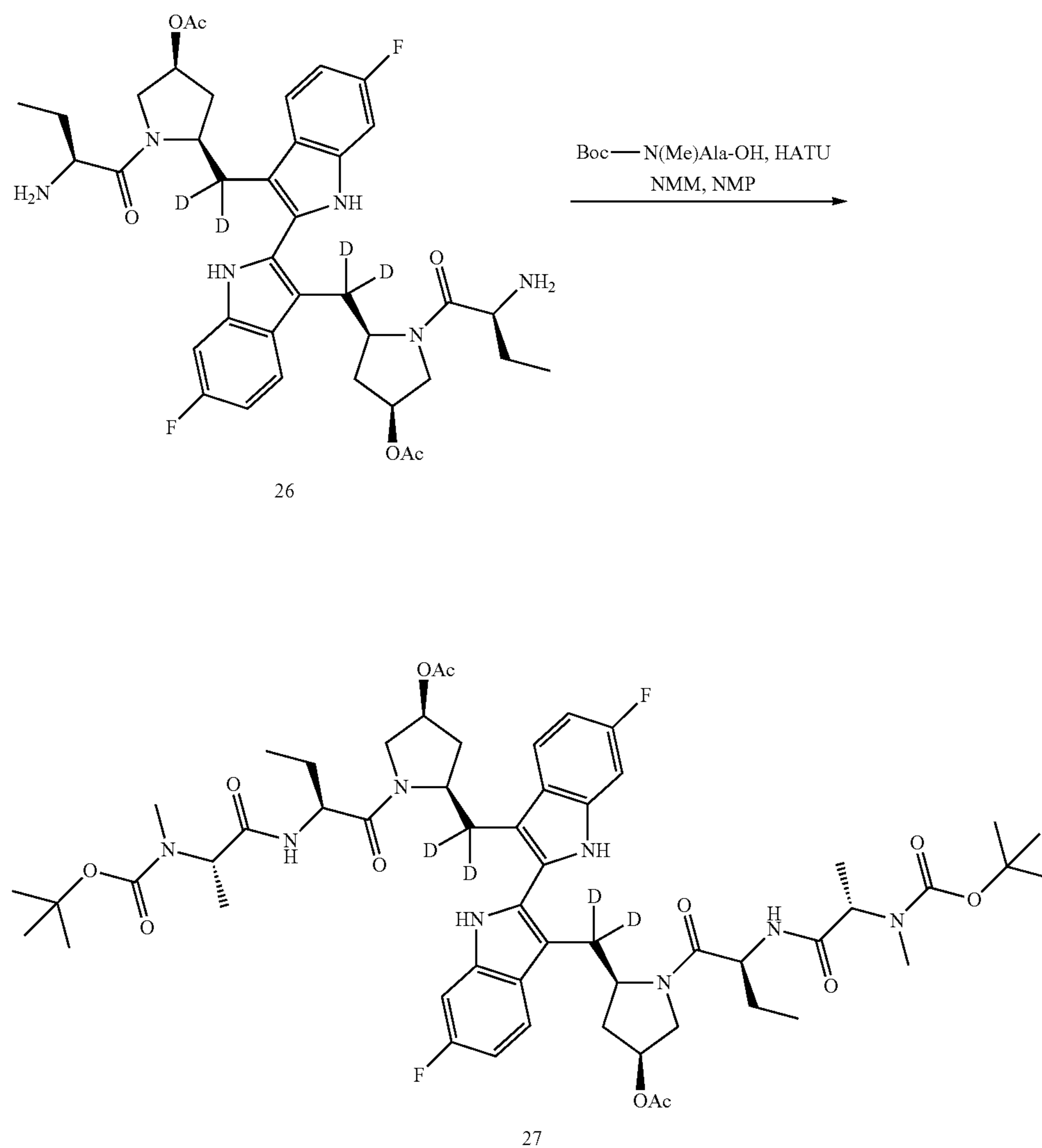
Scheme XXV
