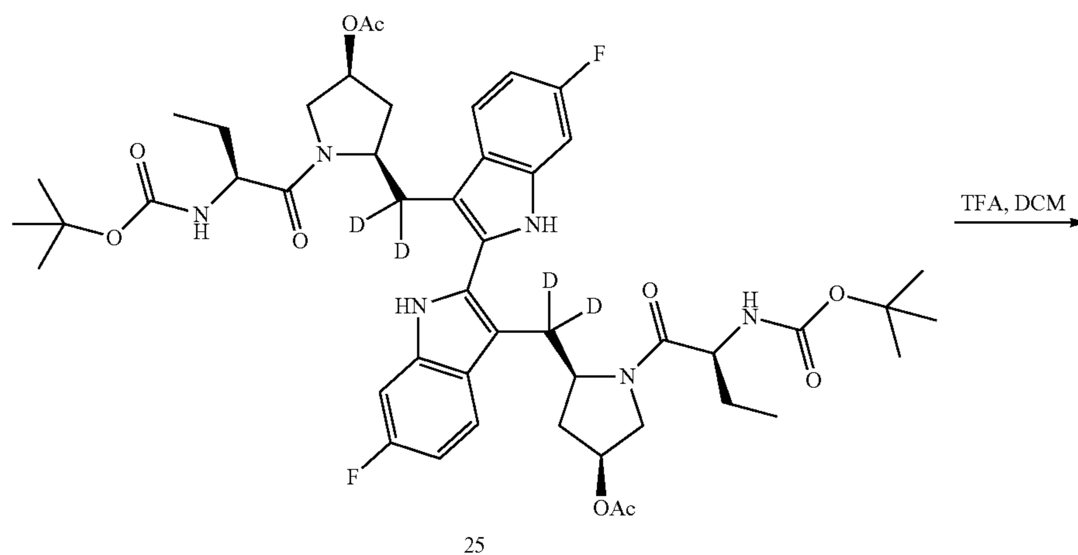
Scheme XXIV
