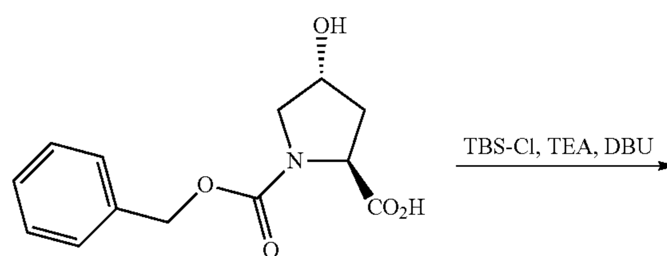
Scheme I
