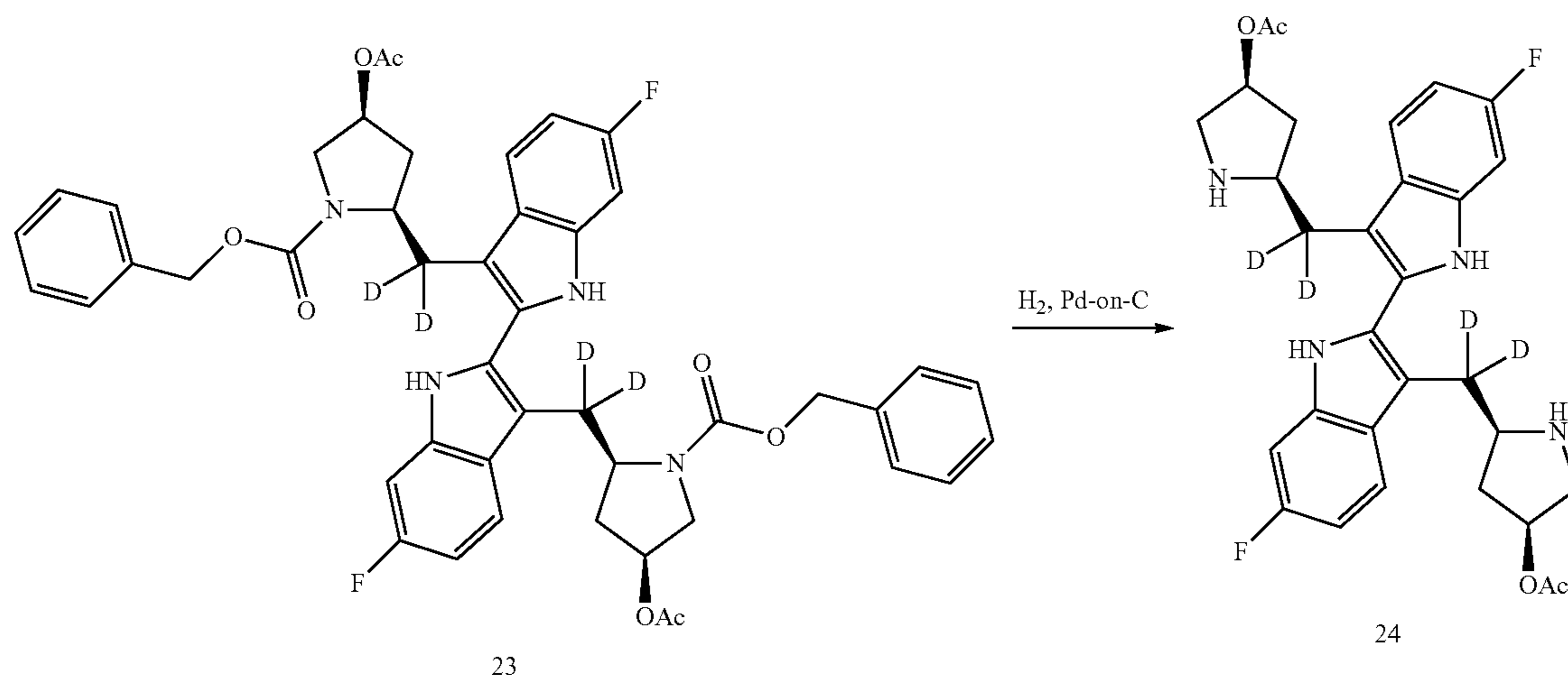
Scheme XXII
