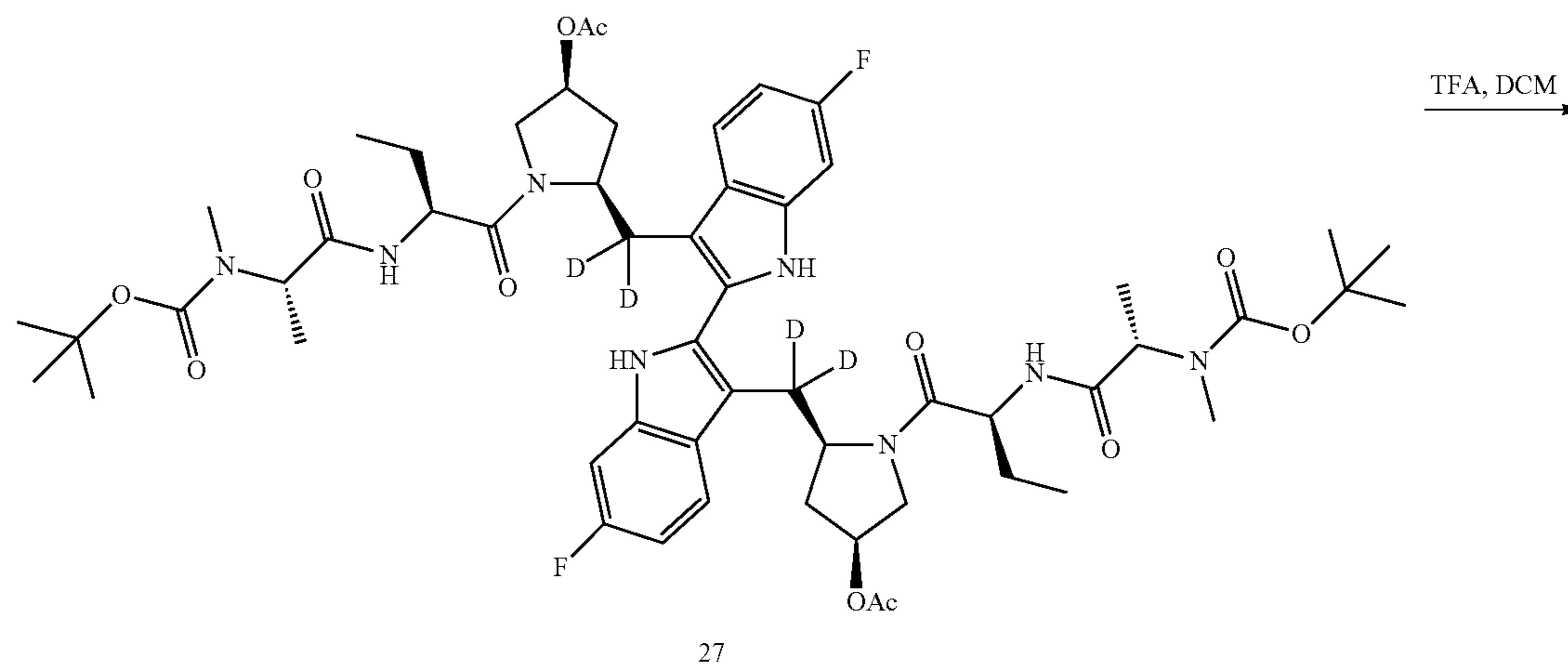
Scheme XXVI
