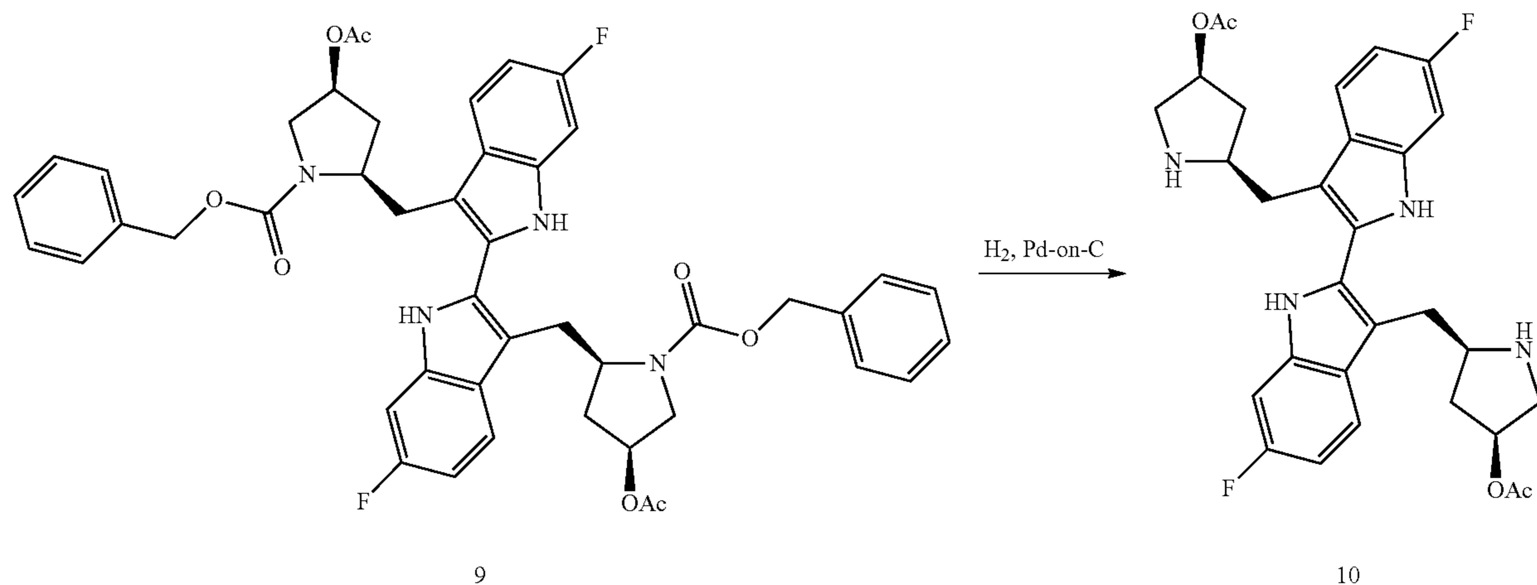
Scheme IX
