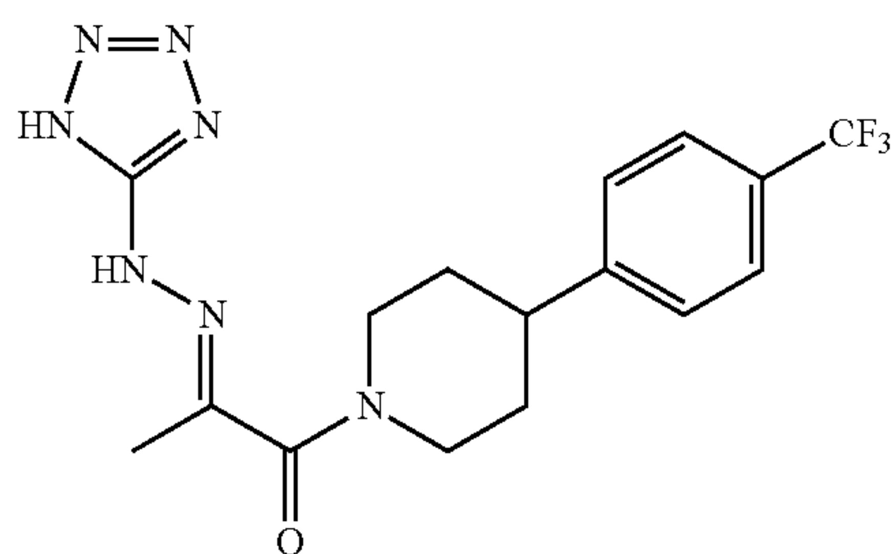
SRX201: (2E)-1-Oxo-1-{4-[4-(trifluoromethyl)phenyl]piperidin-1-yl}acetone 1H-tetrazol-5-ylhydrazone
