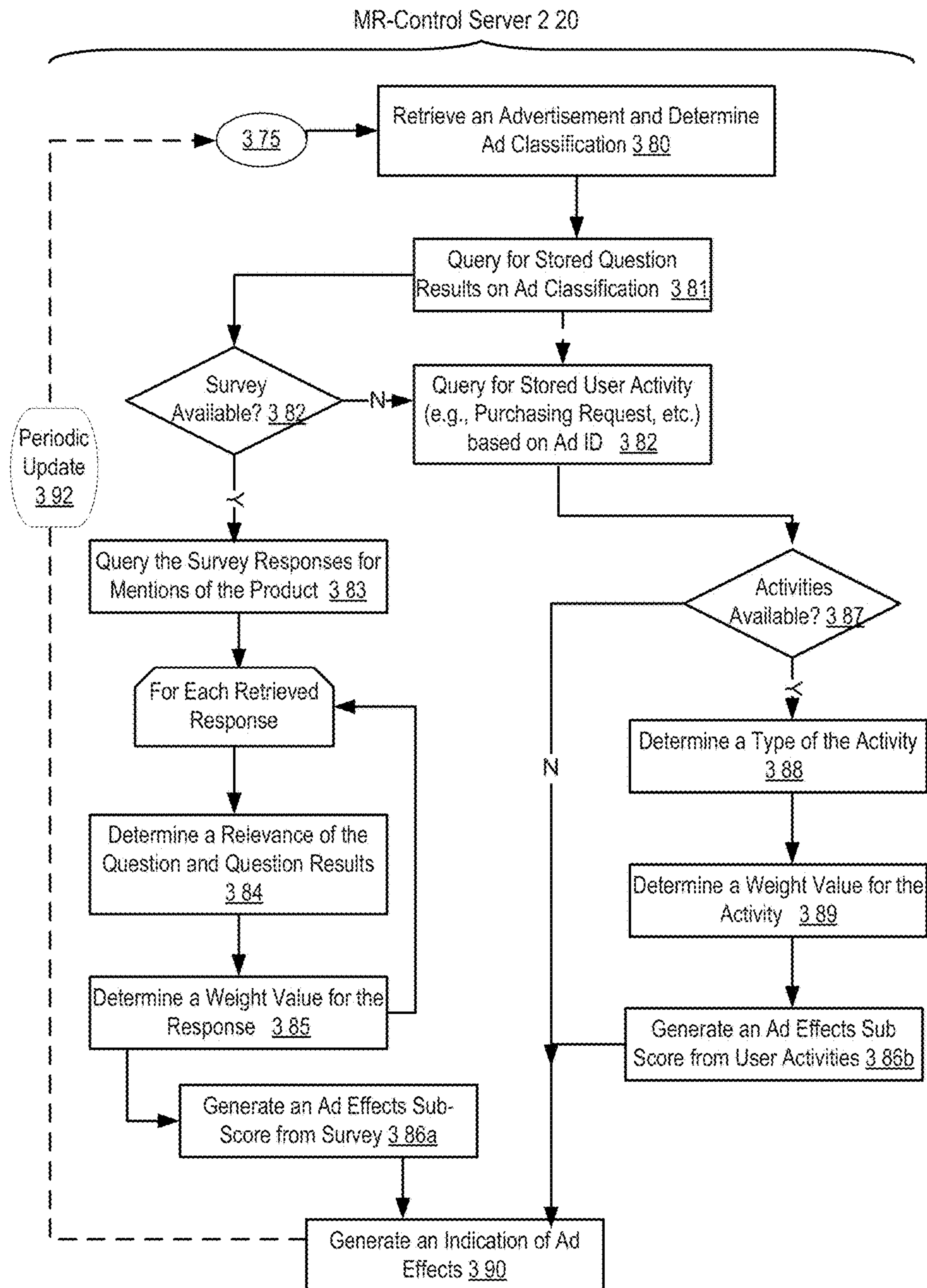
MR-Control Example Logic Flow: Ad Delivery Analysis
