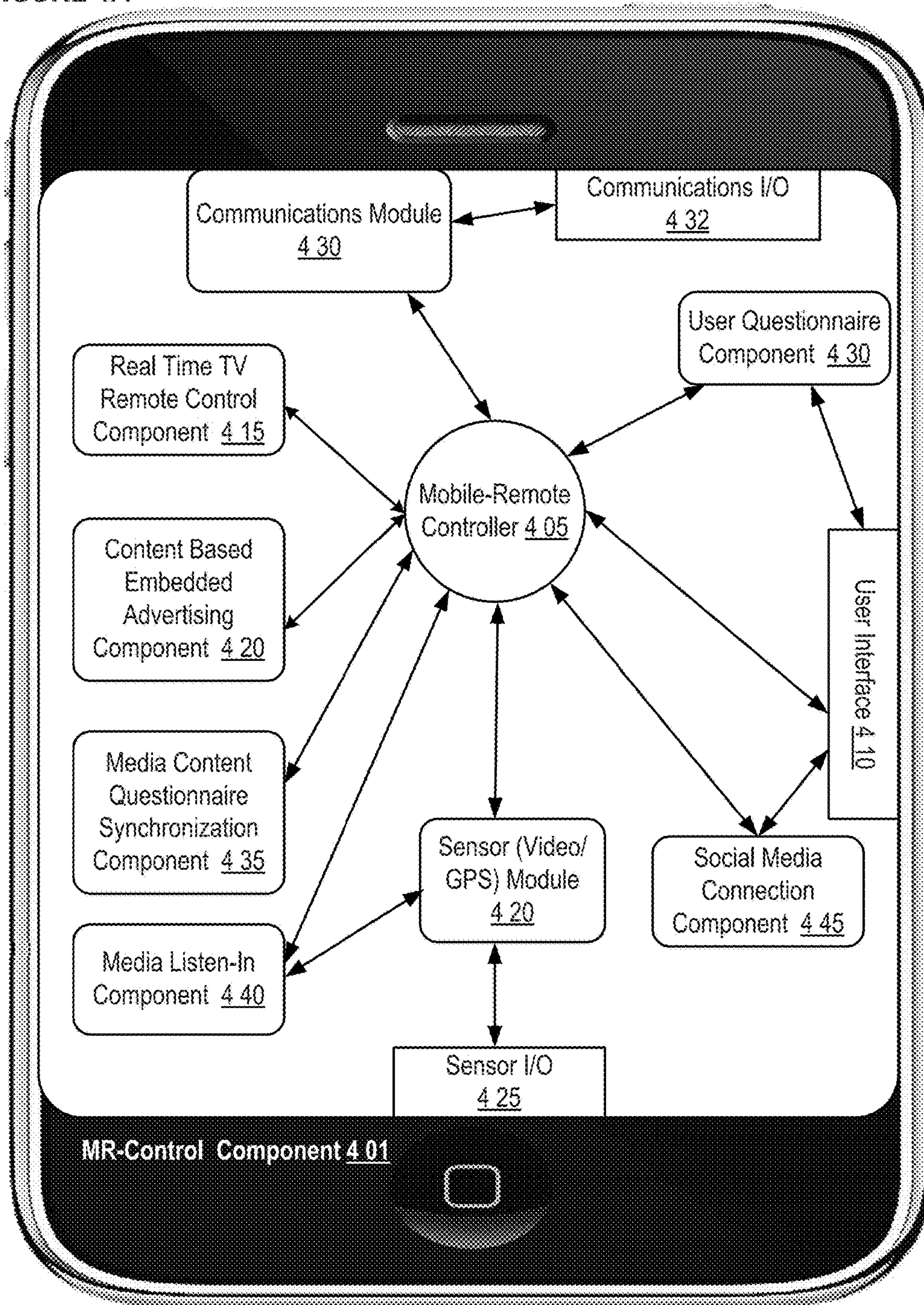
MR-Control Example Client Mobile App Block View
