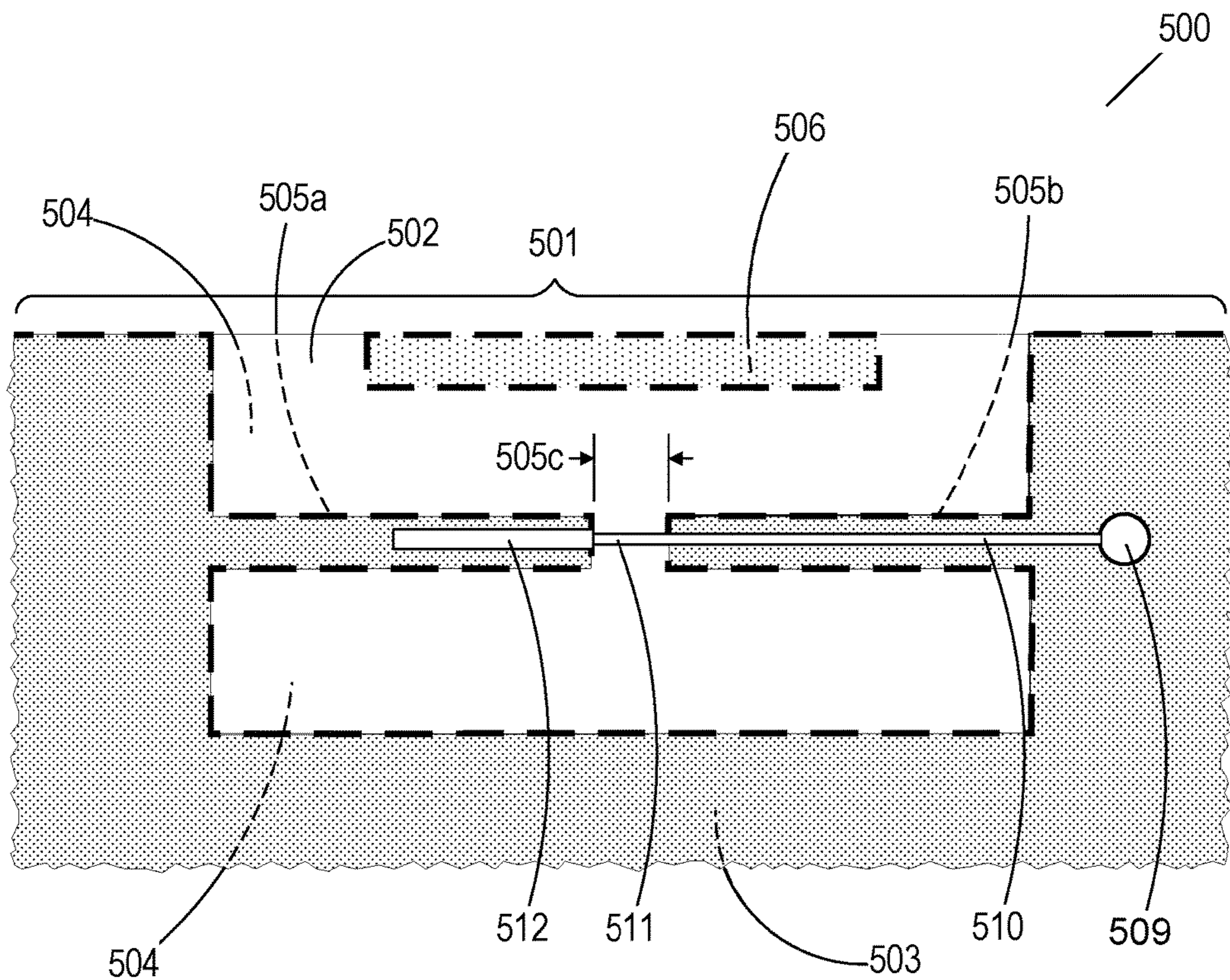
FIG. 5 (bottom view)
