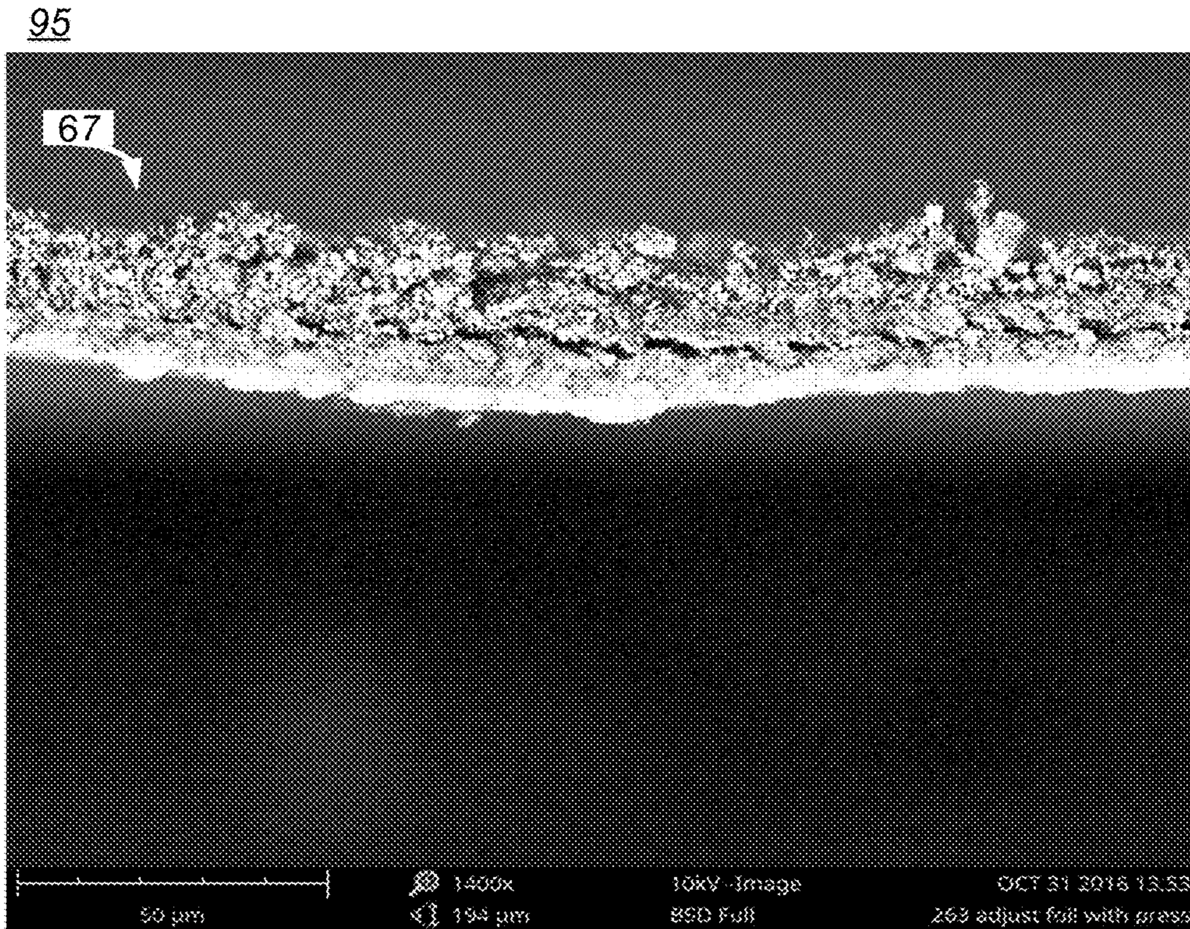
Figure 17A – Prior art
