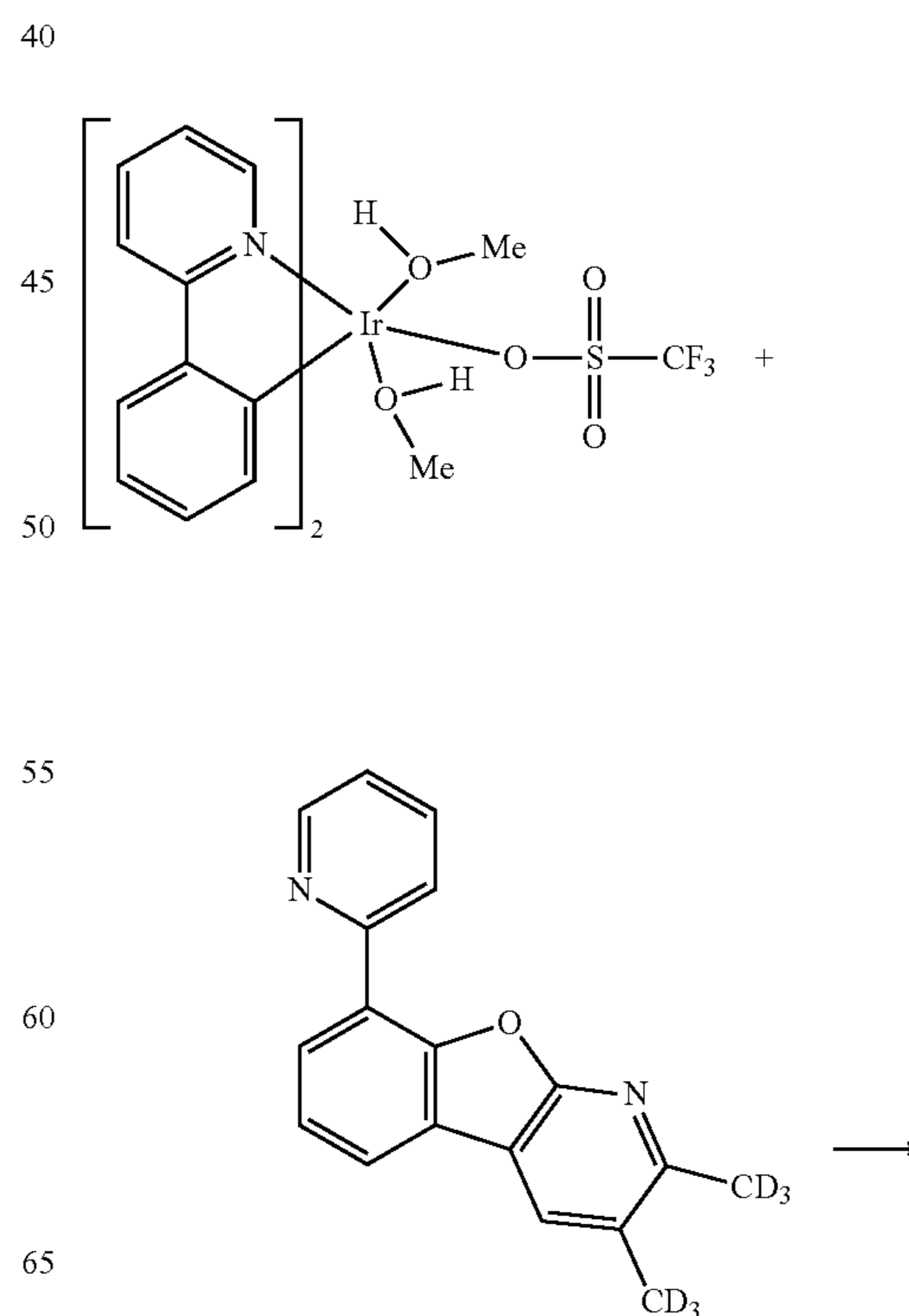
Synthesis Example 2 for an Example of the Novel Compound, Compound \text{IrL}_{A7}(\text{L}_{B1})_2
