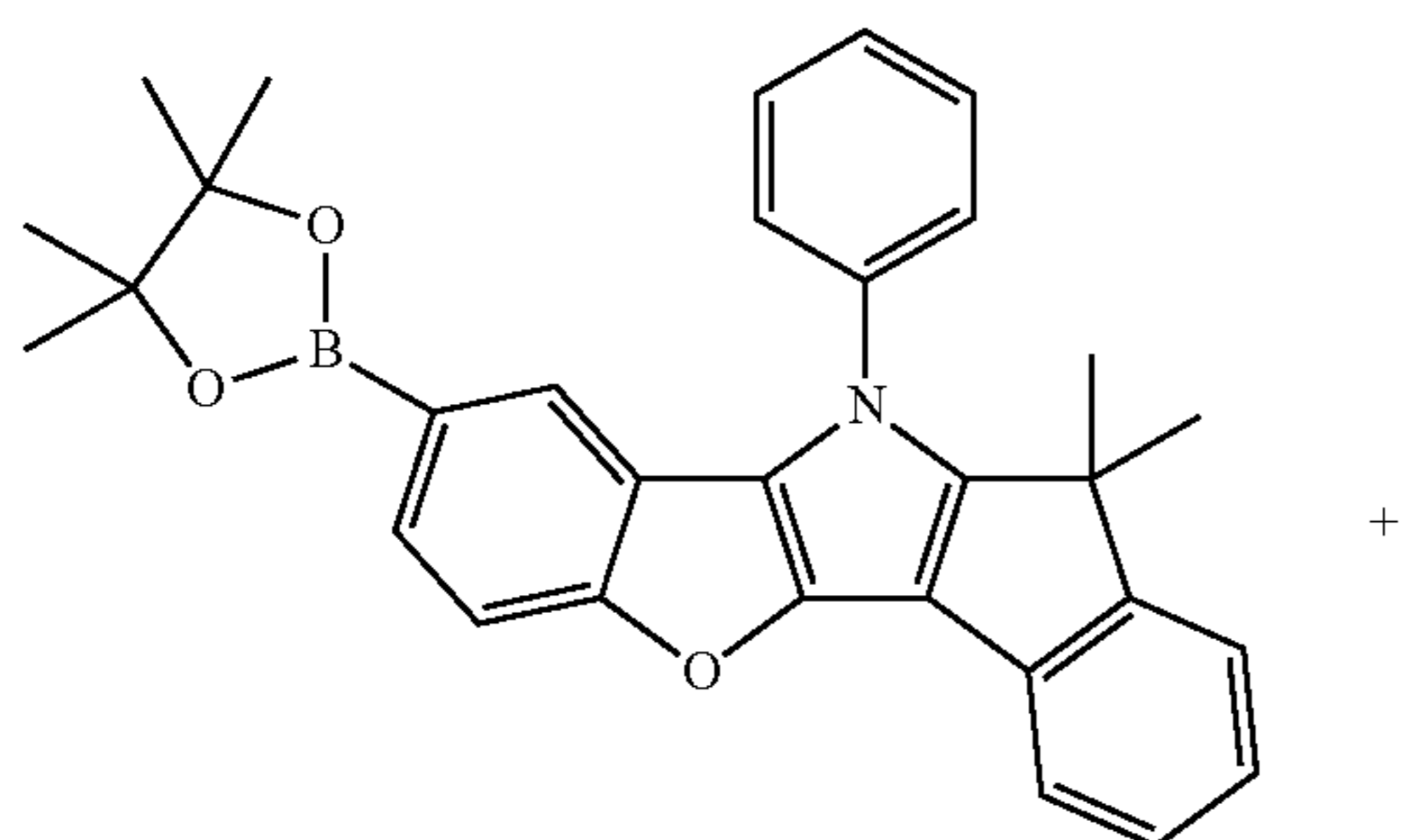
Intermediate H
