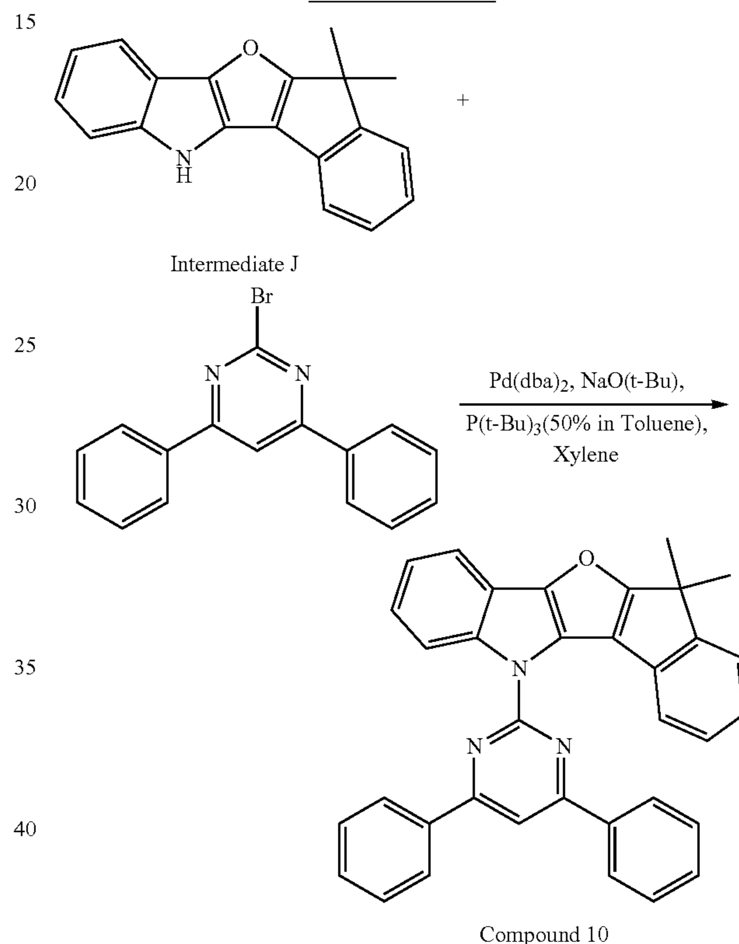
Reaction Scheme 10
