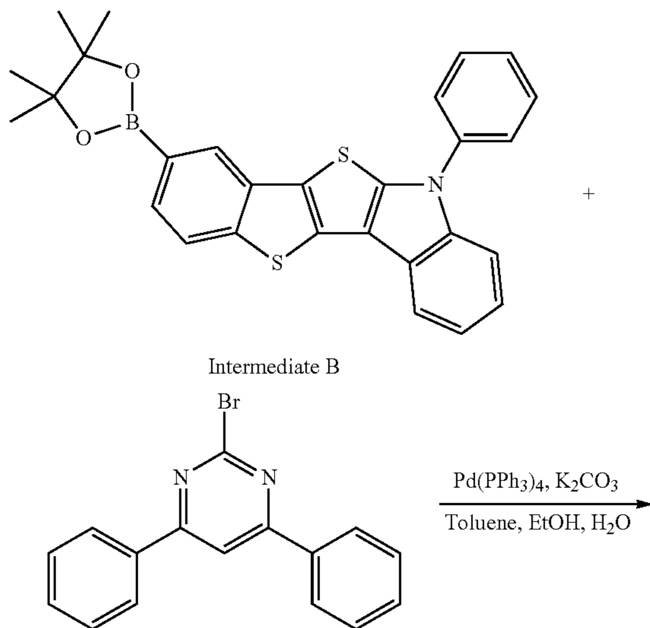
Reaction Scheme 2
