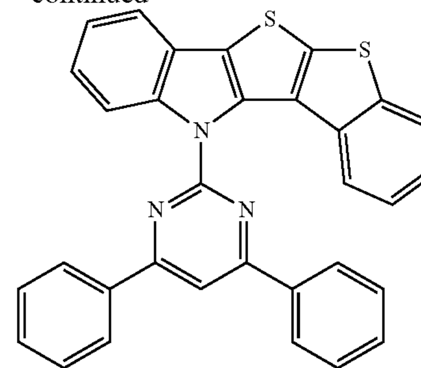
Compound 4
