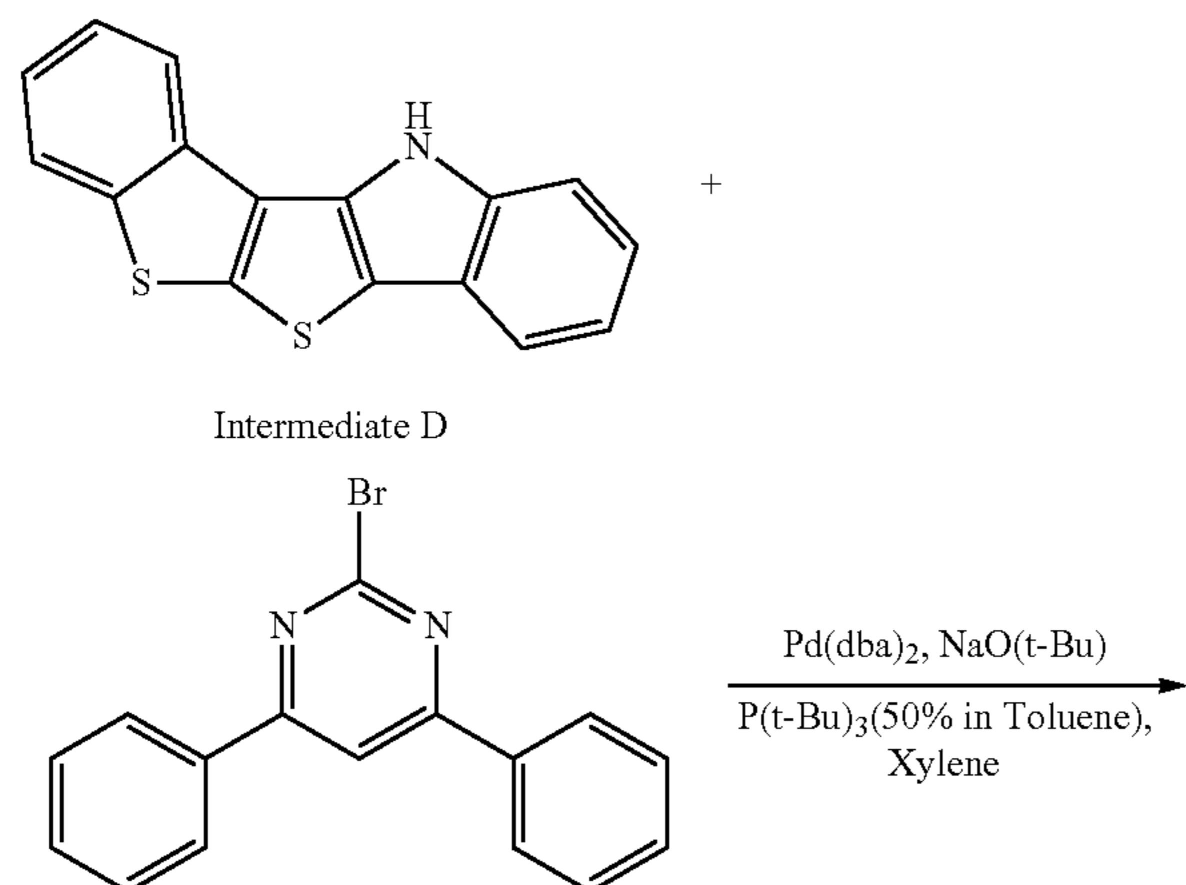
Reaction Scheme 4
