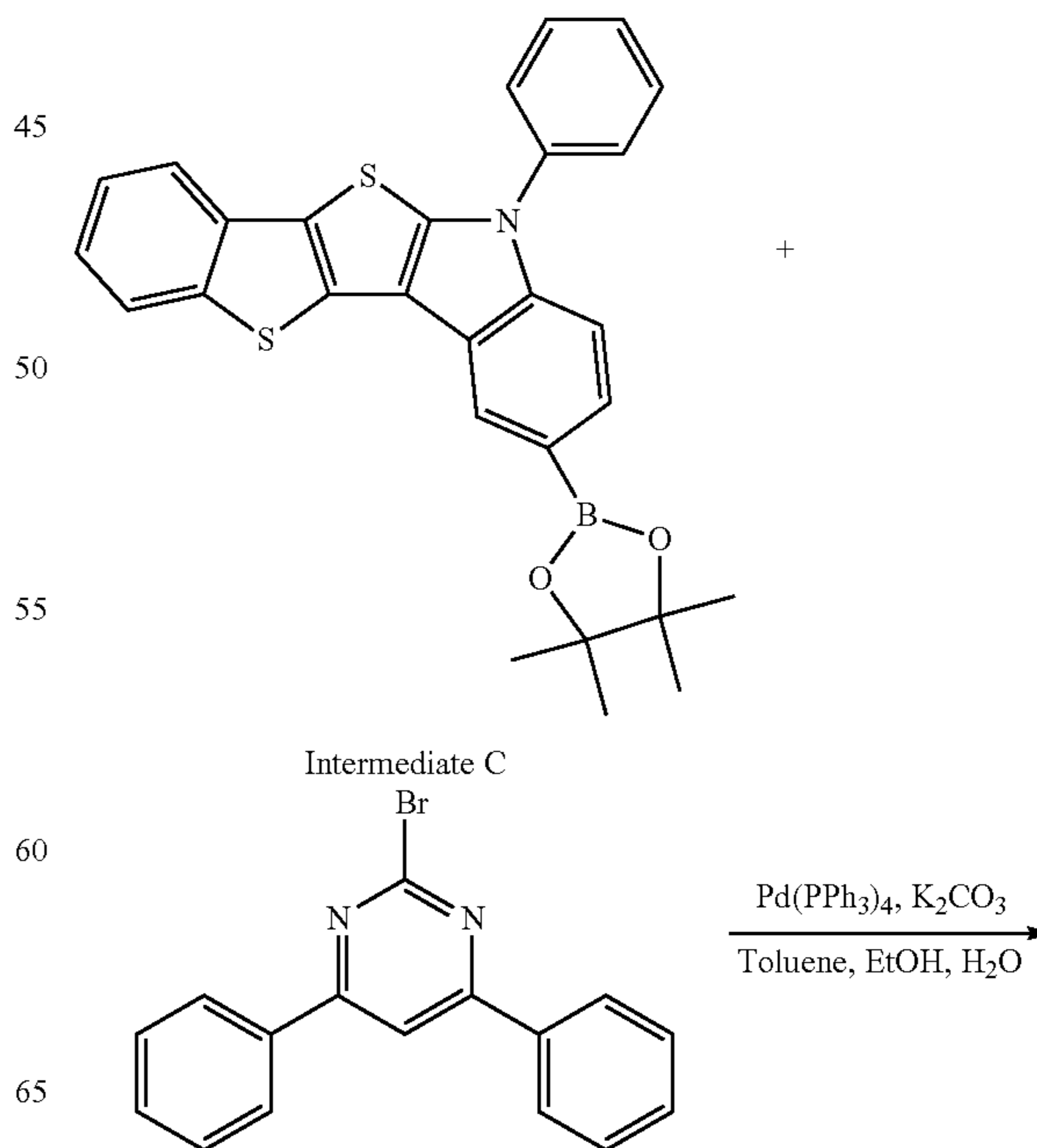
Reaction Scheme 3
