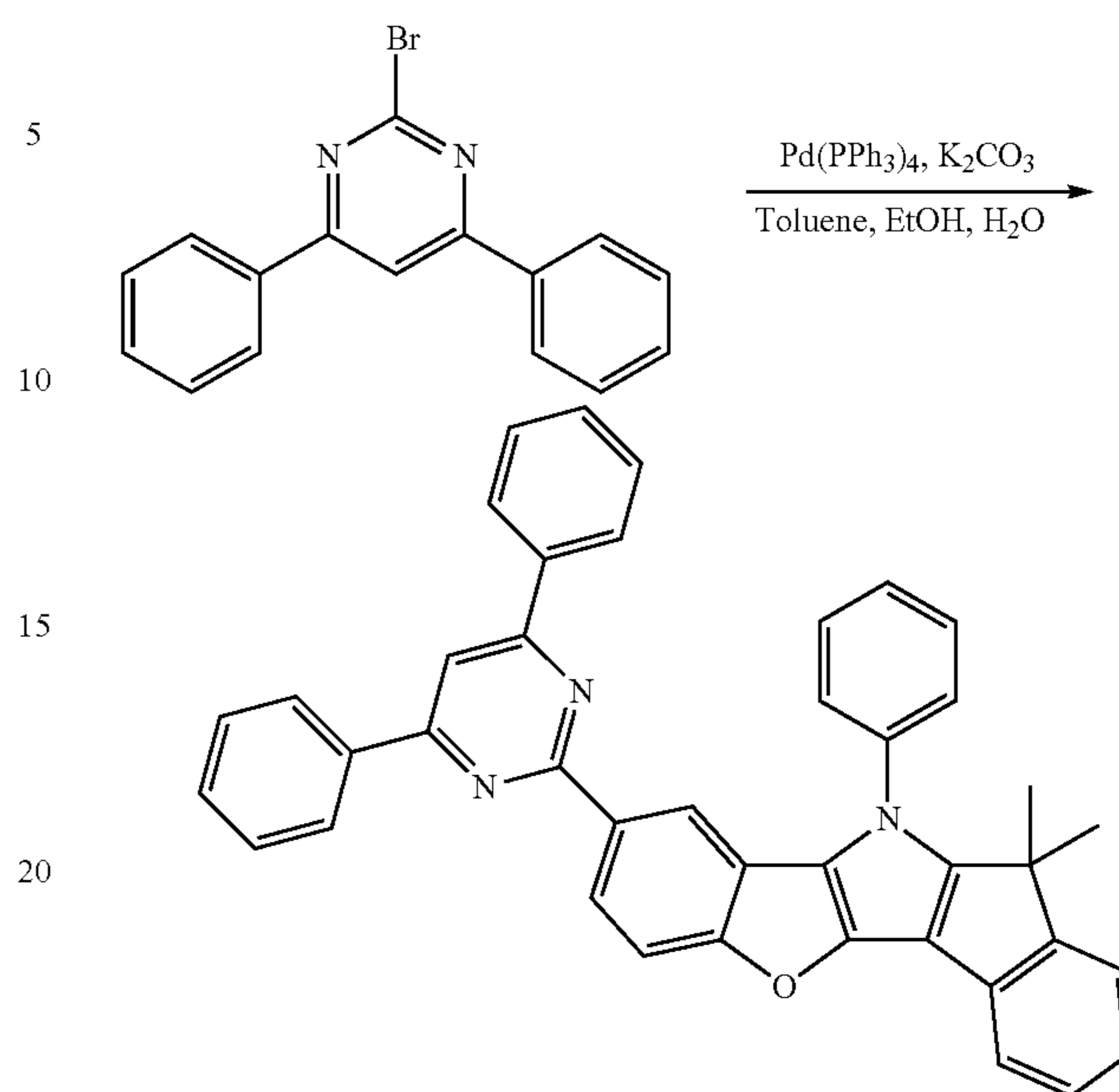
Compound 8
