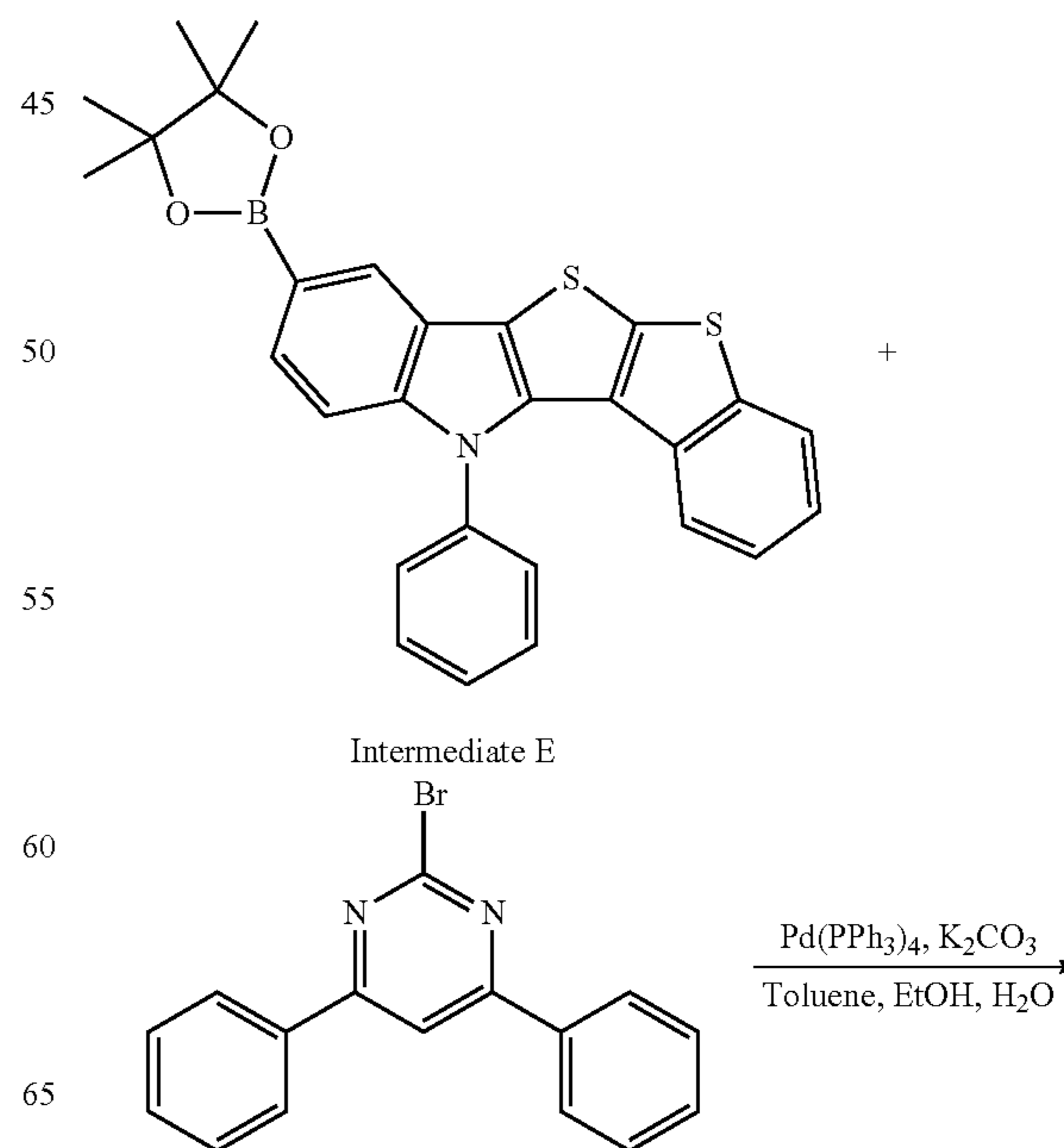
Reaction Scheme 5
