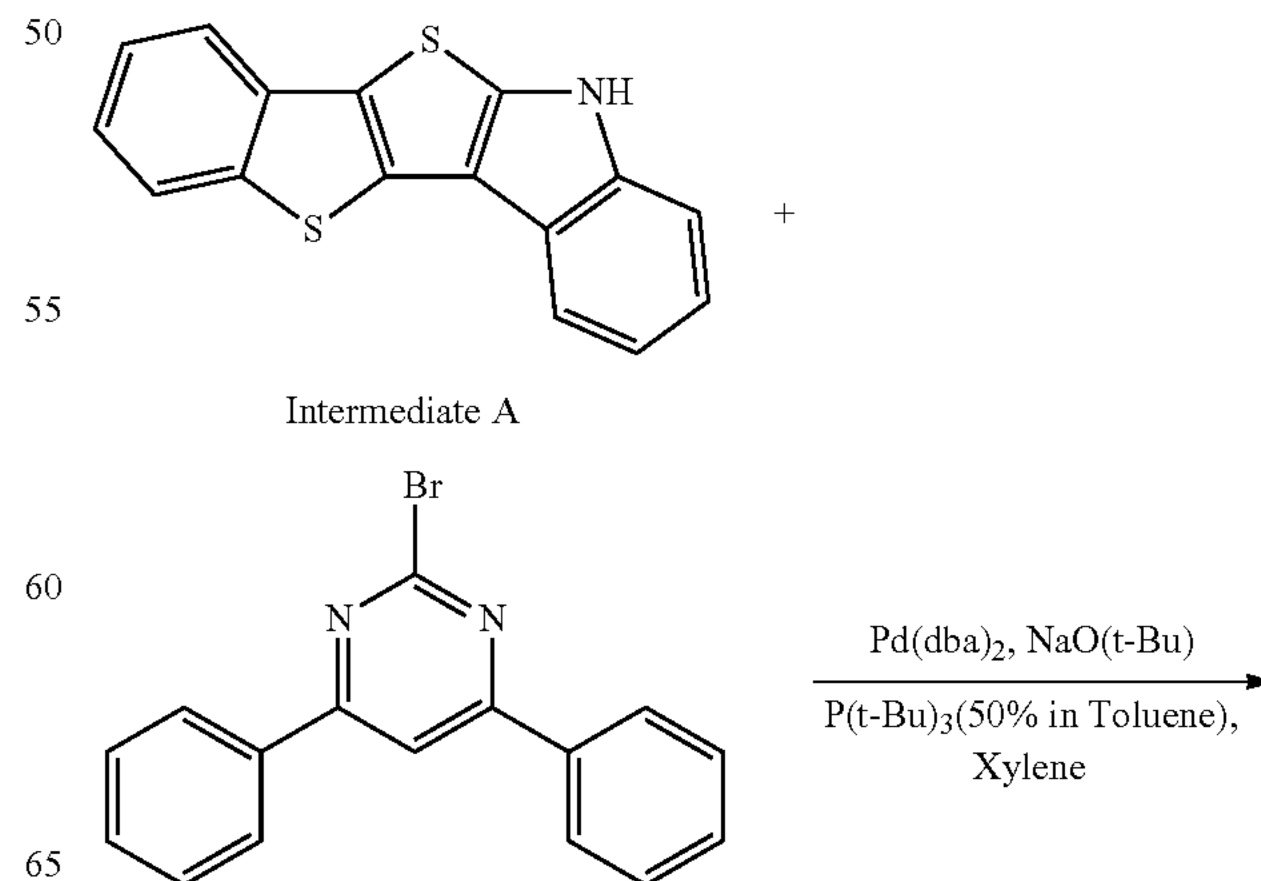
Reaction Scheme 1
