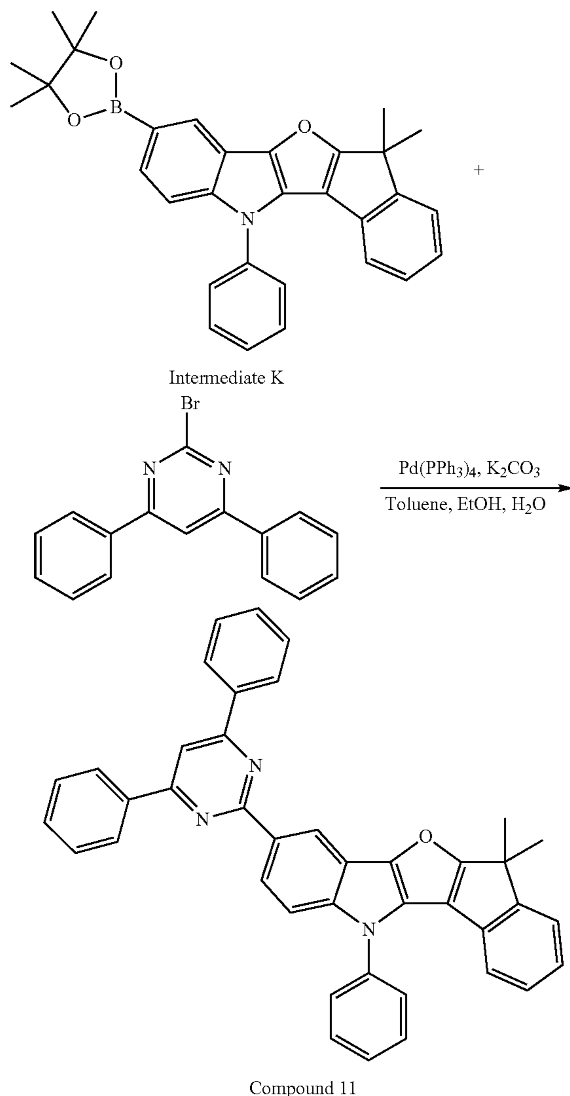
Reaction Scheme 11
