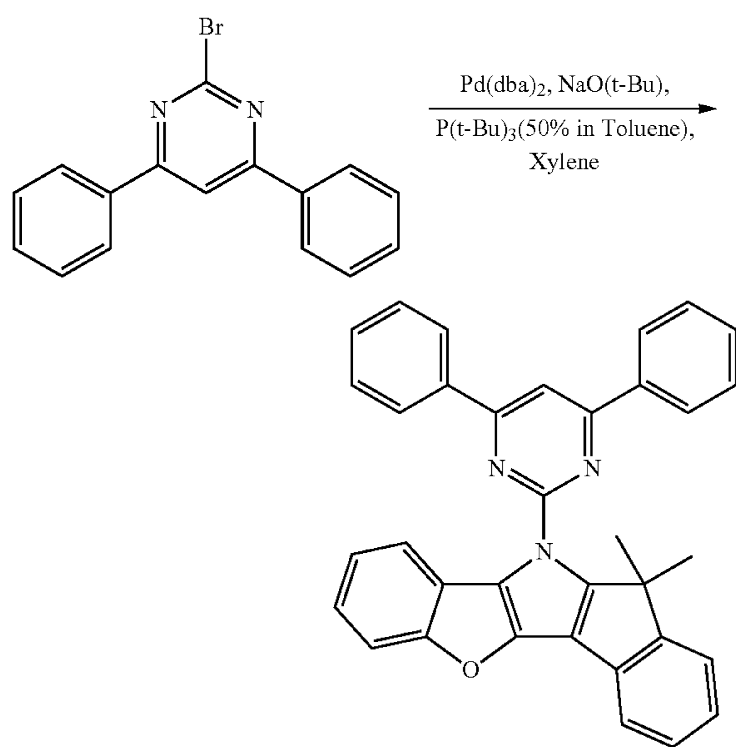
Compound 7
