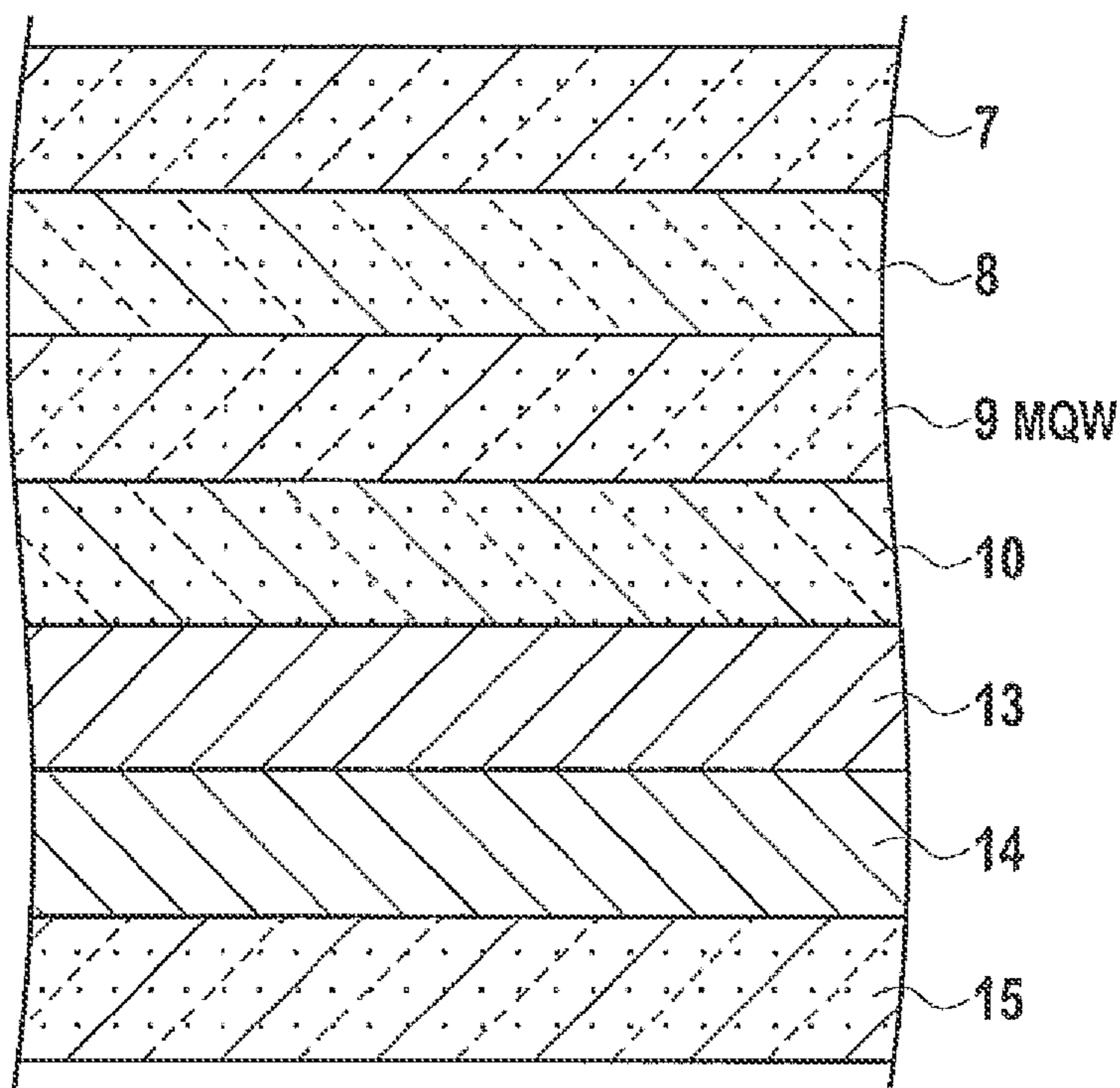
FIG. 23 PRIOR ART
