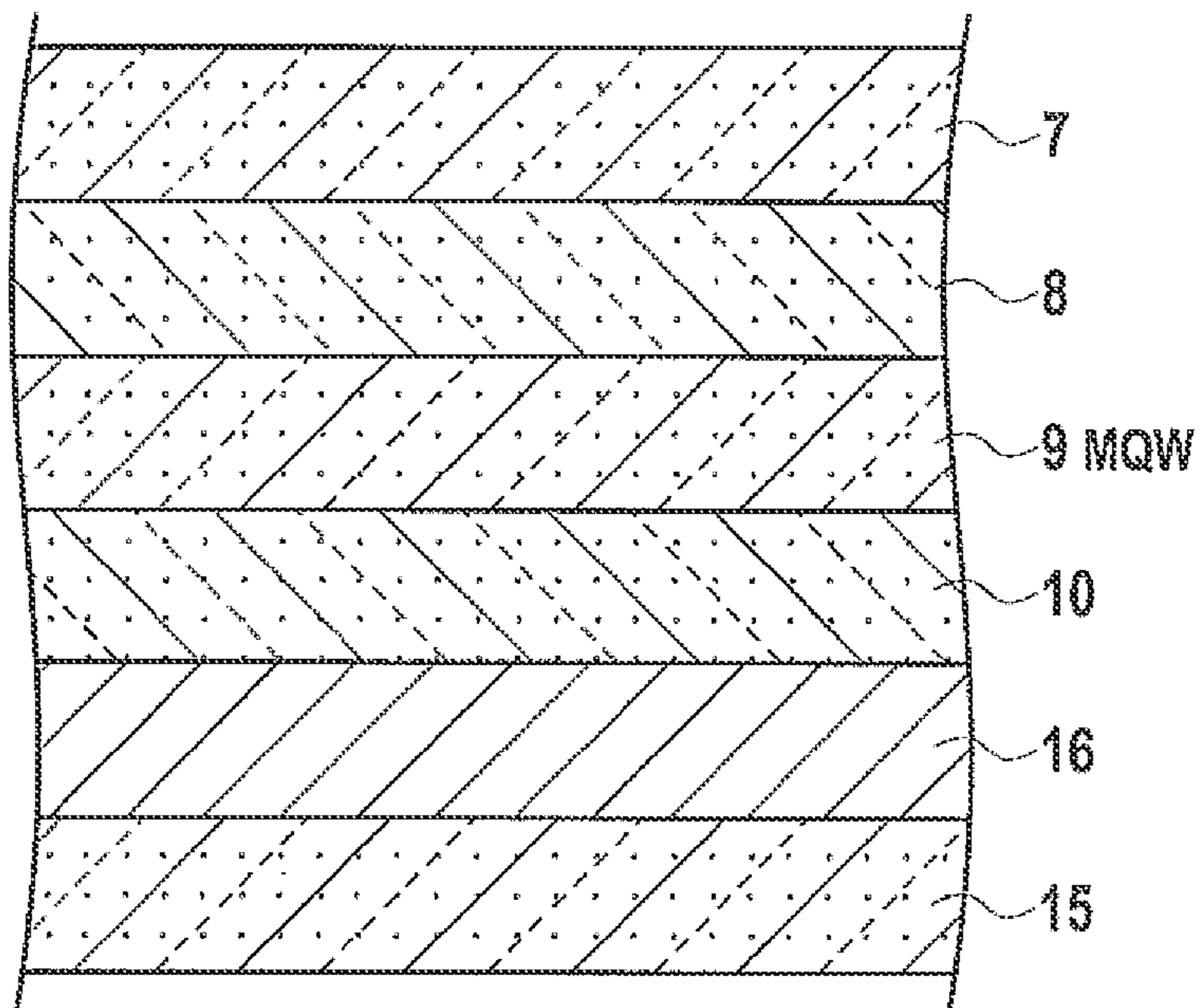
FIG. 24 PRIOR ART
