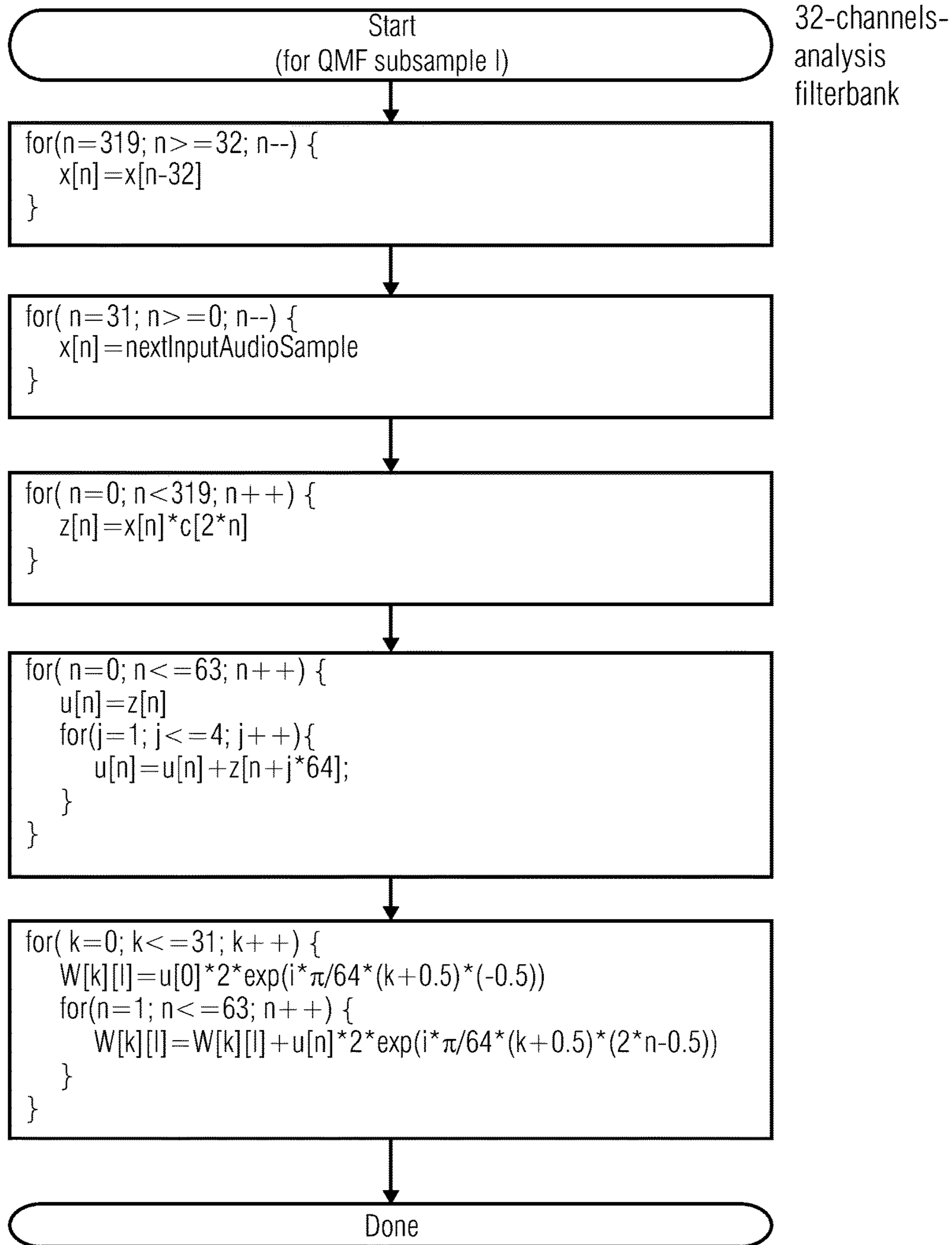
FIG 25B (CORRESPONDING TO FIG. 4.41 OF ISO/IEC 14496-3:2005(E))
