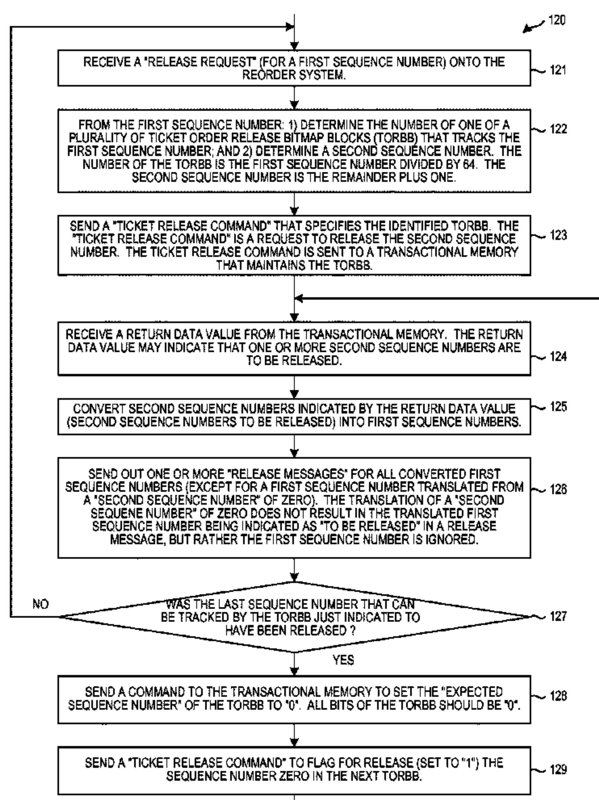
EXAMPLE OPERATION OF THE ORDERING SYSTEM
