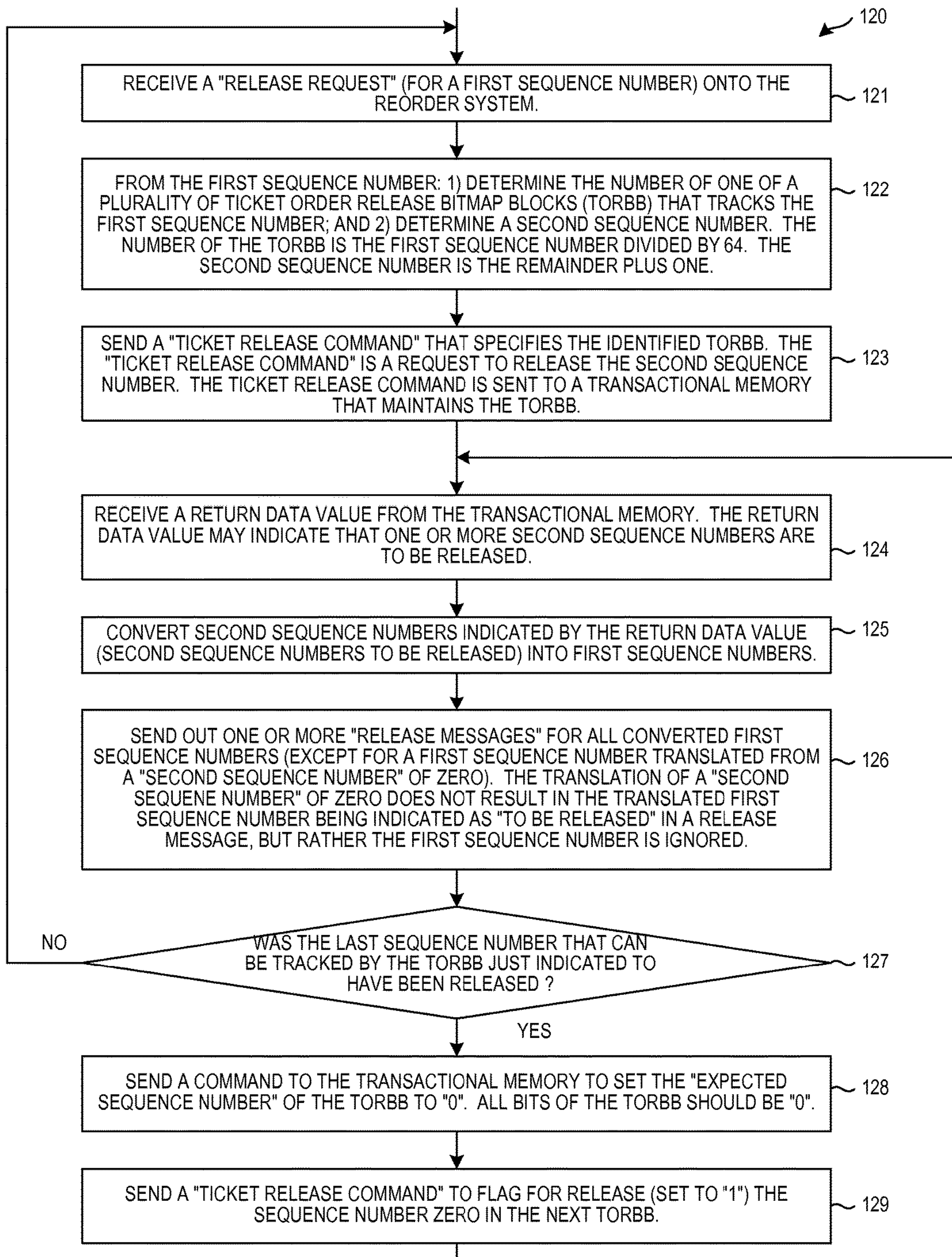
EXAMPLE OPERATION OF THE ORDERING SYSTEM
