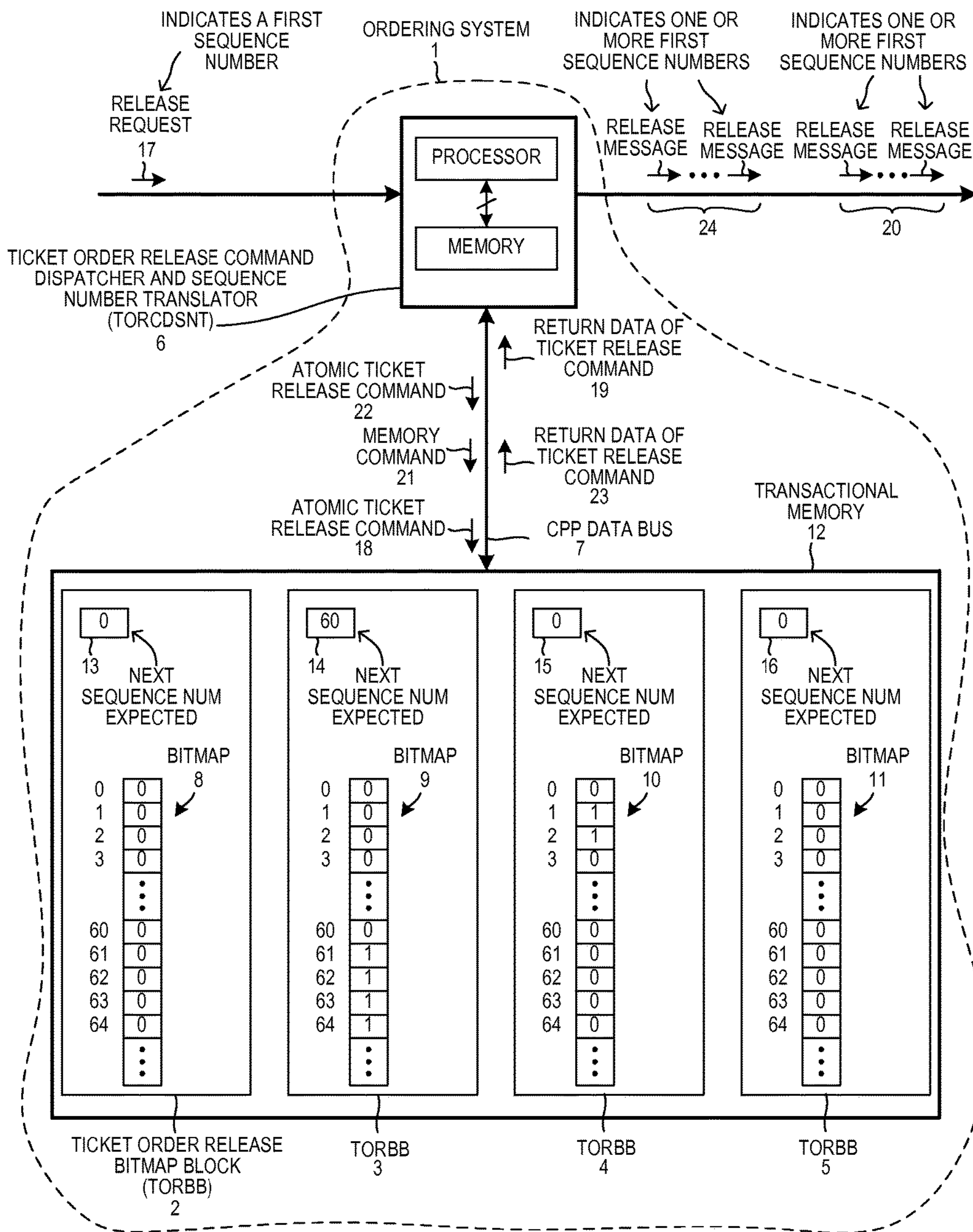
ORDERING SYSTEM EMPLOYING CHAINED TICKET RELEASE BITMAP BLOCK FUNCTIONS
