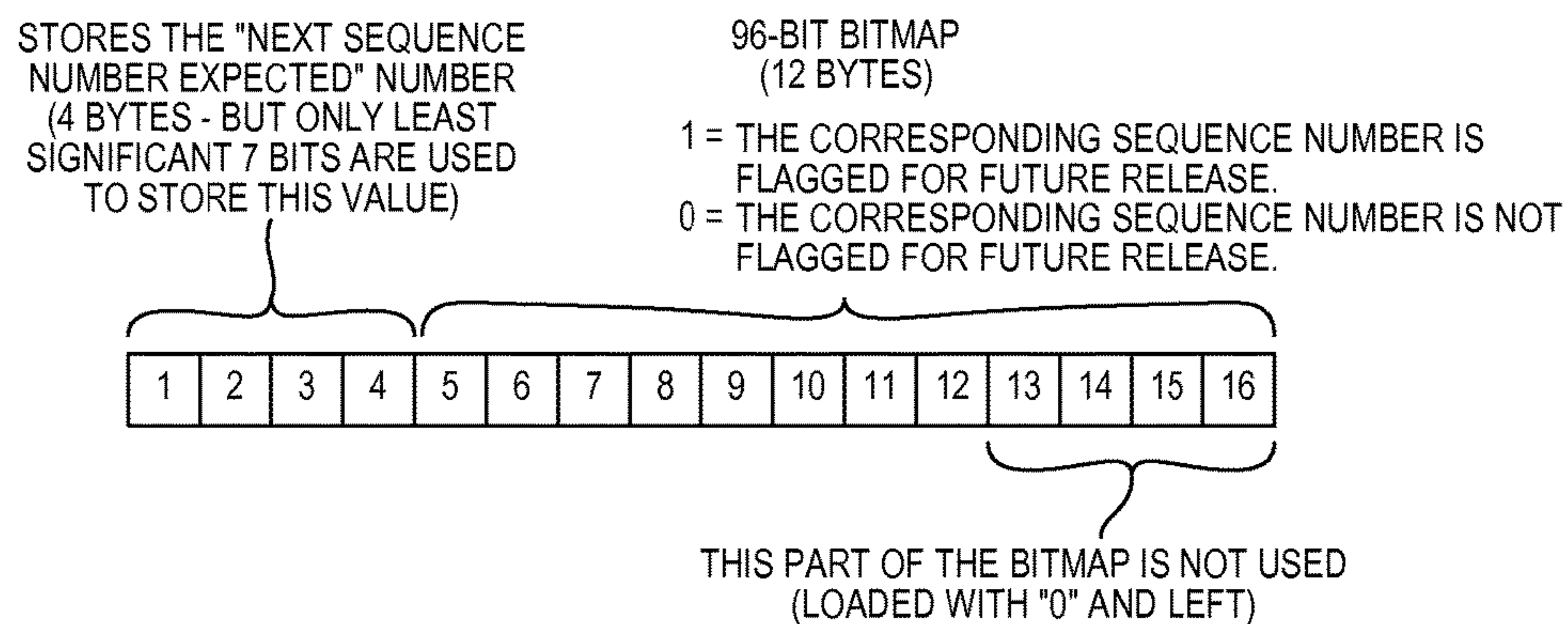
ONE 16-BYTE TICKET ORDER RELEASE BITMAP BLOCK
