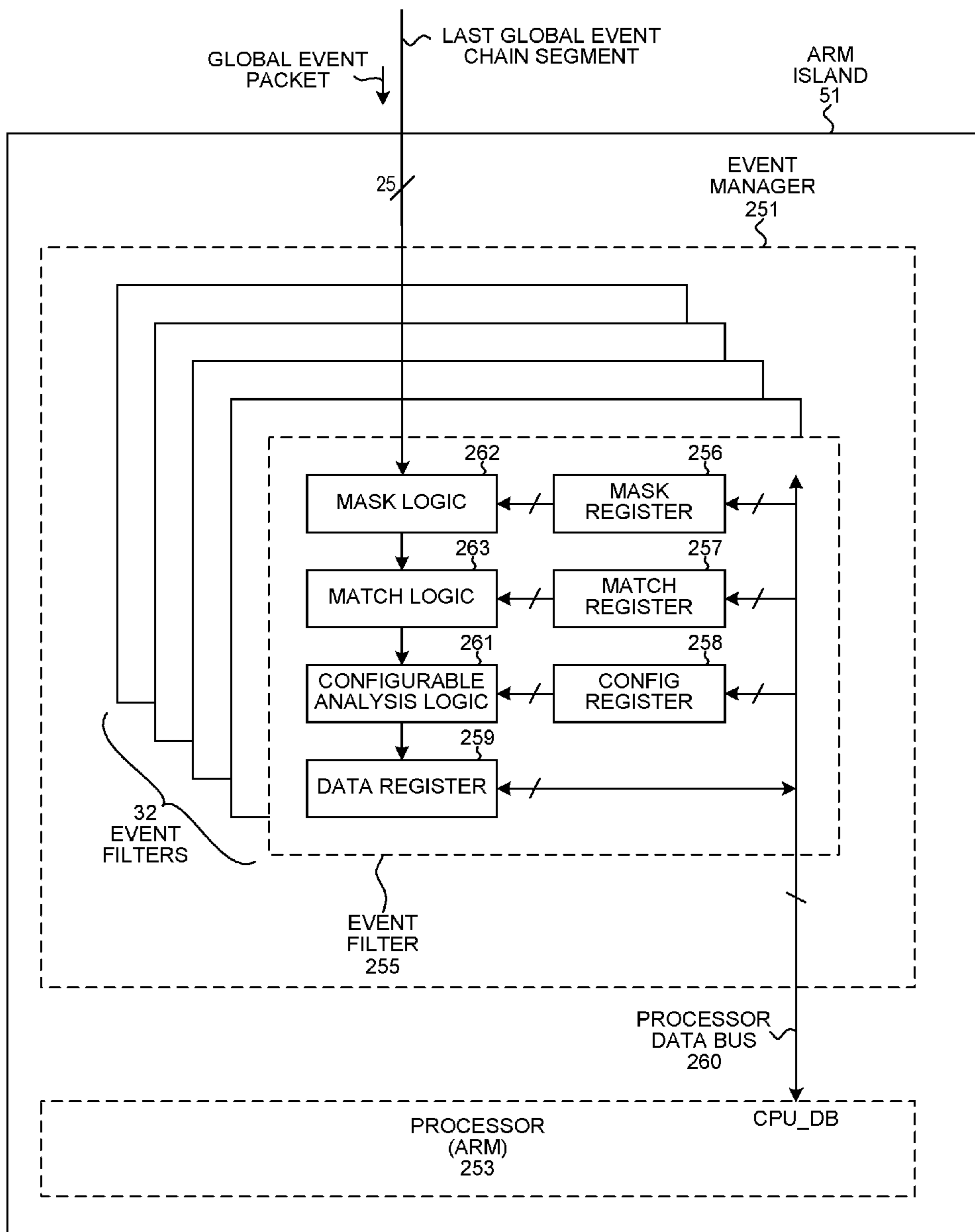
EVENT MANAGER FIG. 42
