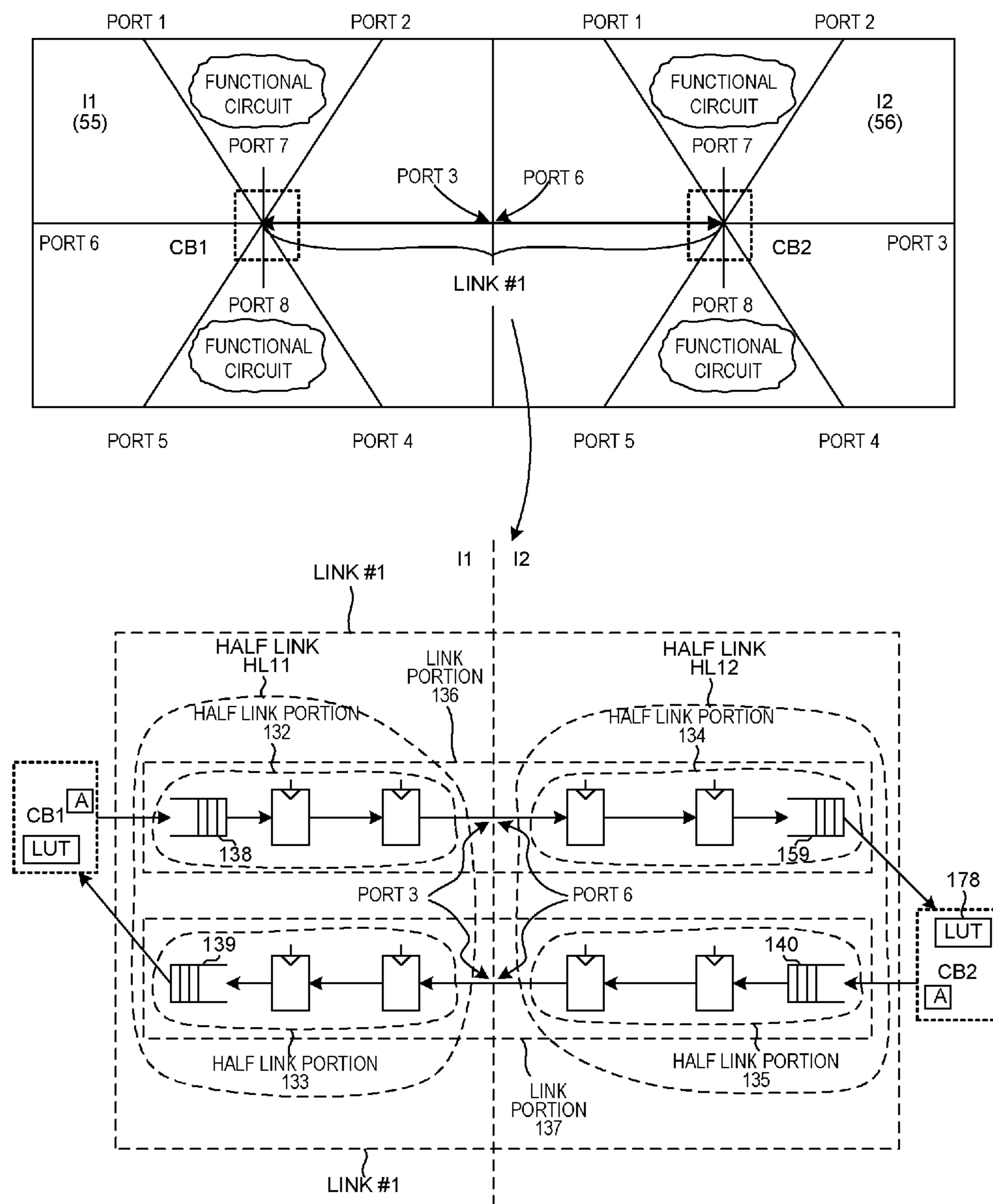
LINK BETWEEN TWO CROSSBAR SWITCHES
