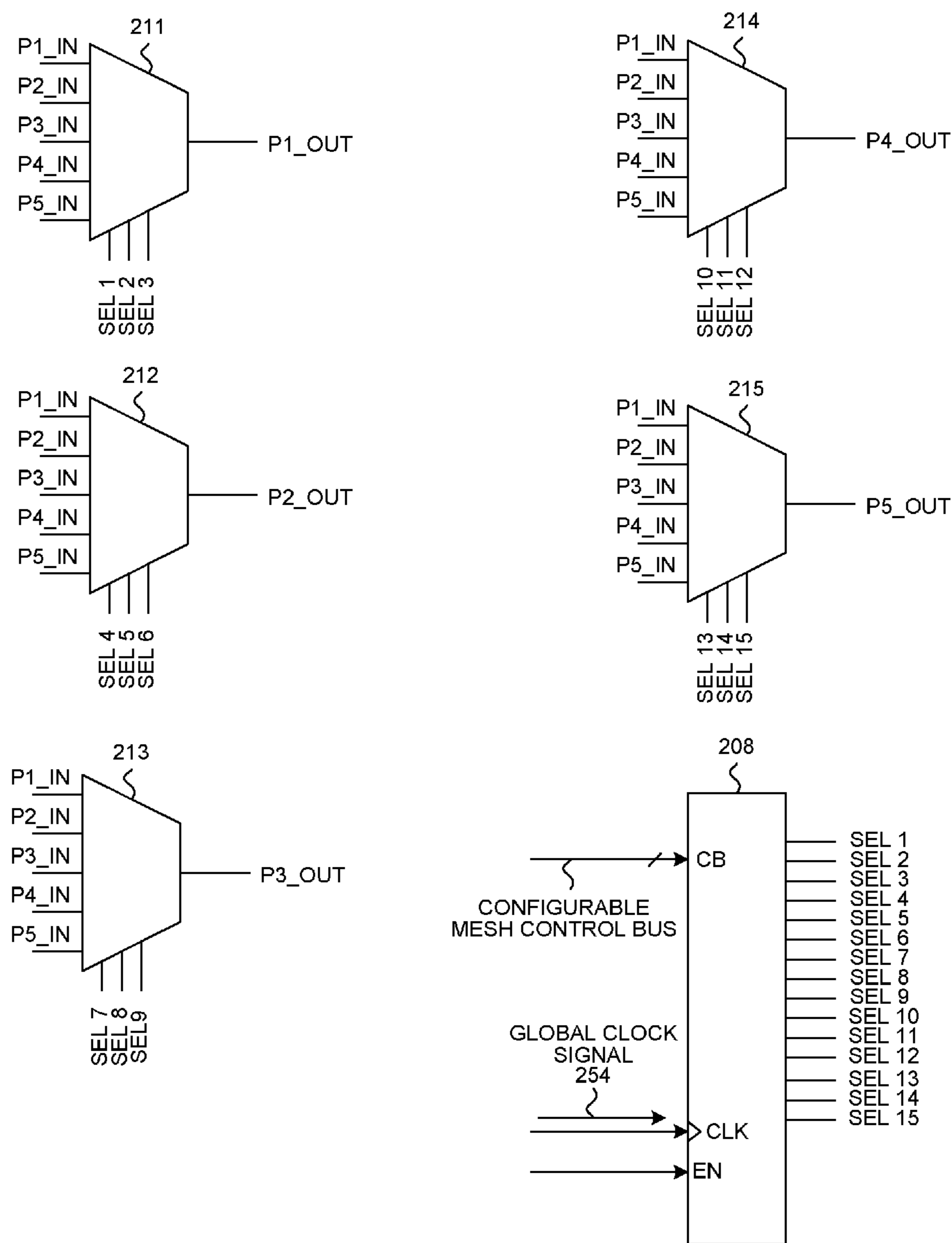
RUN TIME CONFIGURABLE SWITCH CIRCUIT FIG. 35
