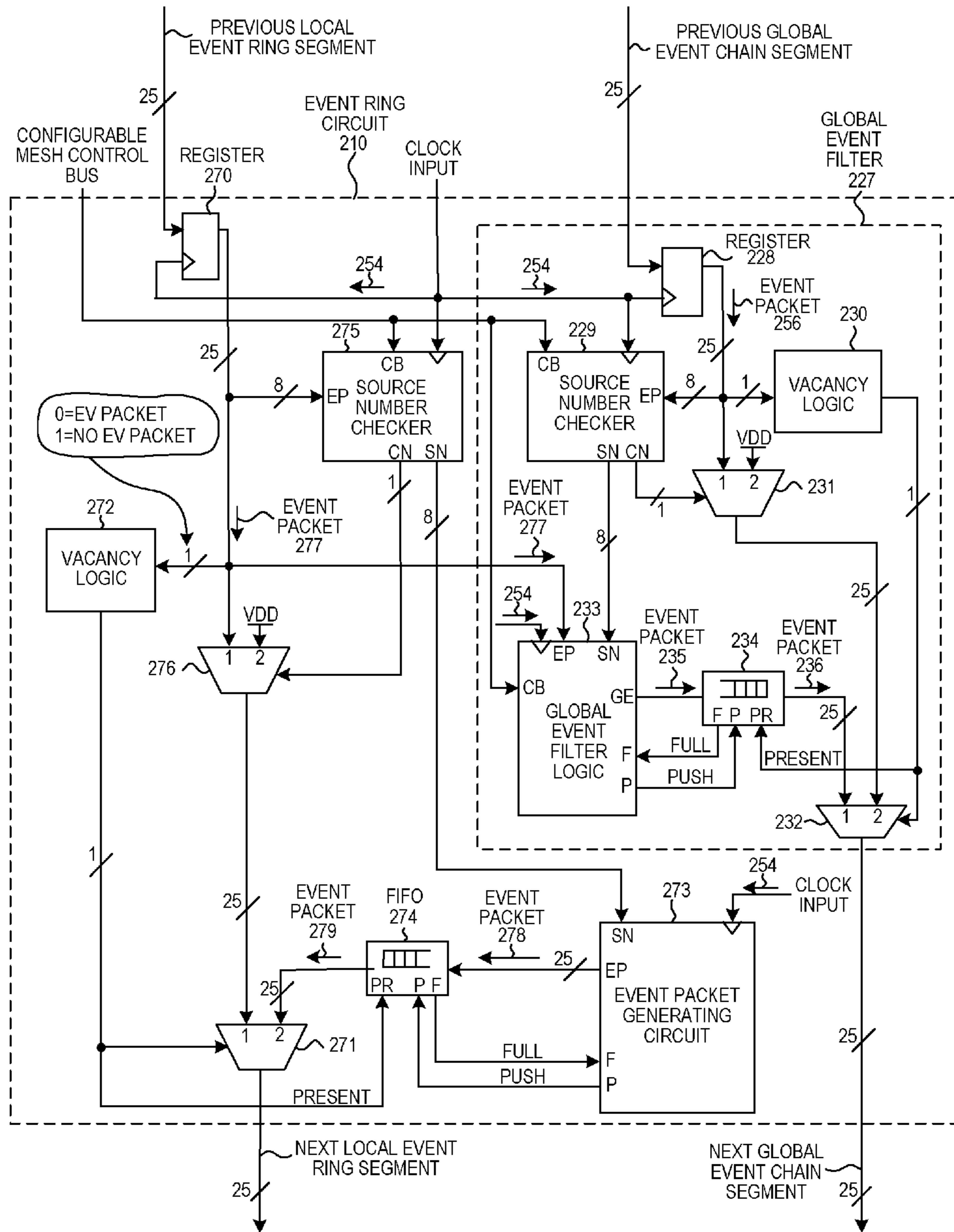
EVENT RING CIRCUIT WITH GLOBAL EVENT FILTER FIG. 37
