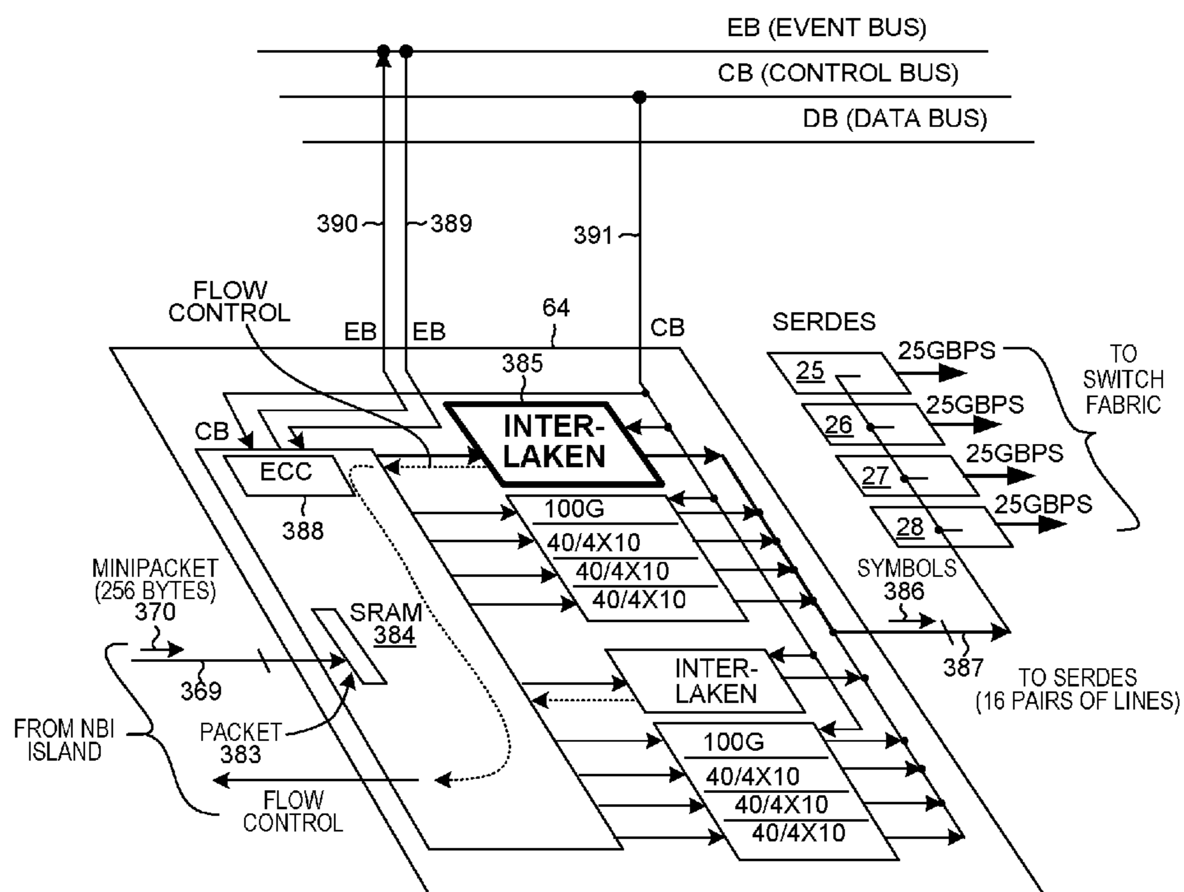
MAC ISLAND (EGRESS)
