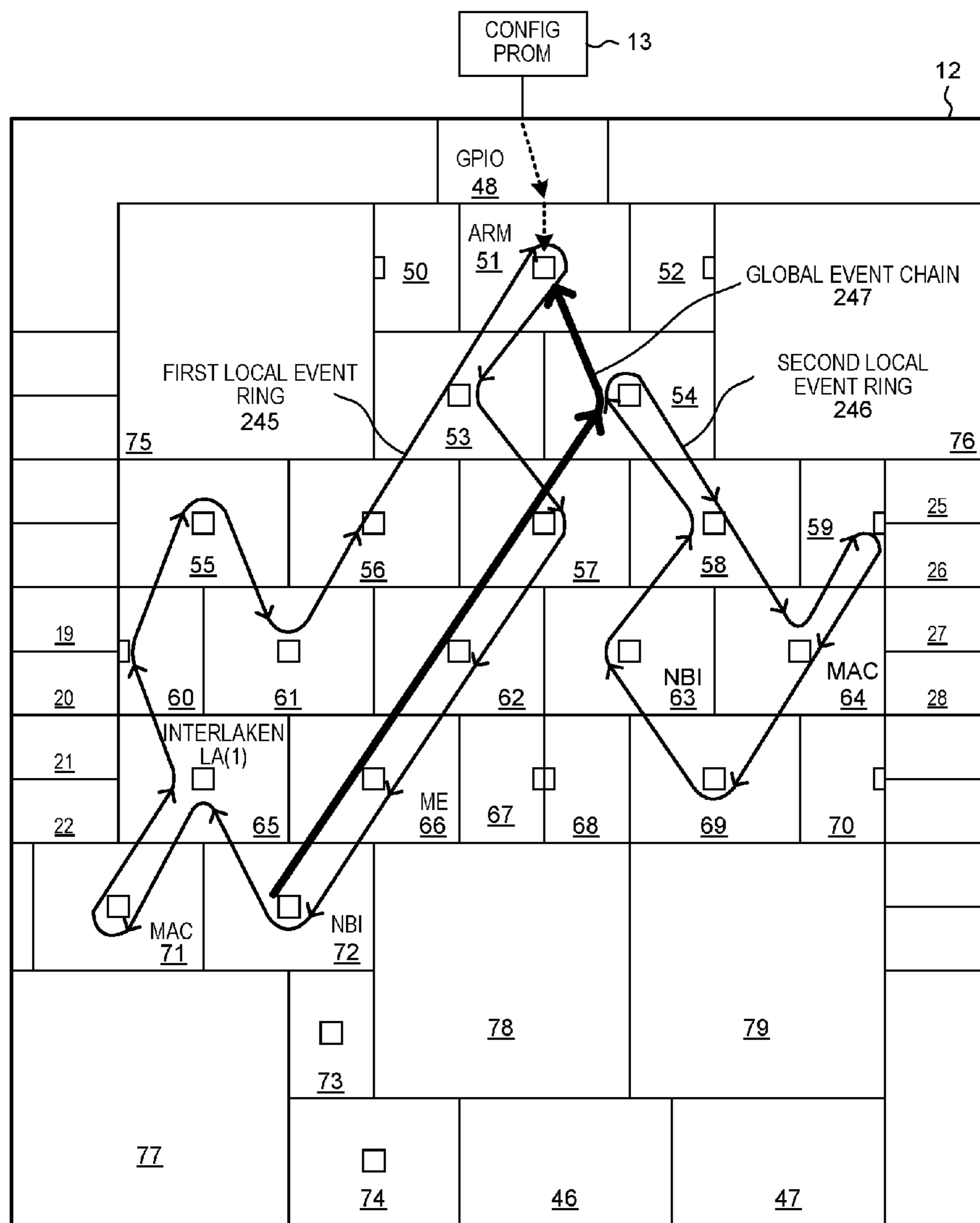
CONFIGURED CONFIGURABLE MESH EVENT BUS
