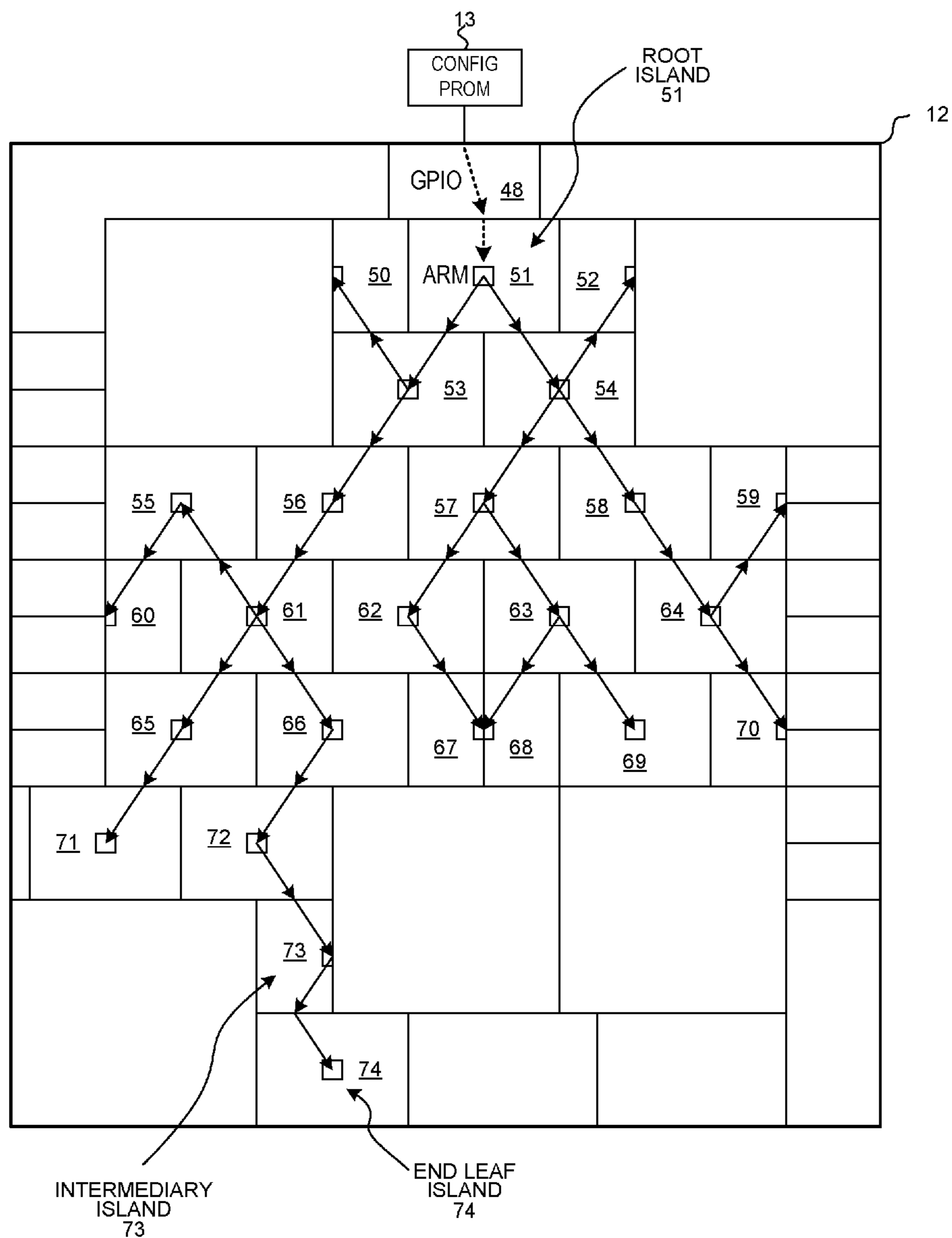
CONFIGURED CONFIGURABLE MESH CONTROL BUS
