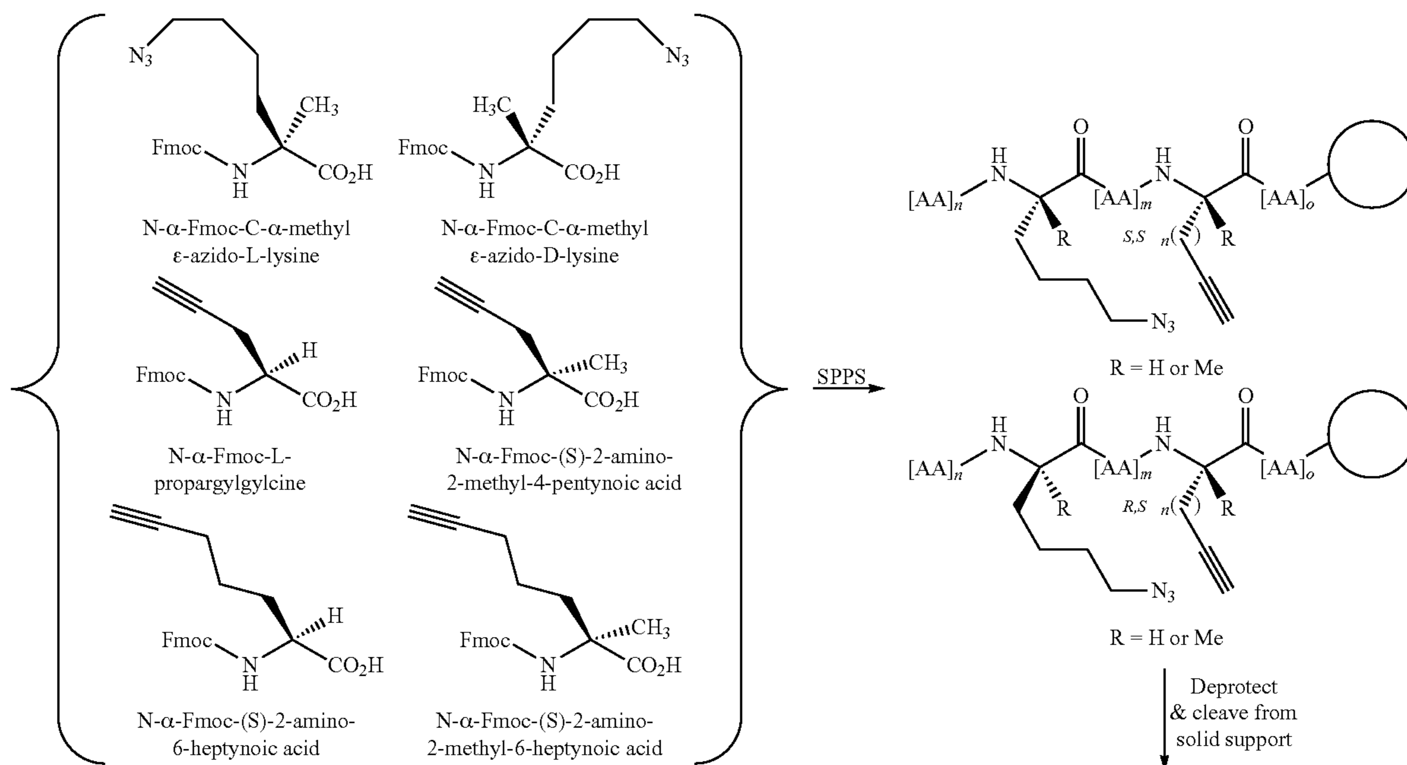
Synthetic Scheme 2:
