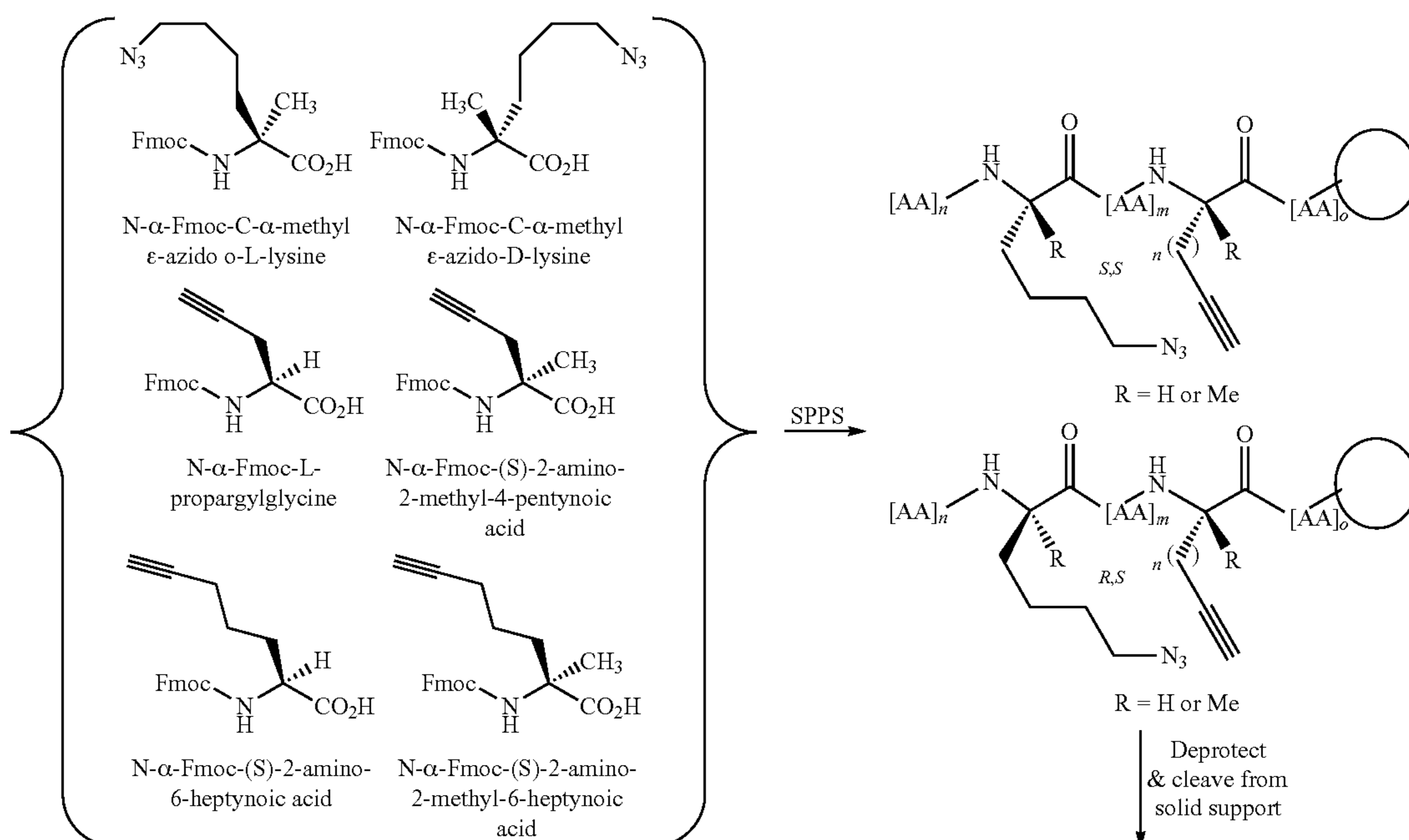
Synthetic Scheme 4:
