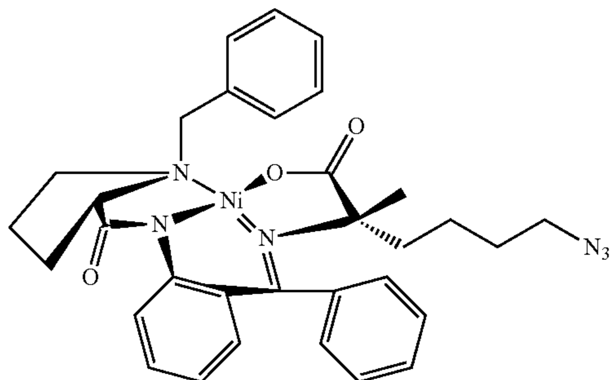
Compound 3
