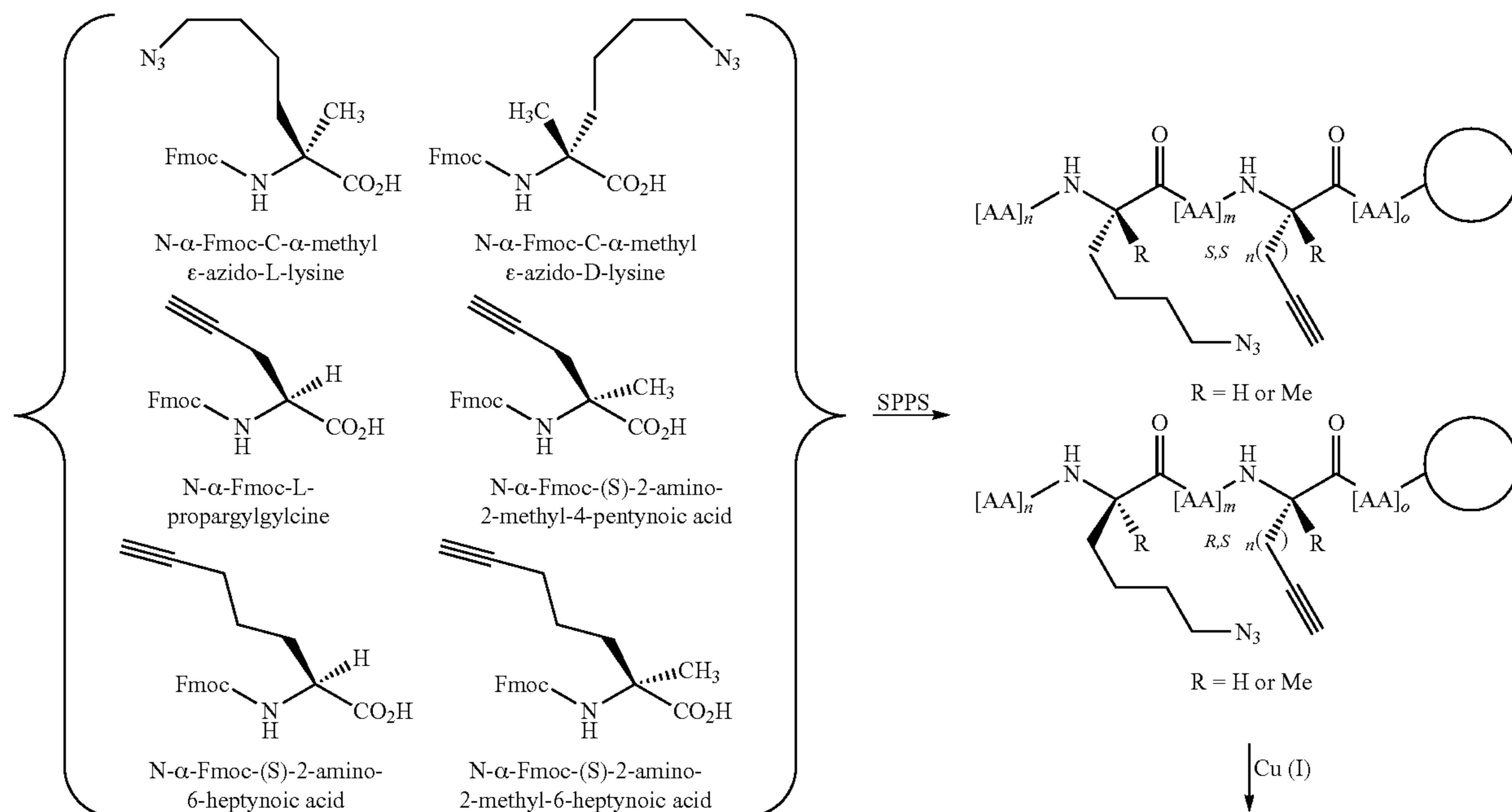
Synthetic Scheme 3:
