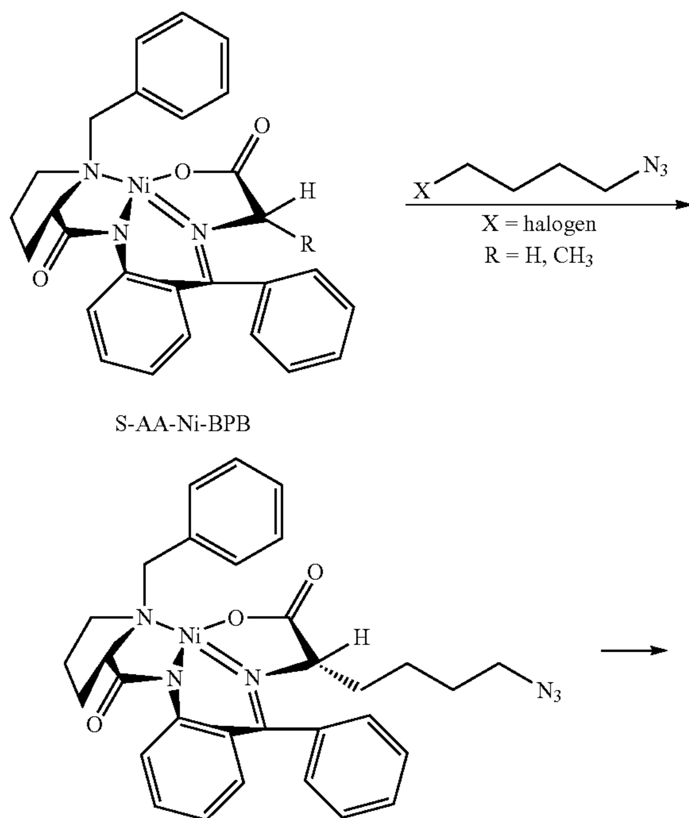
Synthetic Scheme 1:
