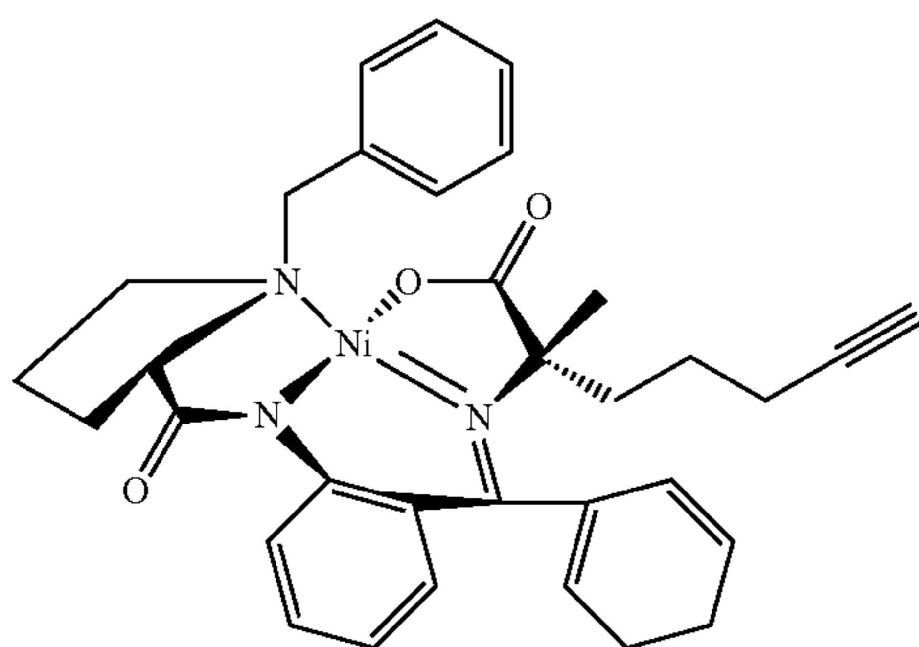
Compound 5
