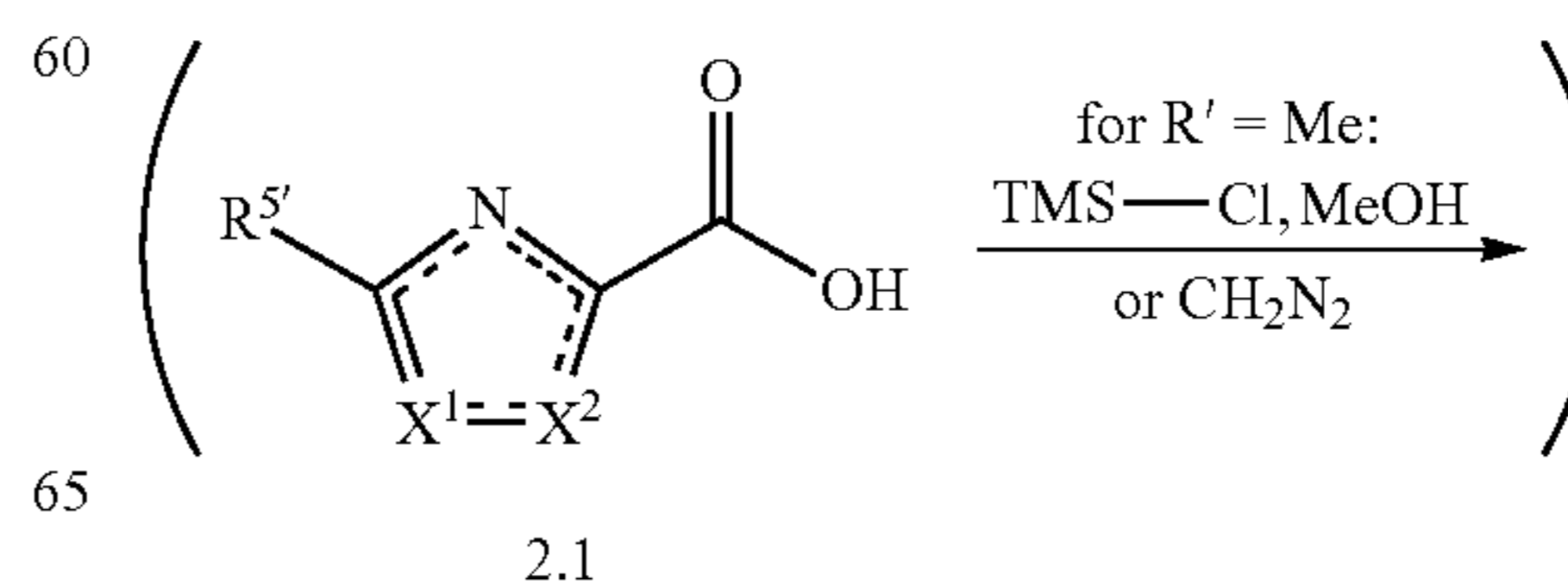
Scheme 4: Formation of acylhydrazide 2.
