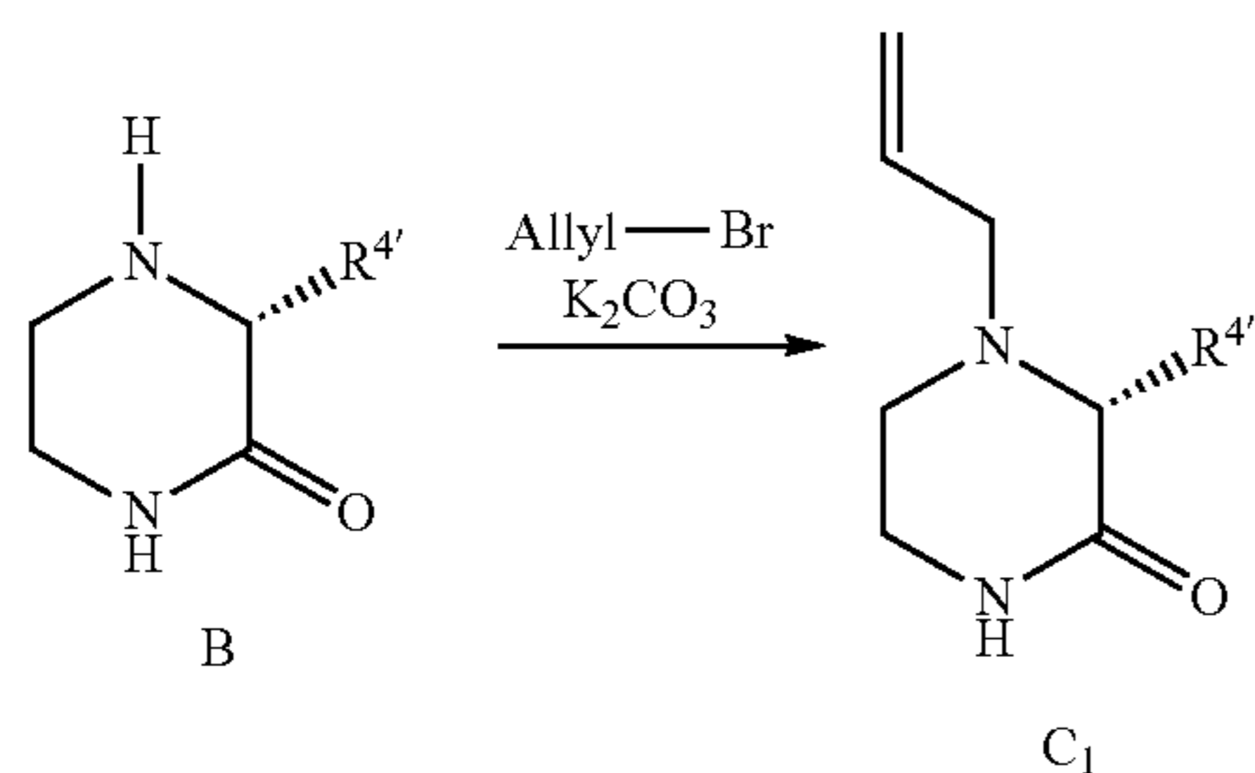
Scheme 8: Allyl protection of B.
