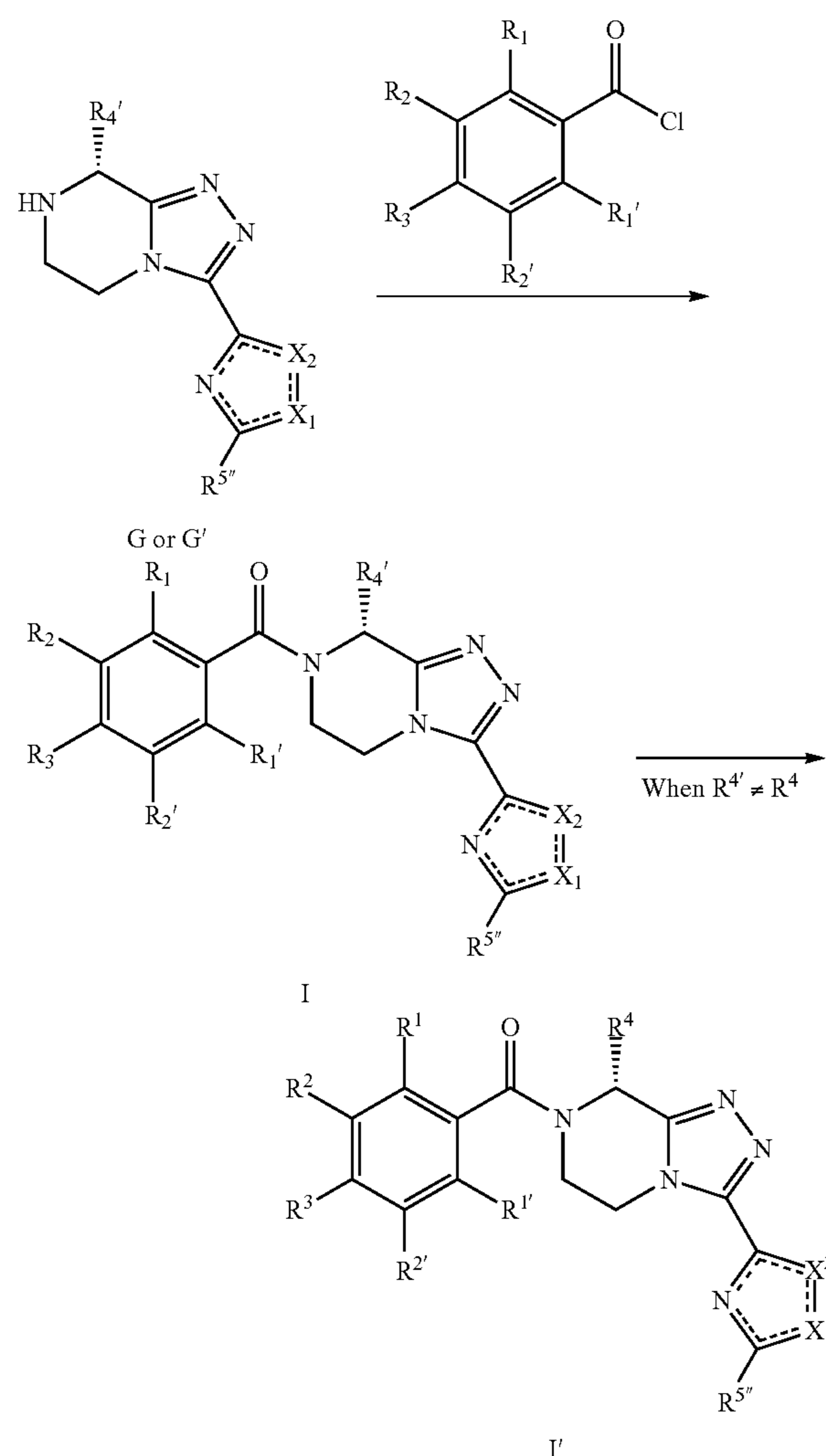
Scheme 16: Acylation.
