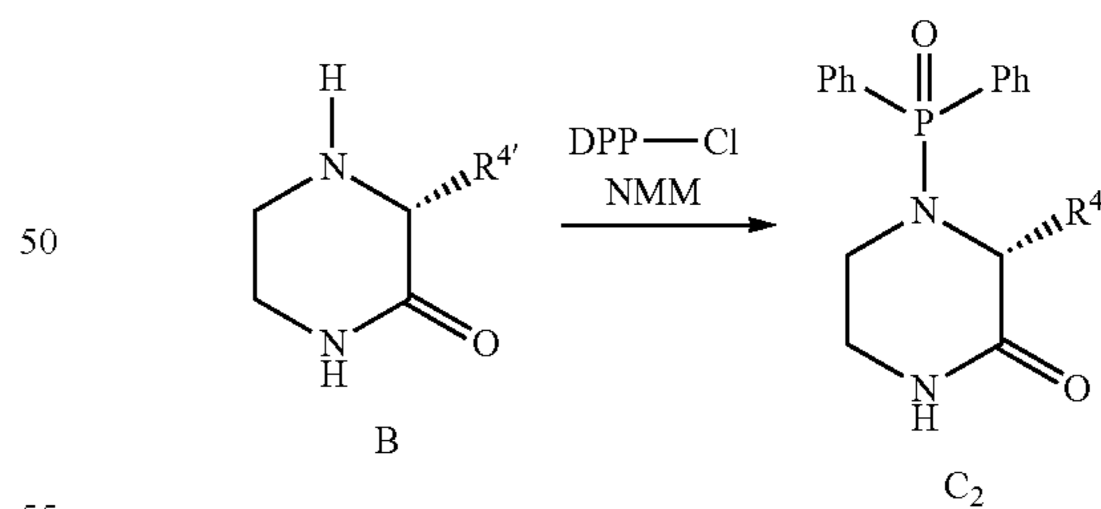
Scheme 9: DPP protection of B.
