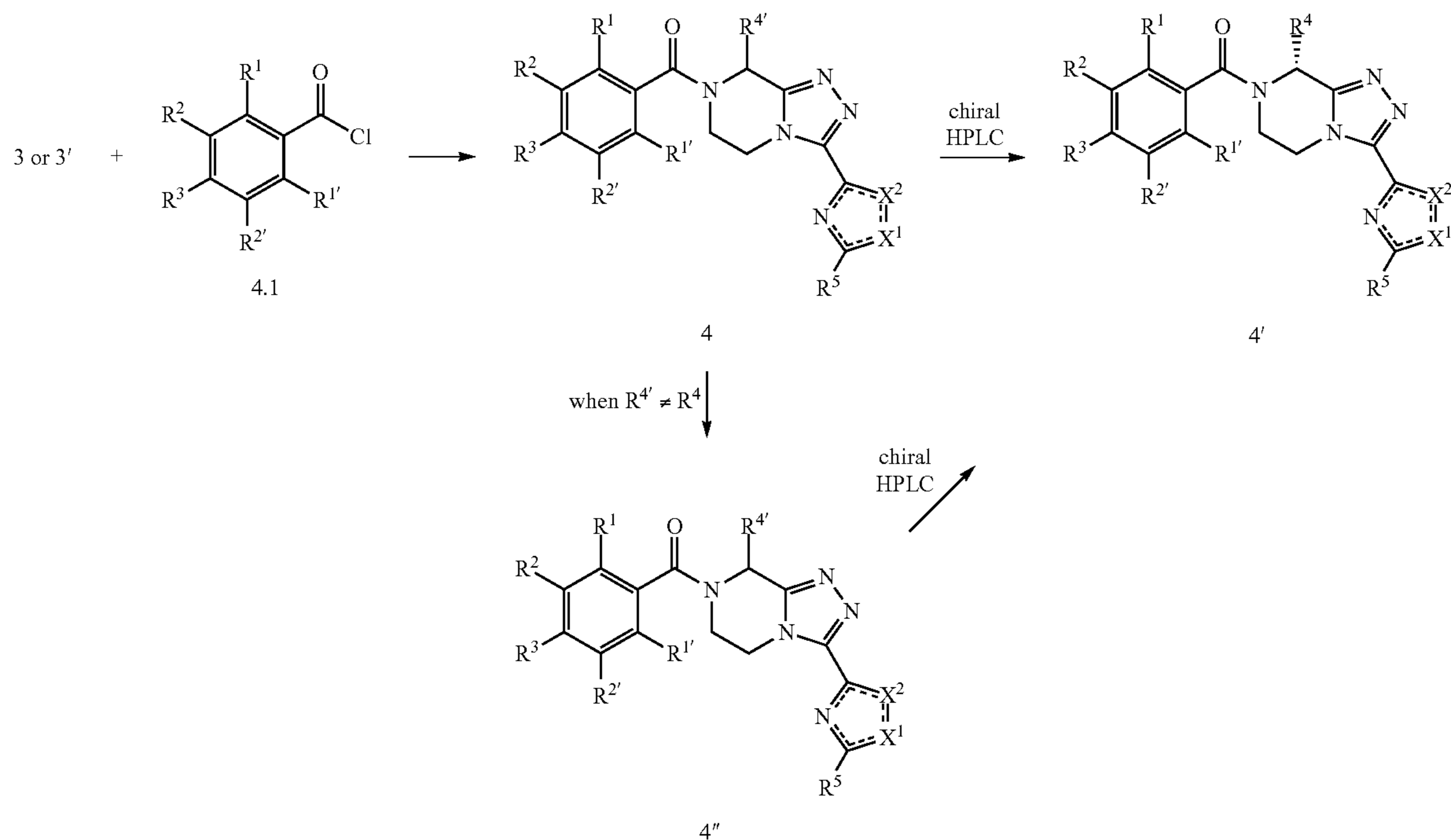
Scheme 6: Acylation and chiral HPLC purification.
