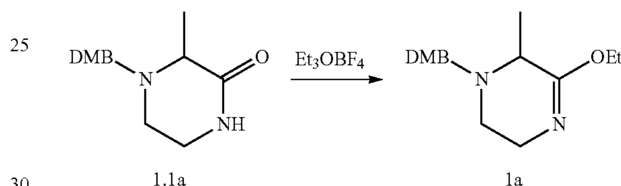
Scheme 3: Synthesis of 1-(2,4-dimethoxybenzyl)-5-ethoxy-6-methyl-1,2,3,6-tetrahydropyrazine 1a.
