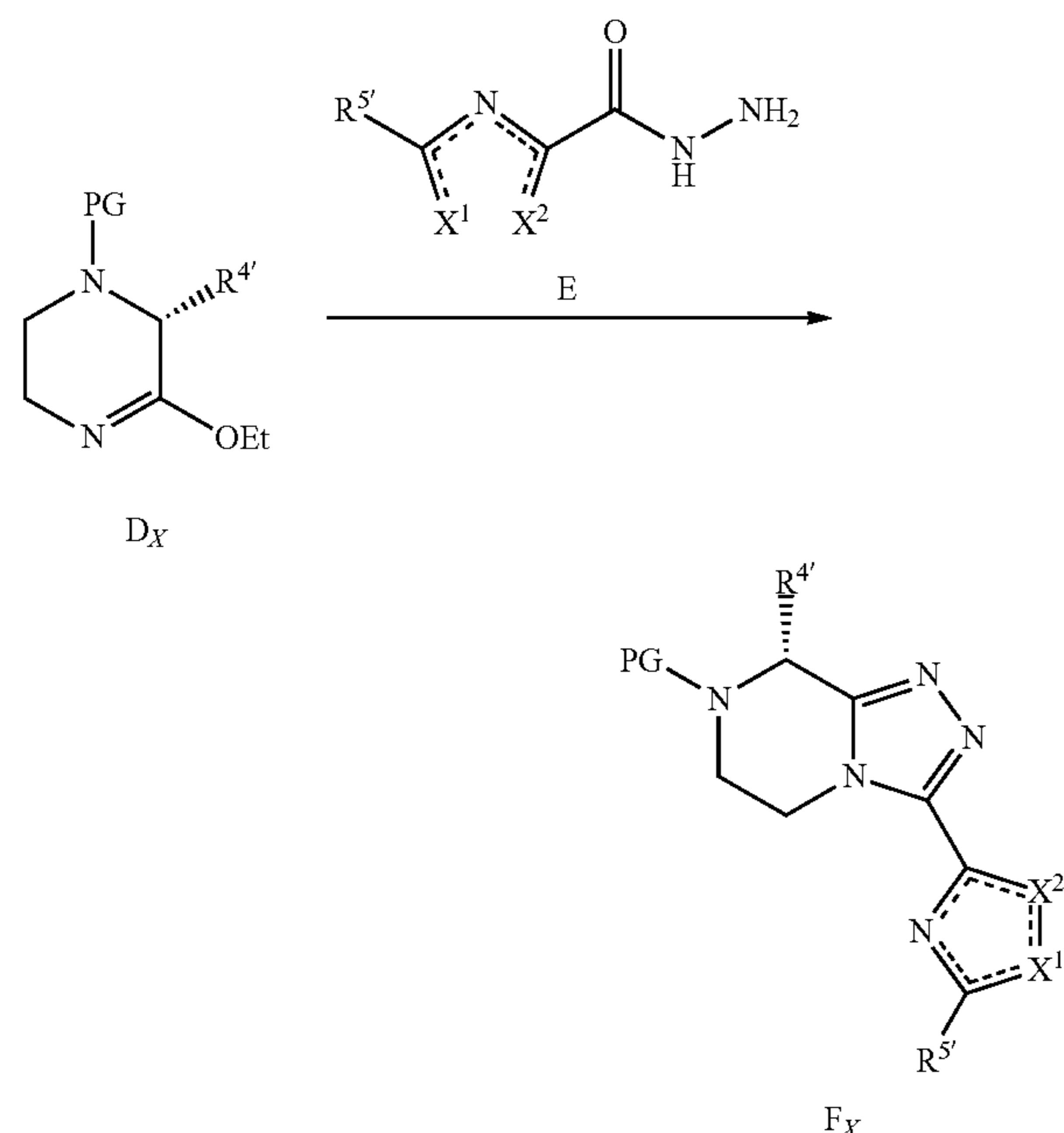
Scheme 13: Formation of acylhydrazide F.
