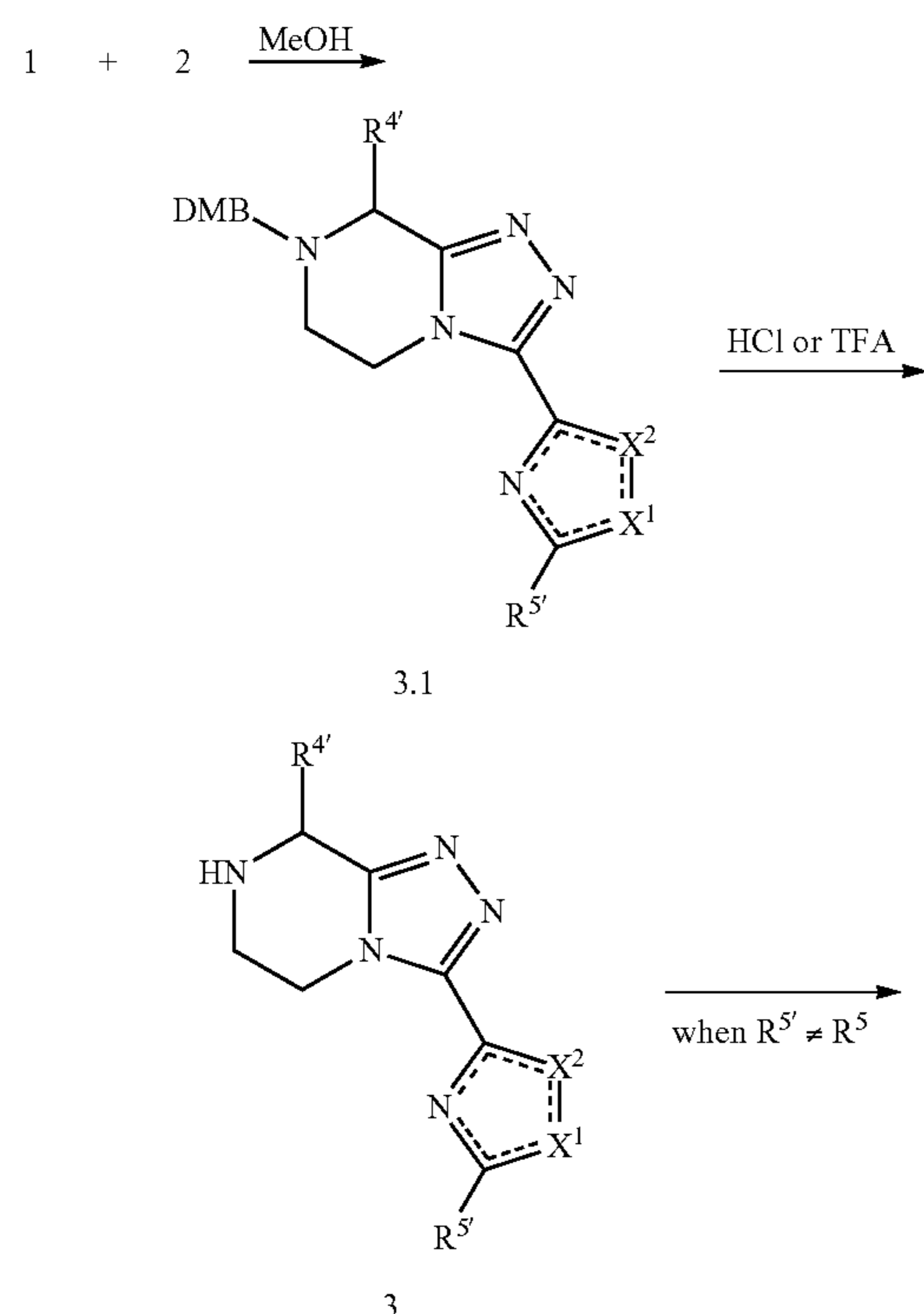
Scheme 5: Cyclodehydration leading to triazolopiperazine 3.
