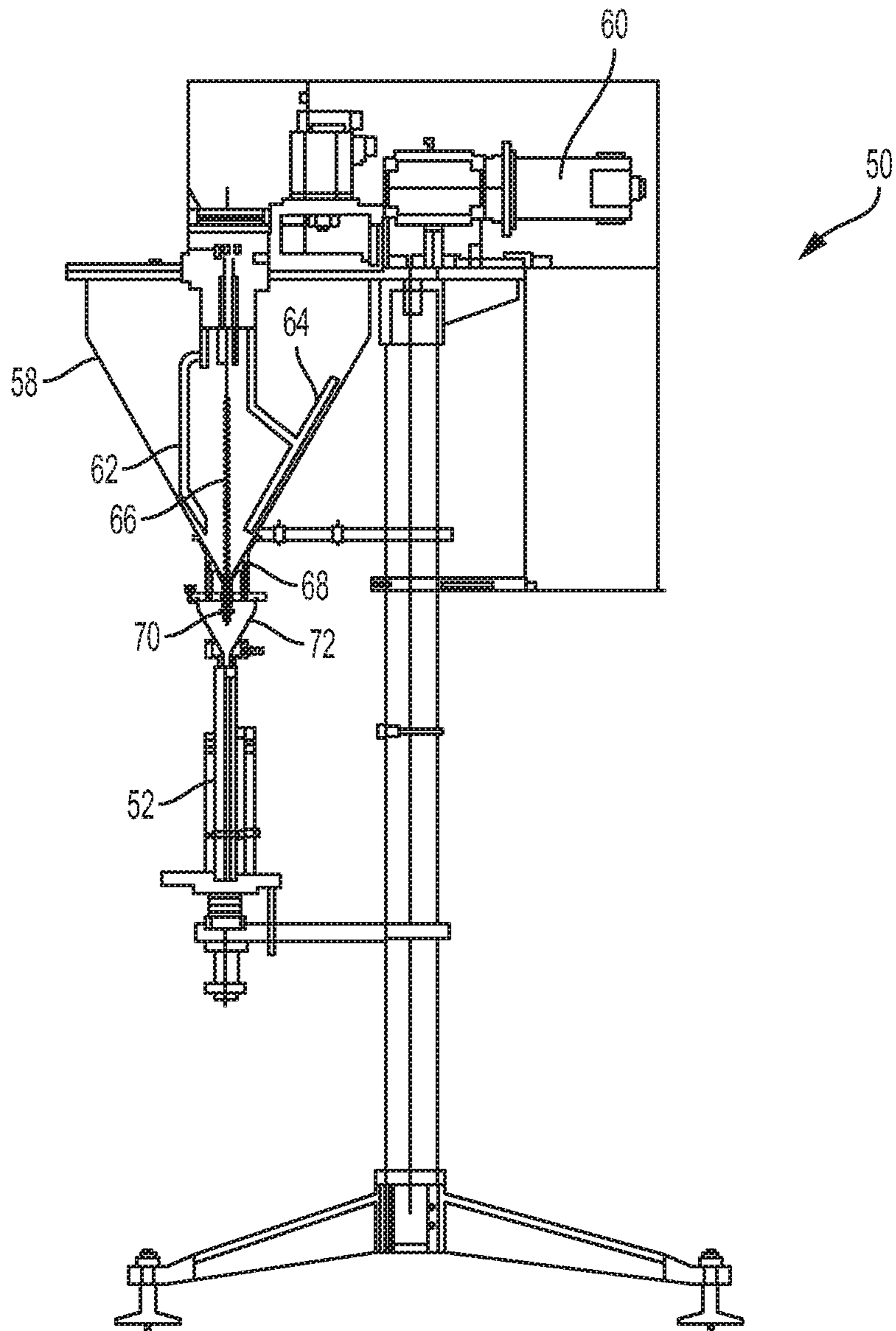
FIG. 3 PRIOR ART
