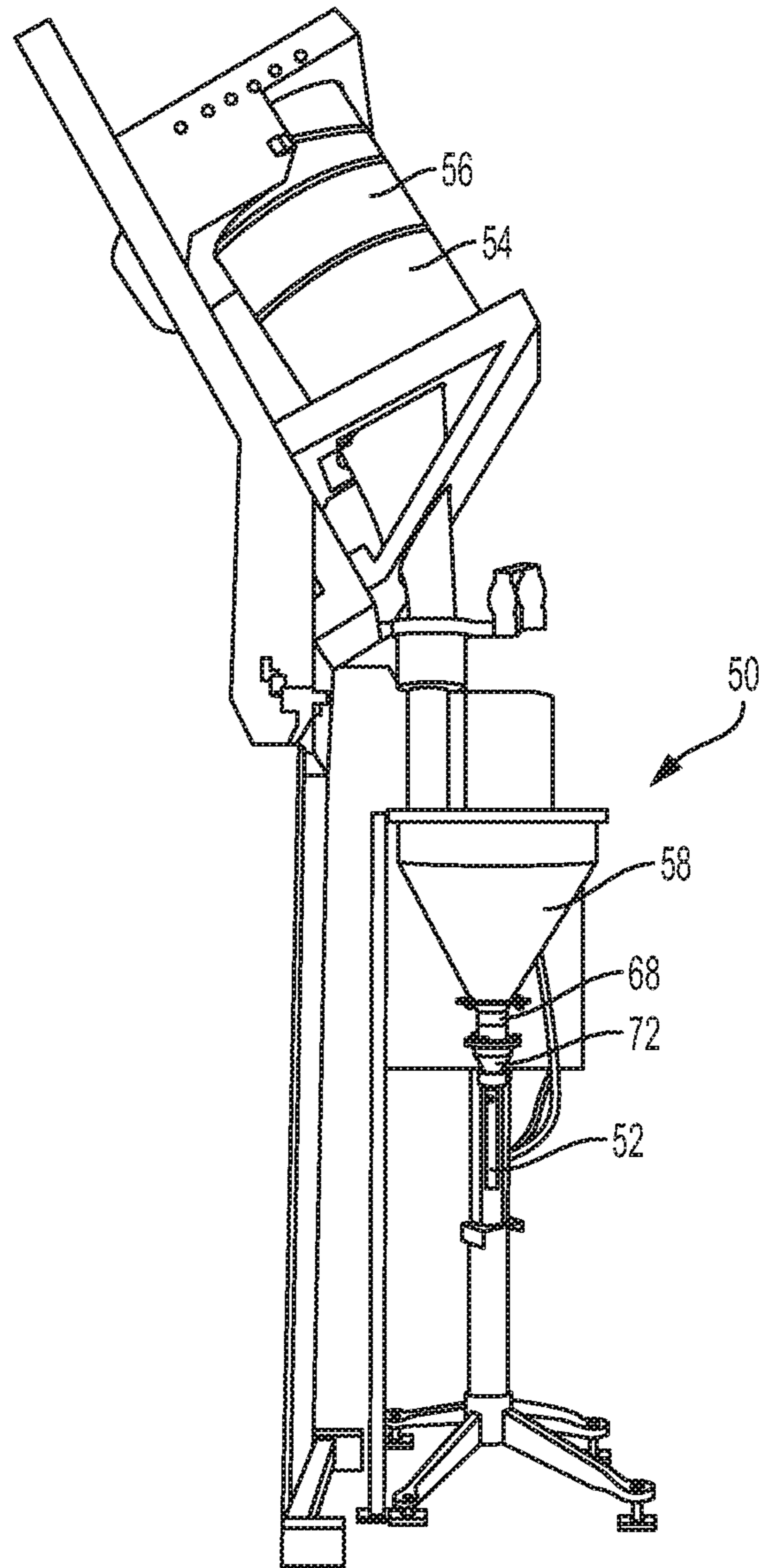
FIG. 1 PRIOR ART
