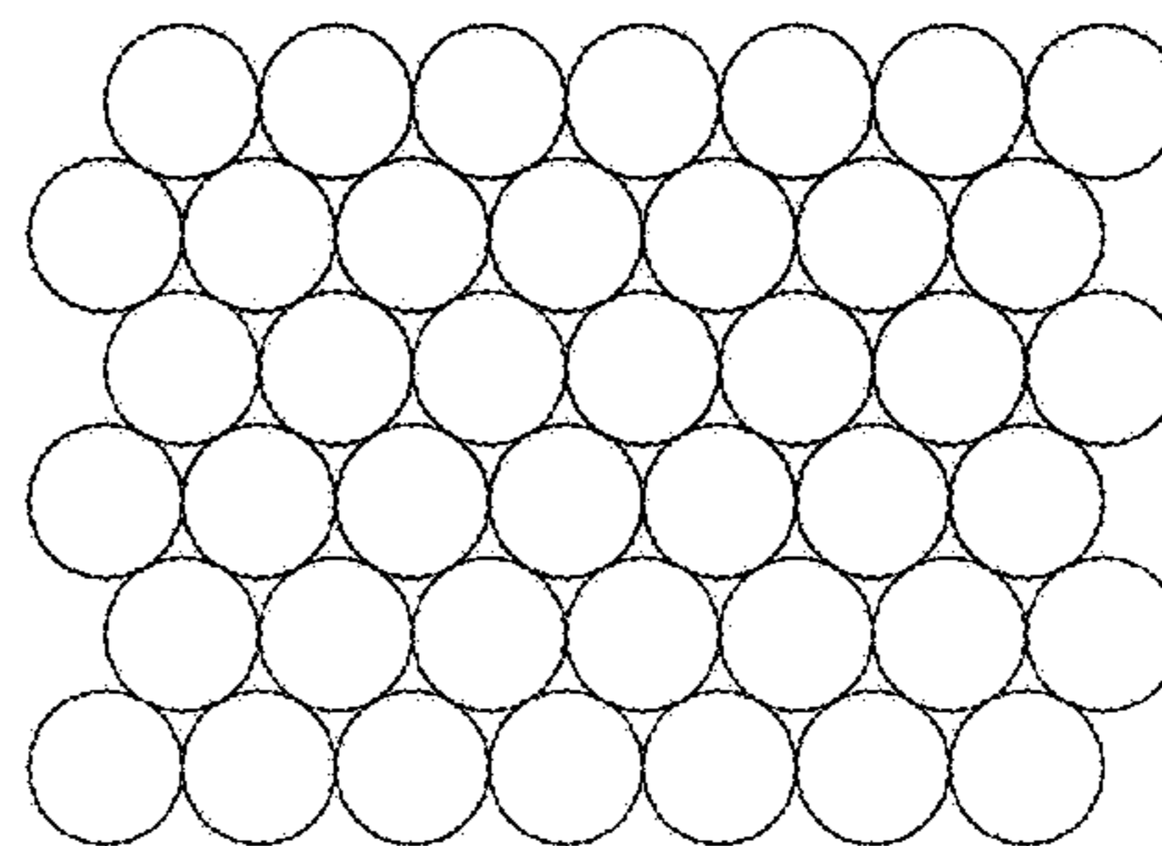
hexagonal packing
