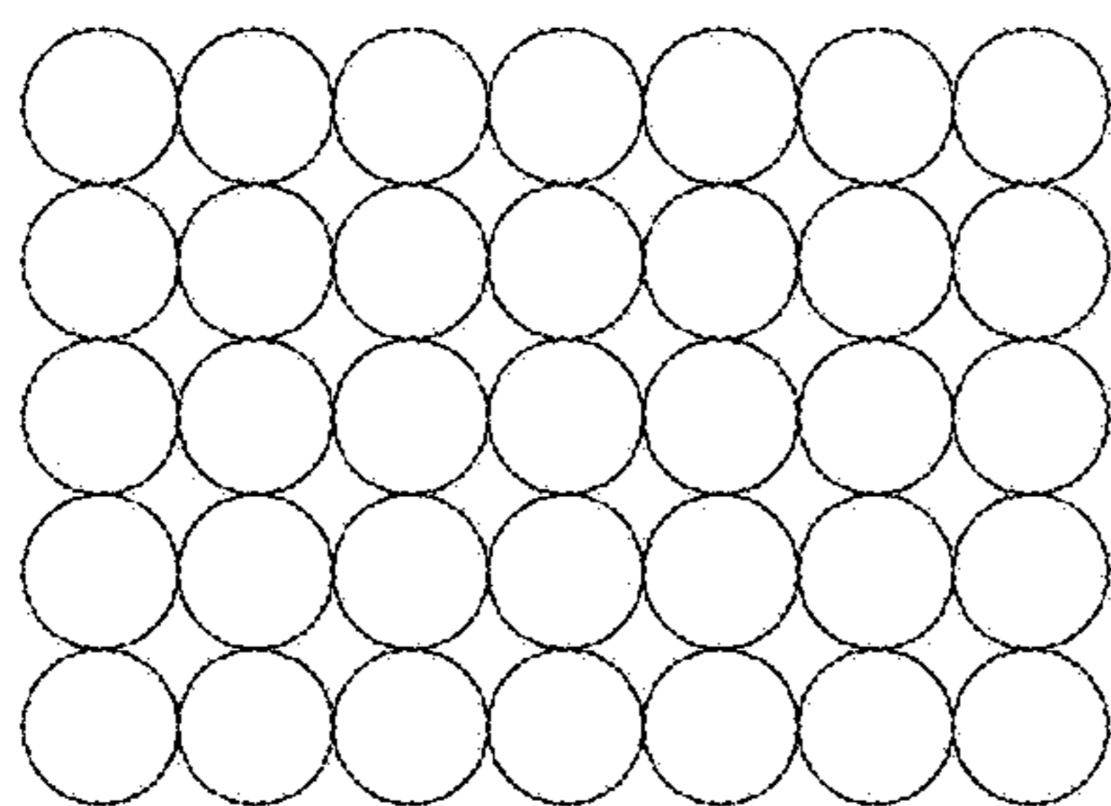
square packing
