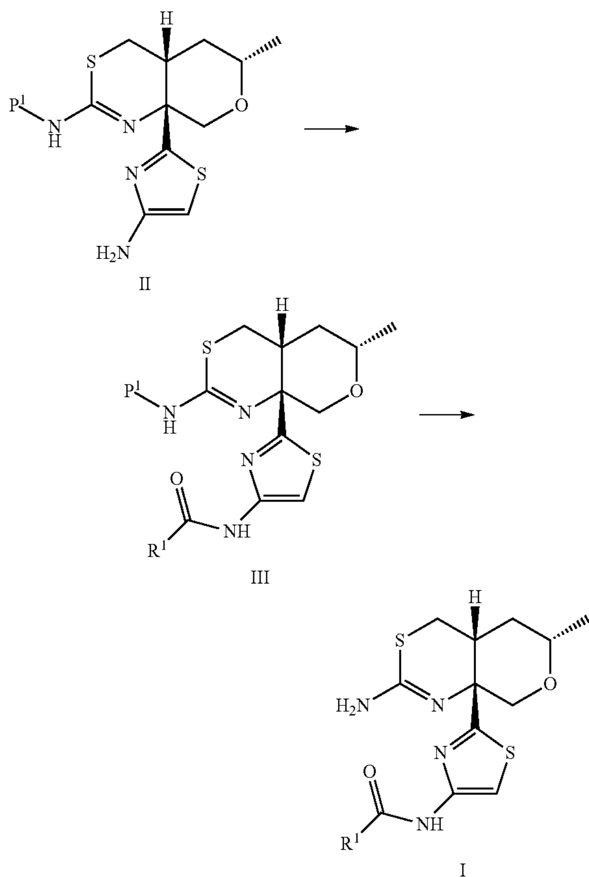
Scheme 1
