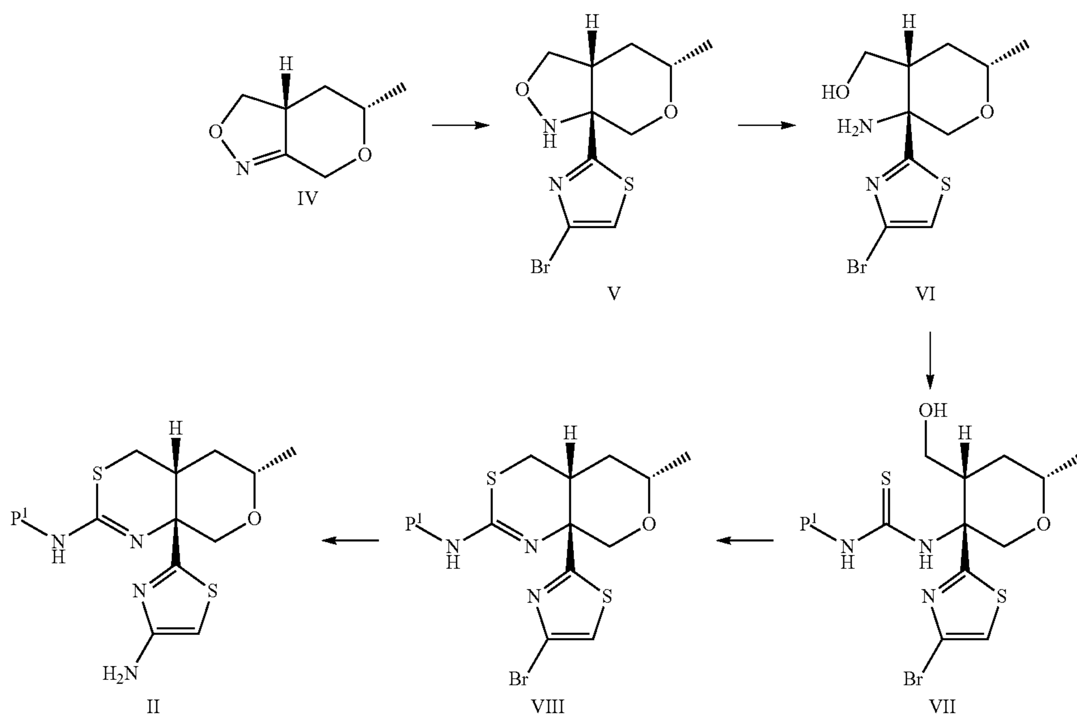
Scheme 2
