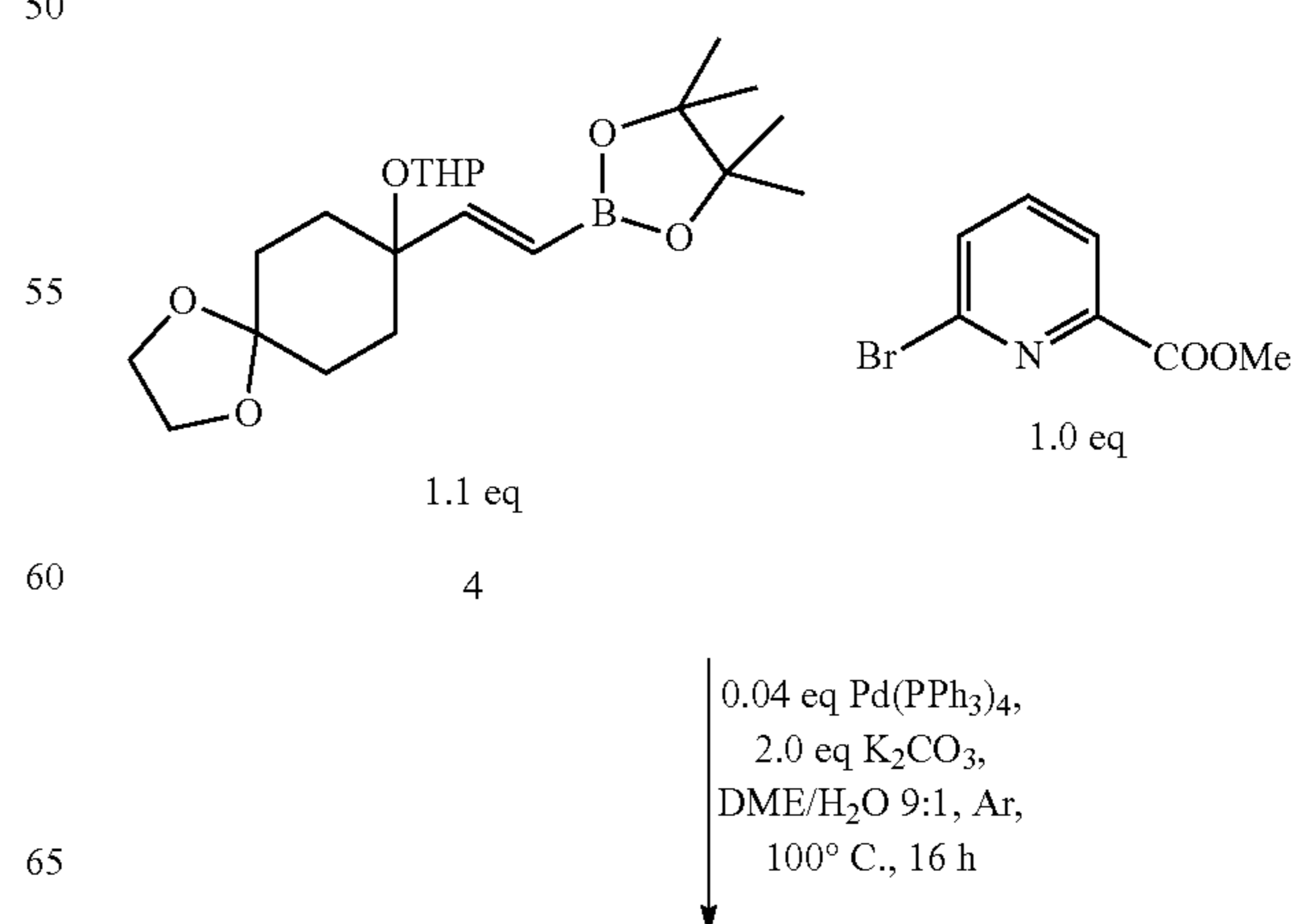
Scheme 16-4
