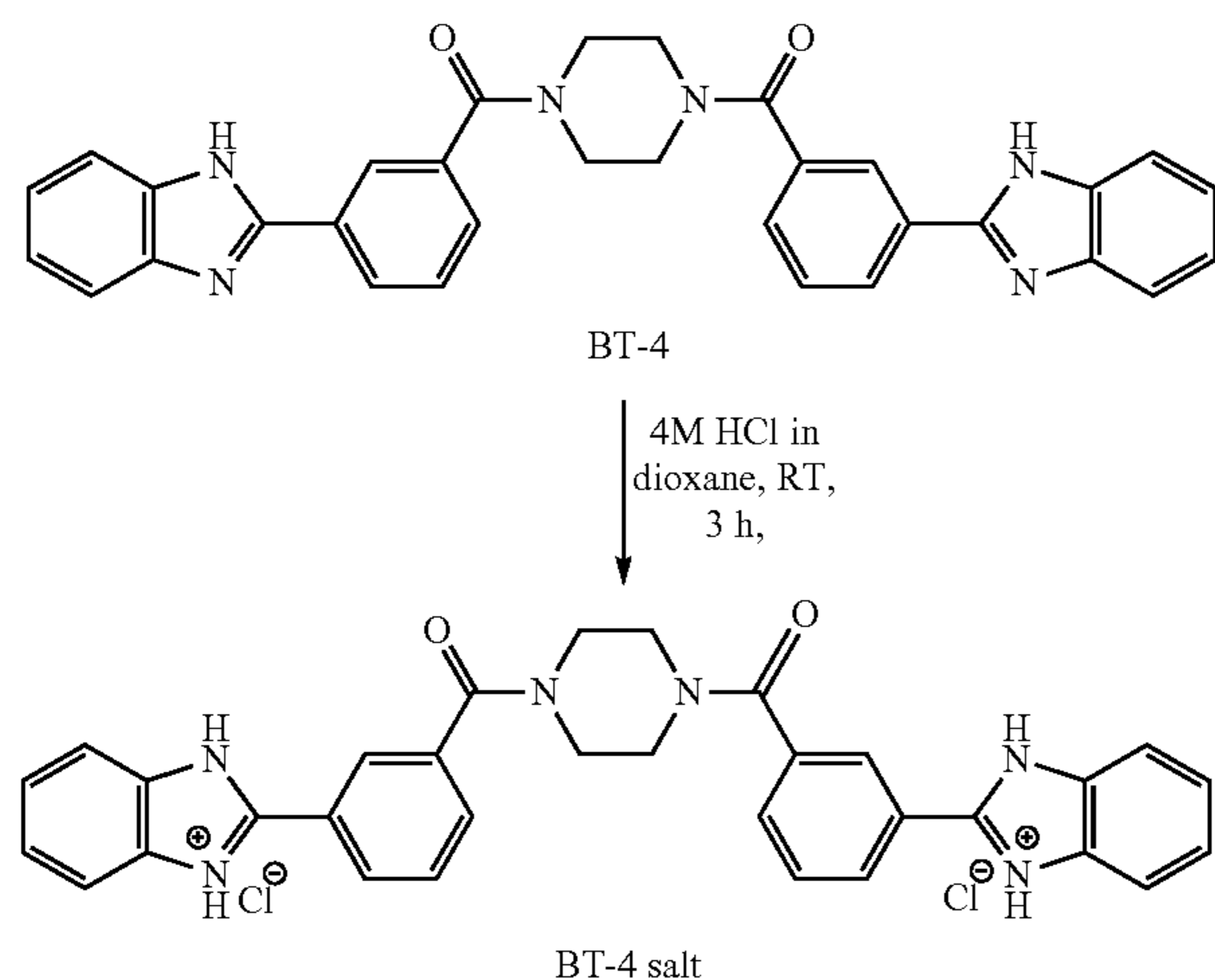
Scheme 7-2
