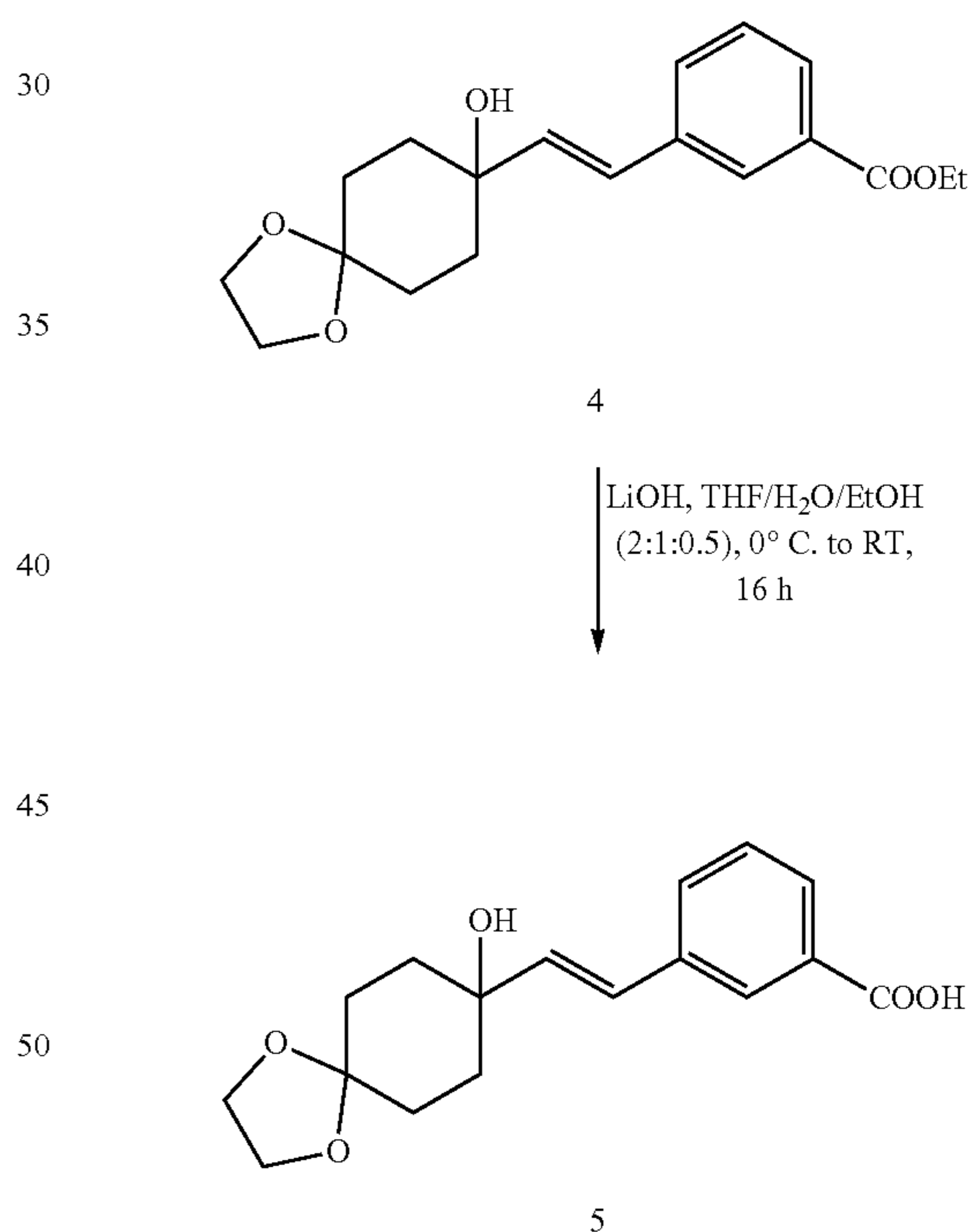
Scheme 15-2
