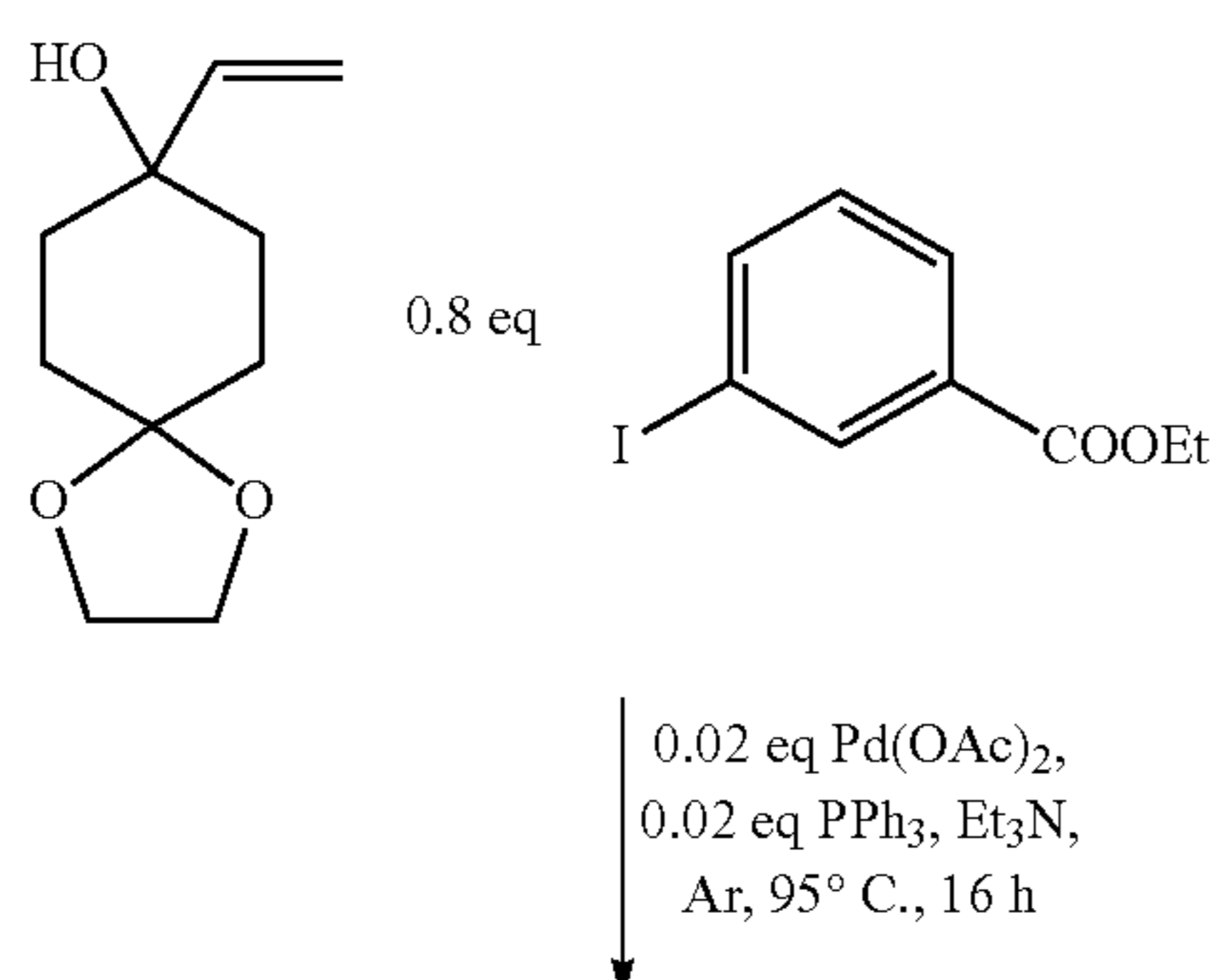
Scheme 15-1
