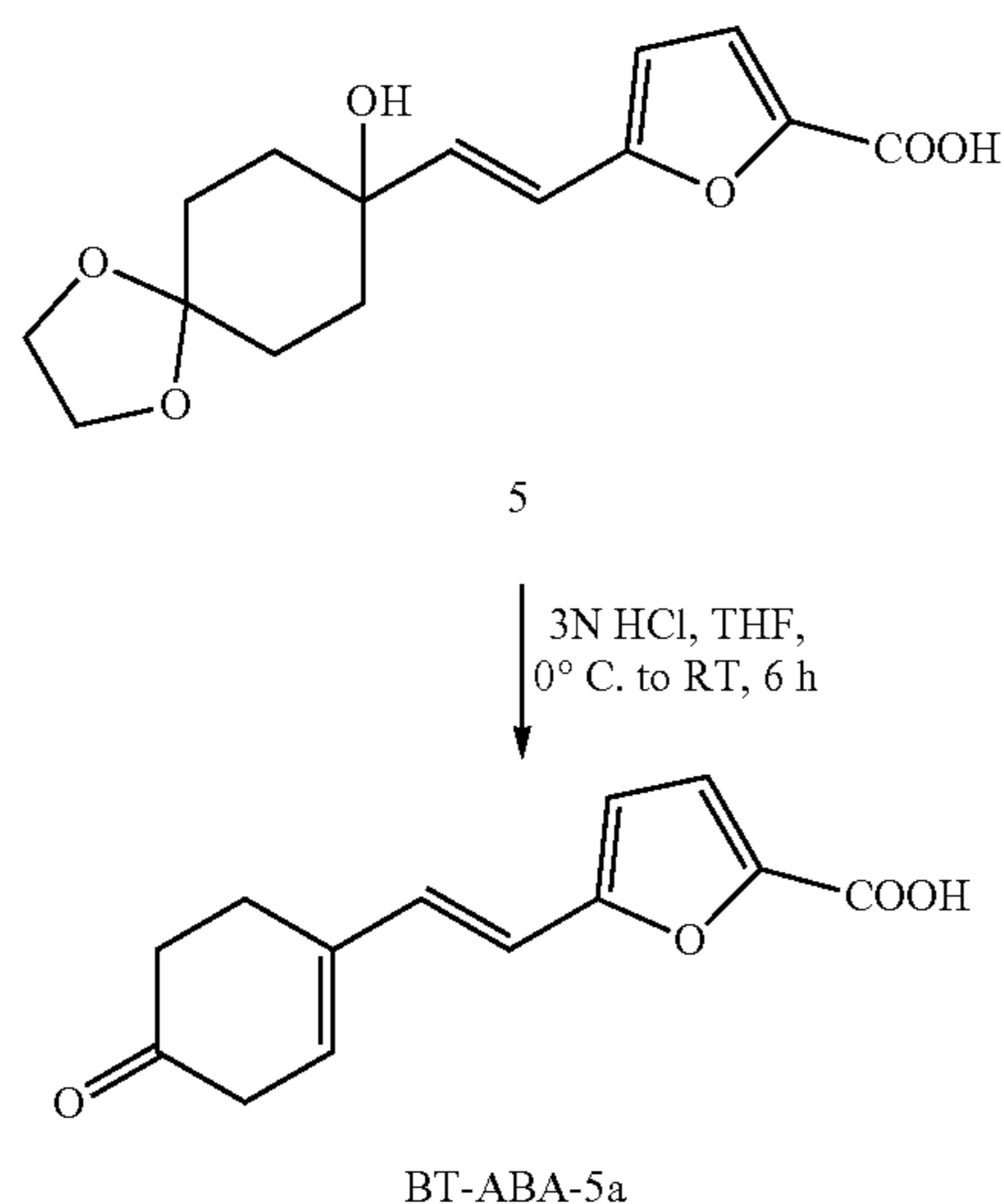
Scheme 14-3
