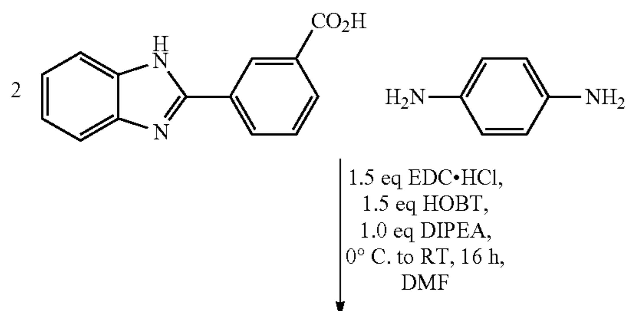
Scheme 8-1
