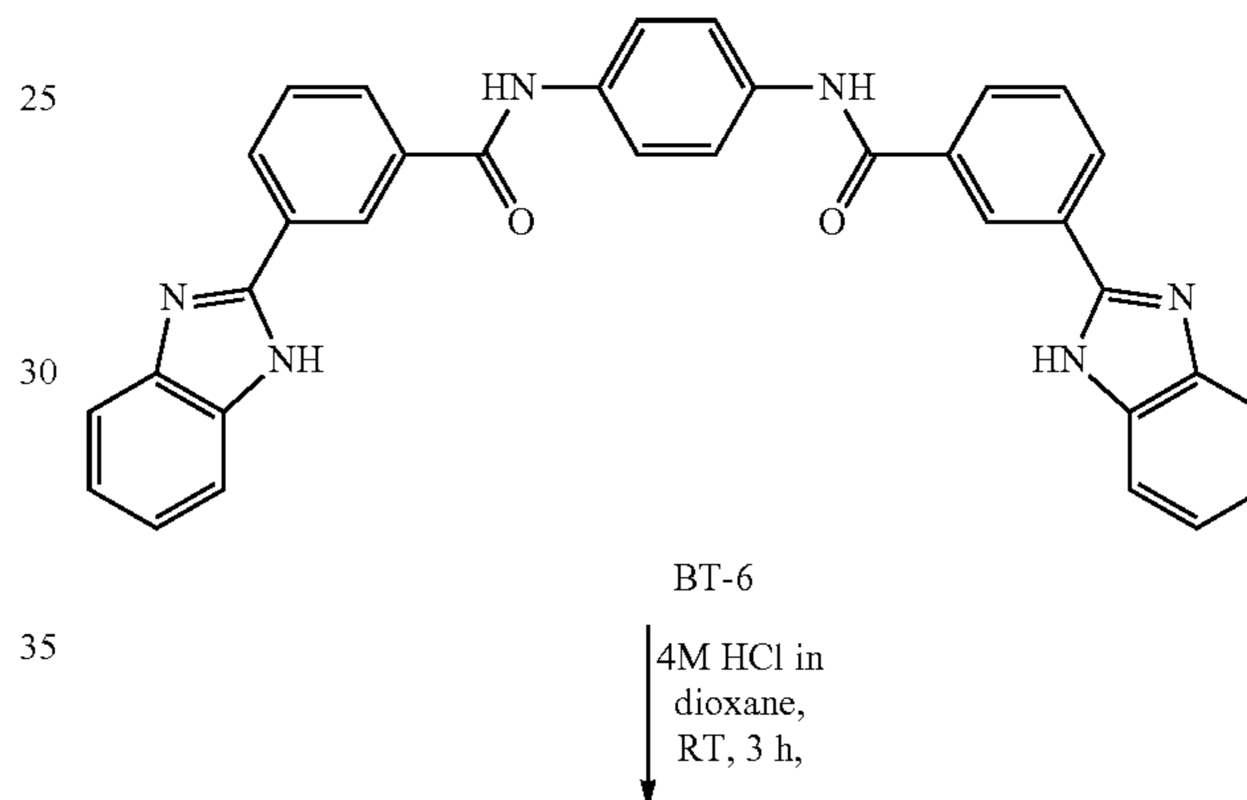
Scheme 8-2
