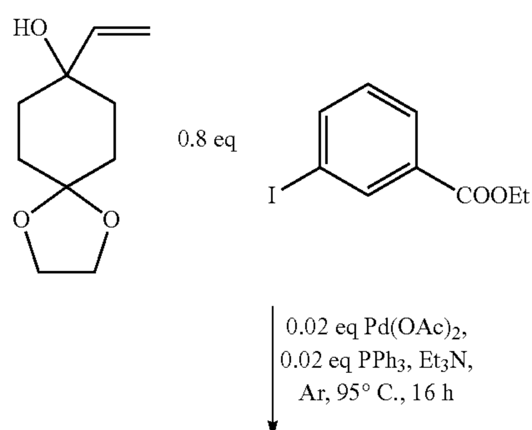
Scheme 15-1
