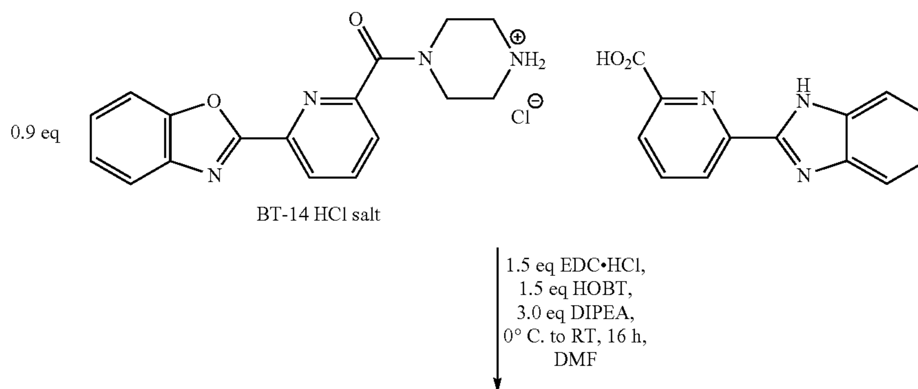
Scheme 5-1
