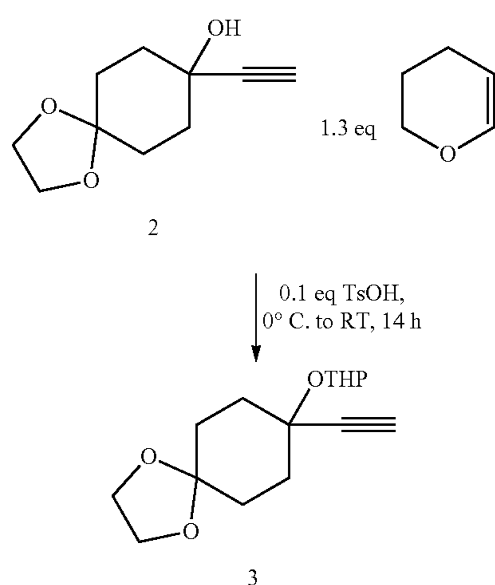
Scheme 16-1
