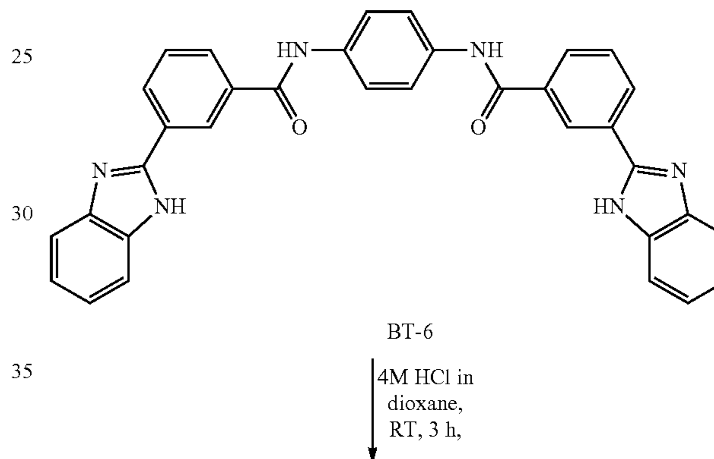
Scheme 8-2
