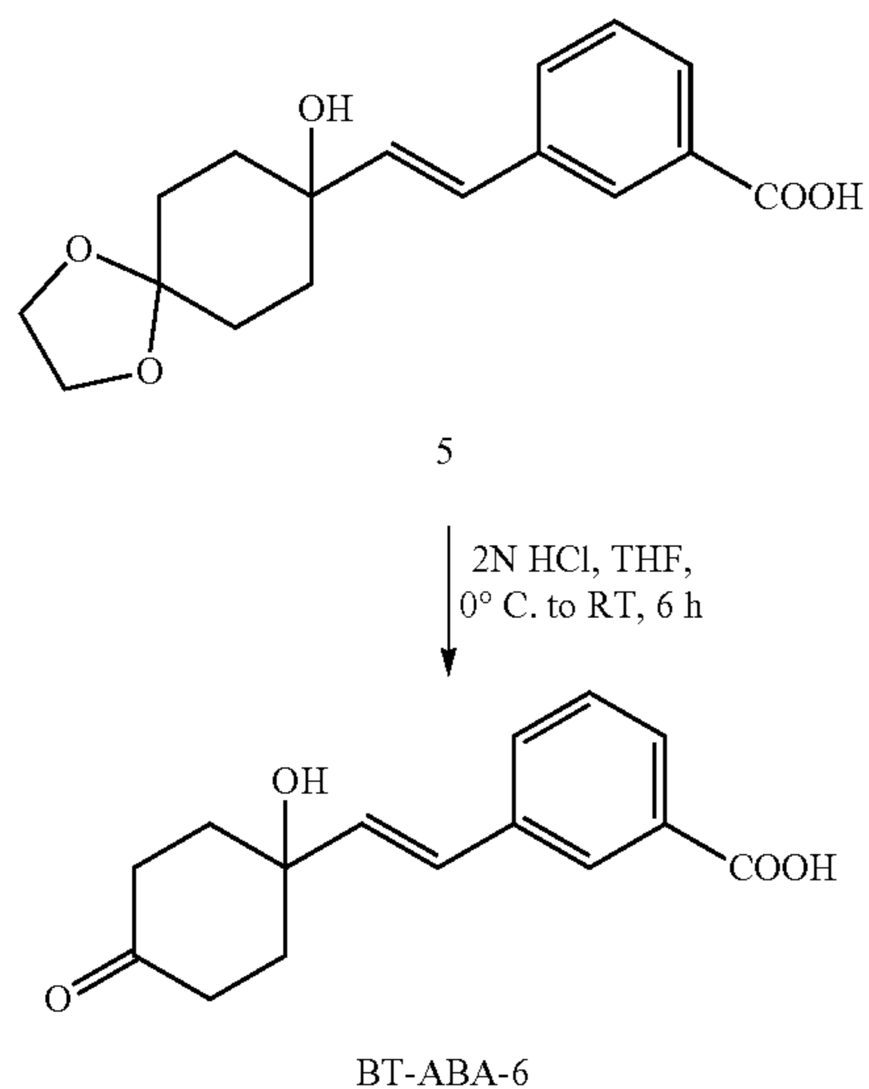
Scheme 15-3
