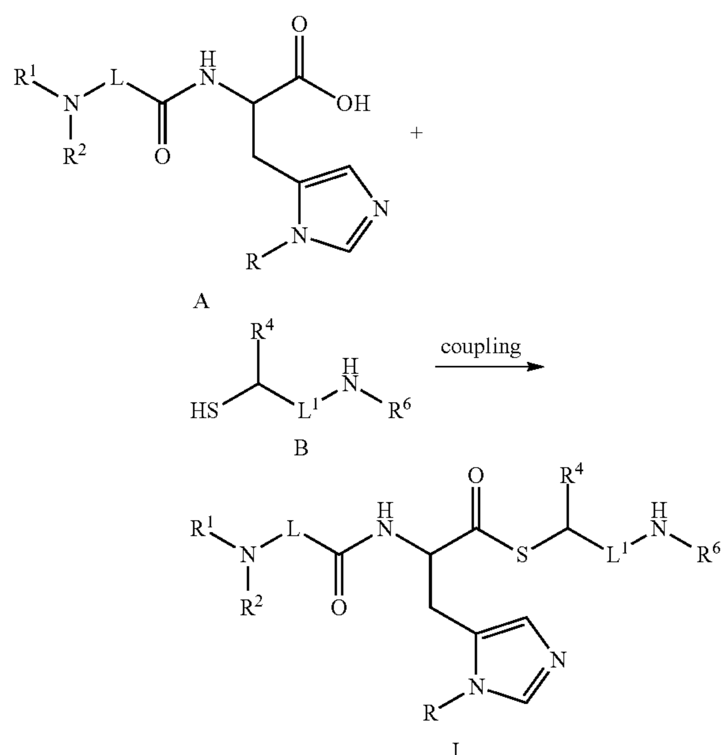
Scheme 1: Coupling of Intermediate acid A and thiol B
