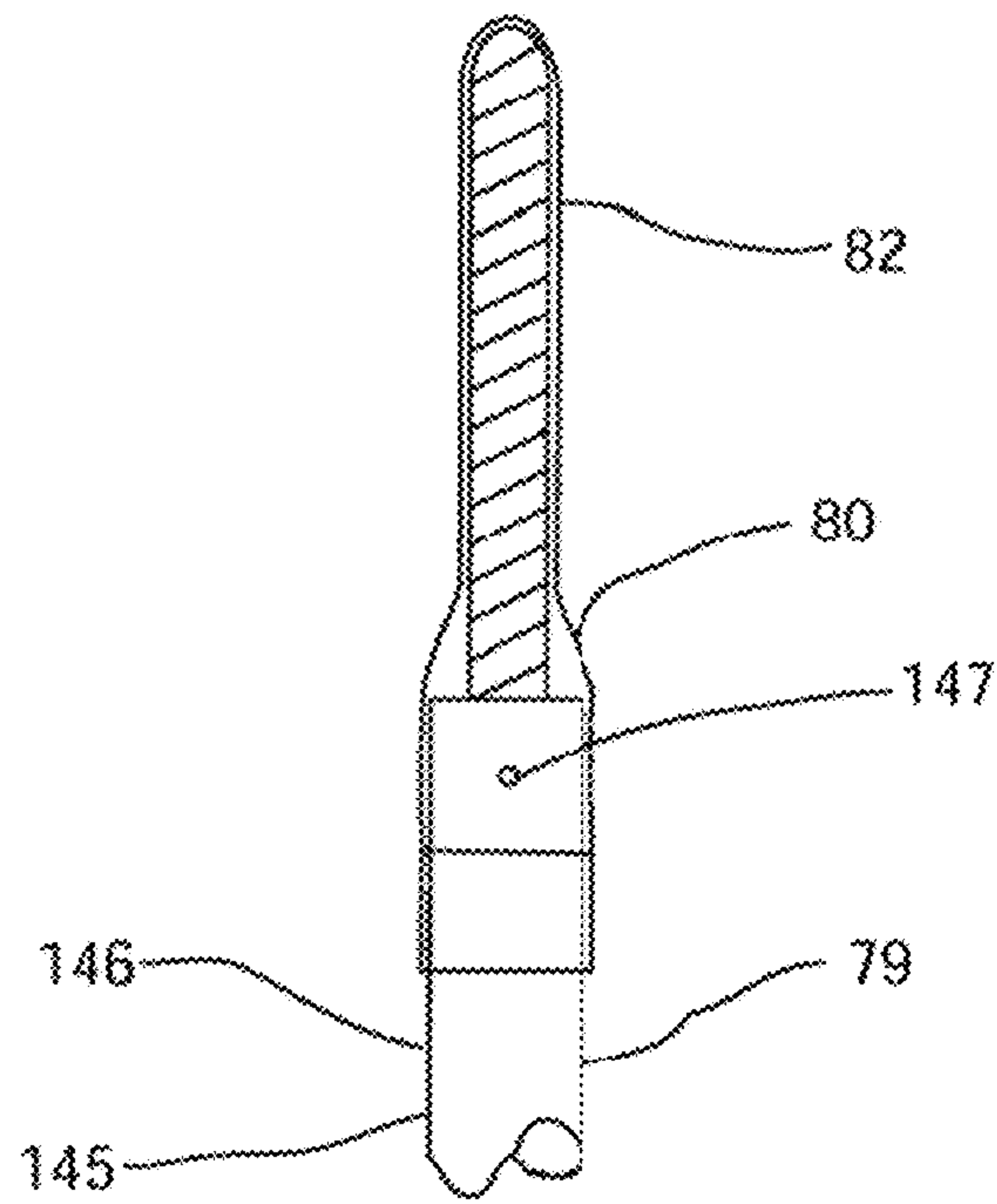
View C-C
