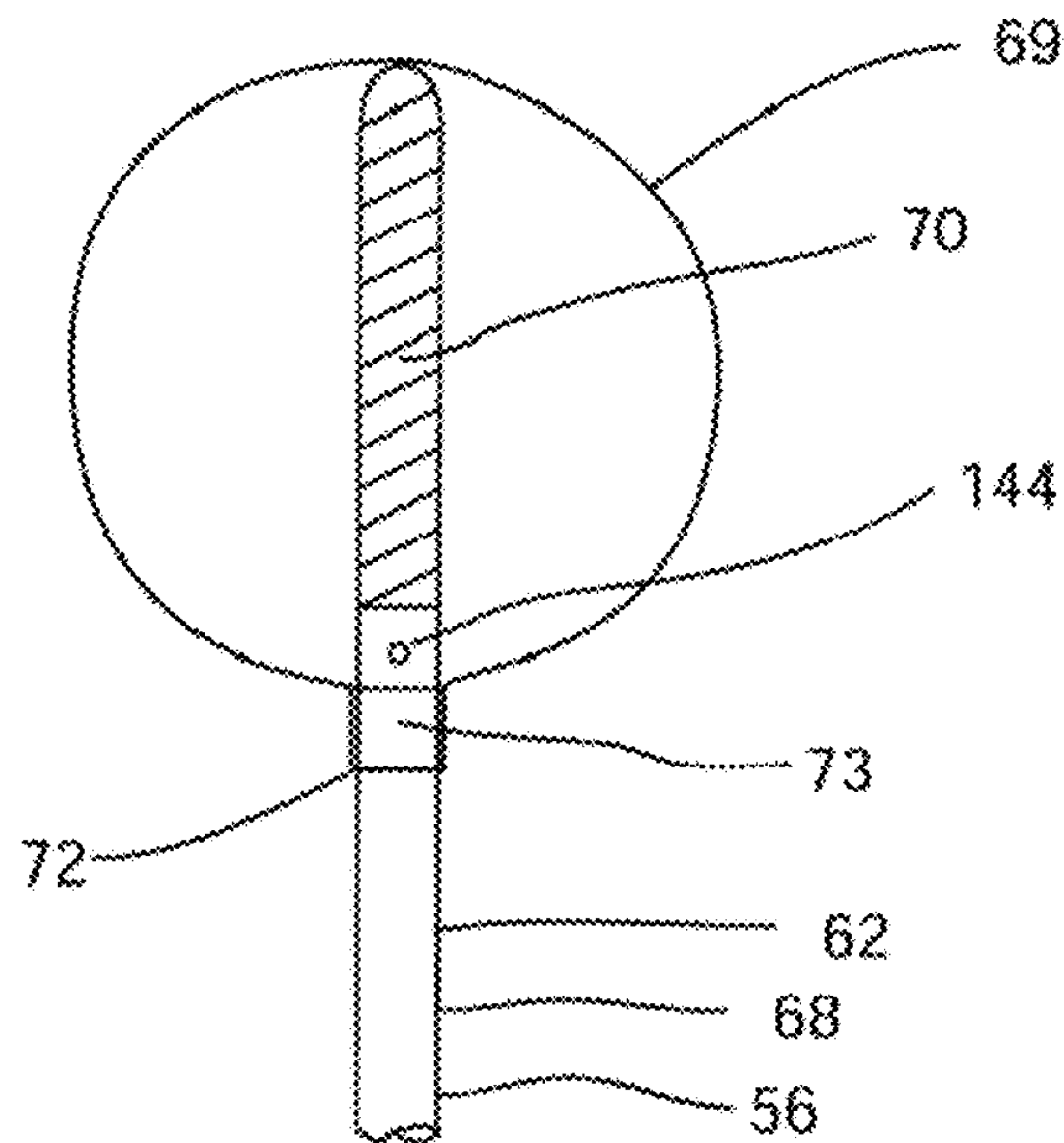
View B-B
