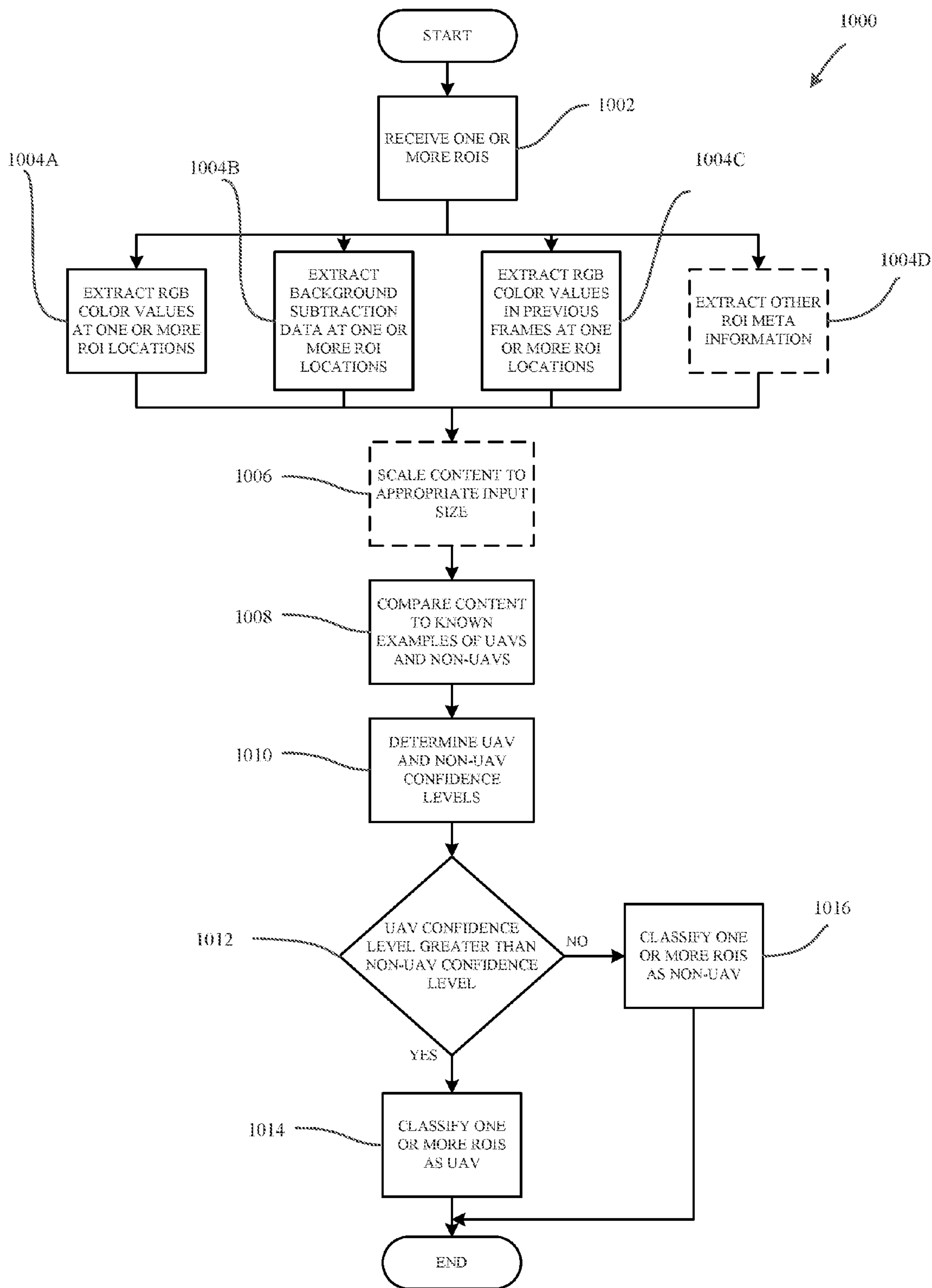
FIG. 10: EXEMPLARY OBJECT CLASSIFICATION PROCESS
