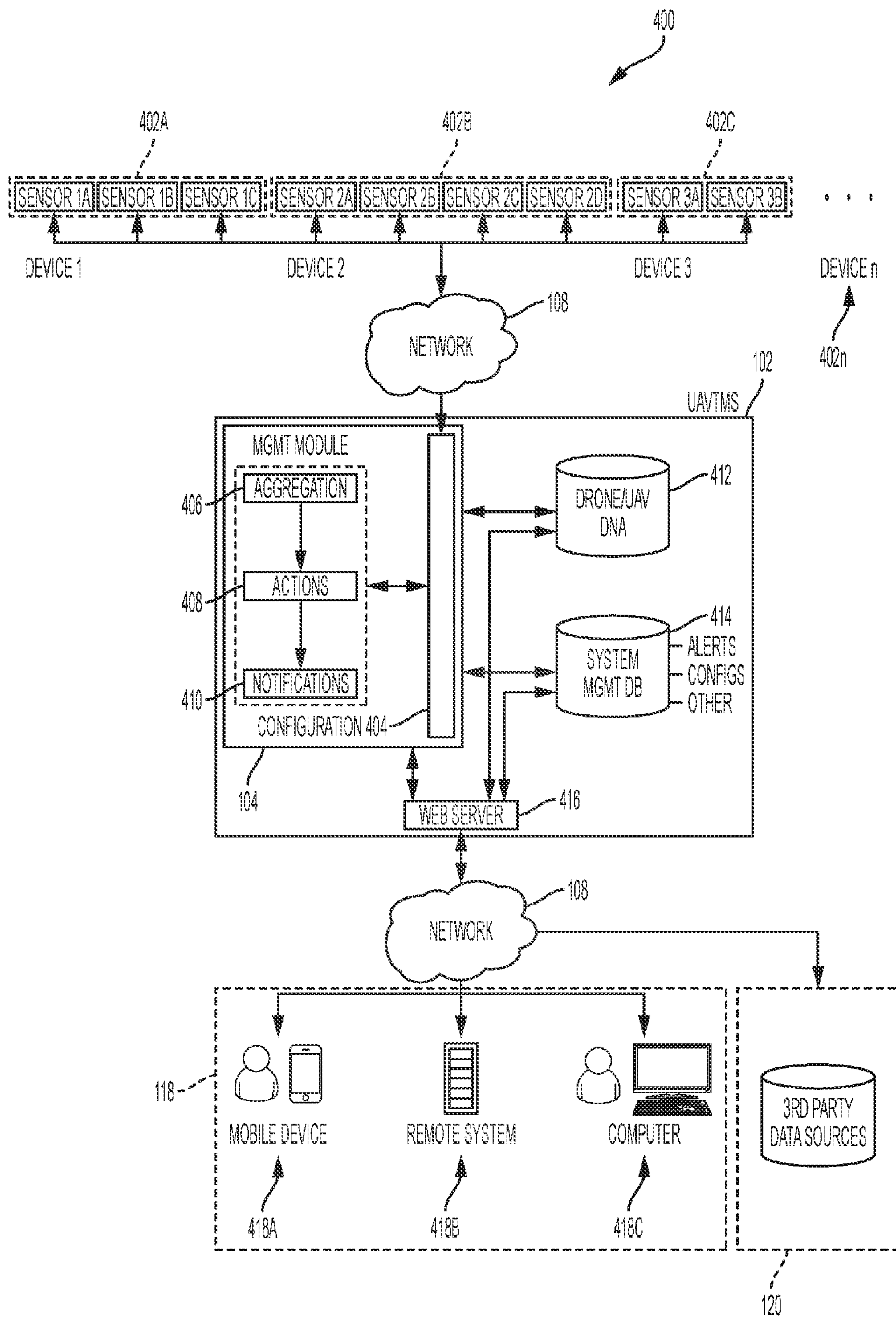
FIG. 4: EXEMPLARY SYSTEM ARCHITECTURE
