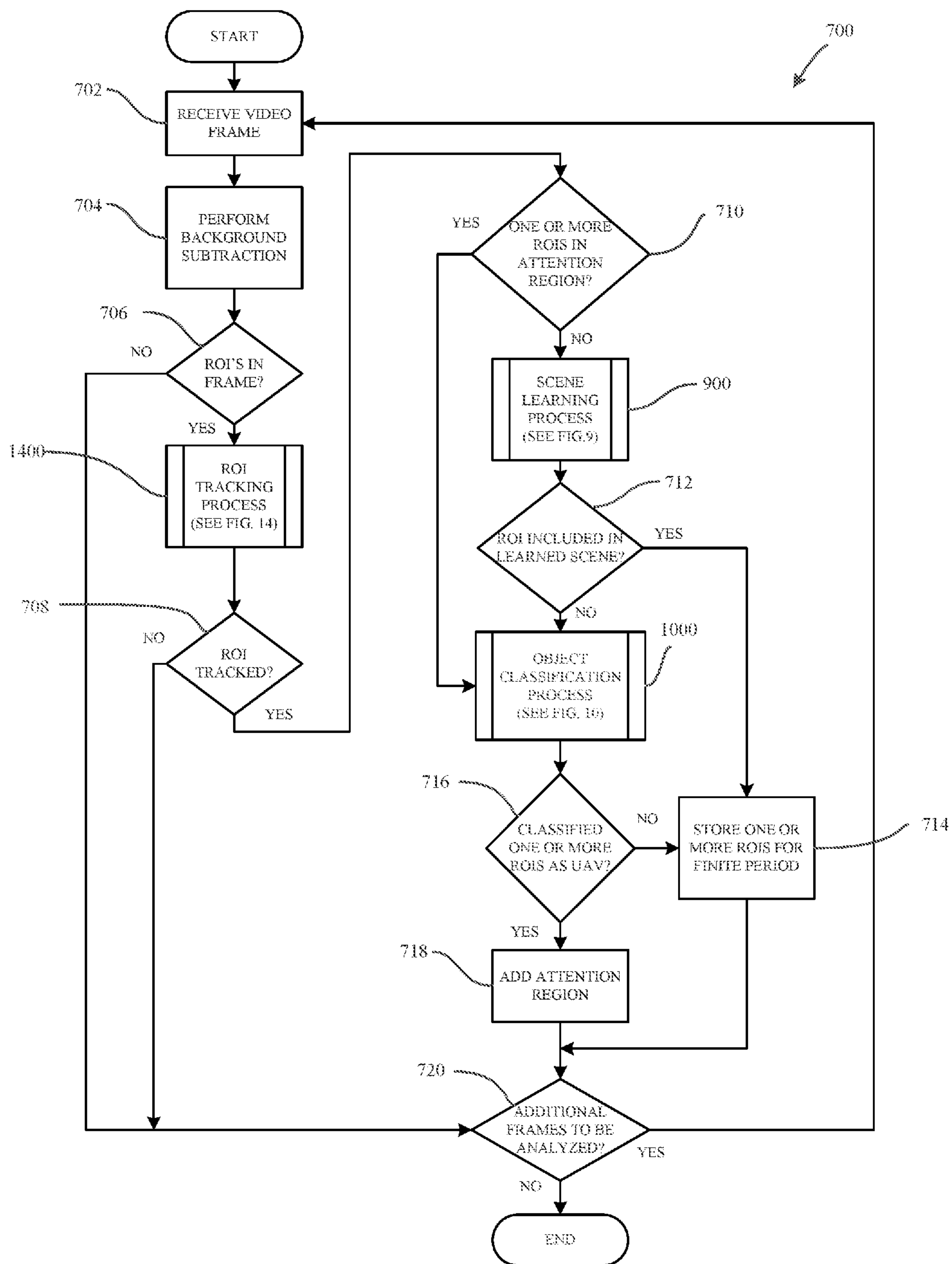
FIG. 7: EXEMPLARY VIDEO DATA ANALYSIS PROCESS
