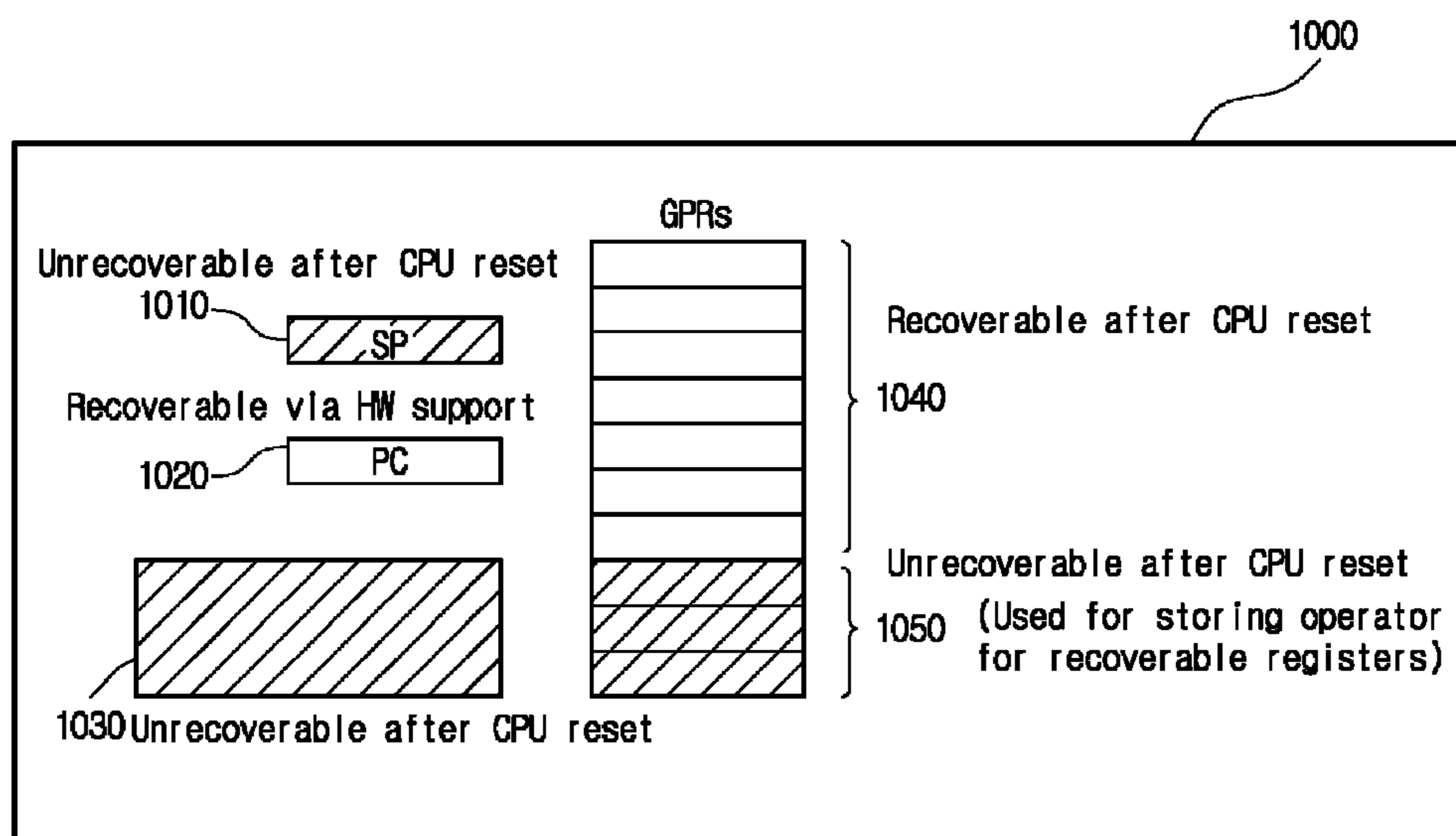
CPU core state after CPU reset
