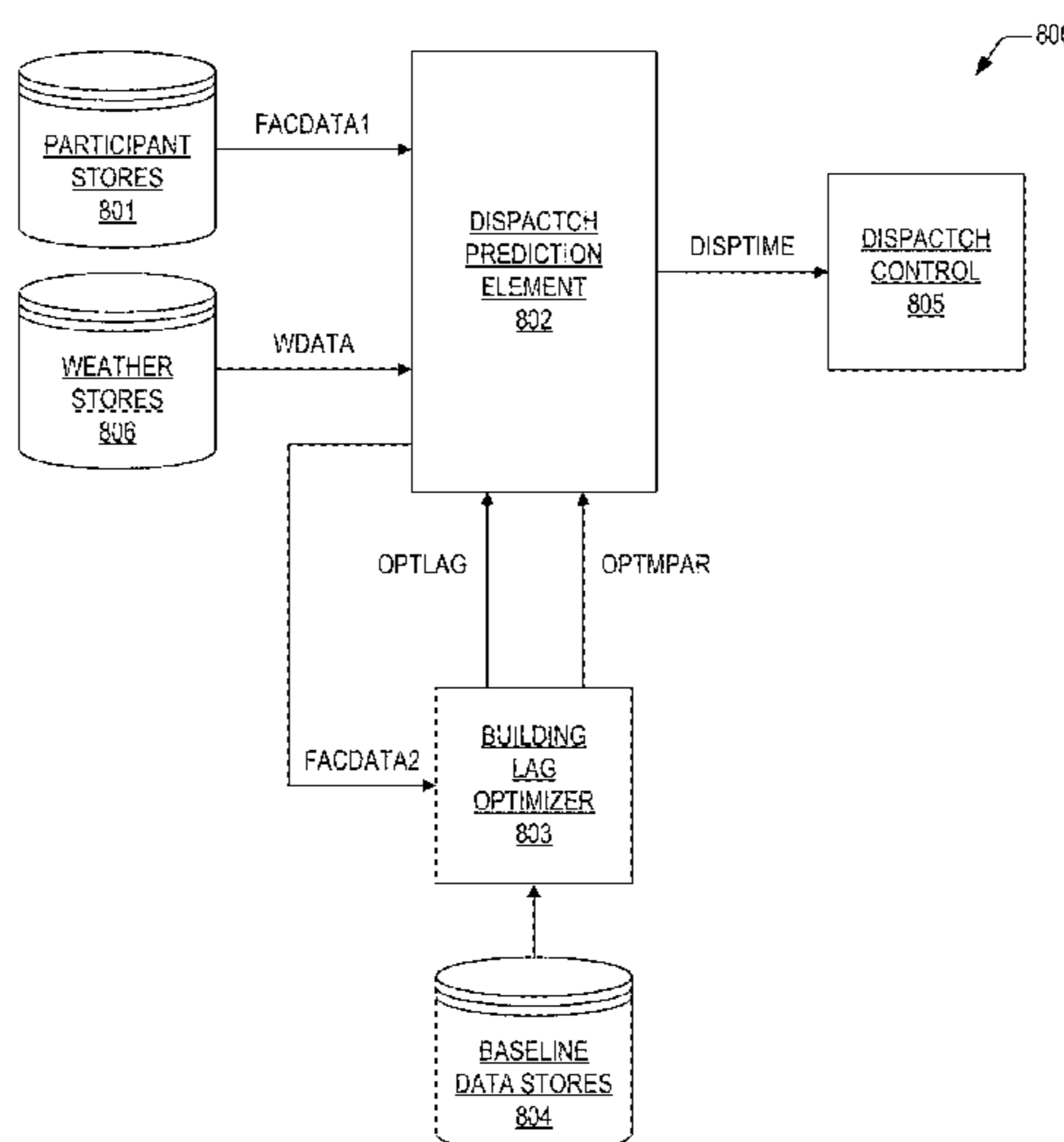
DEMAND RESPONSE DISPATCH PREDICTION SYSTEM
