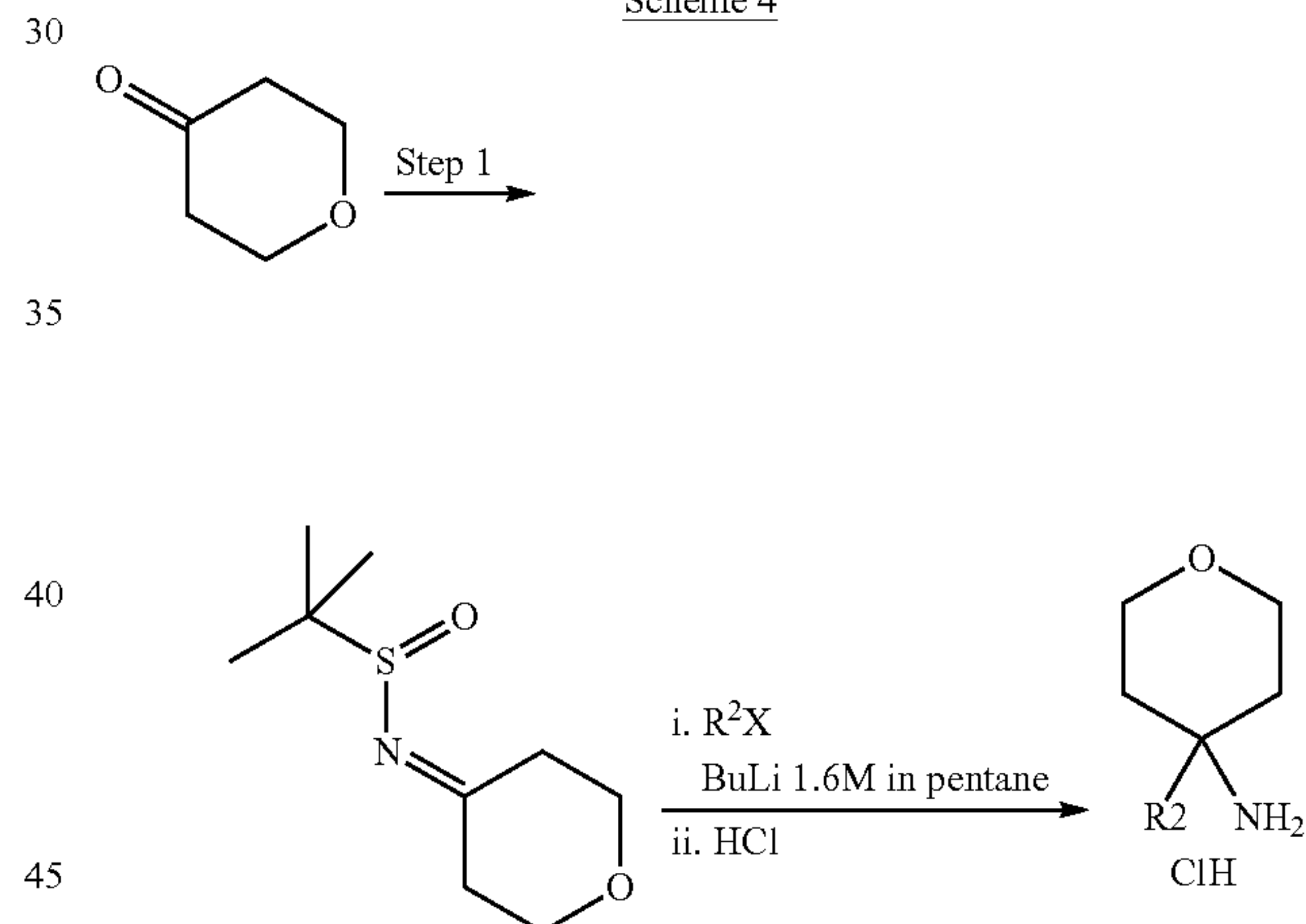
Scheme 4
