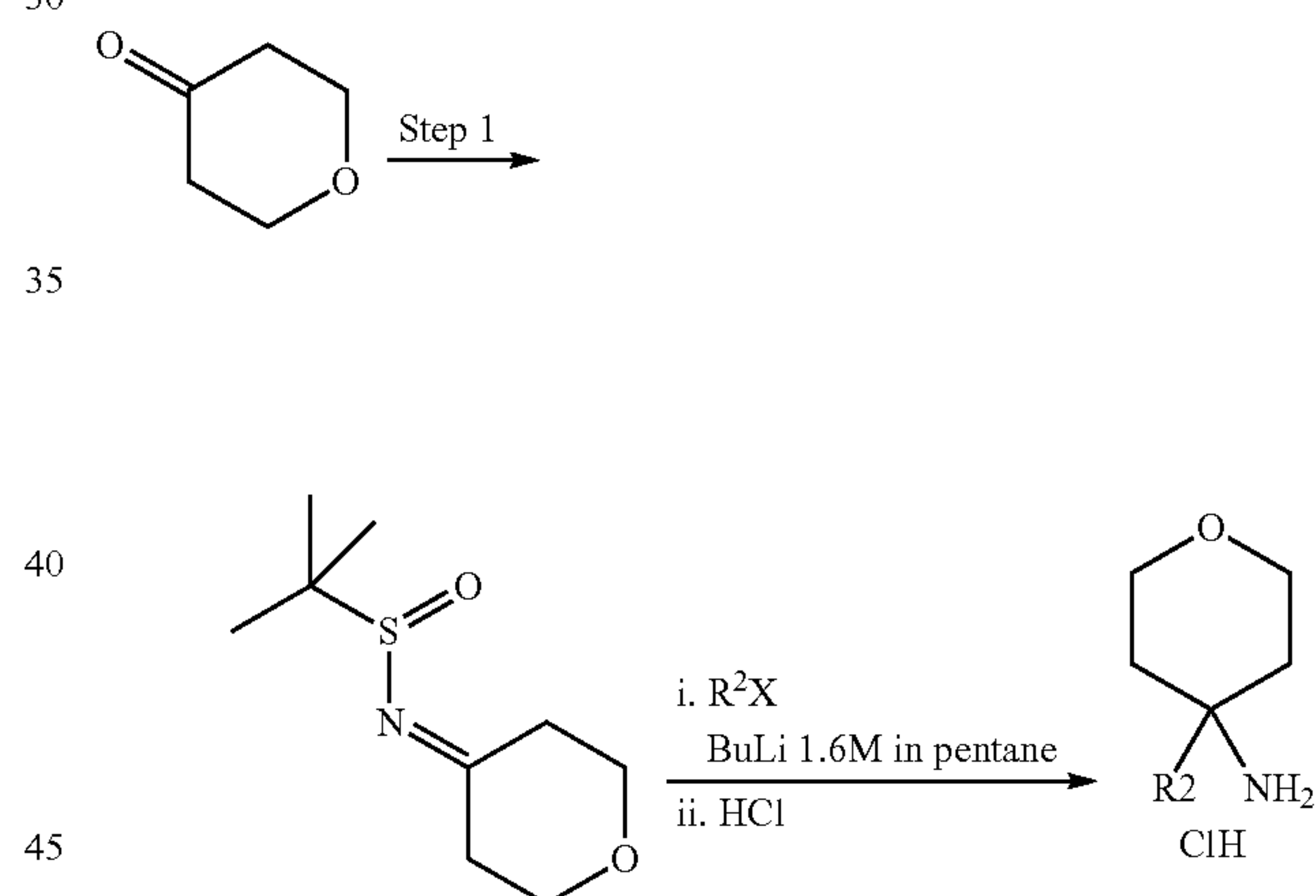
Scheme 4
