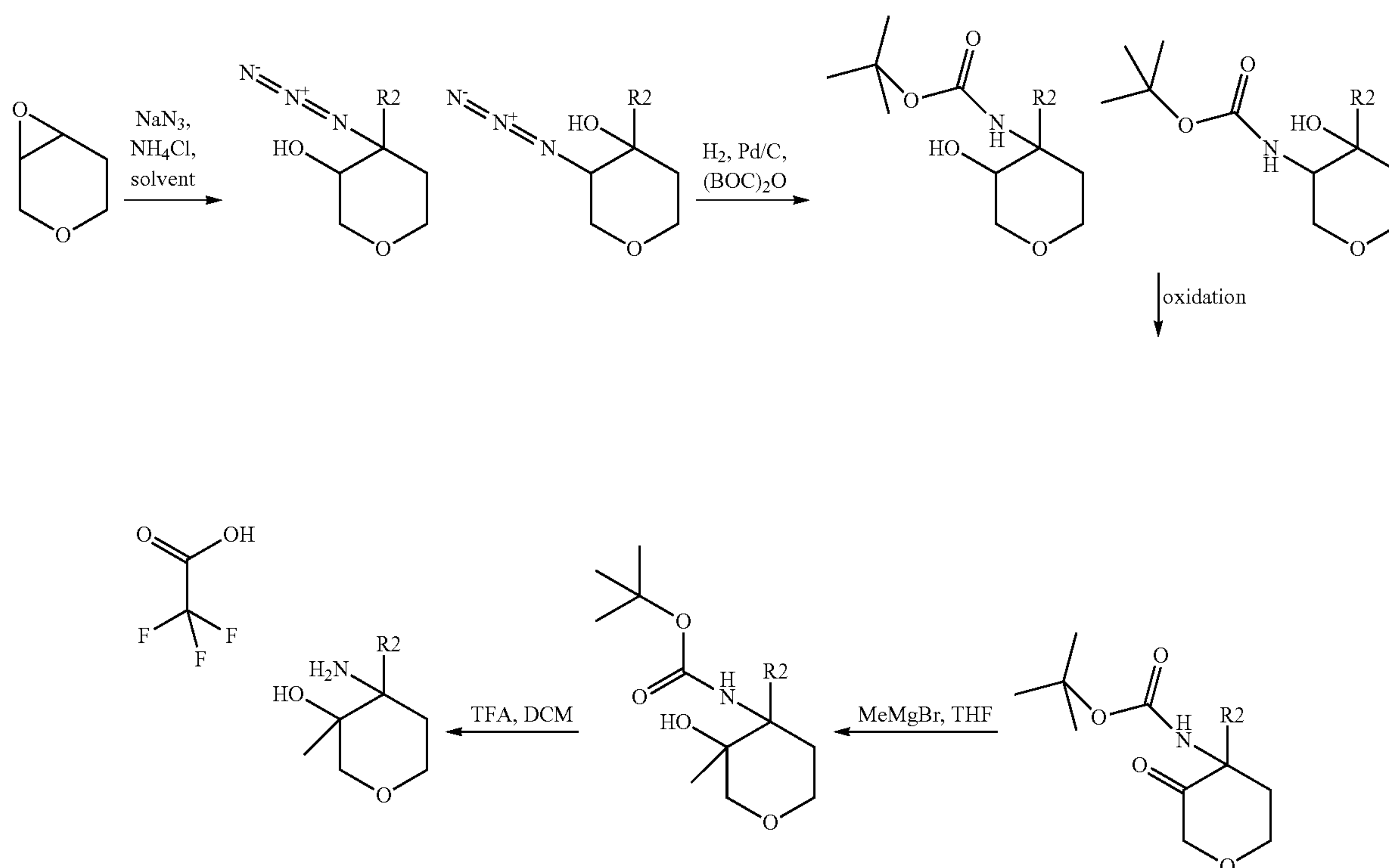
Scheme 7
