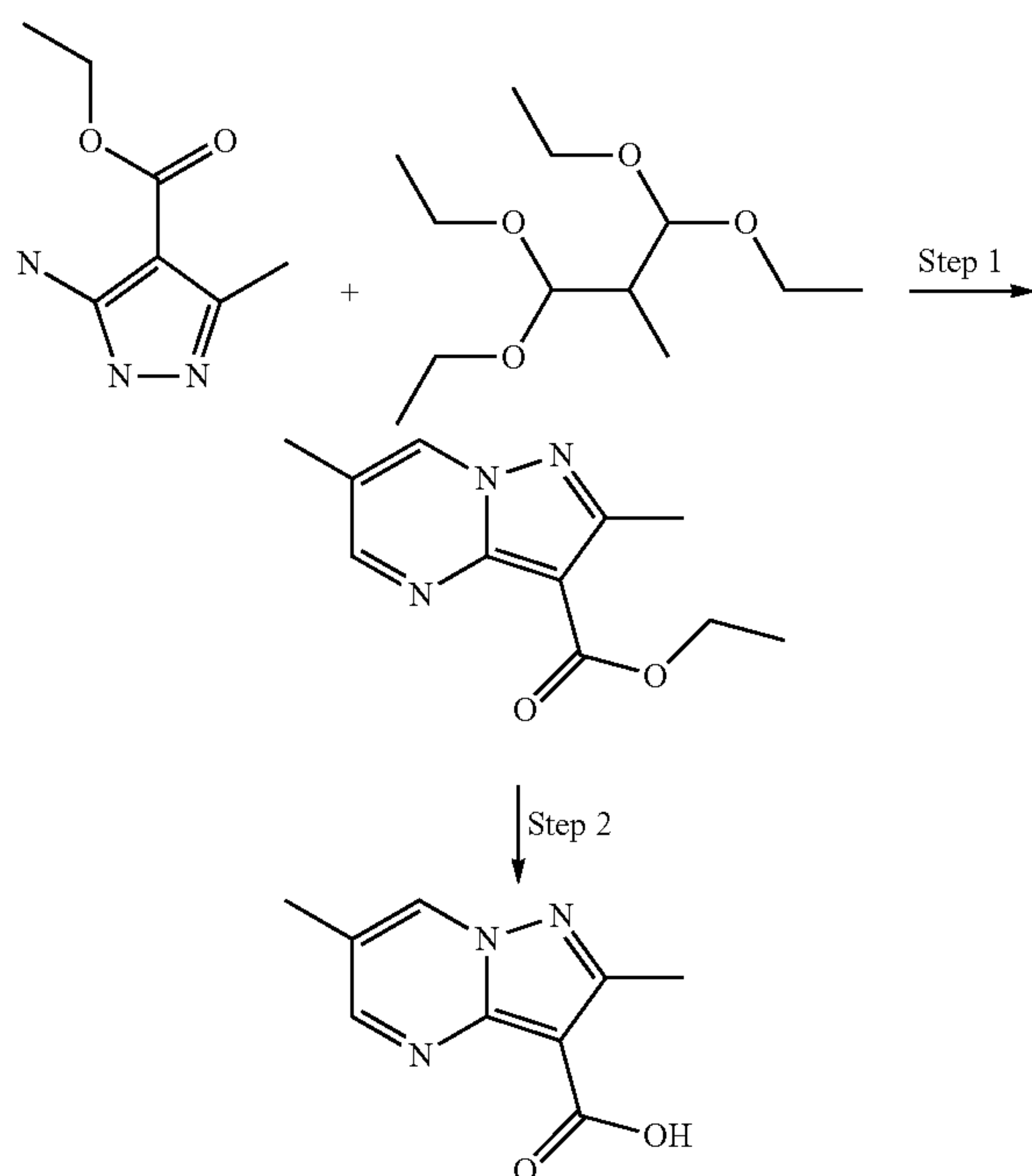
Scheme 3:
