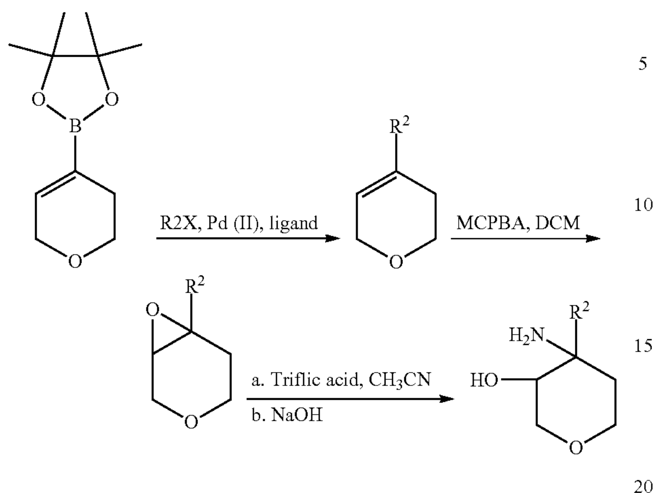
Scheme 5
