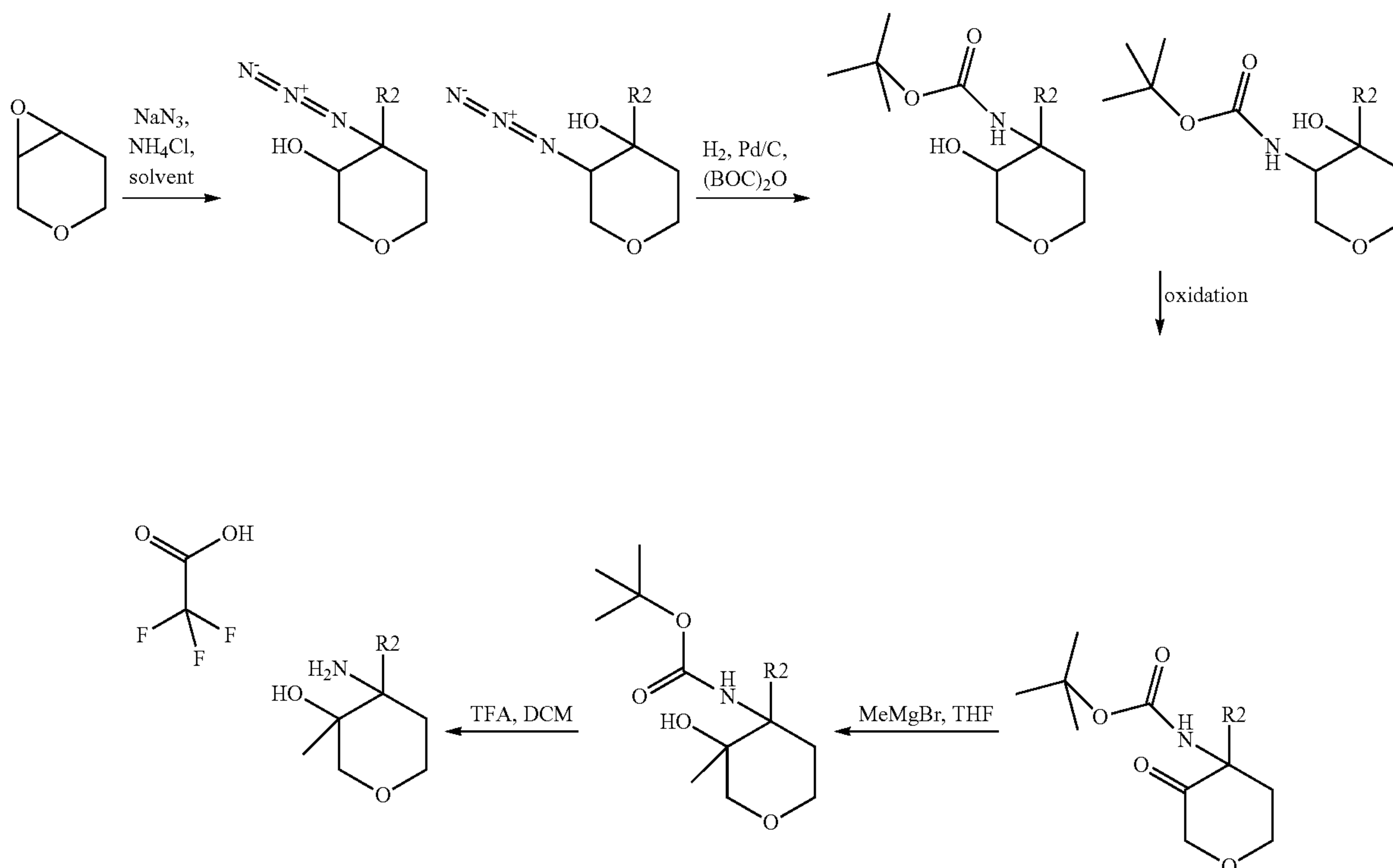
Scheme 7
