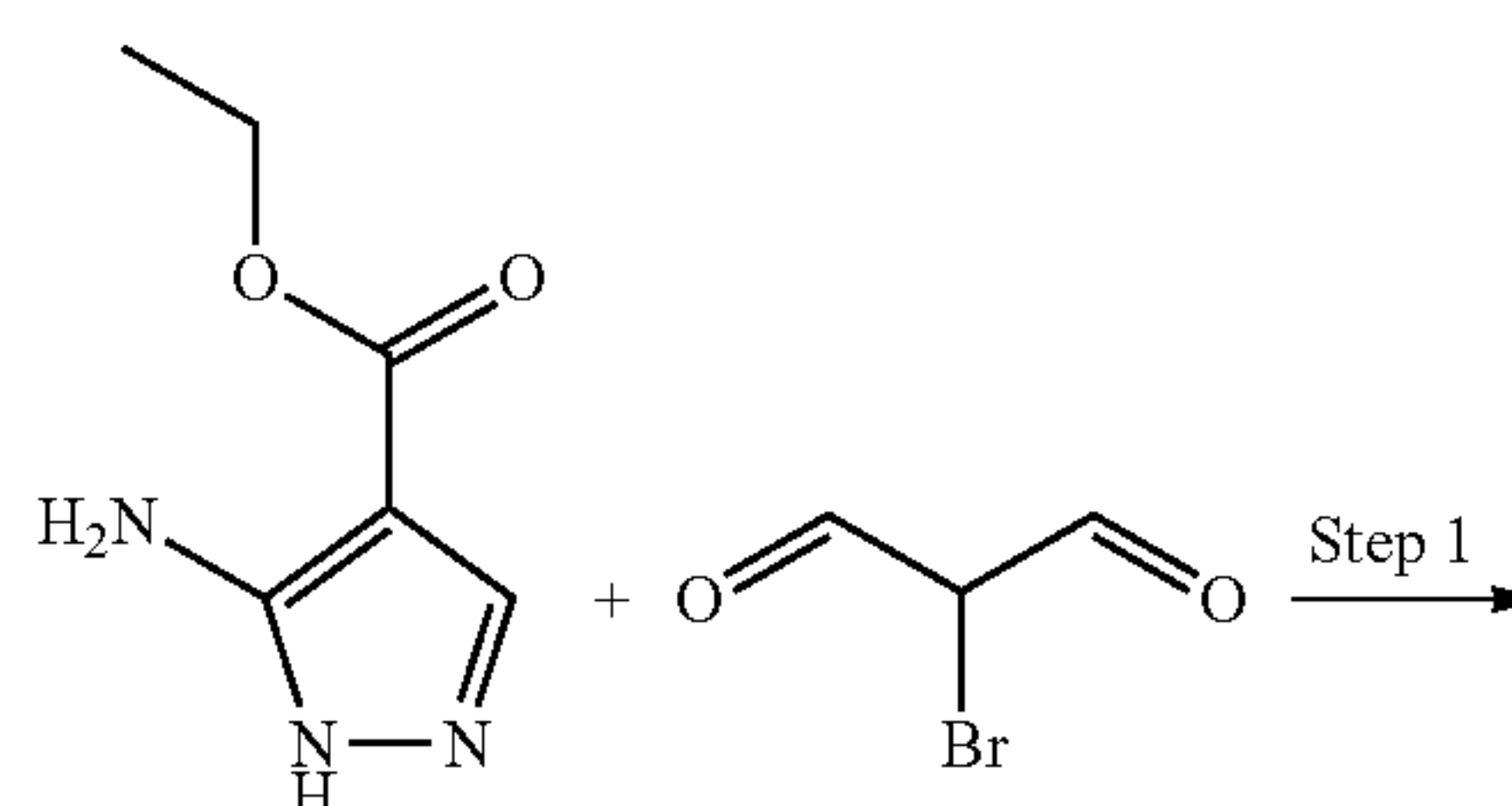
Scheme 1:
