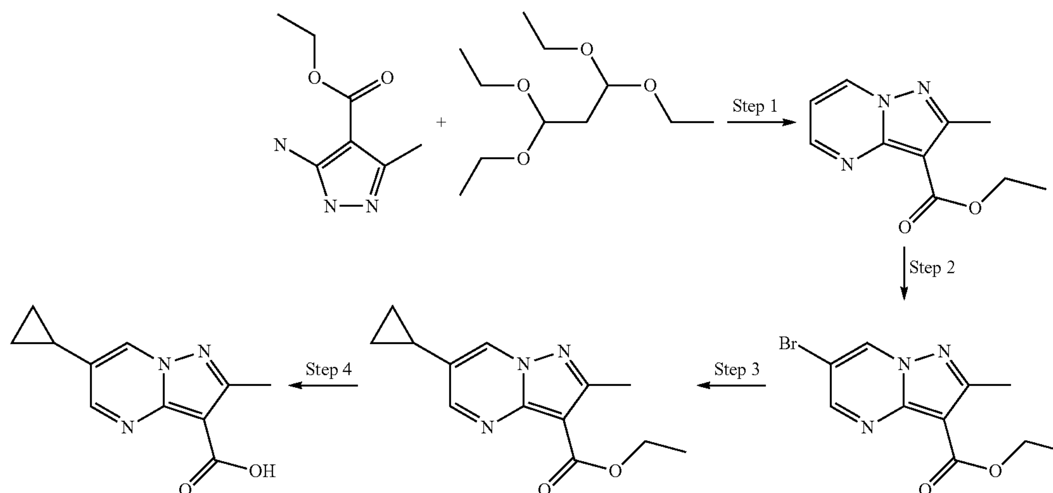
Scheme 2:
