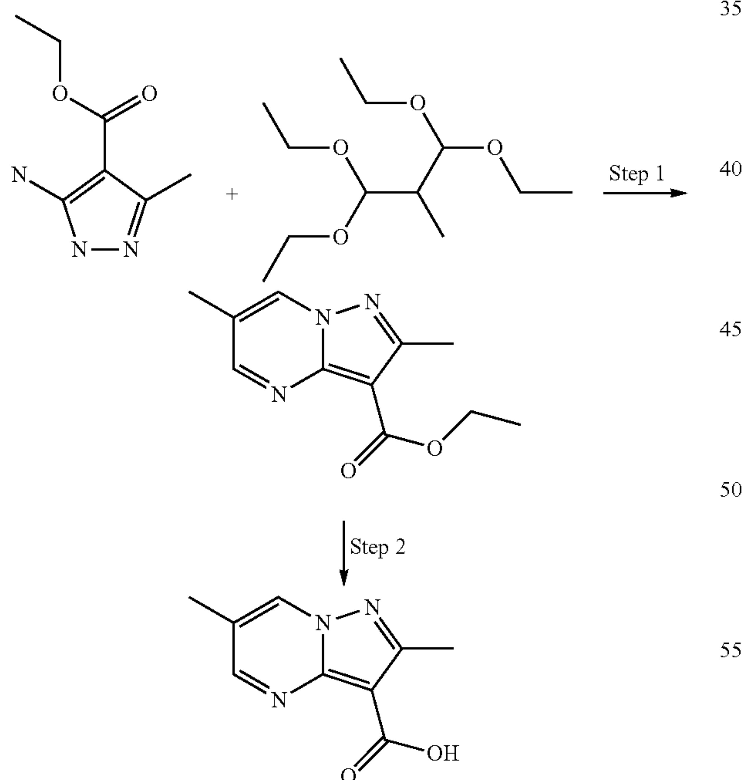
Scheme 3:
