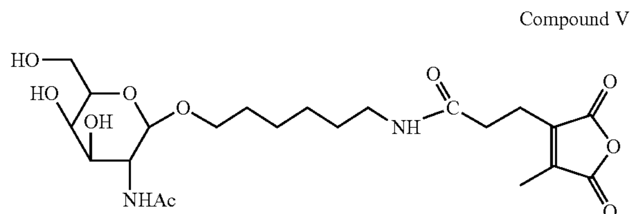
N-Acetyl-galactosamine-C 6 -methyl maleic anhydride masking agent
