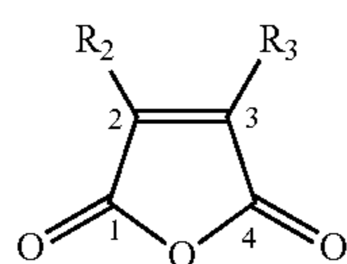
maleic anhydride system
