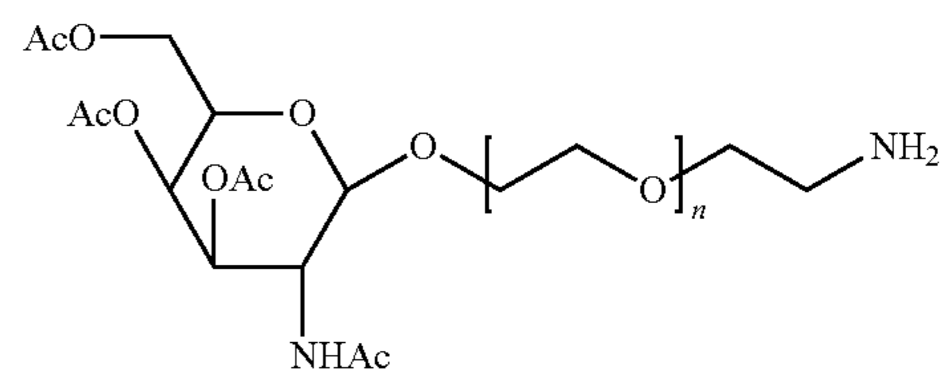
(Aminoethoxy)ethyl derivatives of 2-acetamido-3,4,6-tri-O-acetyl-2-deoxy- \beta -D-galactopyranoside
