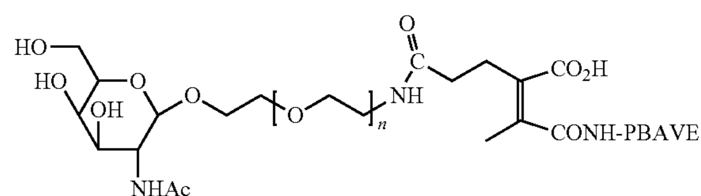
Compound III
