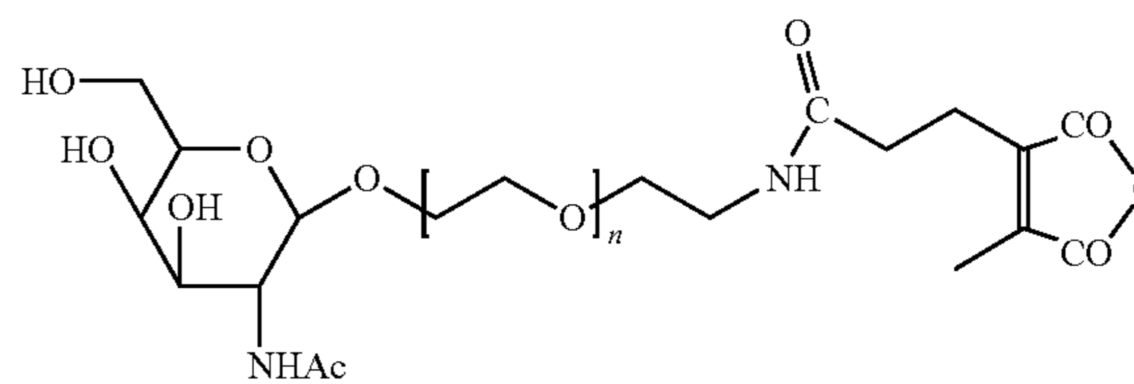
Compound II
