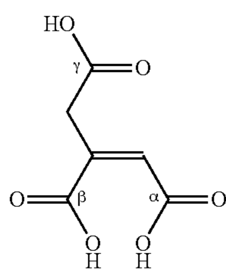
aconitic acid
