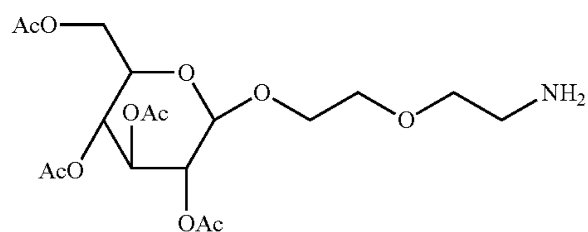
Glc β-isomer
