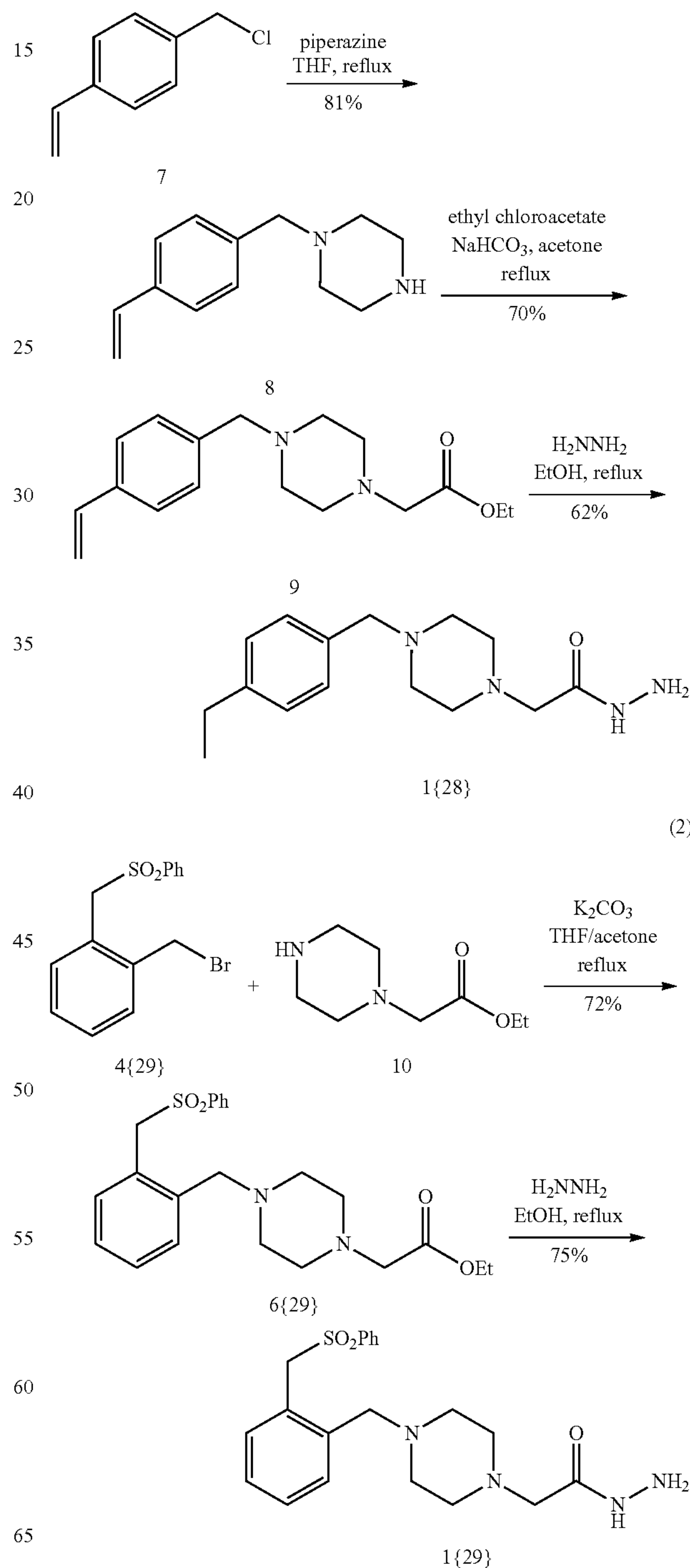
Scheme 2: Synthesis of hydrazides 1{28-31}.
