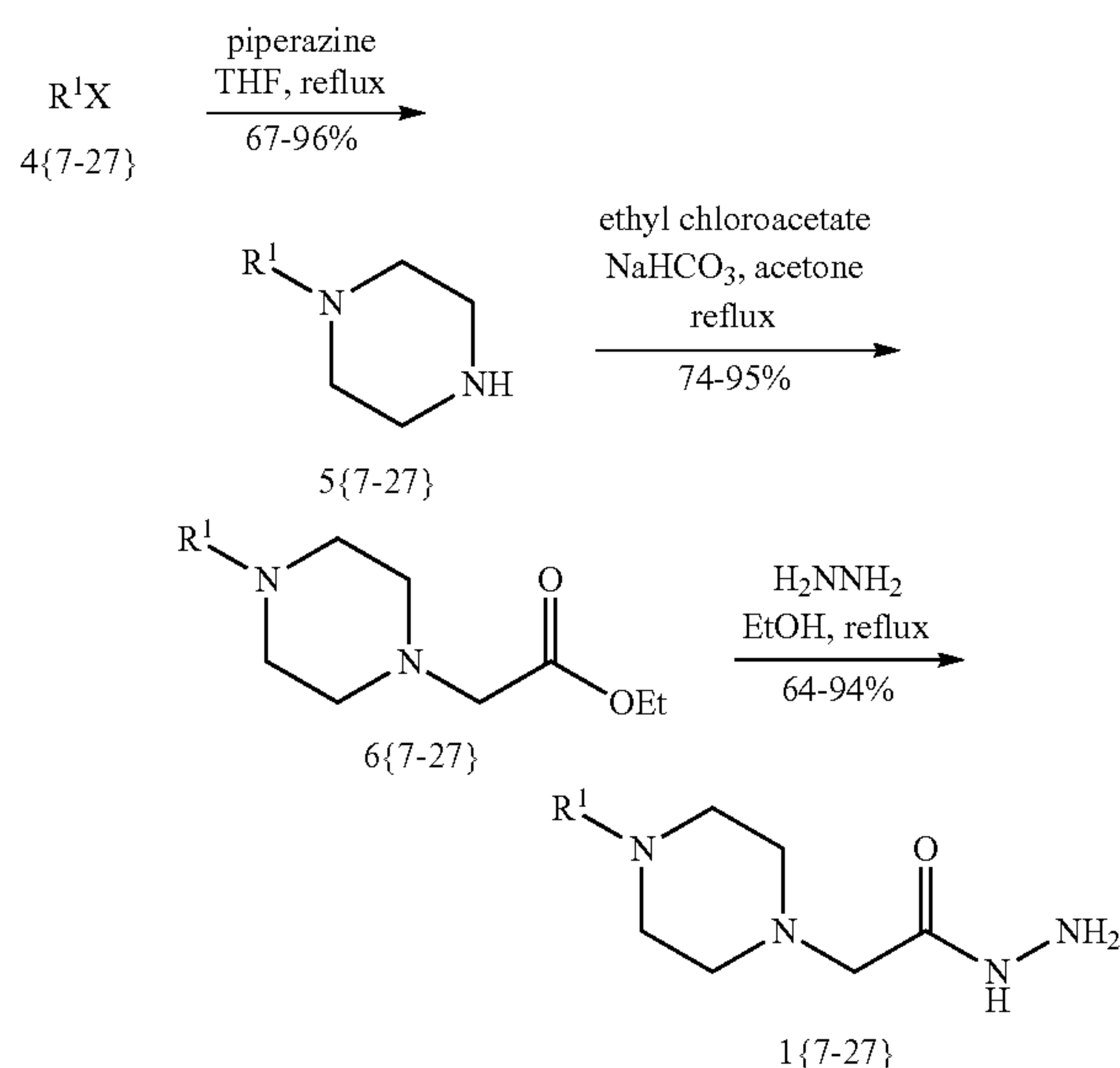
Scheme 1: Synthesis of hydrazides 1{7-27}.
