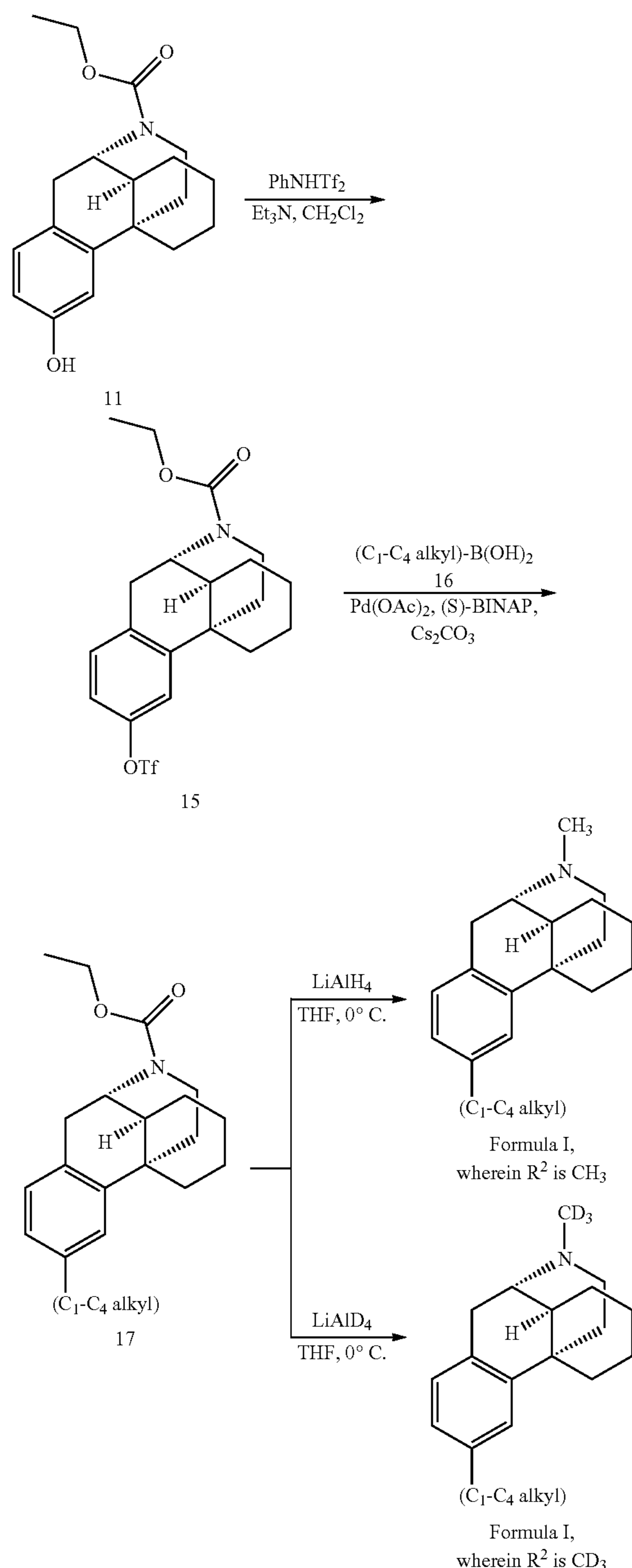
Scheme 2. Synthesis of a Compound of Formula I (R 1 is —(C 1 -C 4 )alkyl)
