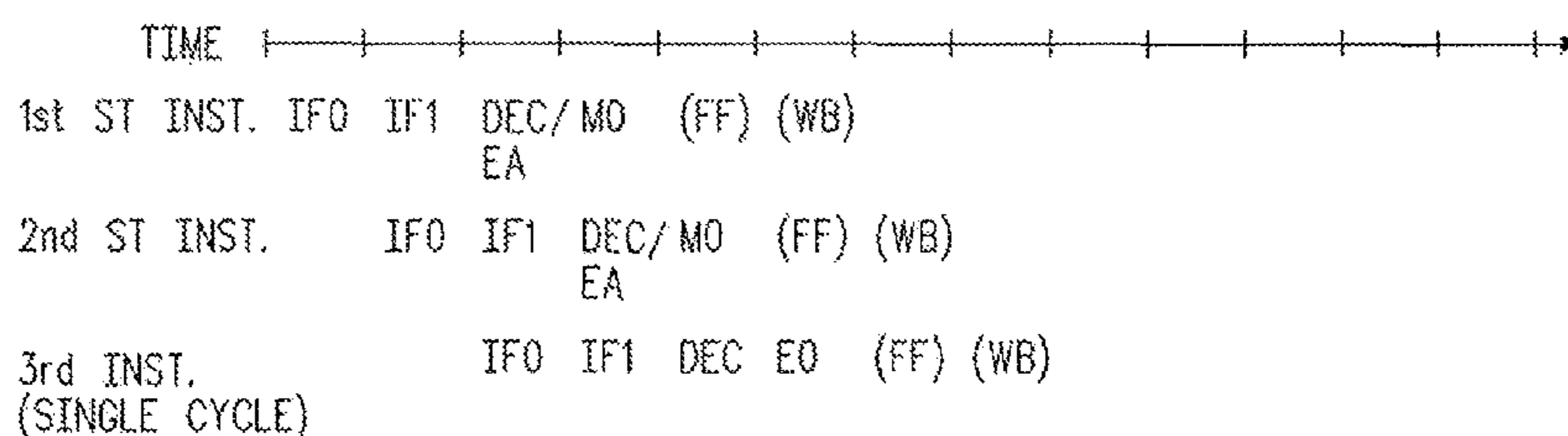
PIPELINE FLOW, STORE INSTRUCTIONS, PARITY MODE
