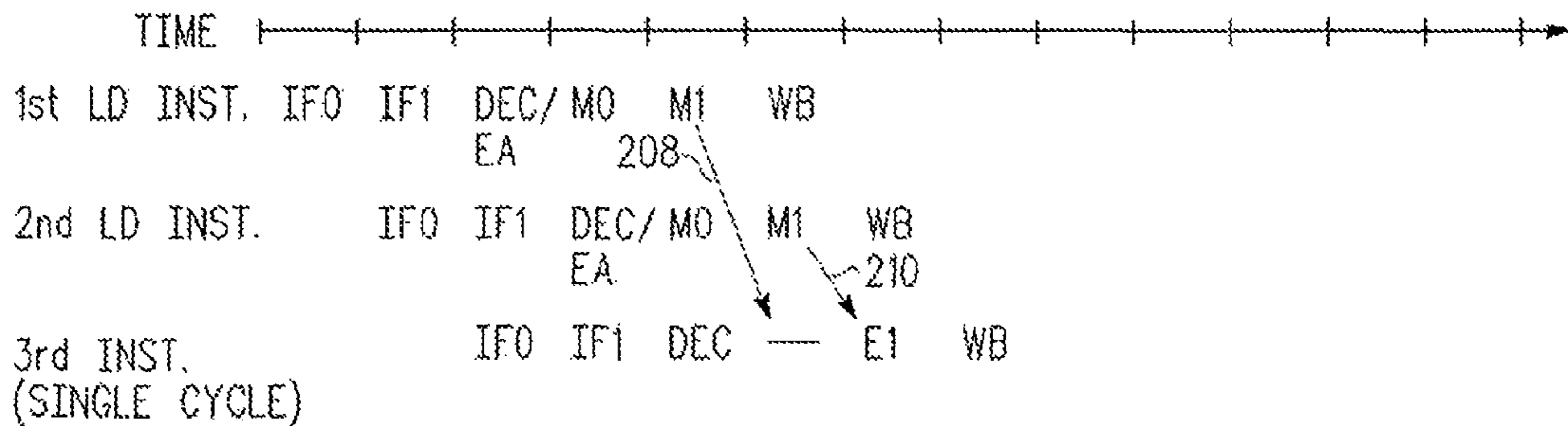
PIPELINE FLOW, LOAD INSTRUCTIONS, ECC MODE
