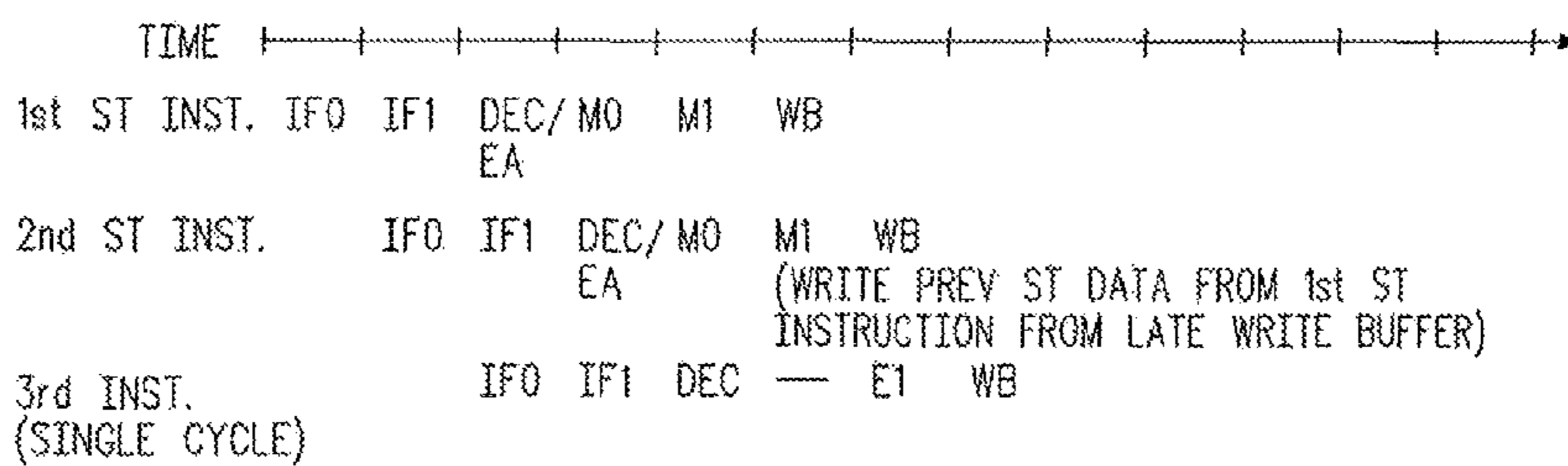
PIPELINE FLOW, STORE INSTRUCTIONS, ECC MODE
