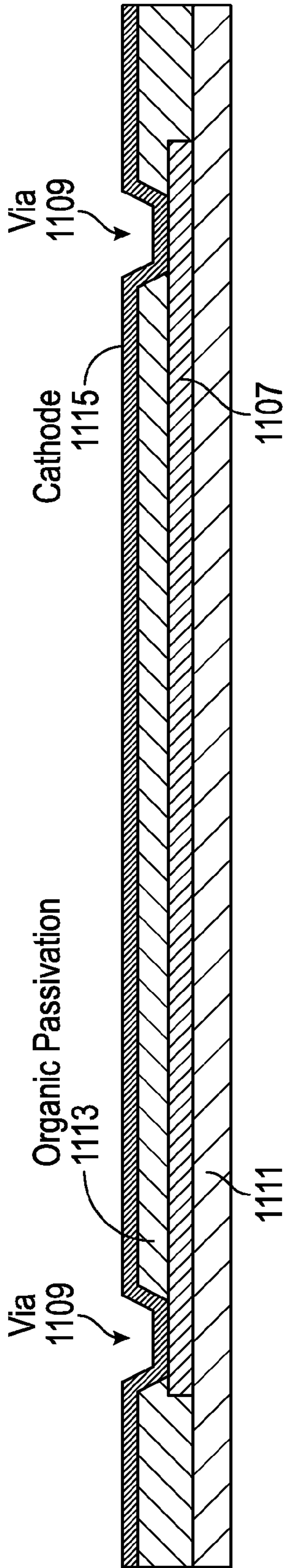
FIG. 11B-1 Anode Connection
