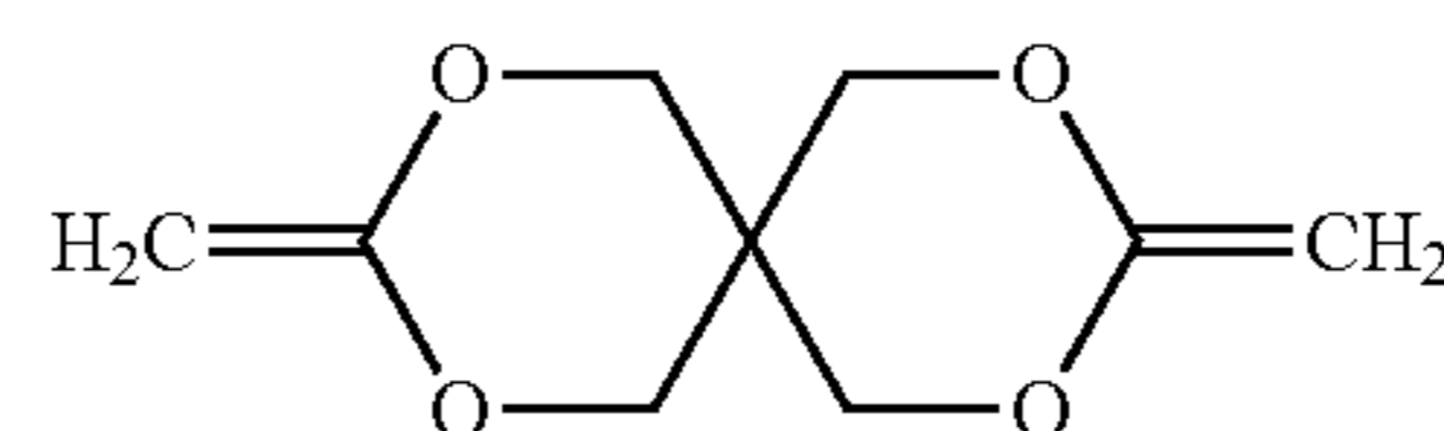
3,9-divinyl-2,4,8,10-tetraoxy-spiro[5.5]undecane
