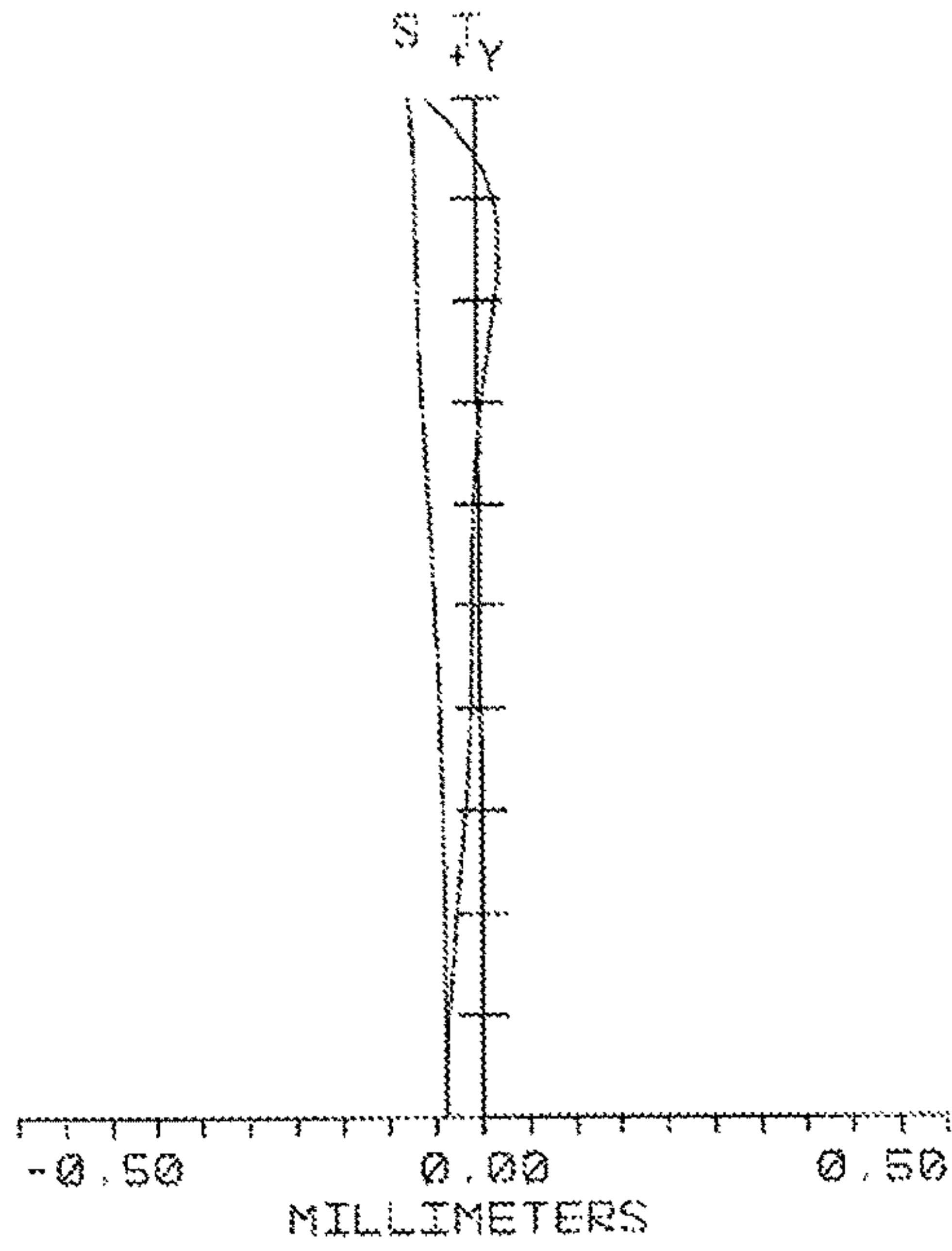
FIG. 3C FIELD CURVATURE
