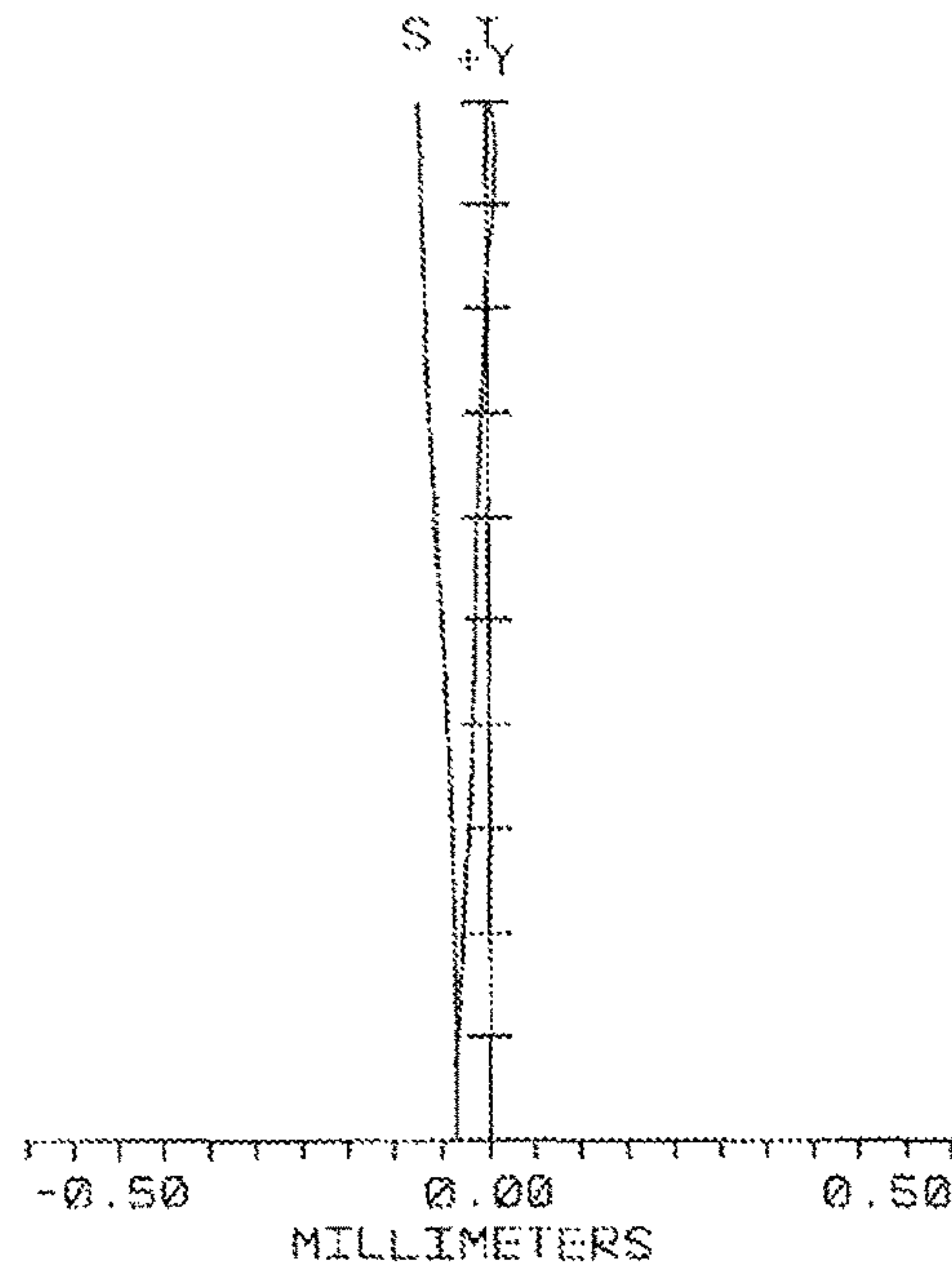
FIG. 6C FIELD CURVATURE
