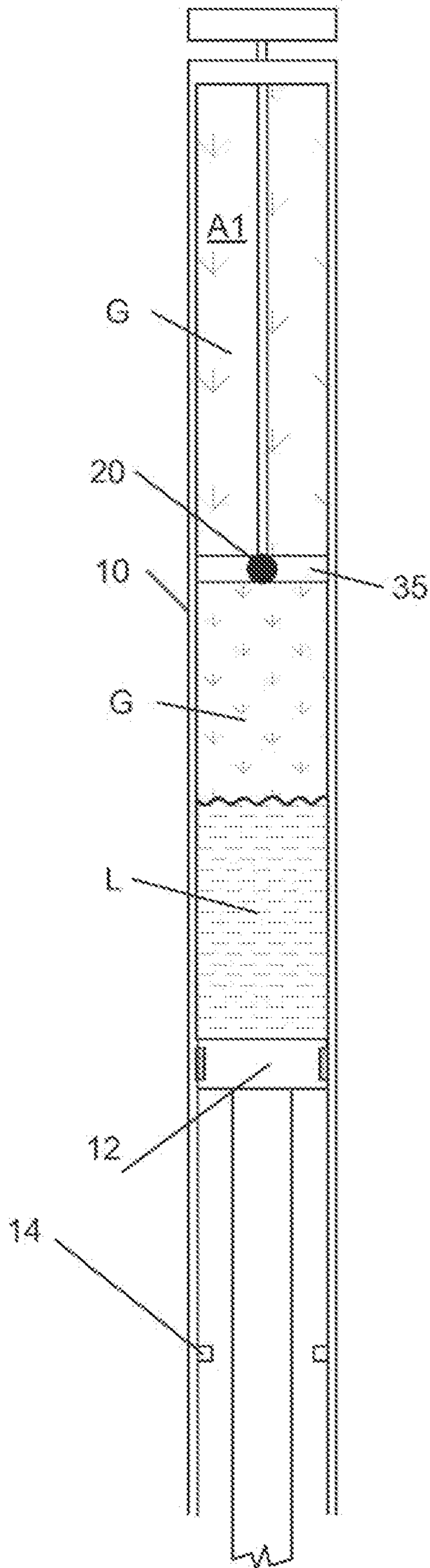
FIG 3A (Short Travel)
