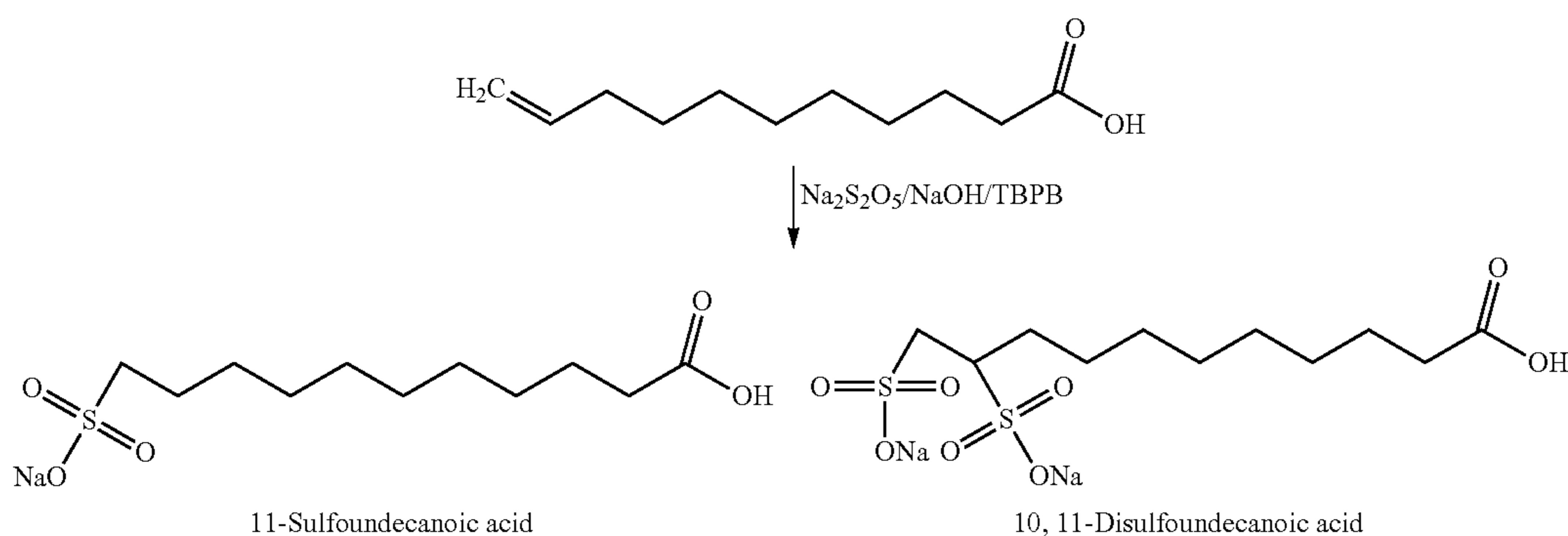
11-Sulfoundecanoic acid
