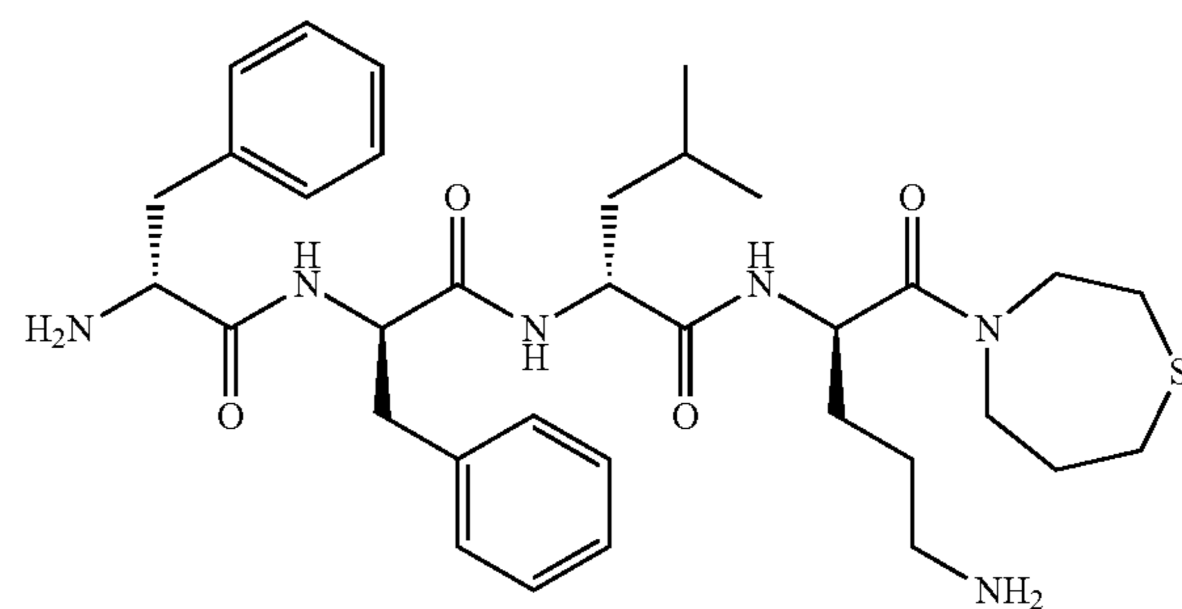
Compound (56) D-Phe-D-Phe-D-Leu-D-Orn-N(homothiomorpholine) (SEQ ID NO: 1):
