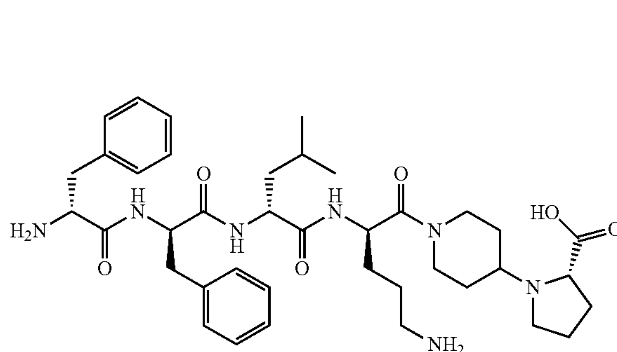
Compound (7) D-Phe-D-Phe-D-Leu-D-Orn-[omega(D/L-2-amino-3-(4-N-piperidiny)propionic acid)]-OH (SEQ ID NO: 1)
