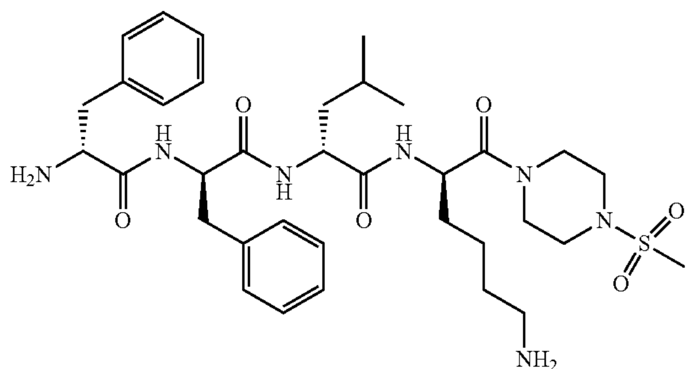
Compound (32): D-Phe-D-Phe-D-Leu-D-Lys-[1-(phenylsulfonyl)piperazine amide] (SEQ ID NO: 5):
