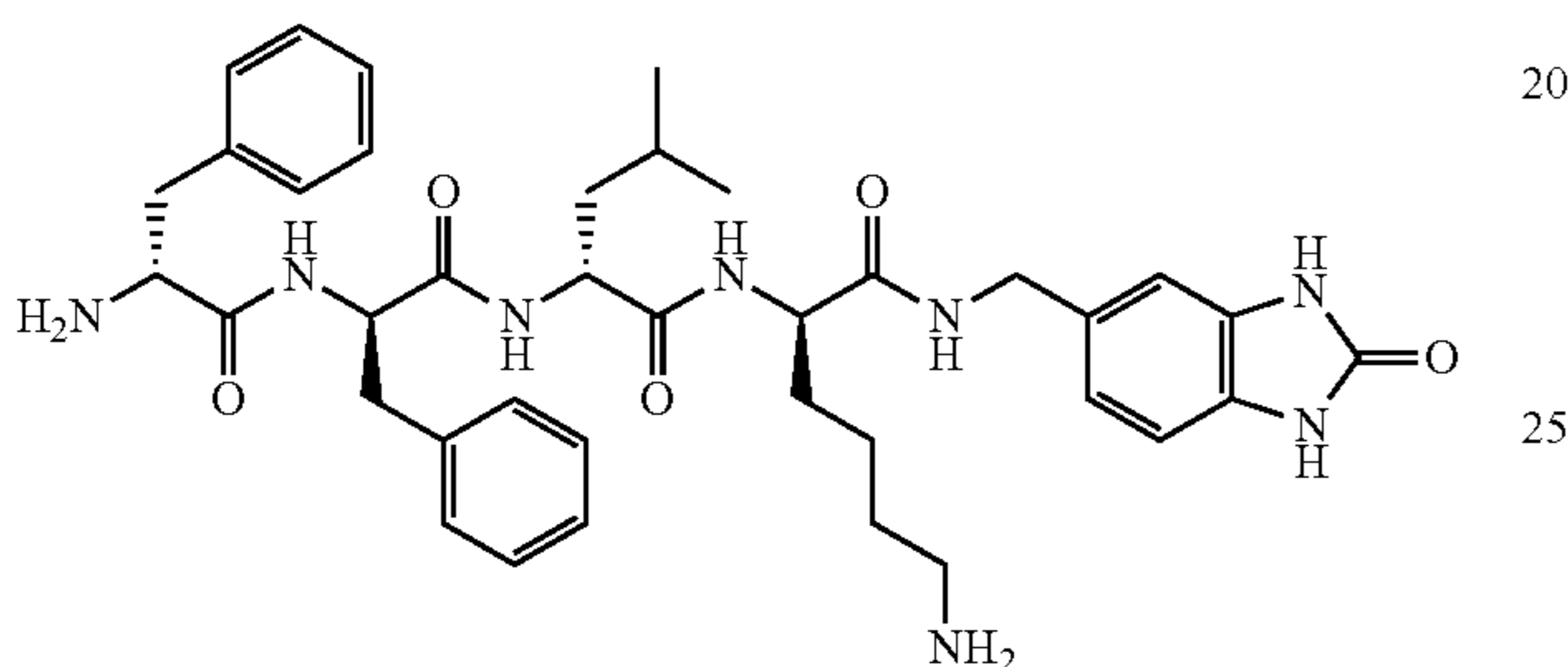
Compound (37): H-D-Phe-D-Phe-D-Leu-D-Lys-[5-(aminomethyl)-1H-benzo[d]imidazol-2(3H)-one amide] (SEQ ID NO: 5):
