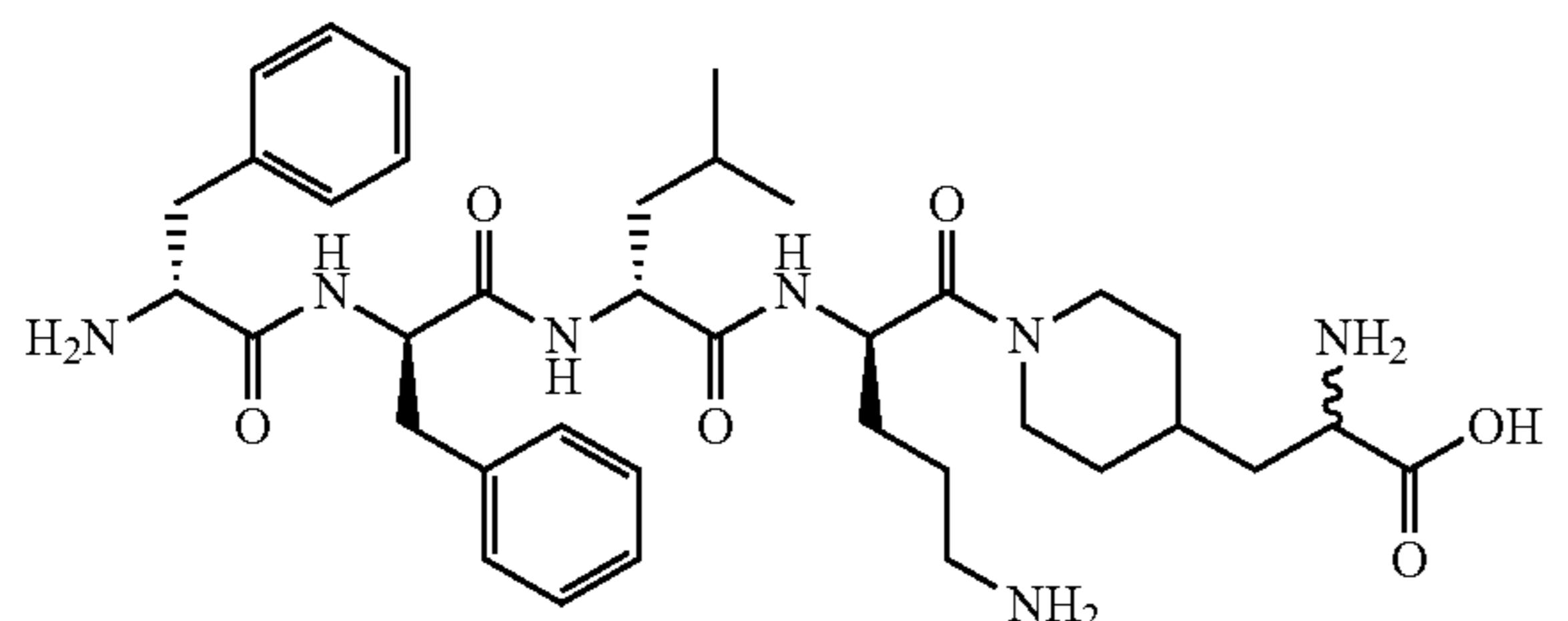
Compound (11) D-Phe-D-Phe-D-Leu-D-Orn-[homopiperazine amide] (SEQ ID NO: 1):
