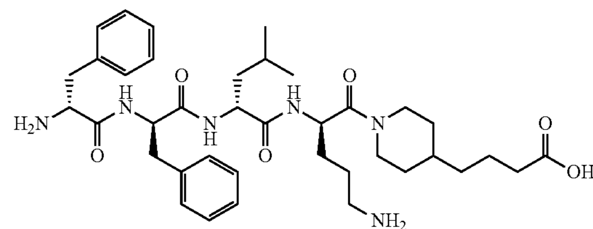
Compound (12) D-Phe-D-Phe-D-Leu-D-Orn-[4-(4-piperidiny)-butanoic acid]-OH (SEQ ID NO: 1):
