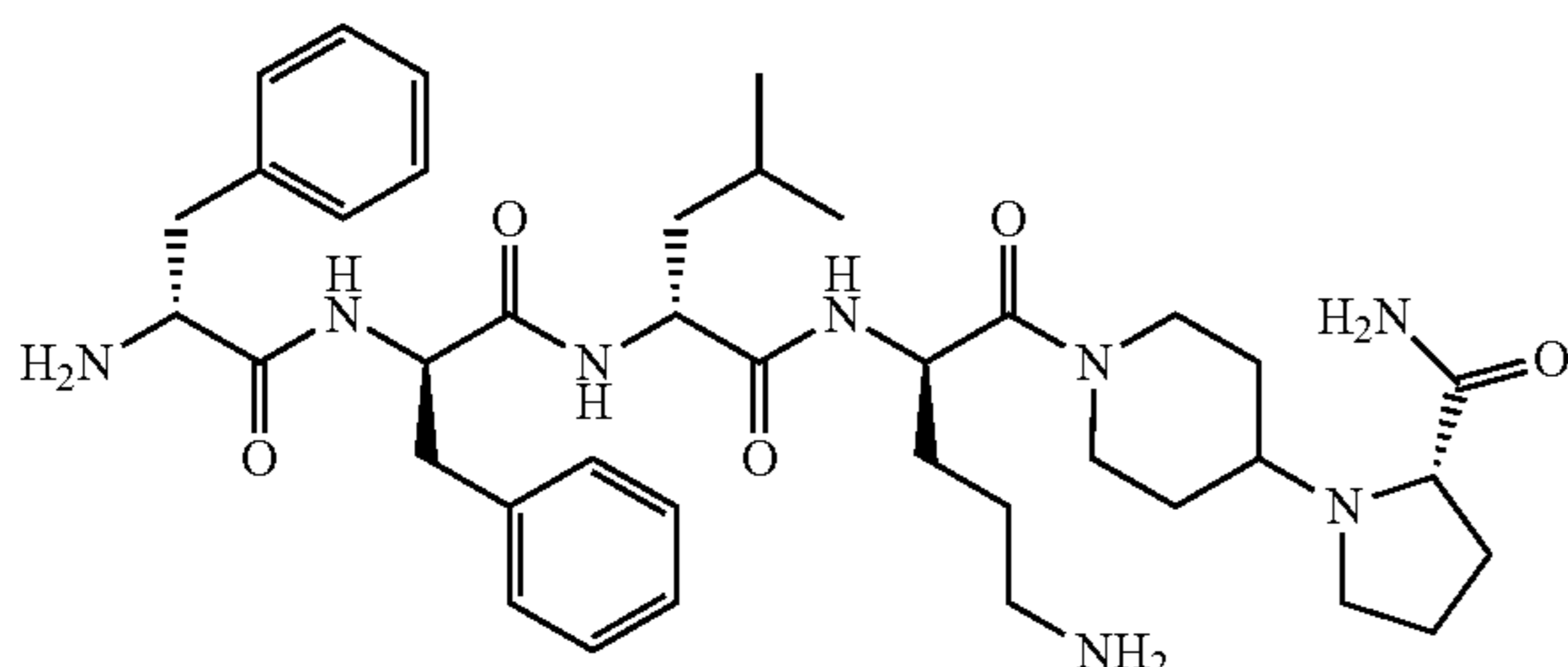
Compound (14) D-Phe-D-Phe-D-Leu-D-Orn-[N-(4-piperidiny)-L-proline]-NH 2 (SEQ ID NO: 1):
