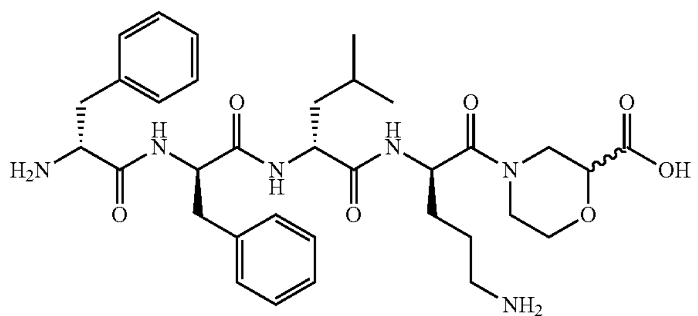
Compound (54) D-Phe-D-Phe-D-Leu-D-Orn-[R/S-2-carboxythiomorpholine]-OH (SEQ ID NO: 1):
