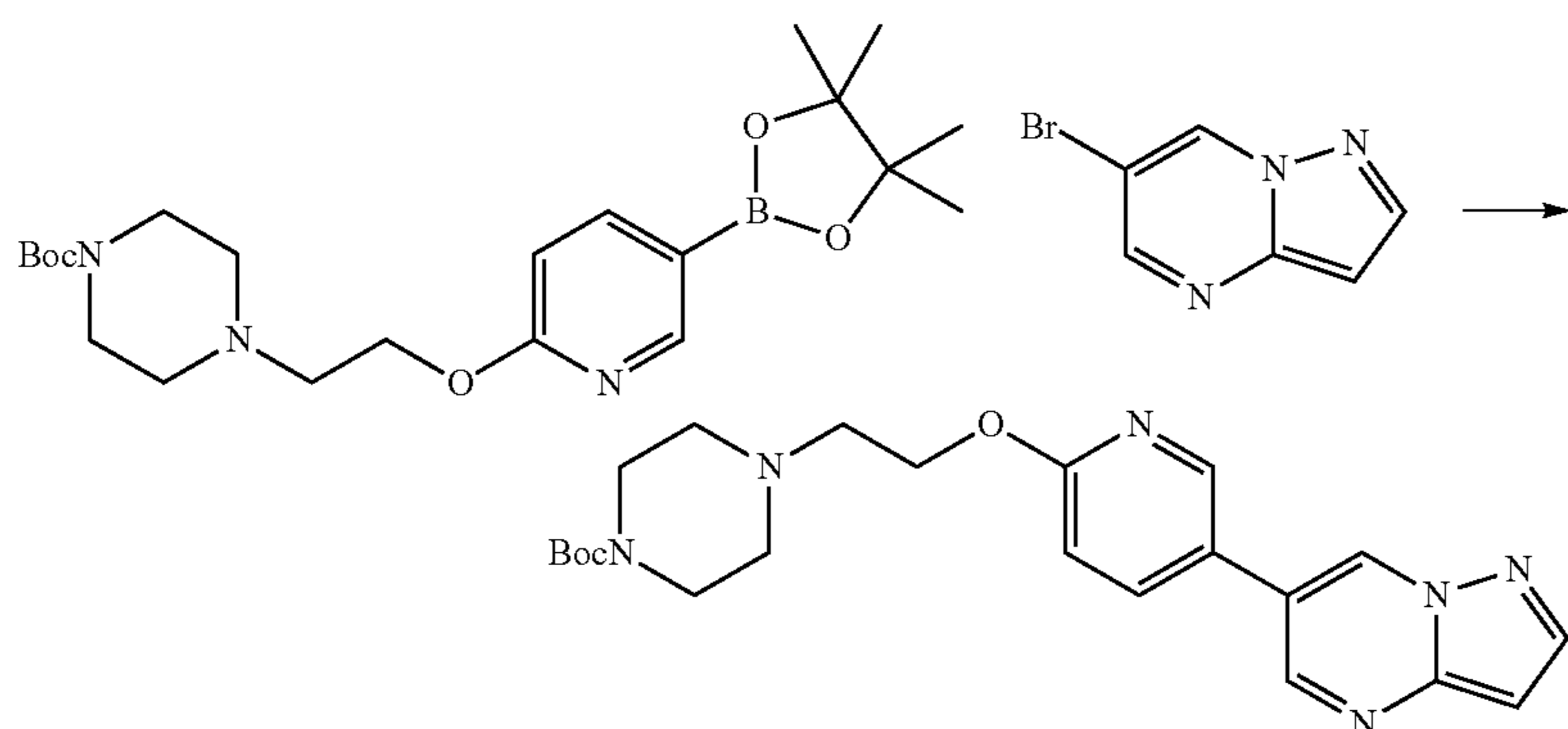
Scheme 151
