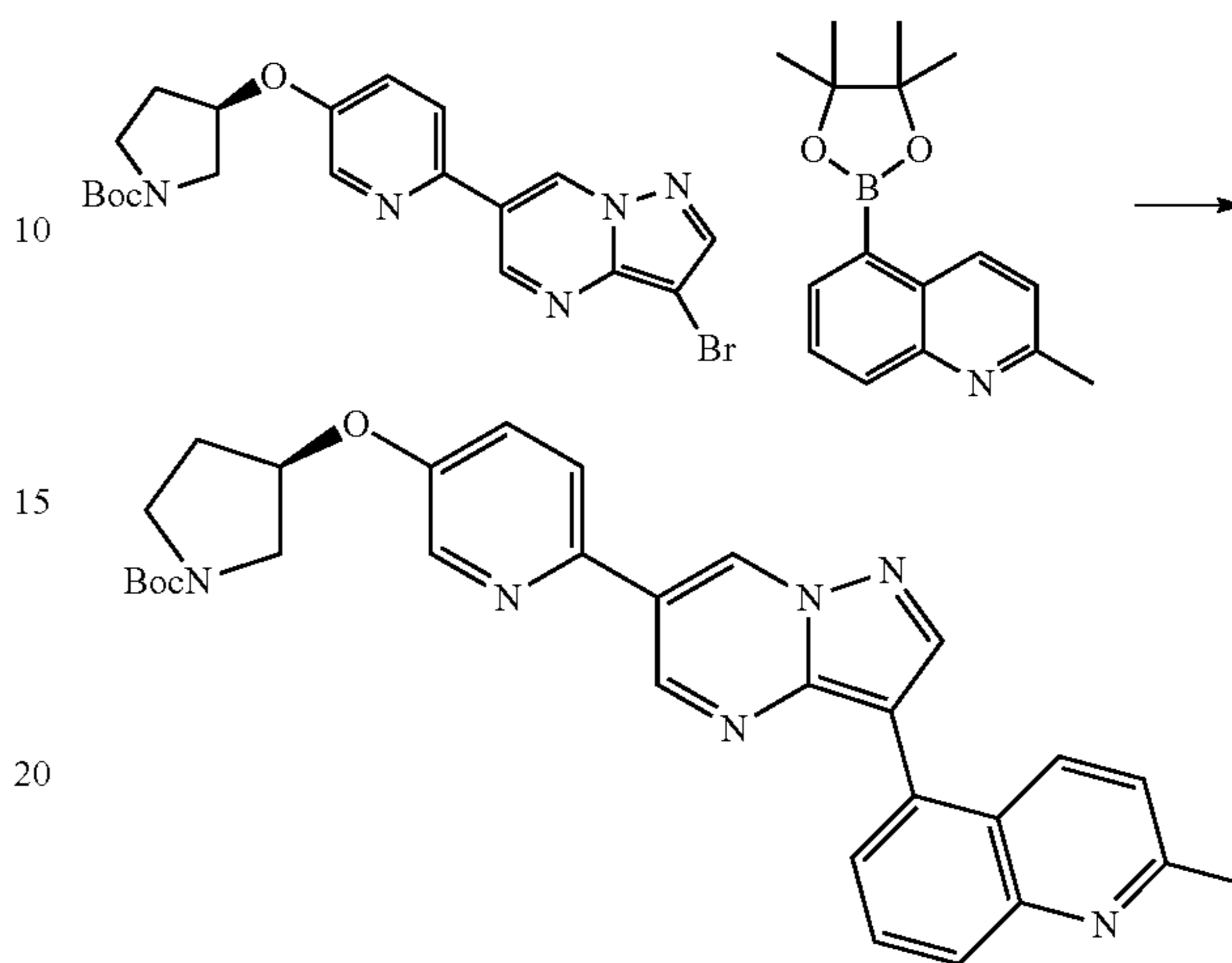
Scheme 208
