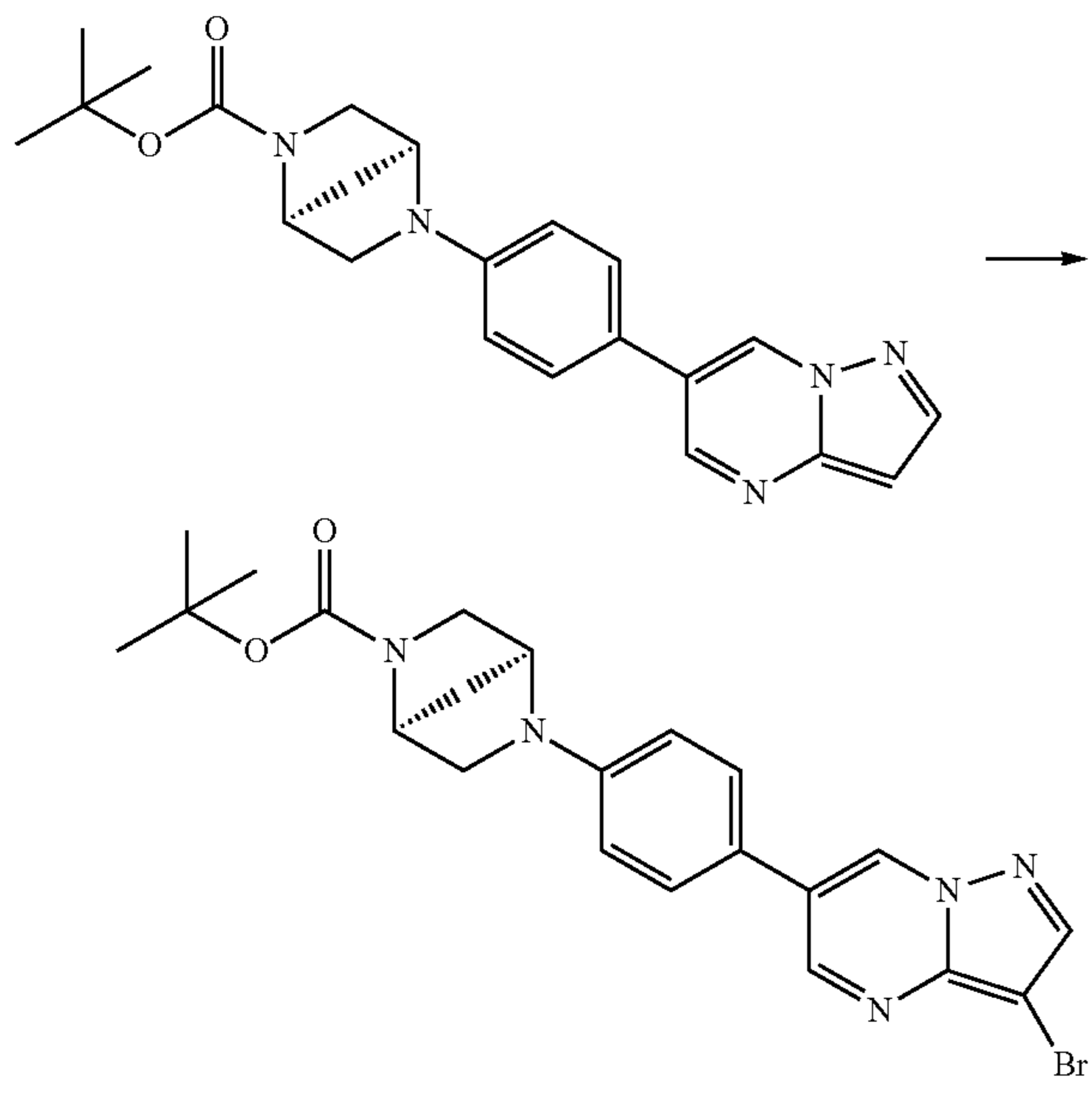
Scheme 15
