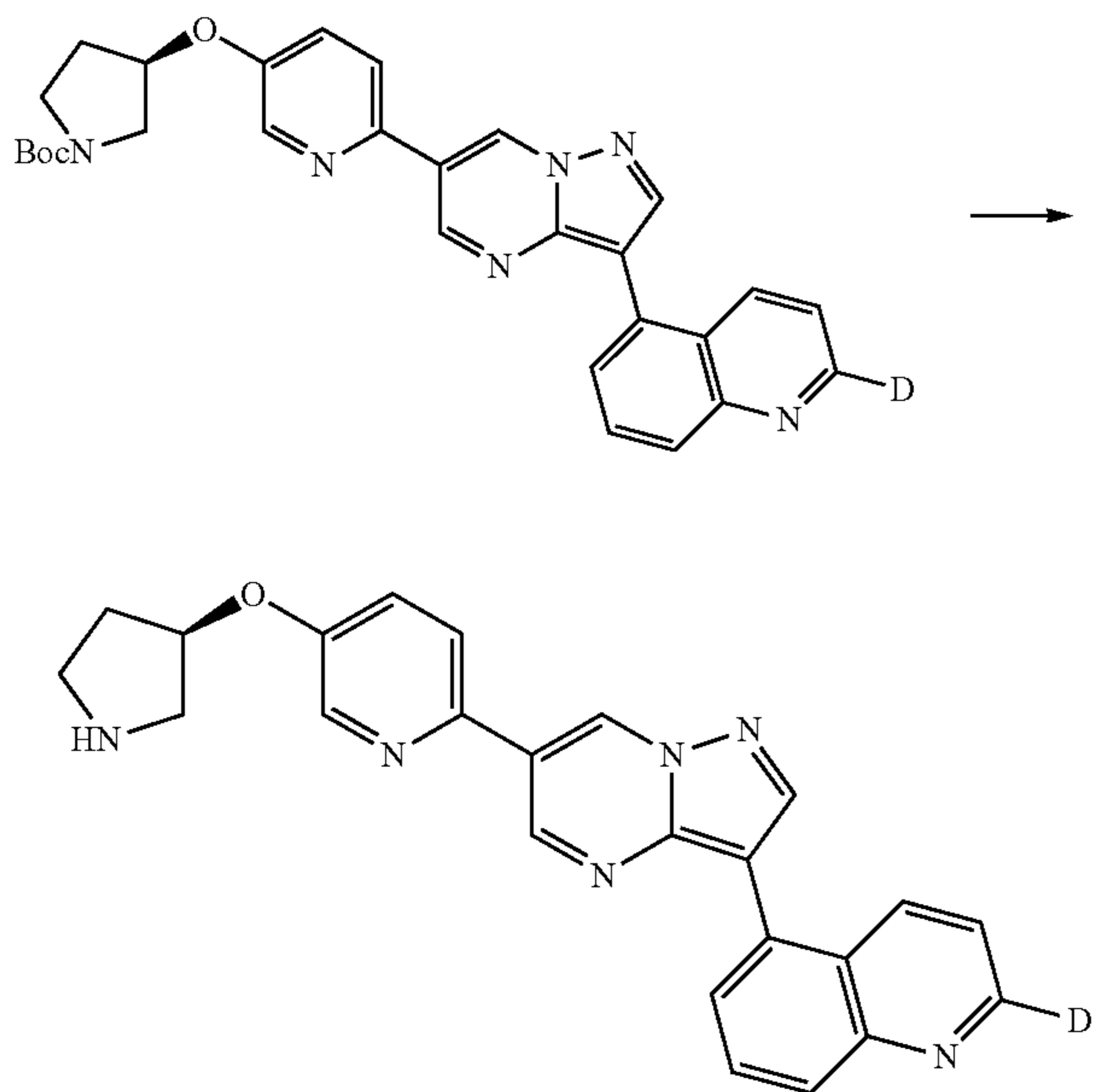
Scheme 207
