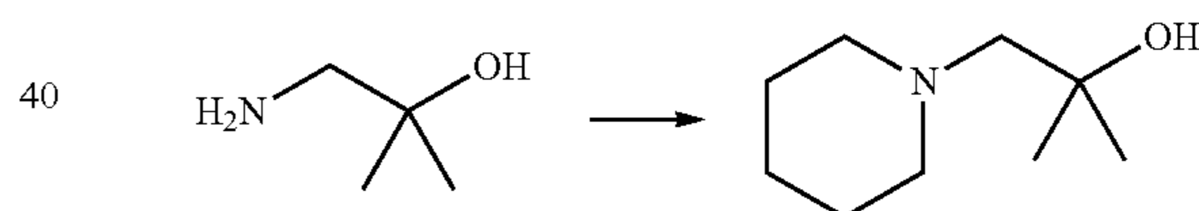
Scheme 105
