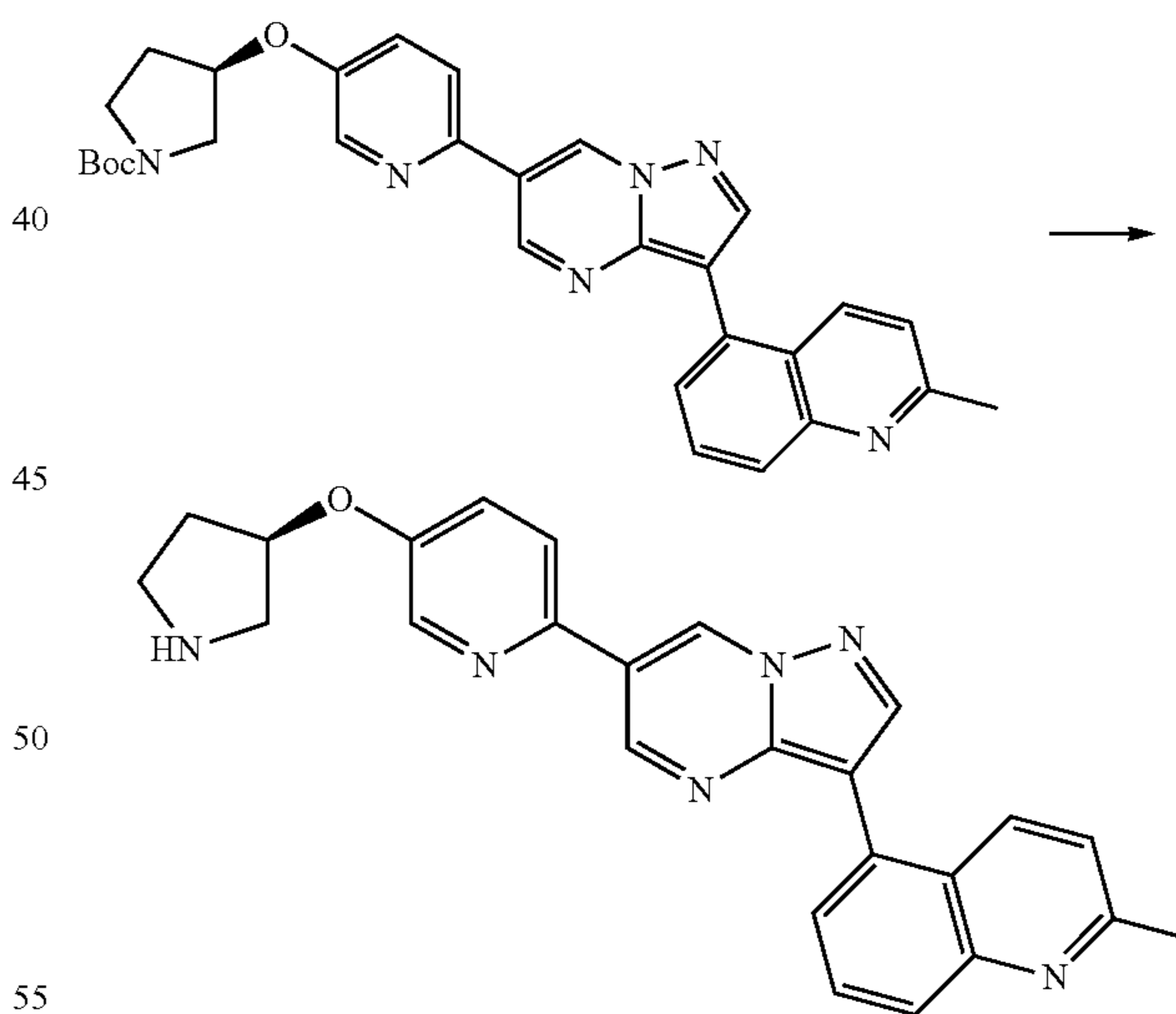
Scheme 209
