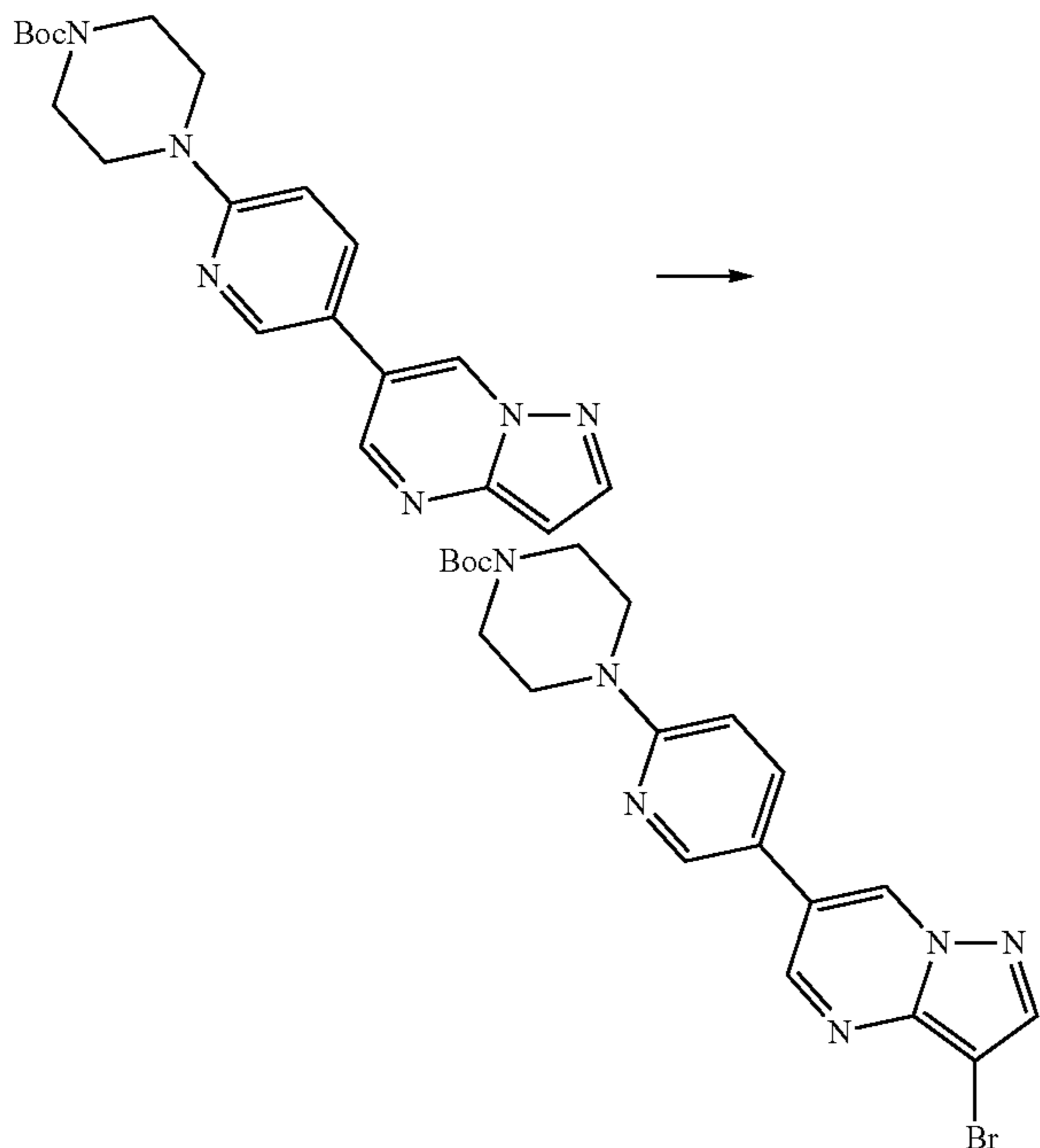
Scheme 38
