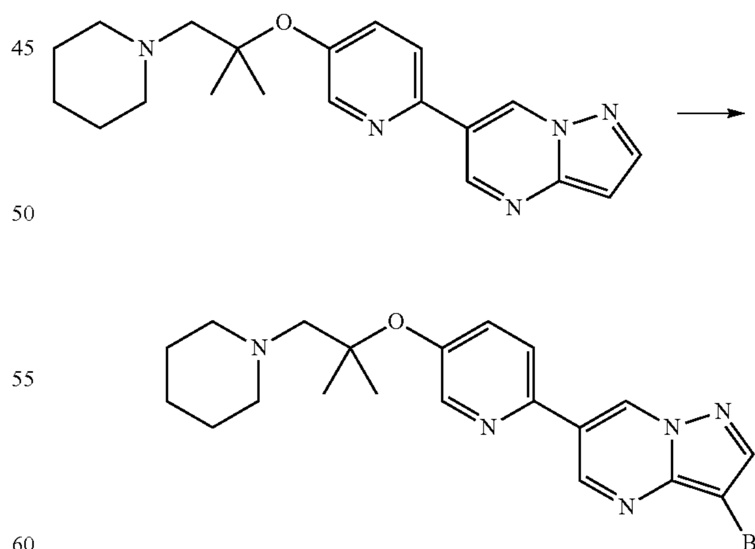
Scheme 191
