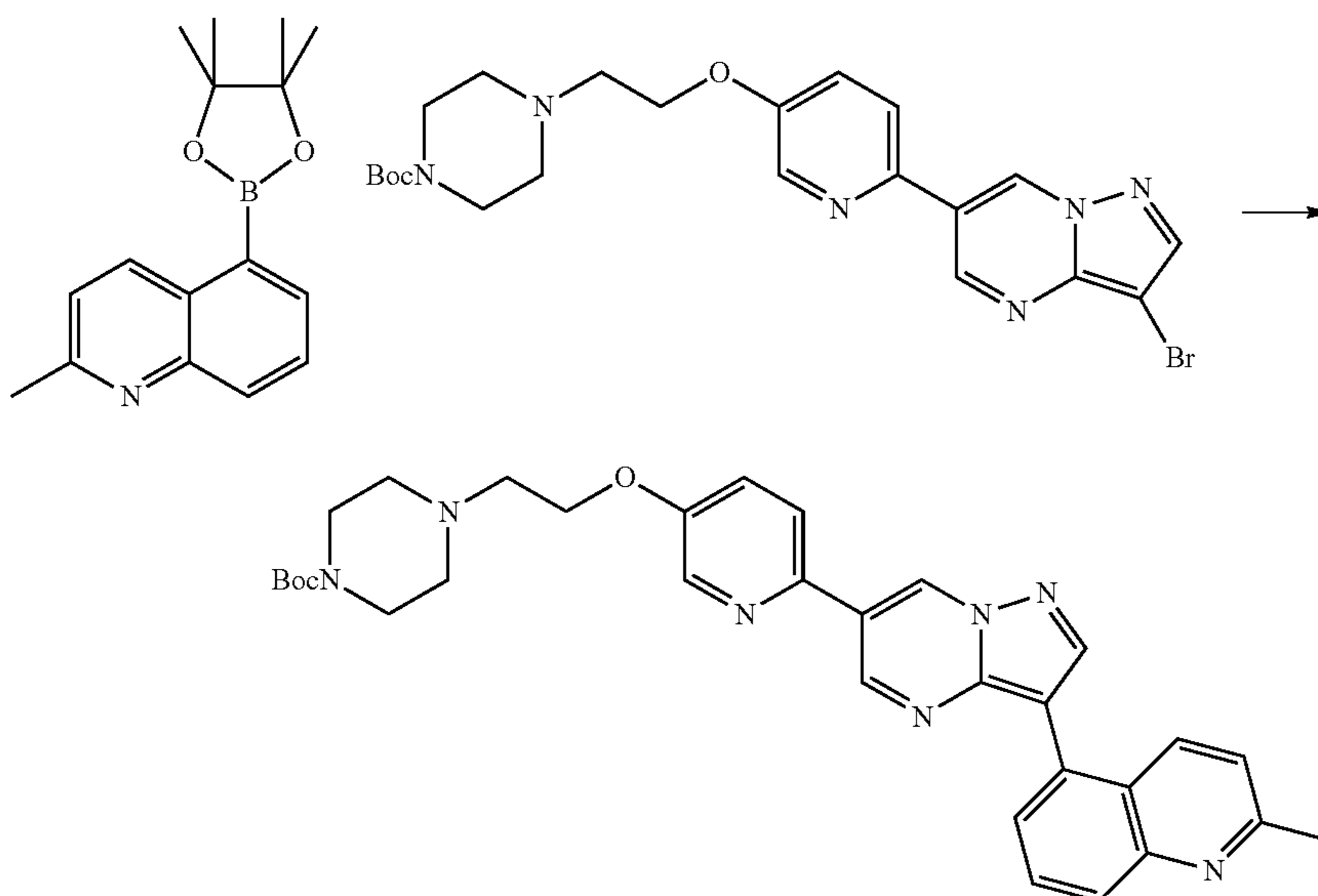
Scheme 177
