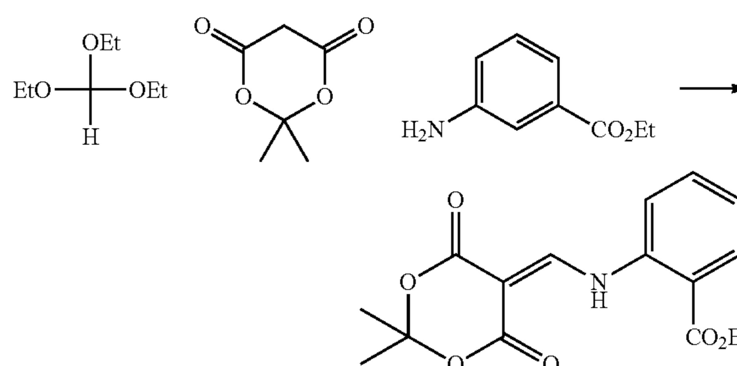
Scheme 68
