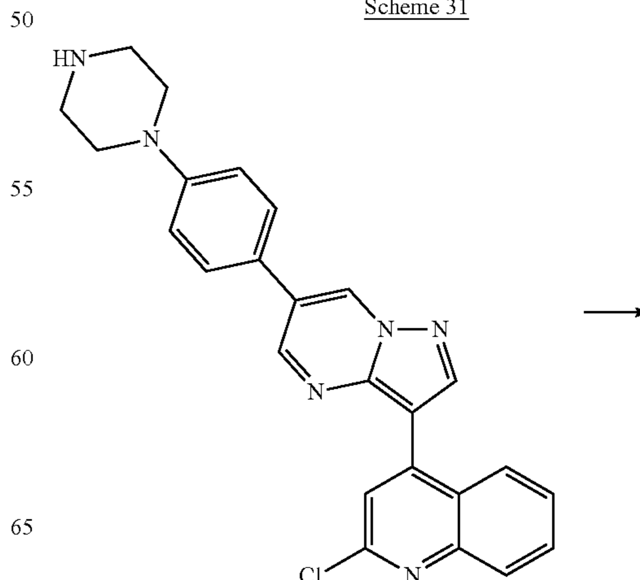
Scheme 31
