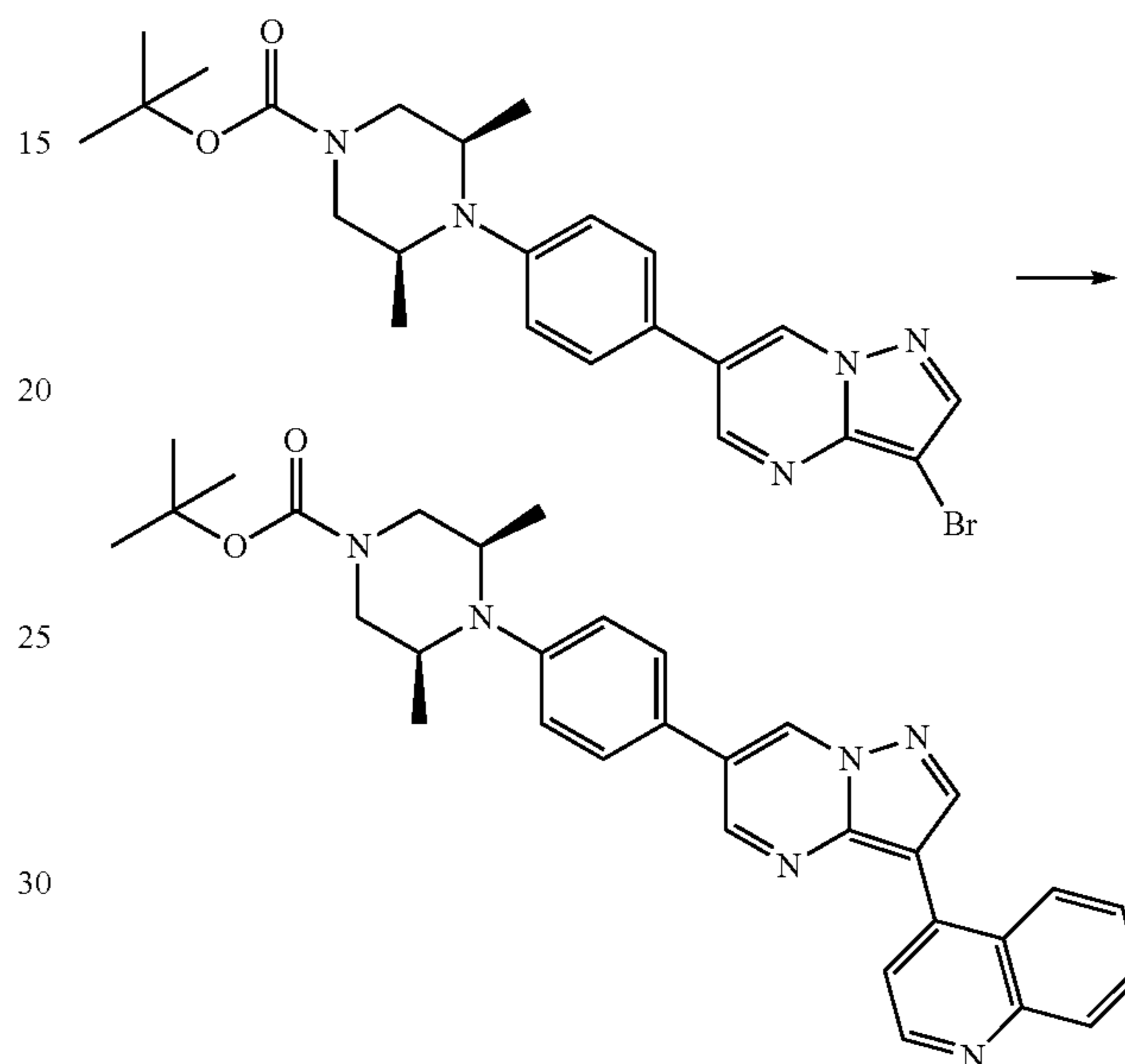
Scheme 5
