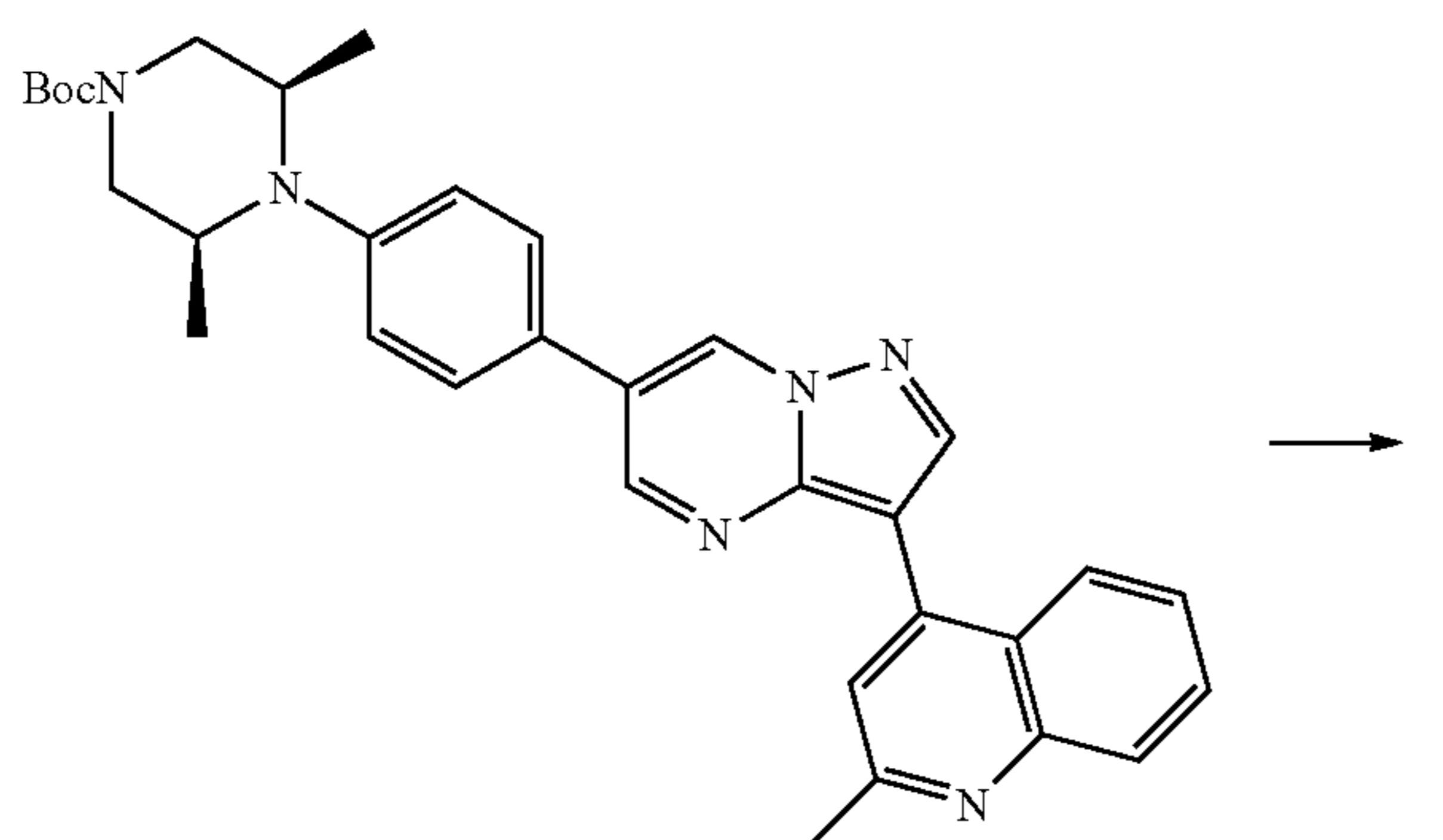
Scheme 36
