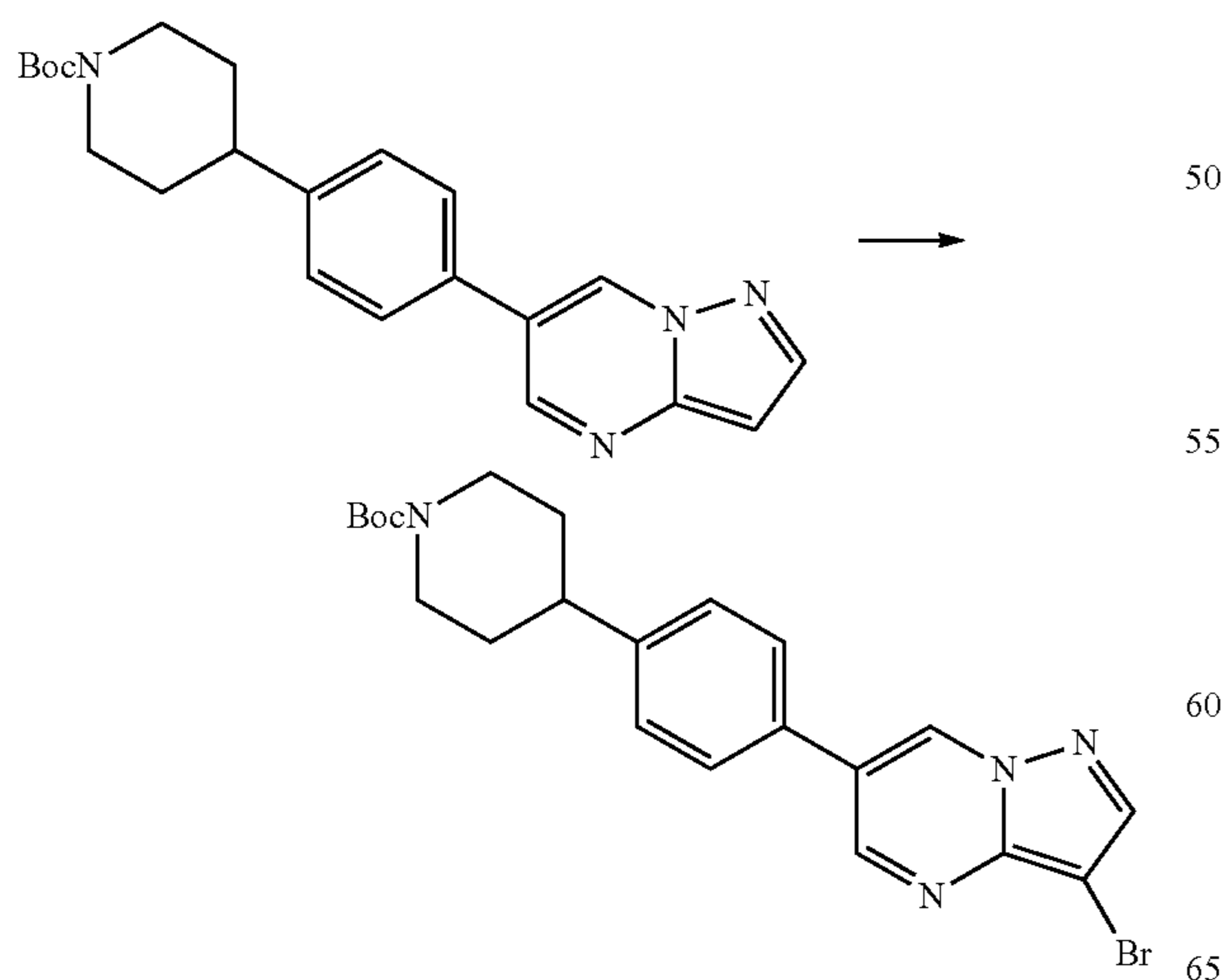
Scheme 43
