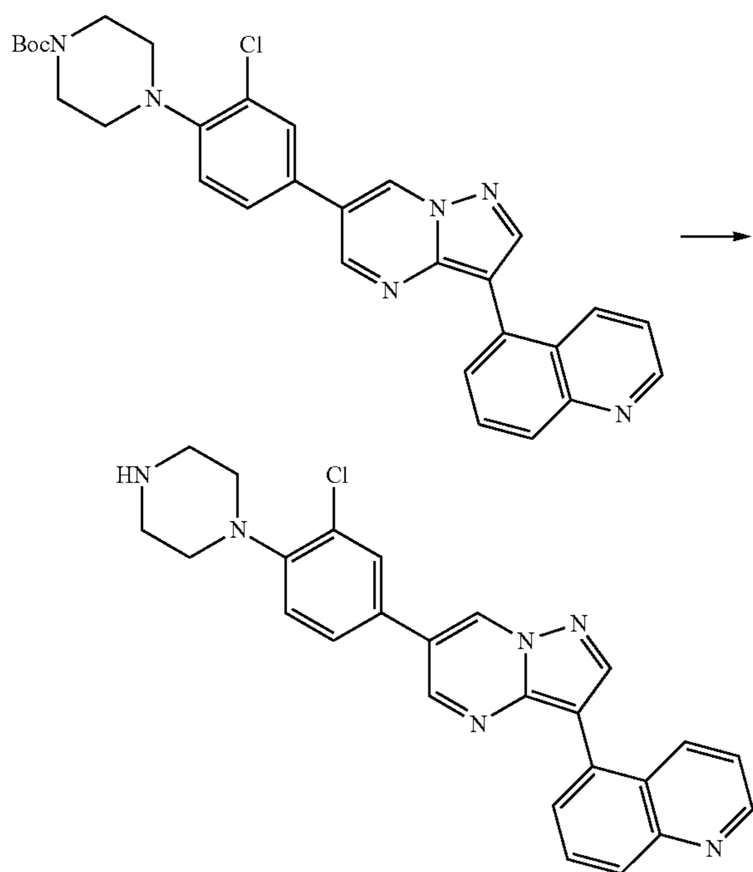
Scheme 130
