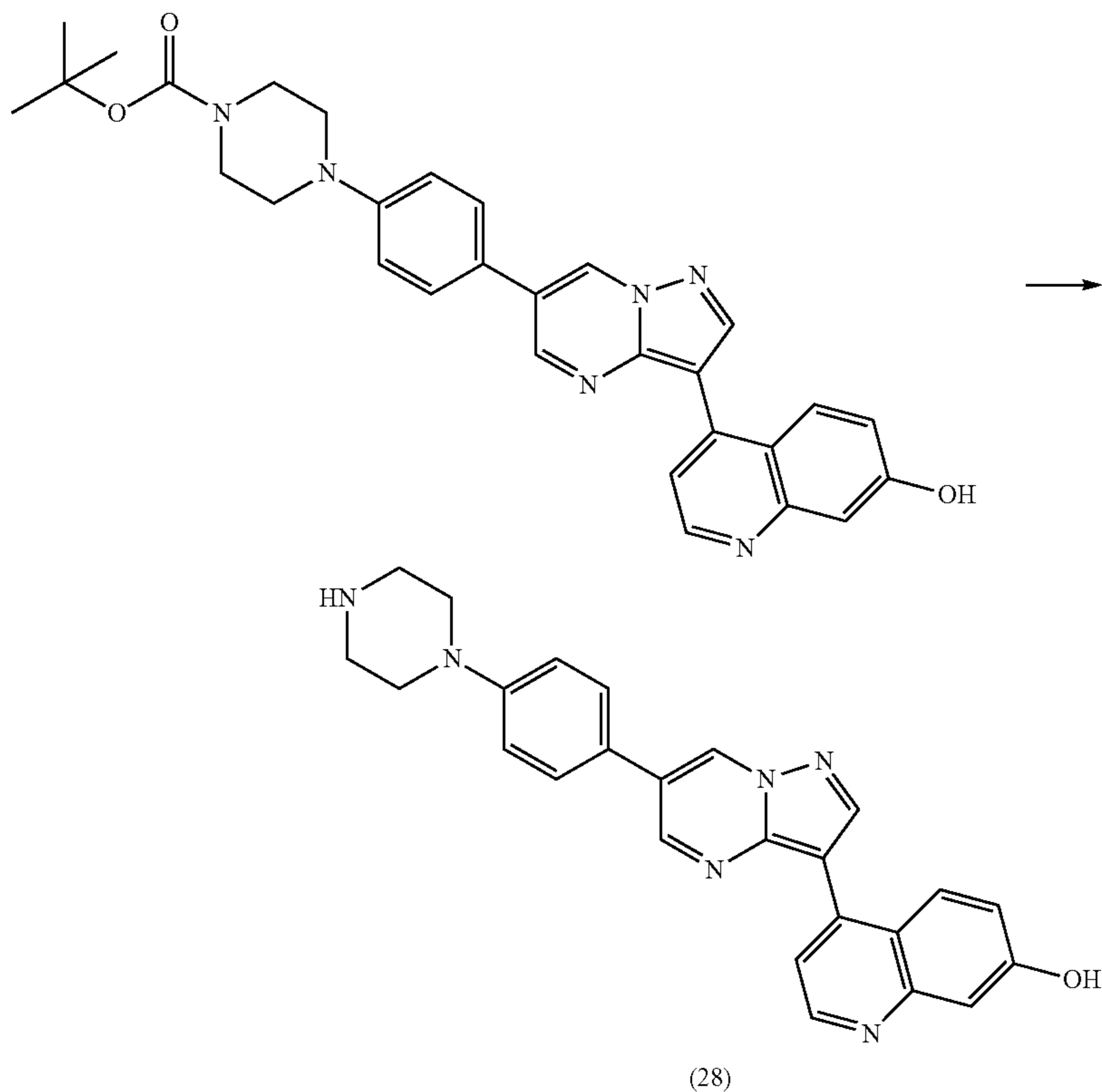
Scheme 95
