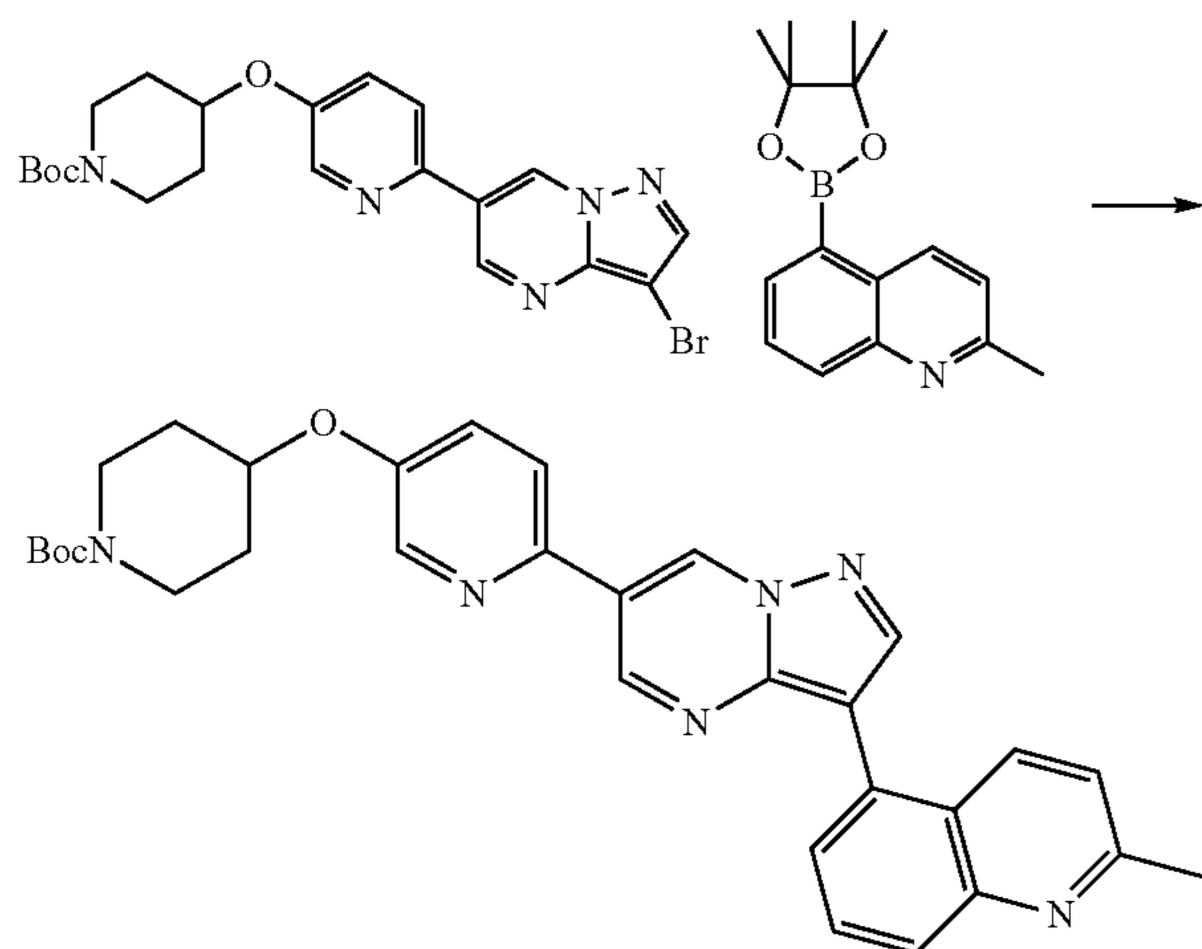
Scheme 202
