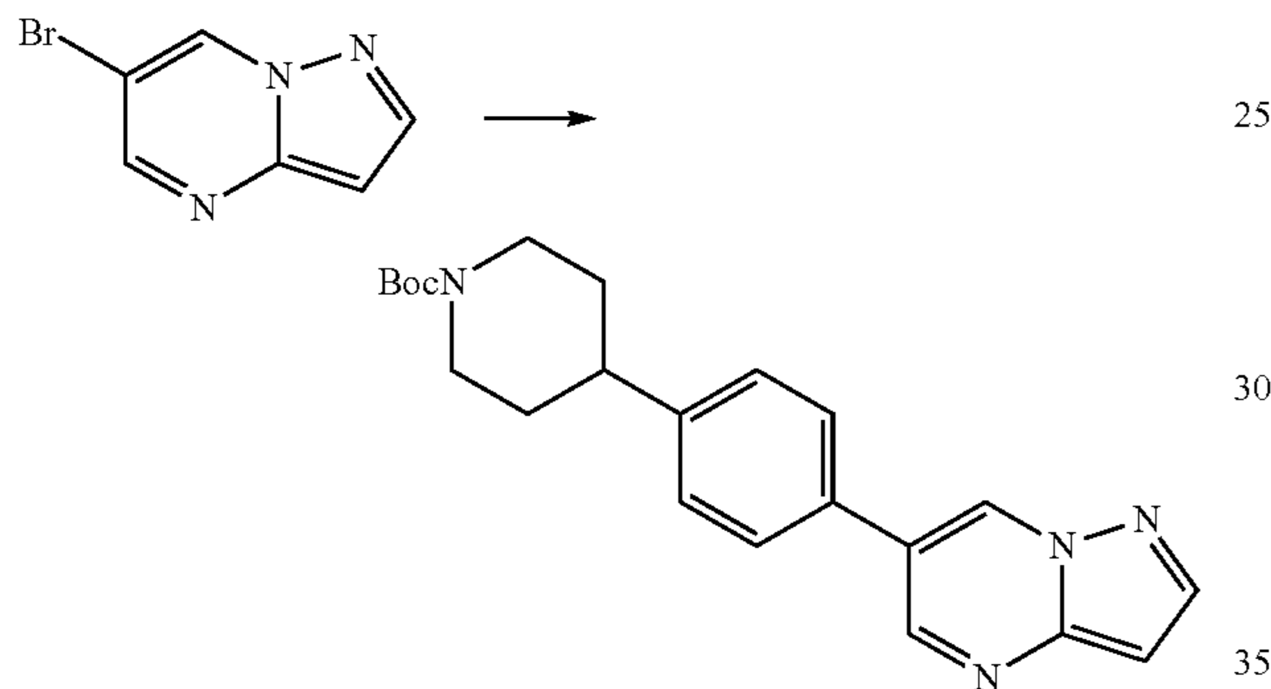
Scheme 42
