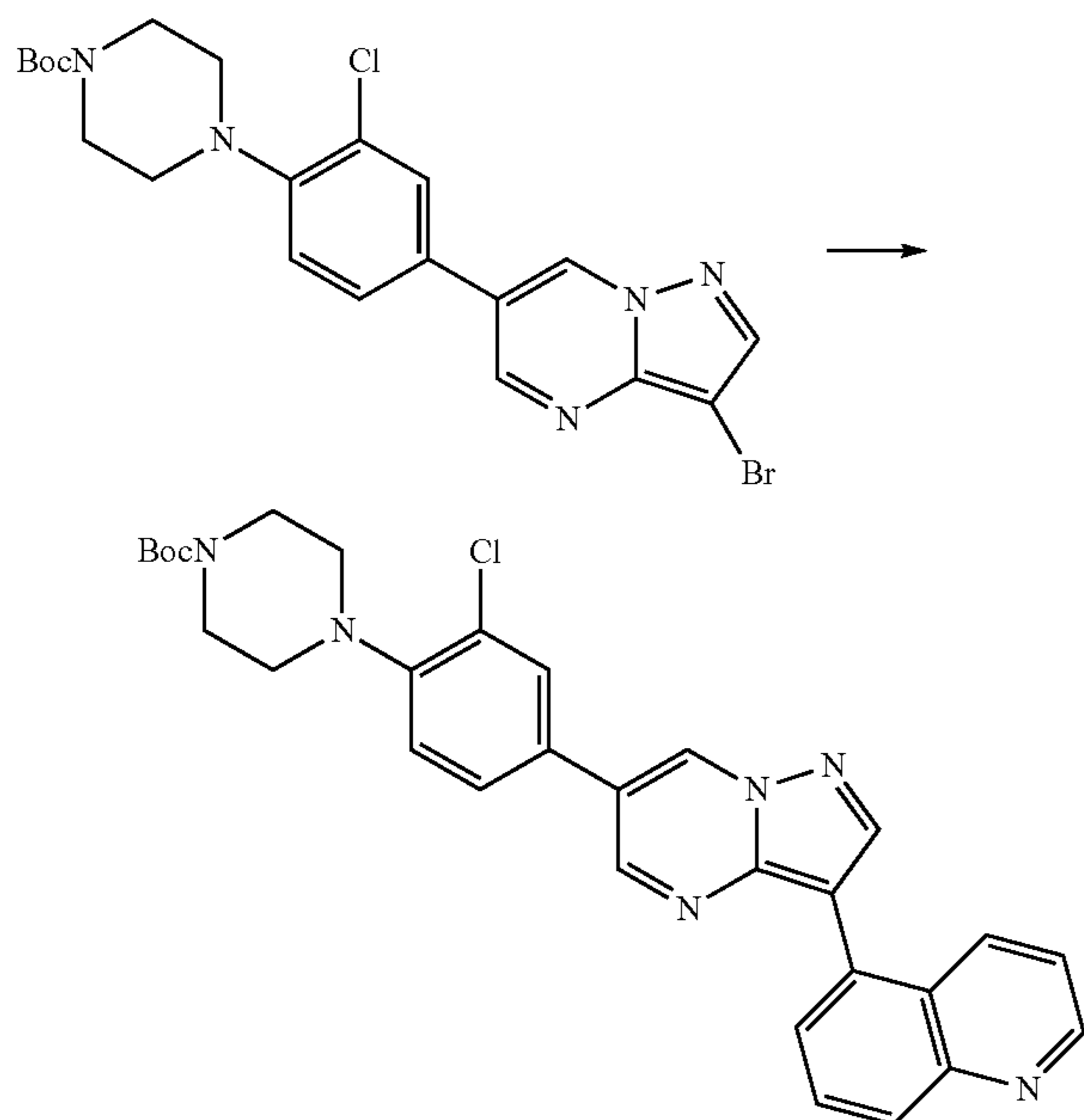
Scheme 129
