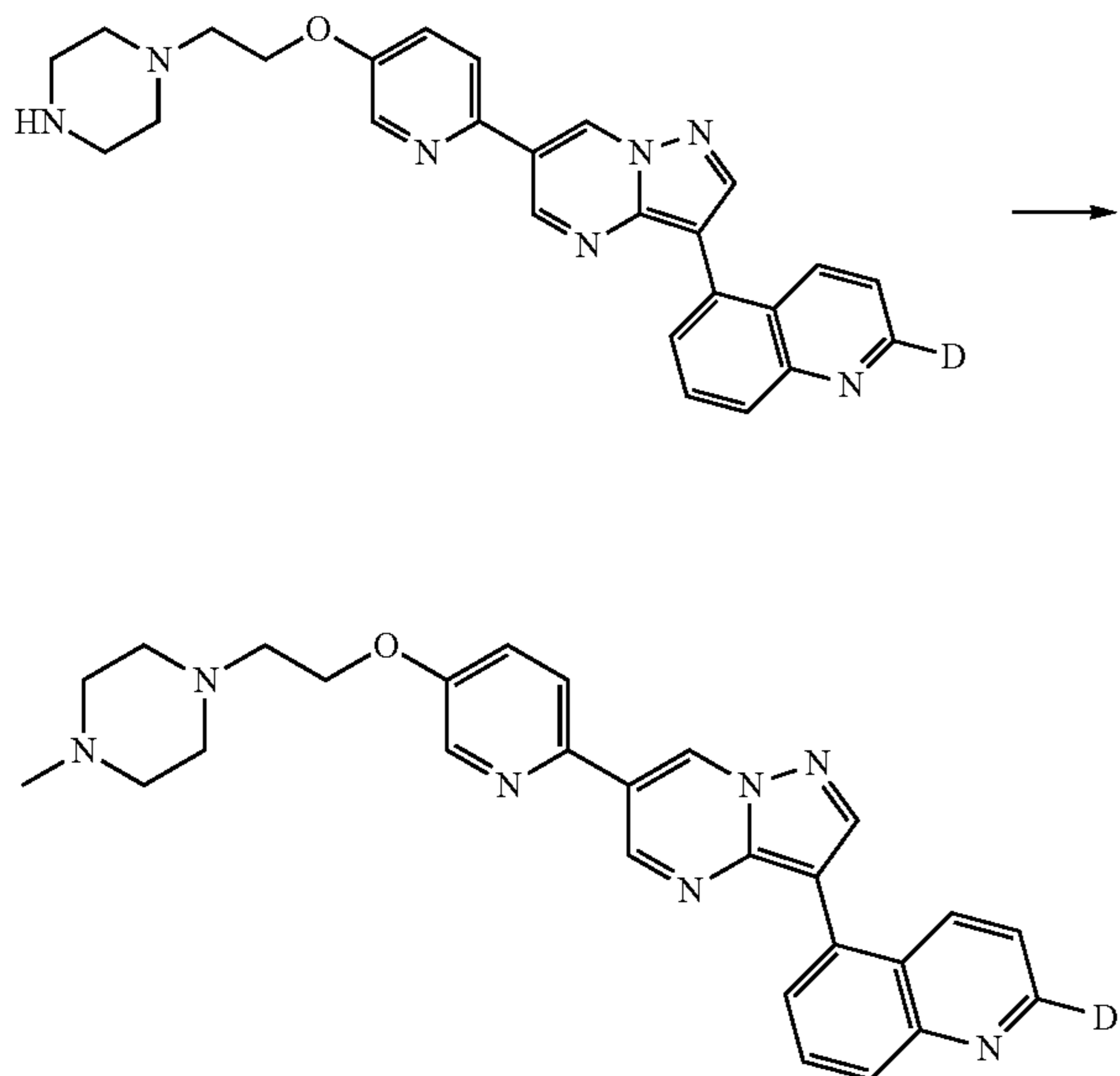
Scheme 179
