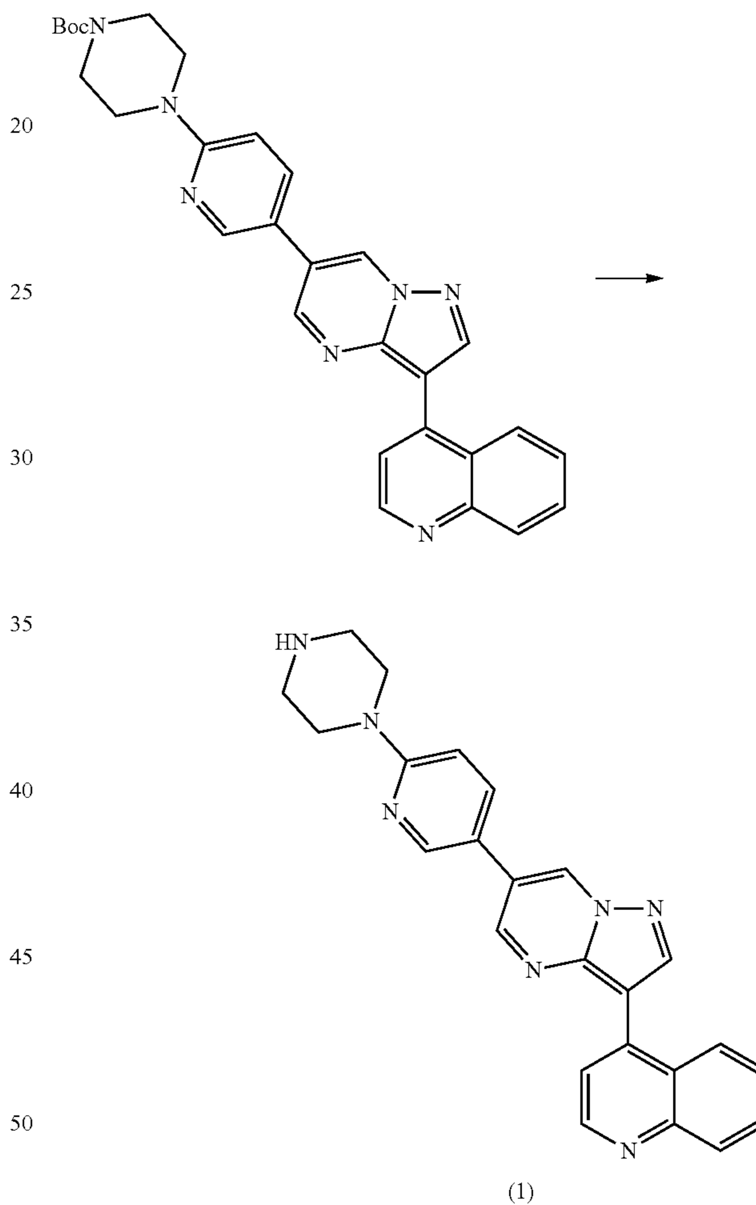
Scheme 2
