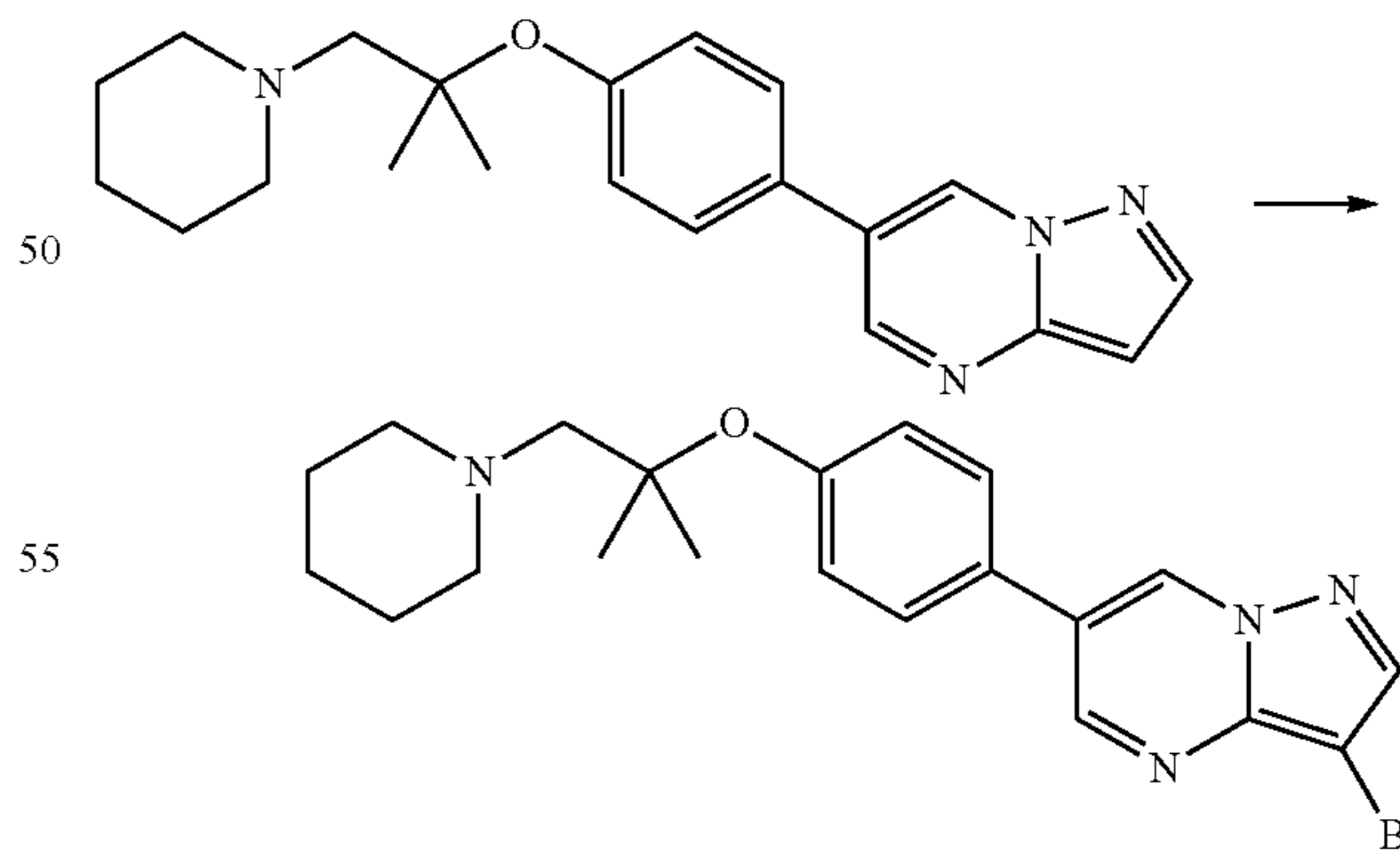
Scheme 111
