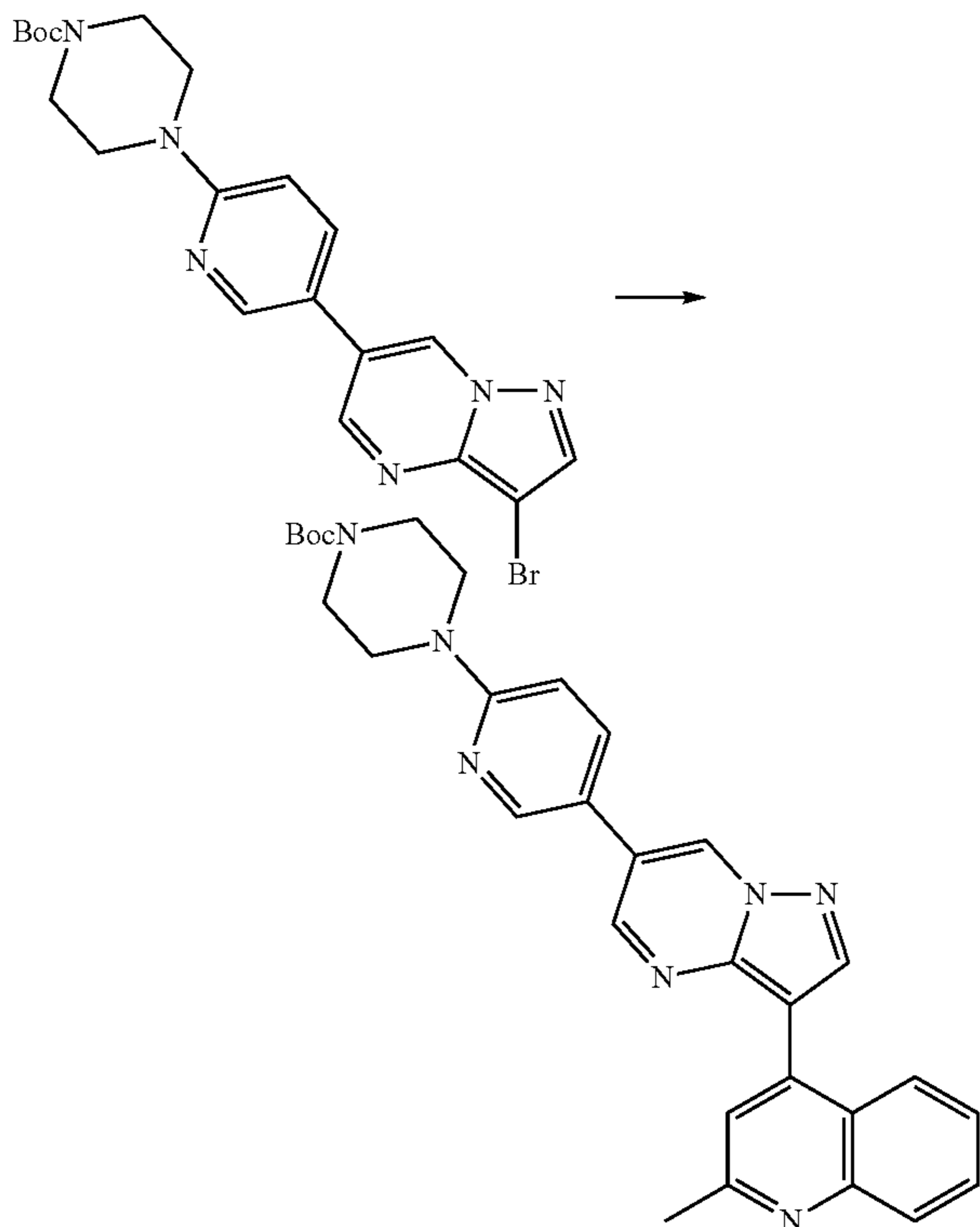
Scheme 39
