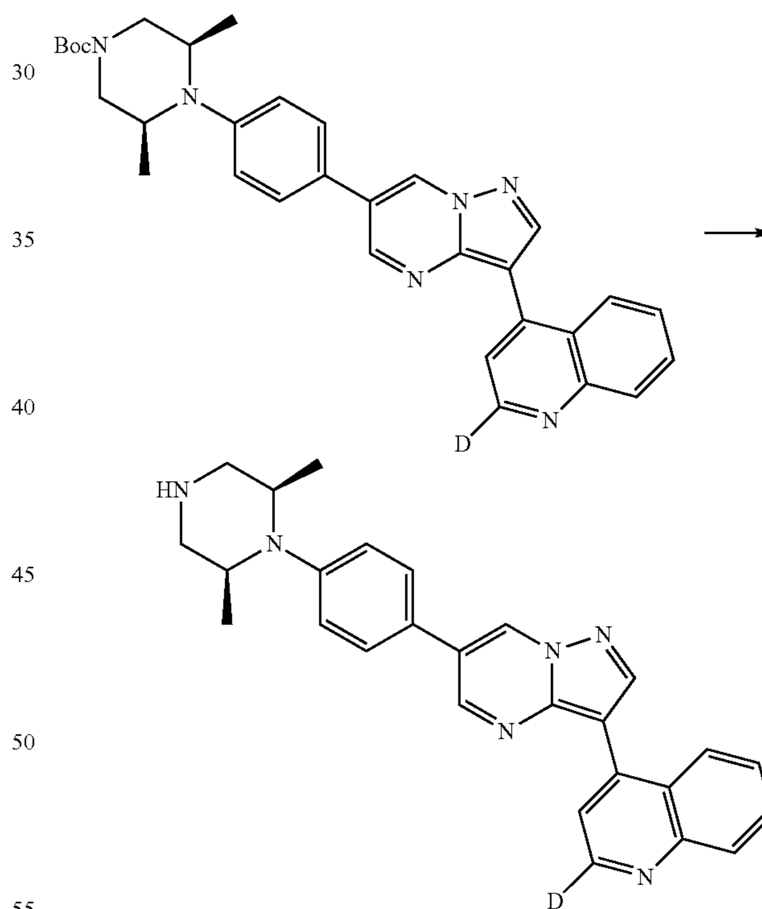
Scheme 181
