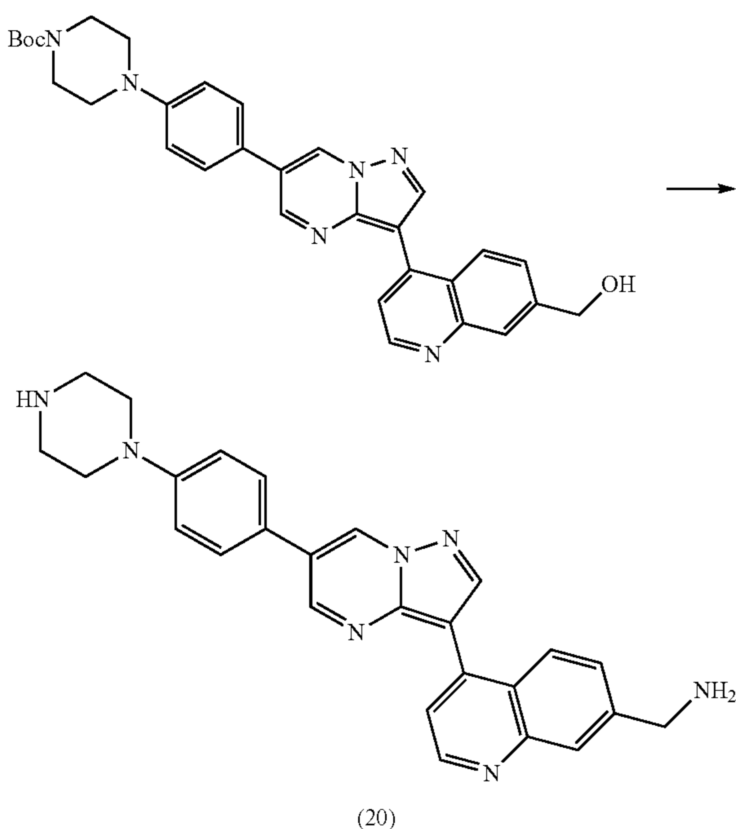
Scheme 66
