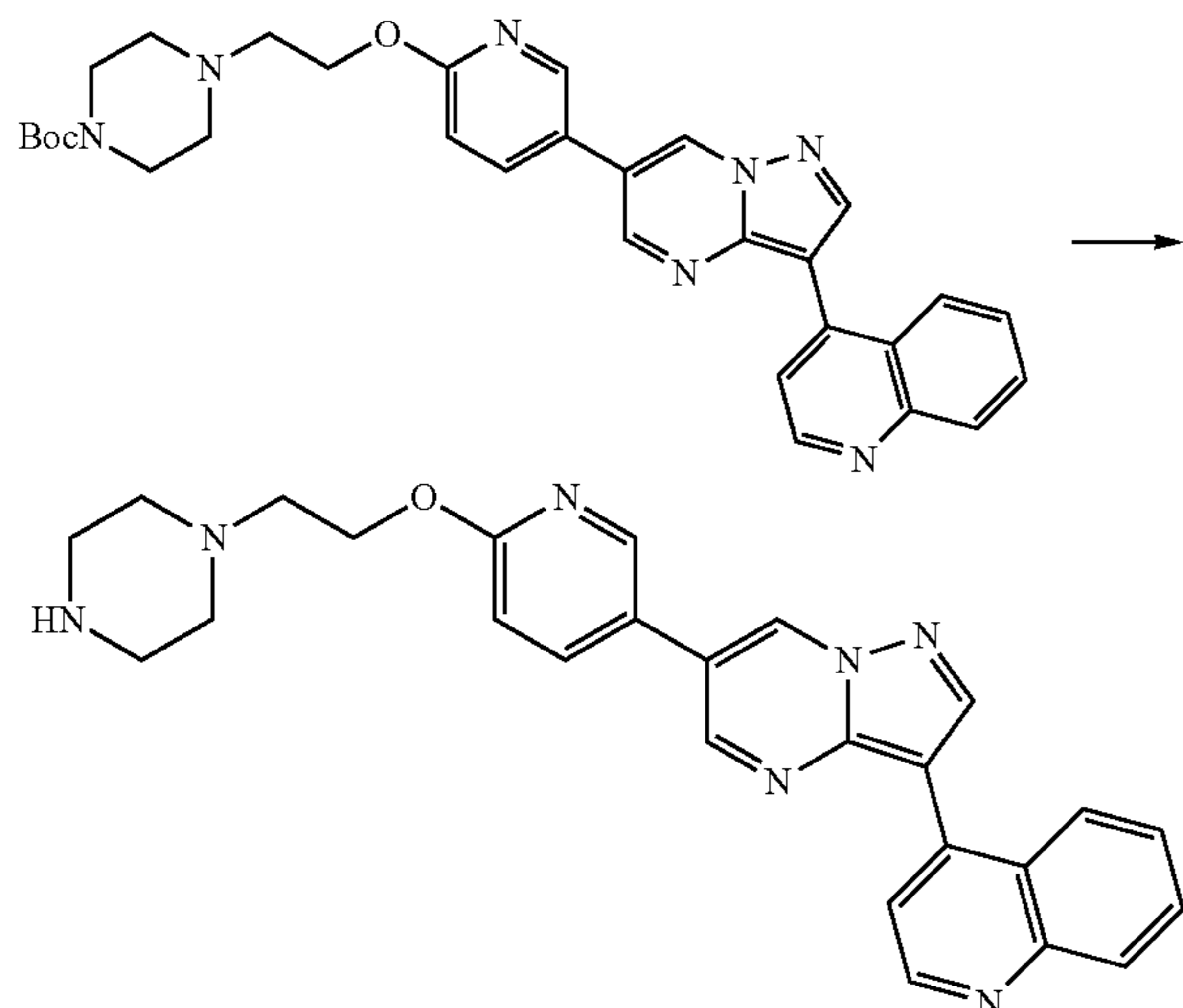
Scheme 154
