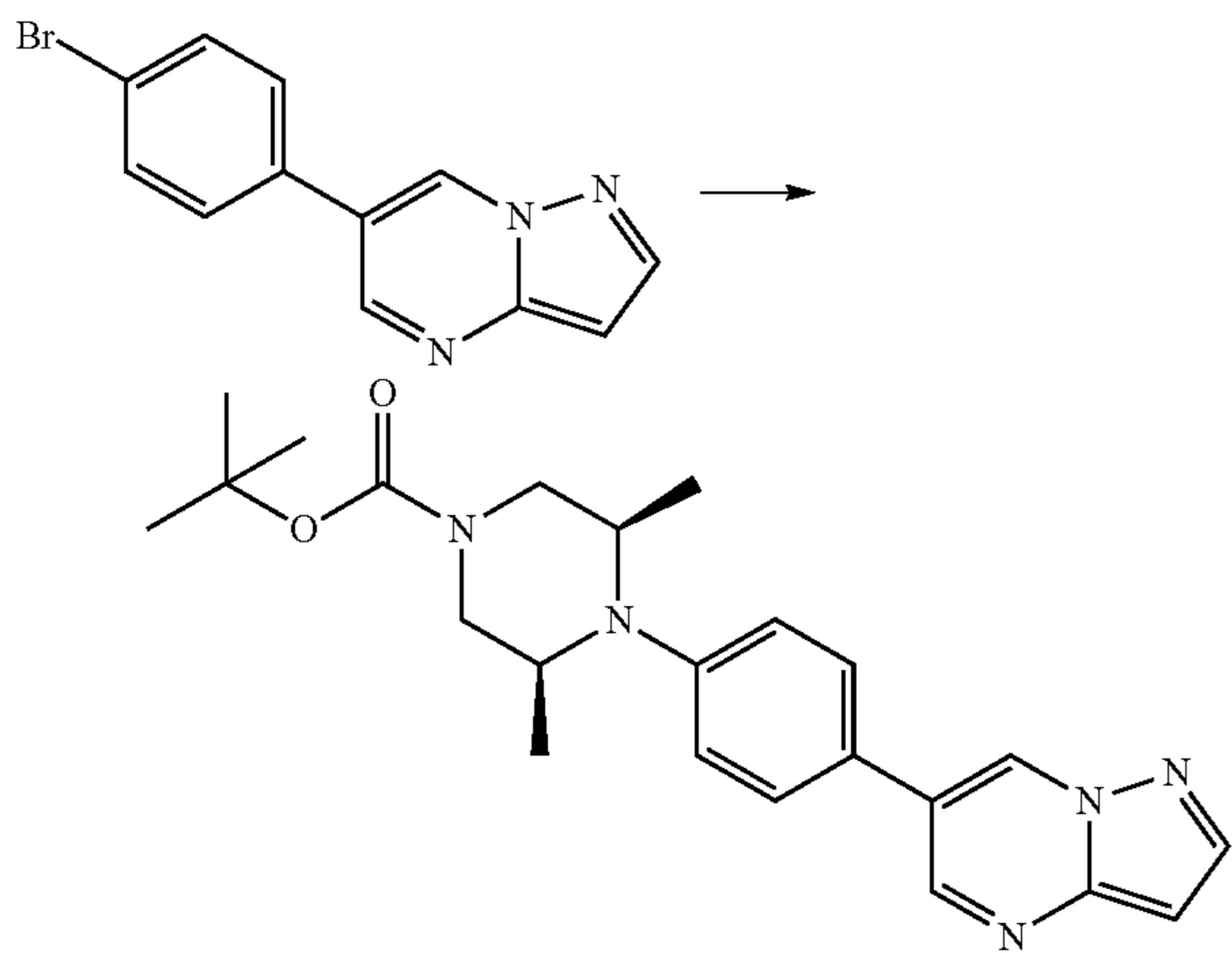
Scheme 3
