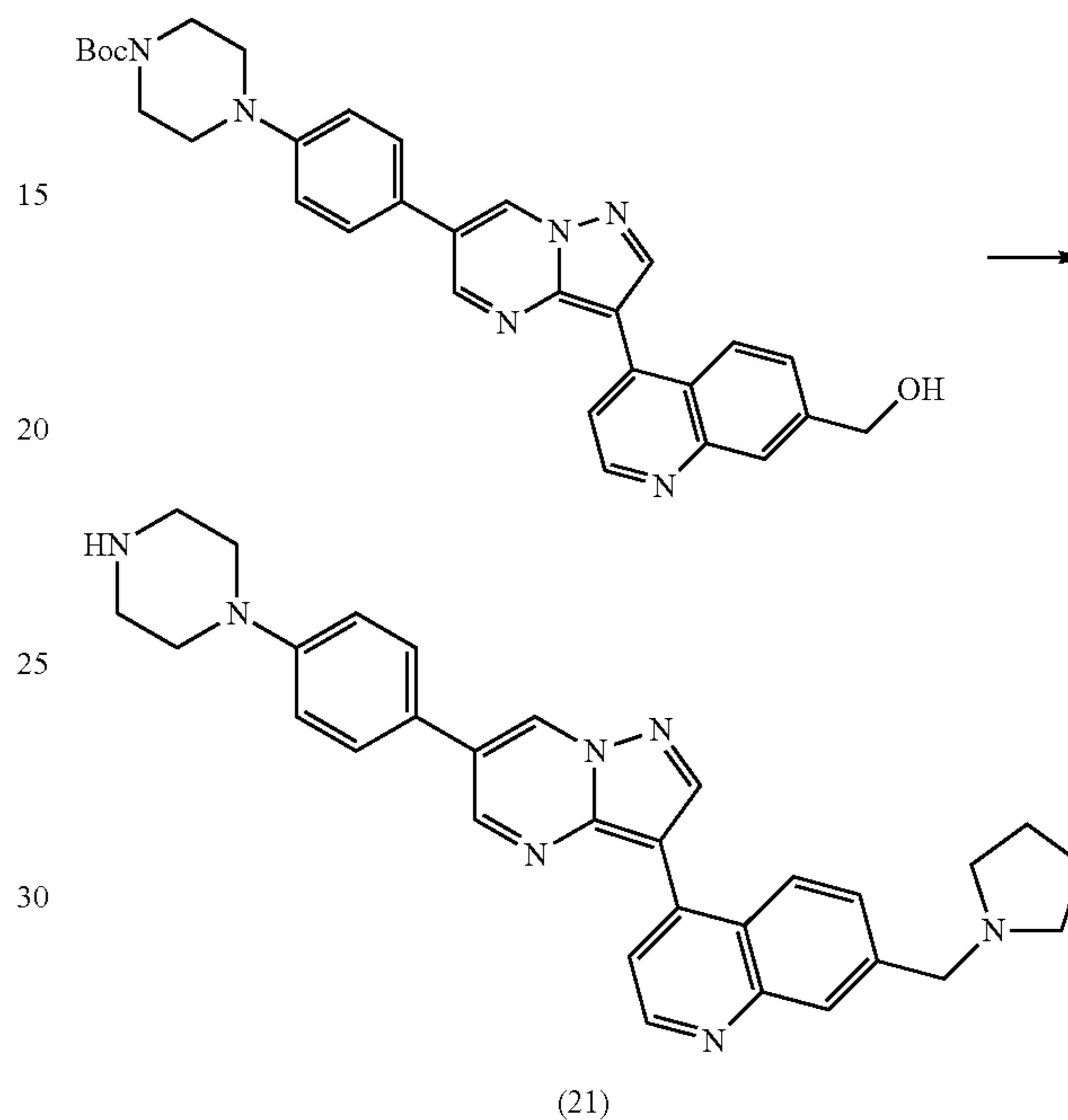
Scheme 67
