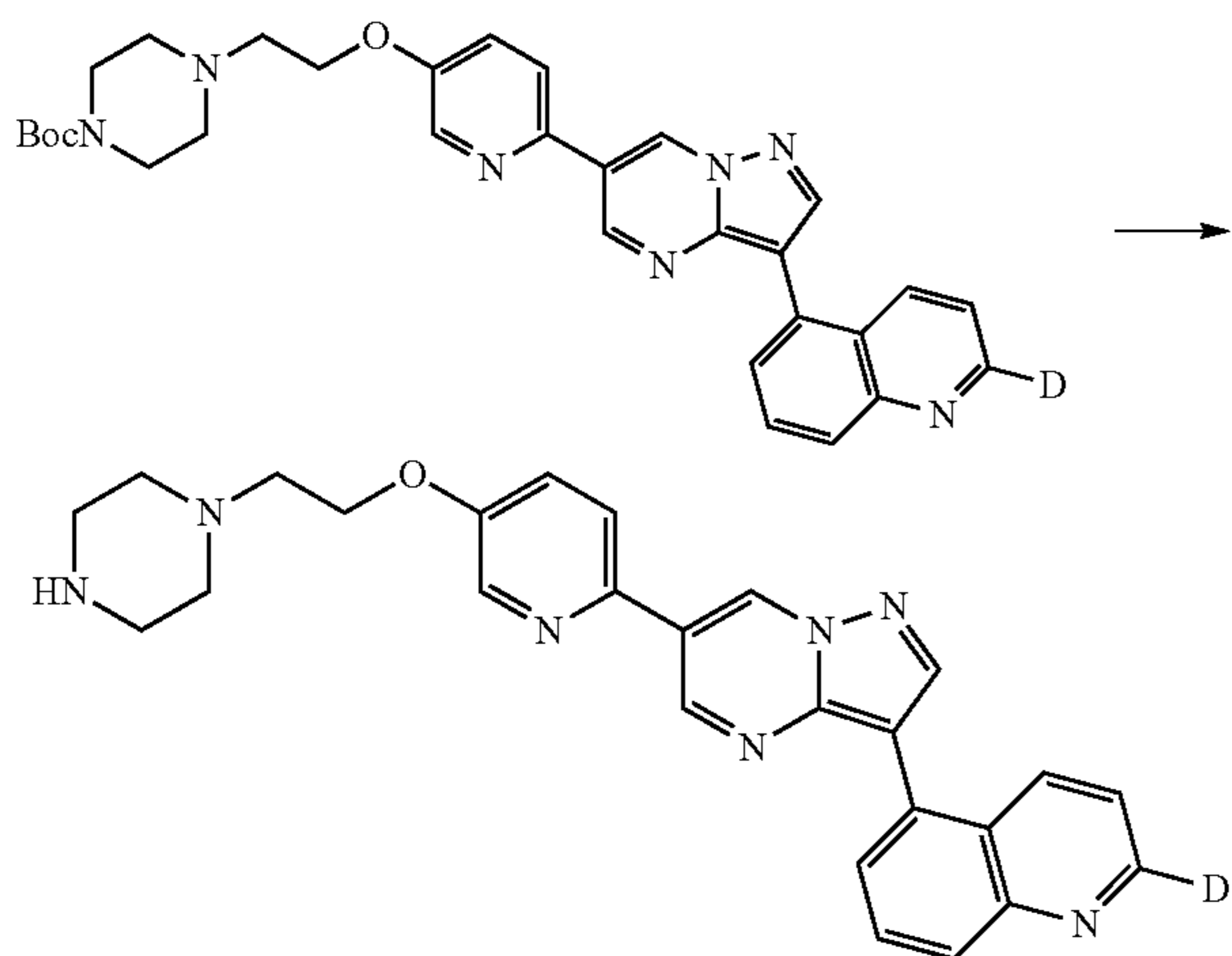
Scheme 176
