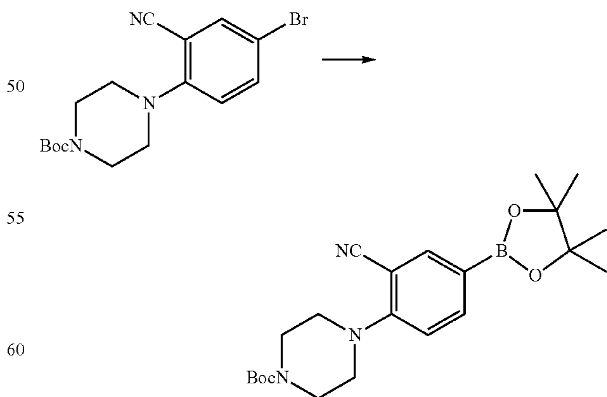
Scheme 133
