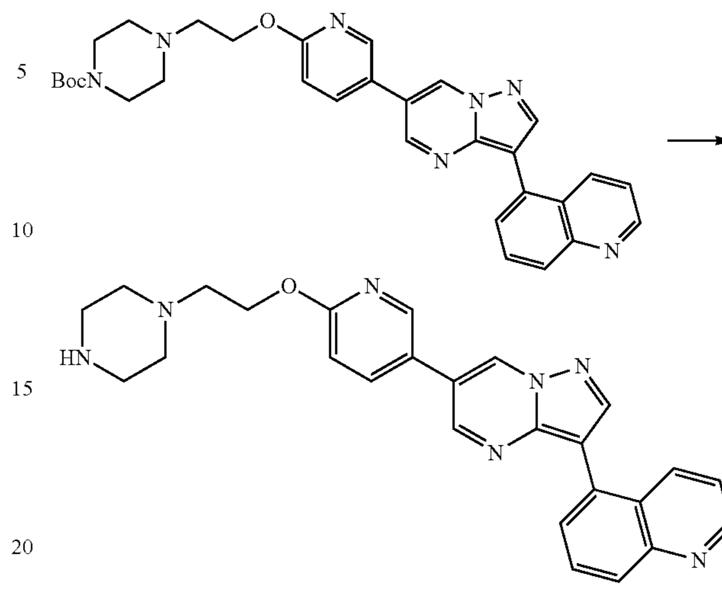
Scheme 156
