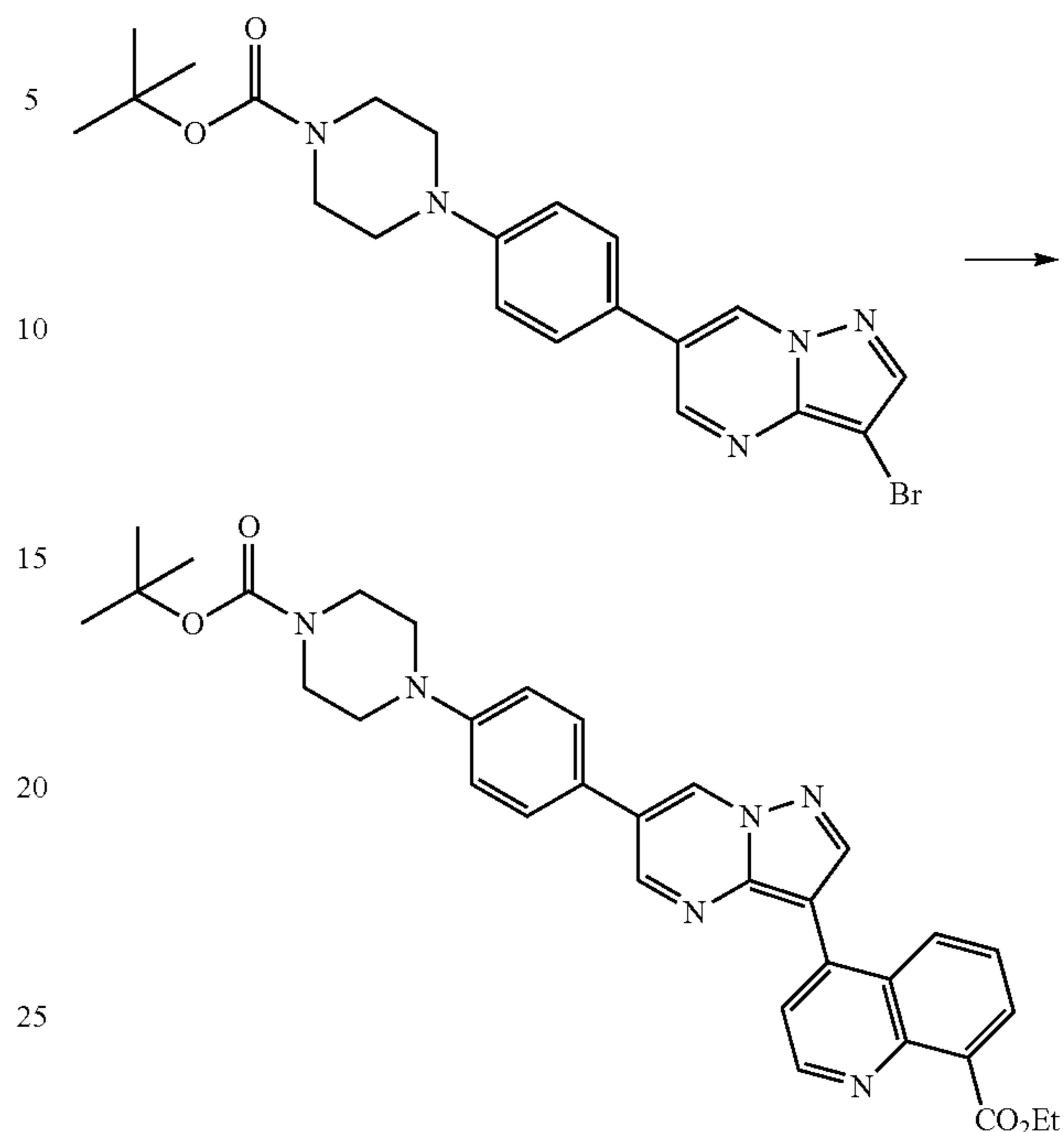
Scheme 72
