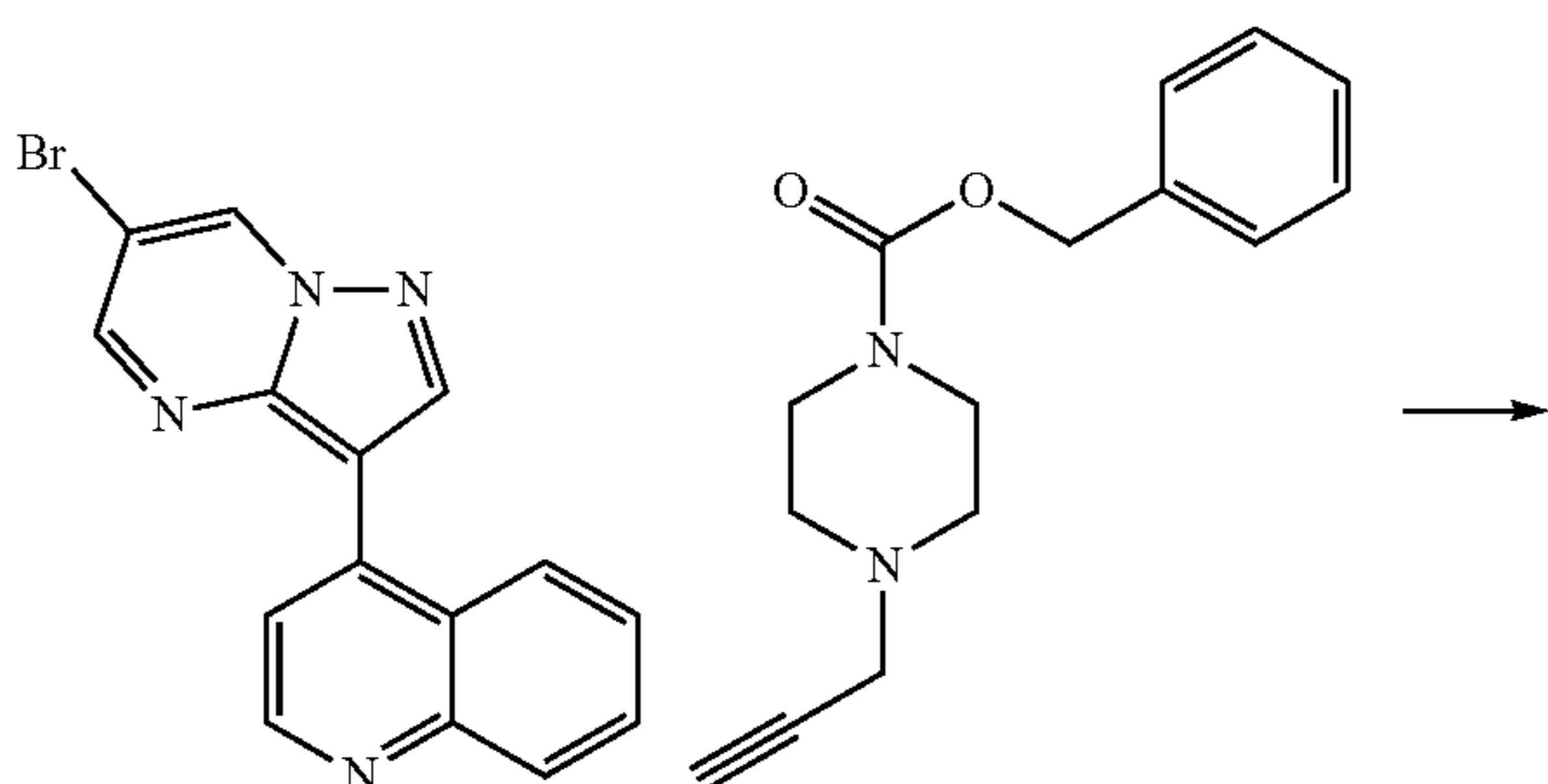
Scheme 10
