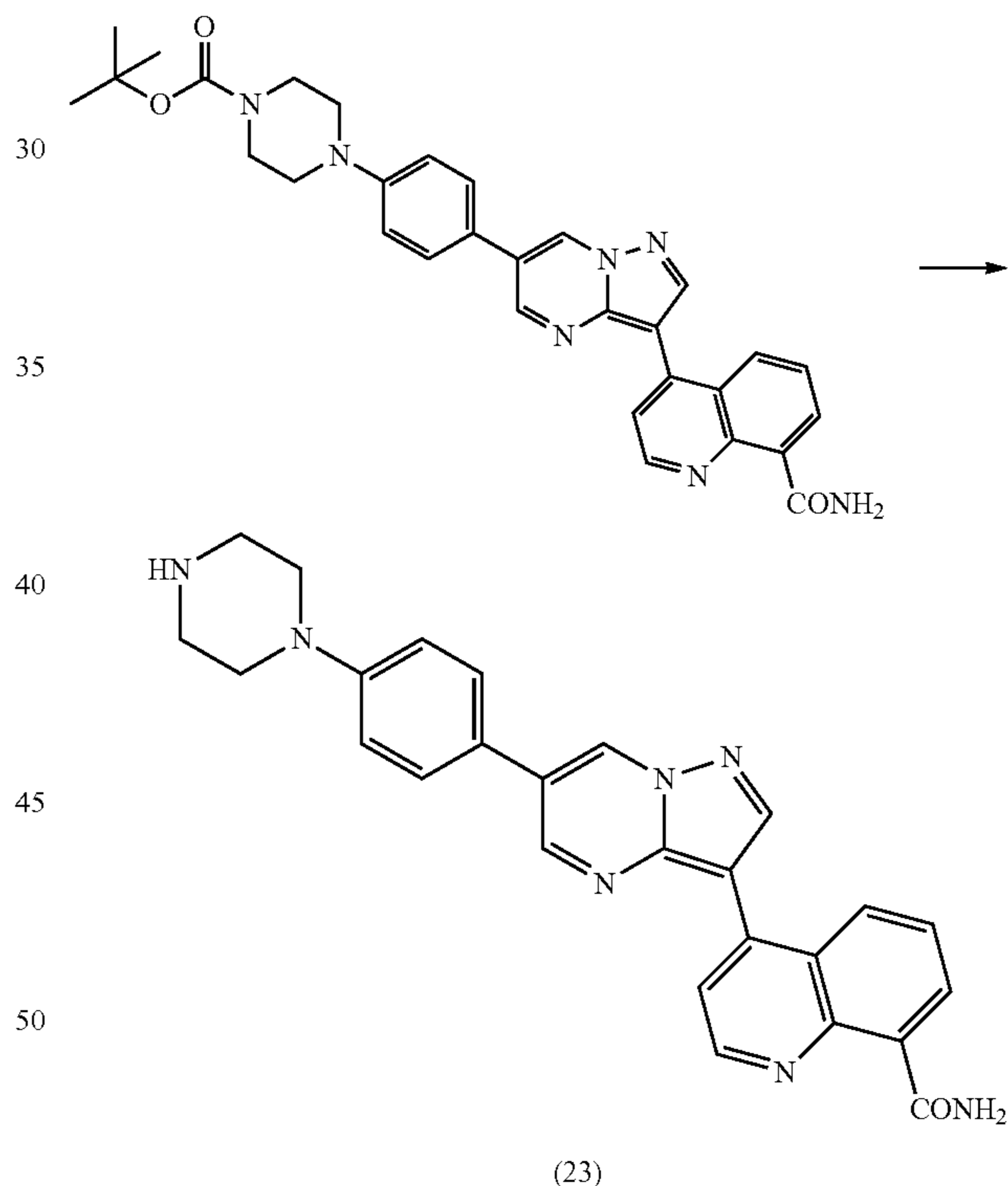
Scheme 76
