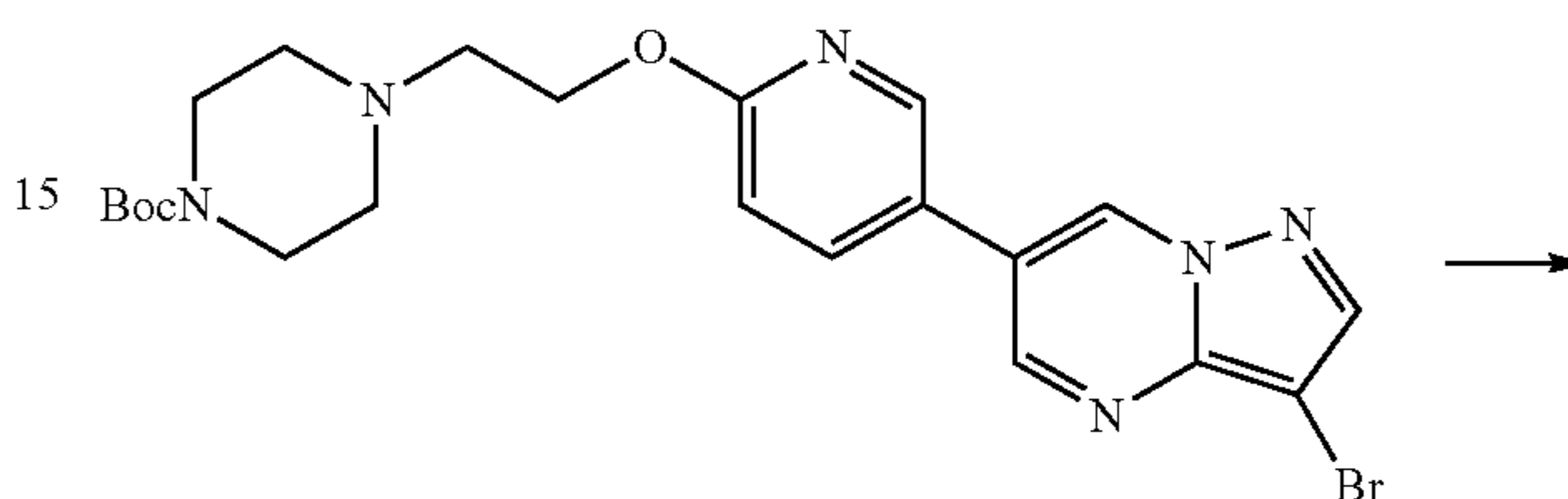
Scheme 153
