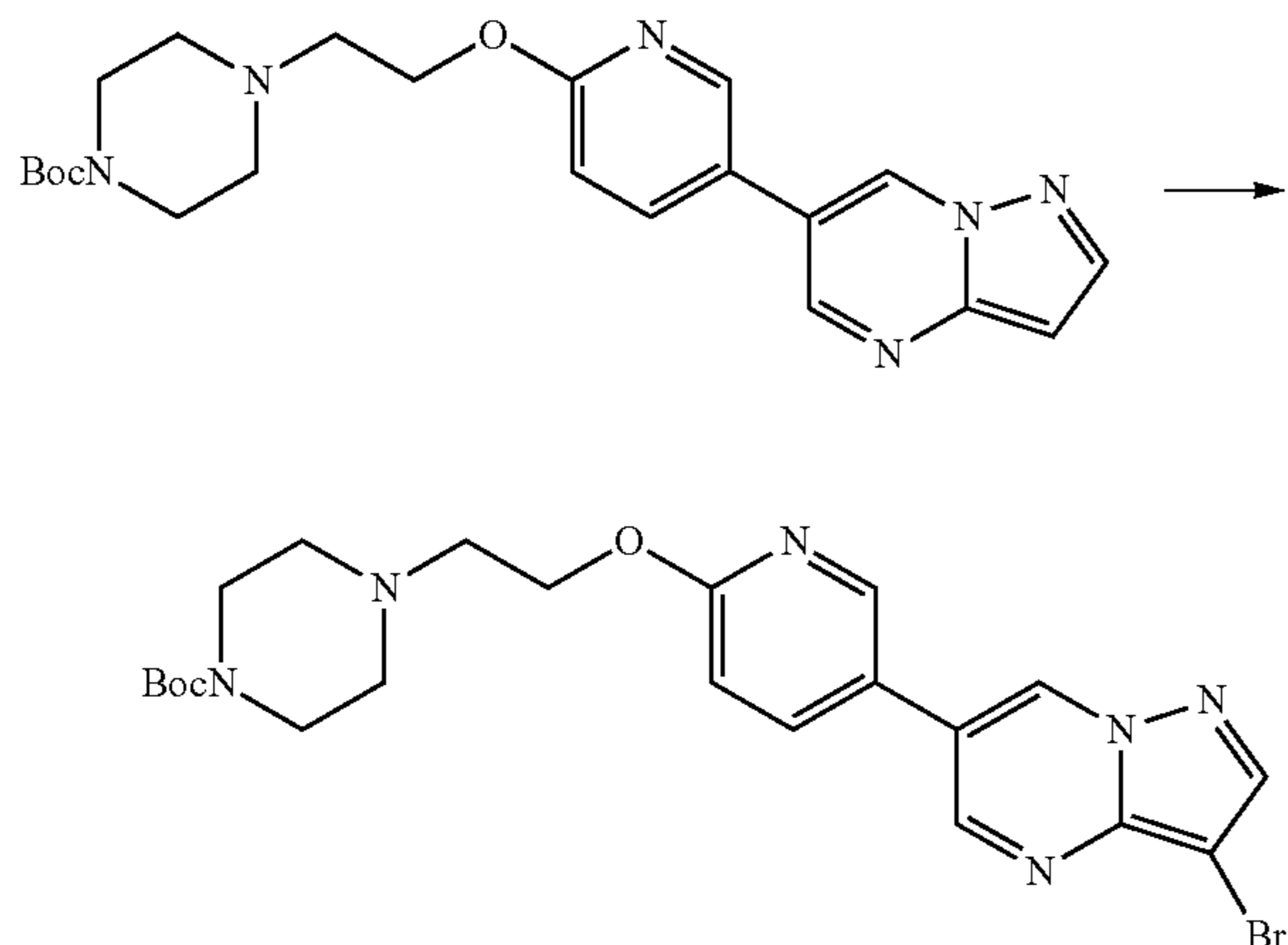
Scheme 152
