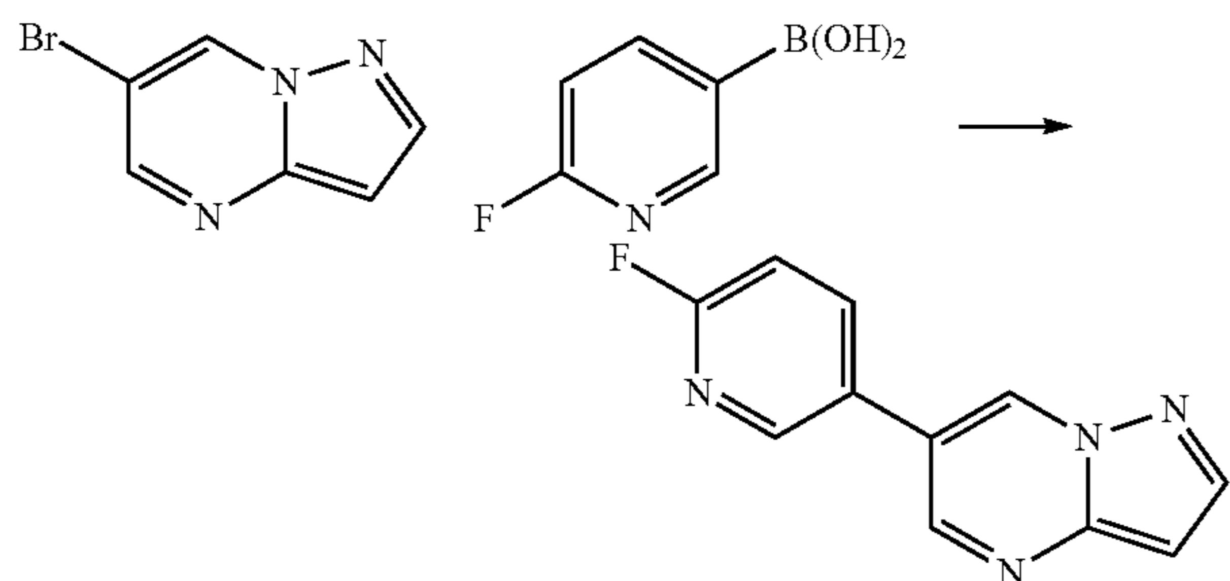
Scheme 96
