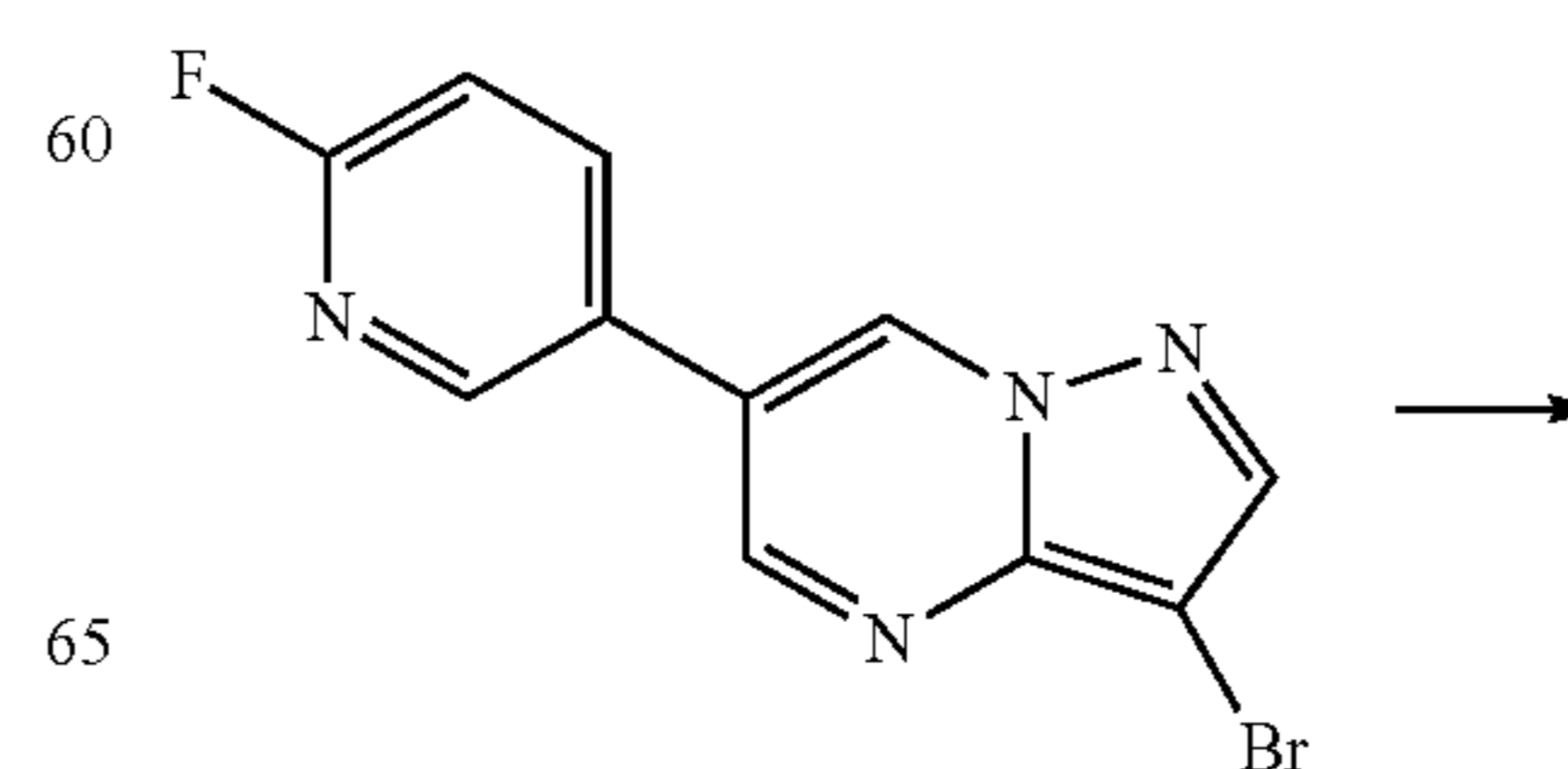
Scheme 98
