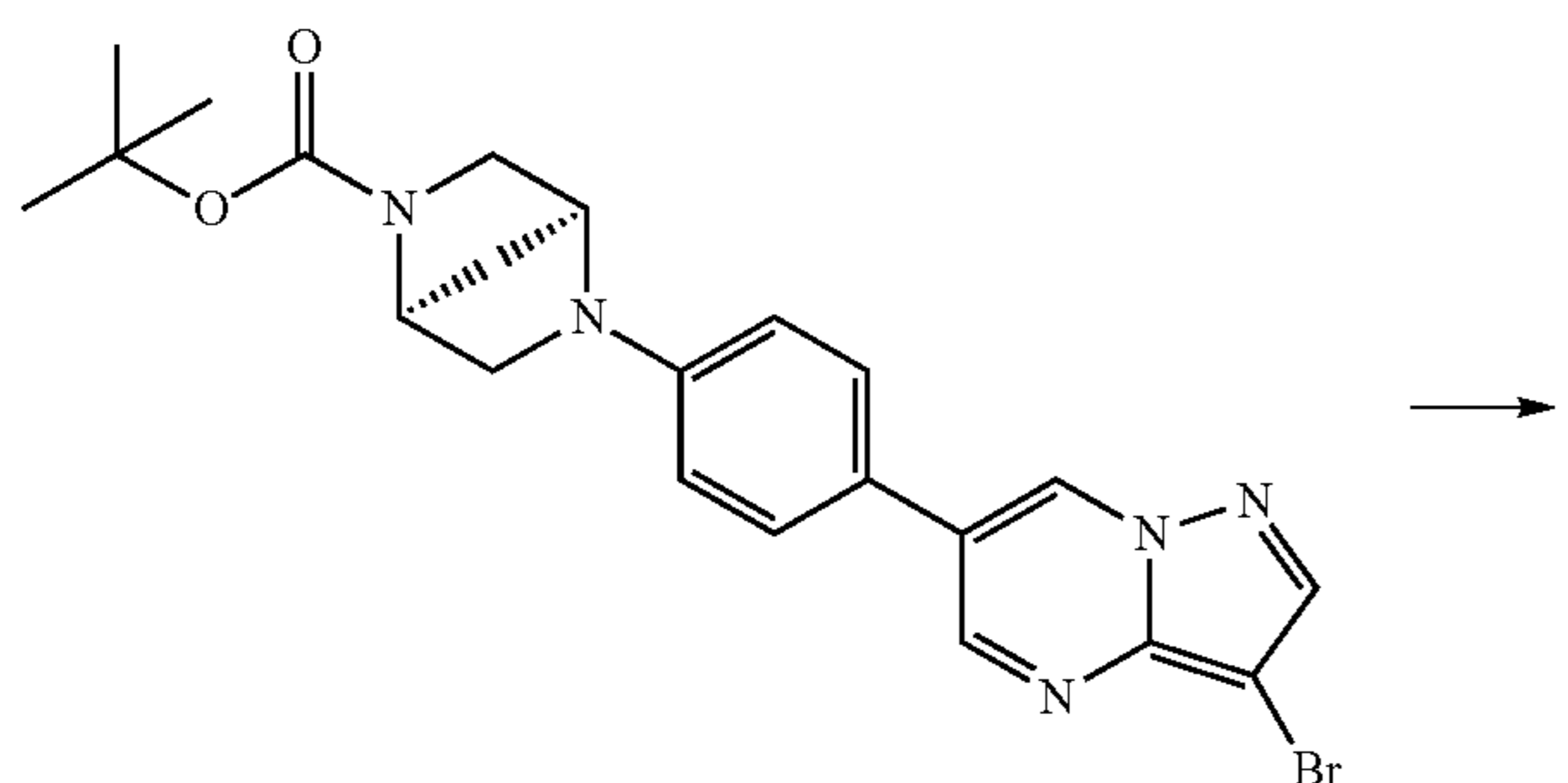
Scheme 16
