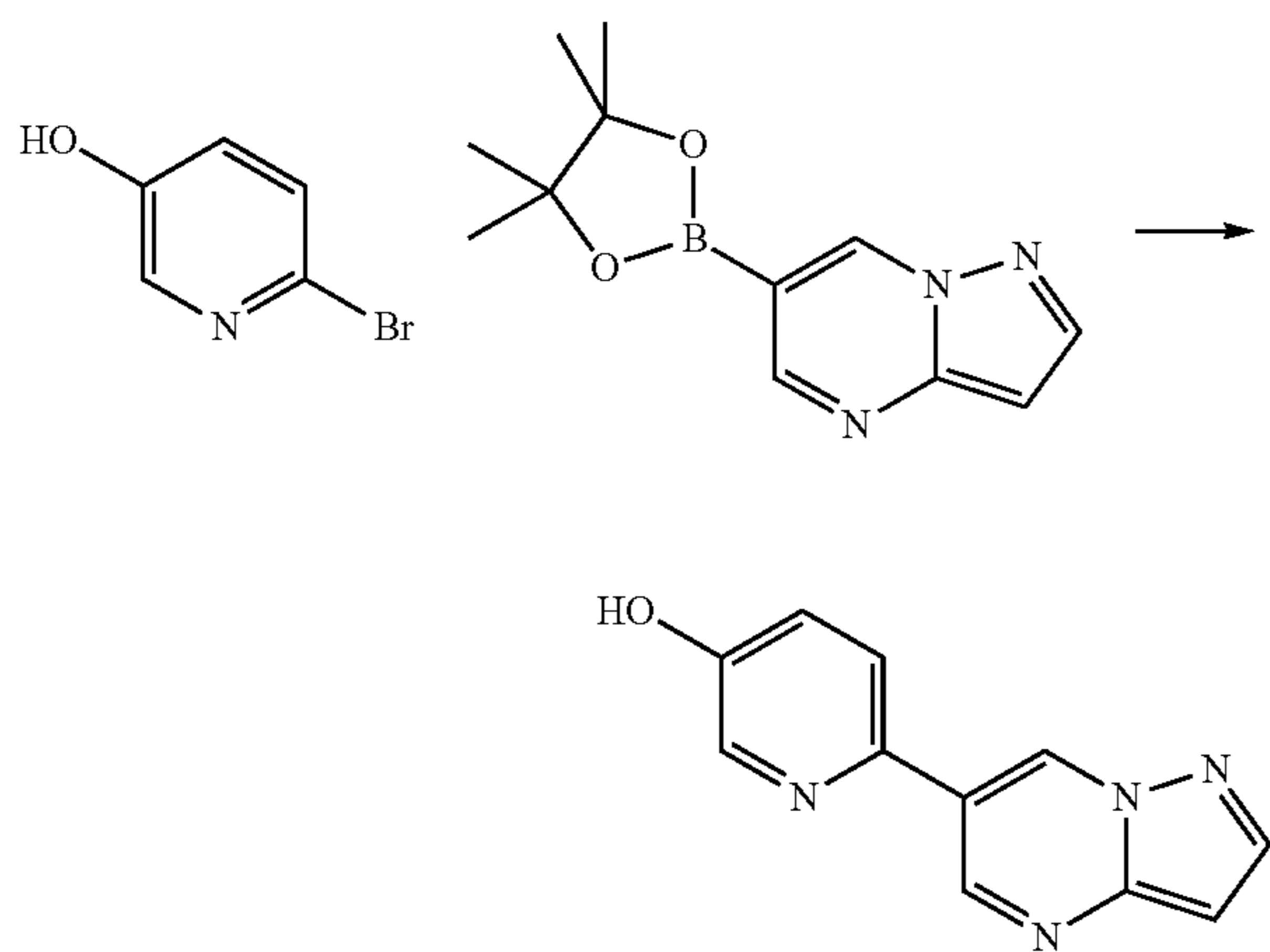
Scheme 167
