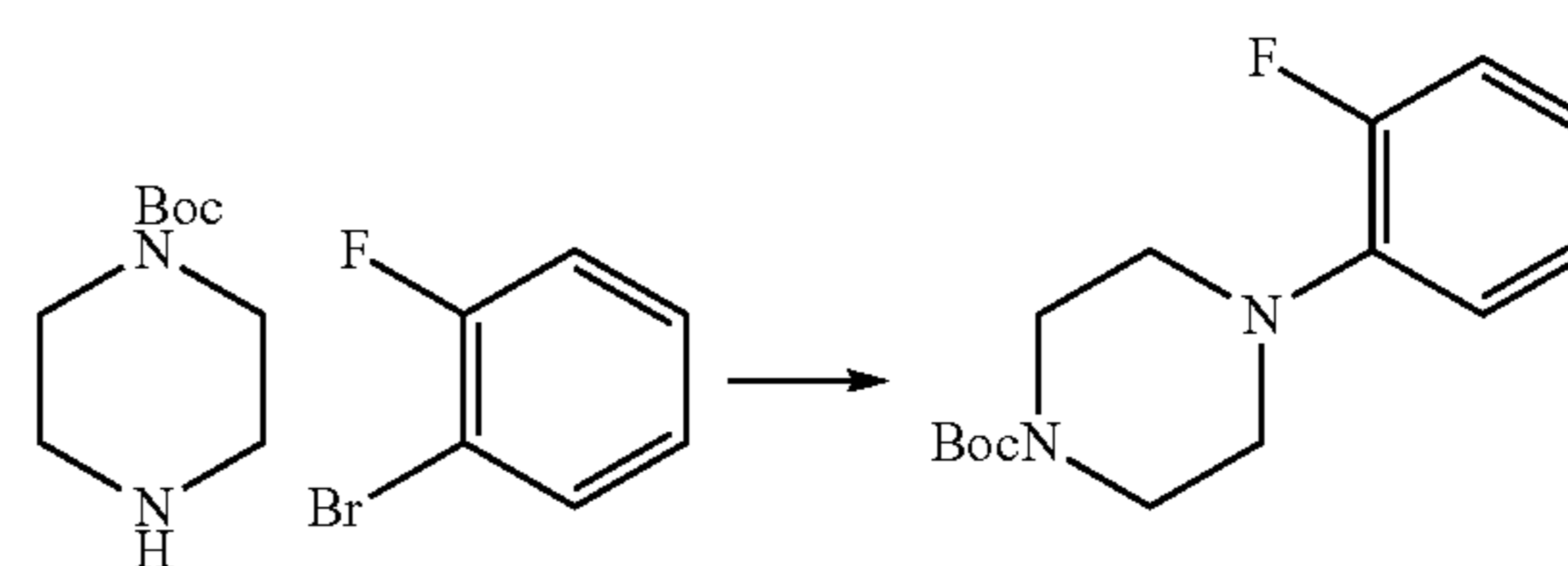
Scheme 140
