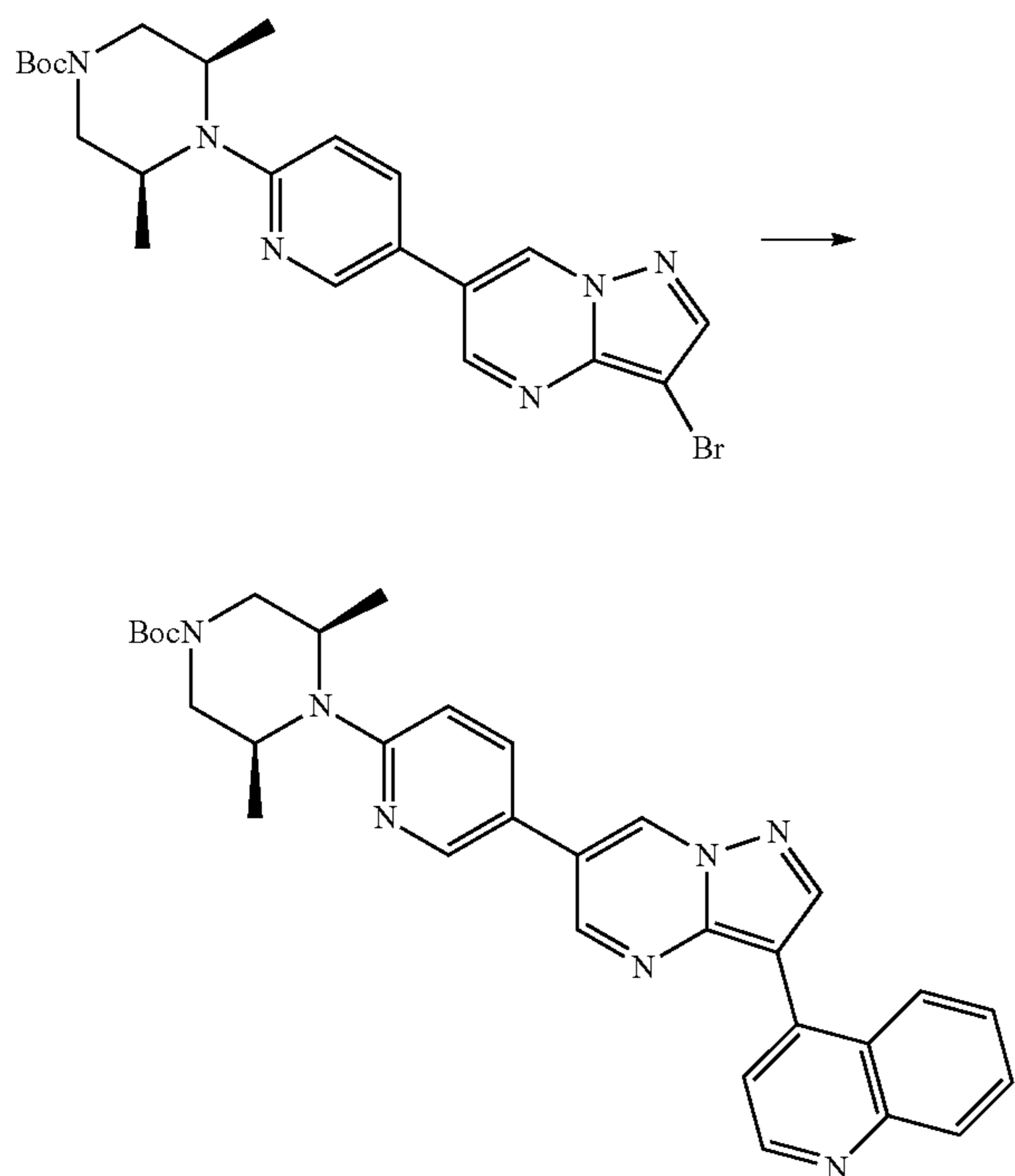
Scheme 118
